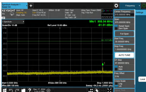
2DH5-Ant1-2480-30~1000-PASS
