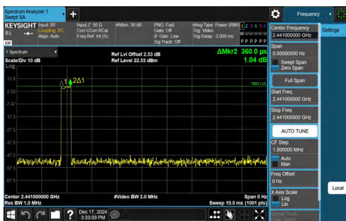
2DH3-Ant1-Hop-PASS
