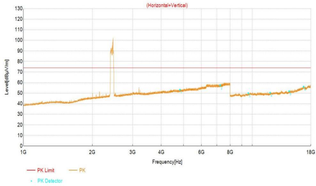
BT_3DH5_2480
