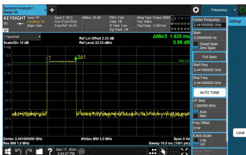
2DH5-Ant1-Hop-PASS
