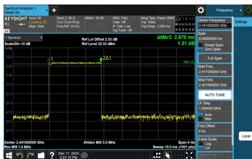
3DH5-Ant1-Hop-PASS
