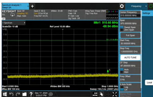
2DH5-Ant1-2402-30~1000-PASS
