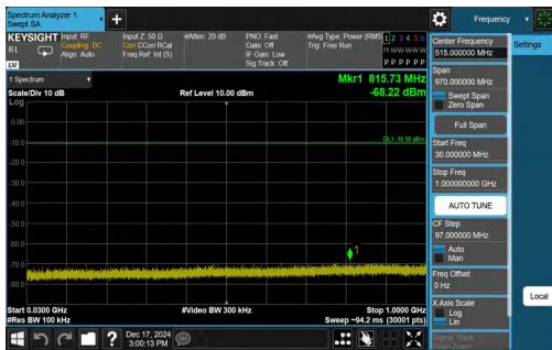
DH5-Ant1-2480-30~1000-PASS
