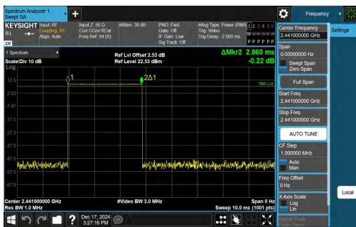
2DH1-Ant1-Hop-PASS
