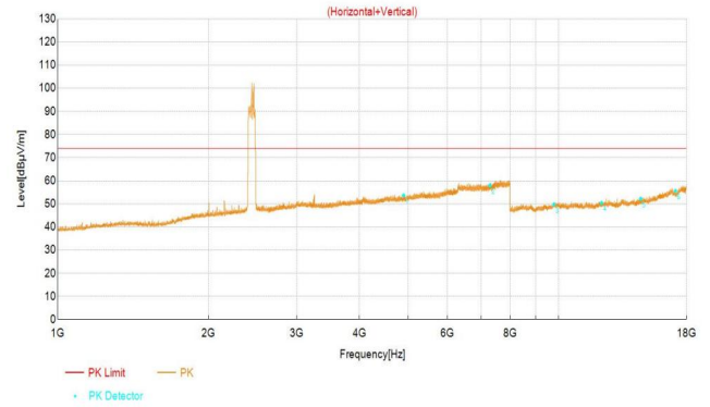
BT_DH5_2402
