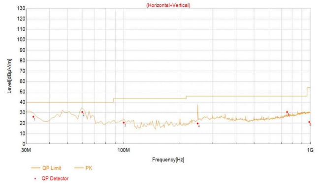
BT_DH5_2402
