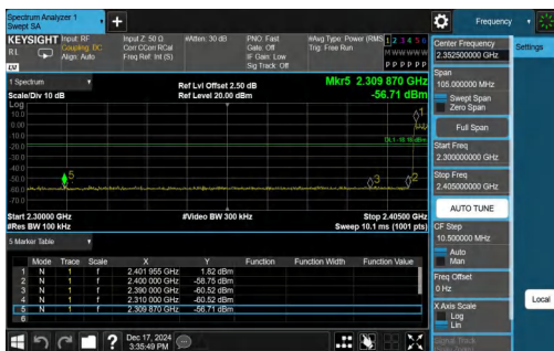
3DH5-Ant1-2402-PASS
