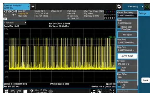
3DH1-Ant1-Hop-PASS
