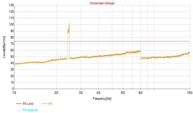
BT_3DH5_2480
