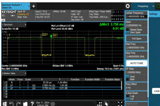
NTNV-3DH5-Ant1-2480
