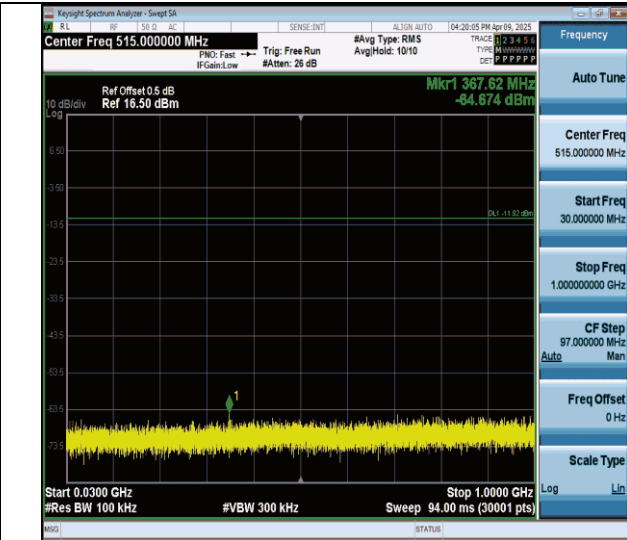
DH5-Ant0-2480-30~1000-PASS
