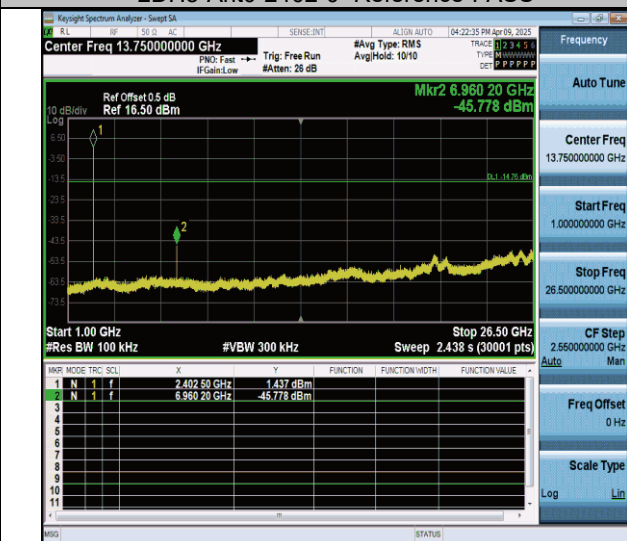
2DH5-Ant0-2402-1000~26500-PASS
