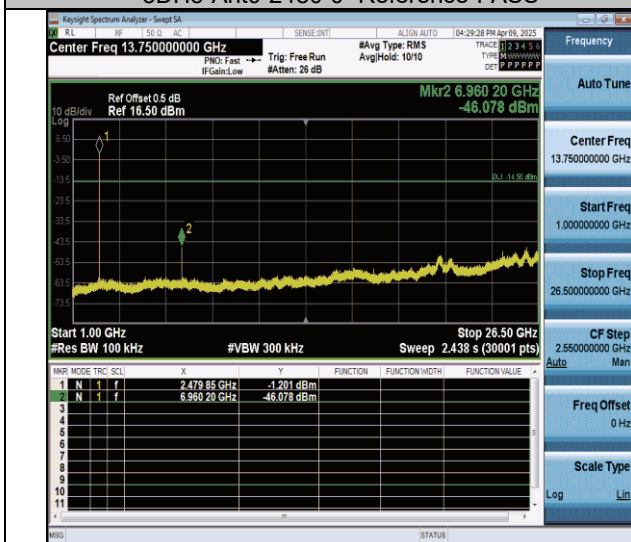
3DH5-Ant0-2480-1000~26500-PASS
