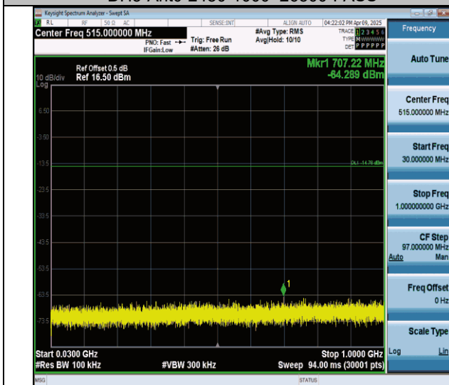
2DH5-Ant0-2402-30~1000-PASS
