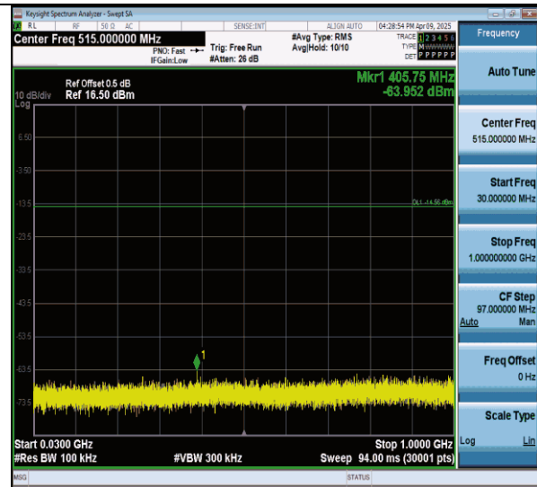
3DH5-Ant0-2480-30~1000-PASS
