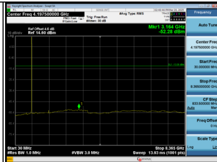
LTE Band 26_15MHz_CH26915 Spectrum Plot
