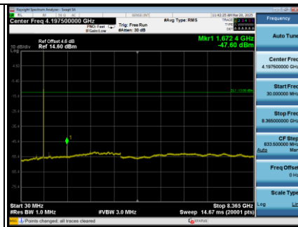
LTE Band 5_5MHz_CH20525 Spectrum Plot
