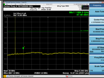
LTE Band 5_10M_CH20525 Spectrum Plot
