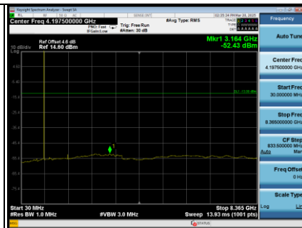
LTE Band 26_5MHz_CH26915 Spectrum Plot
