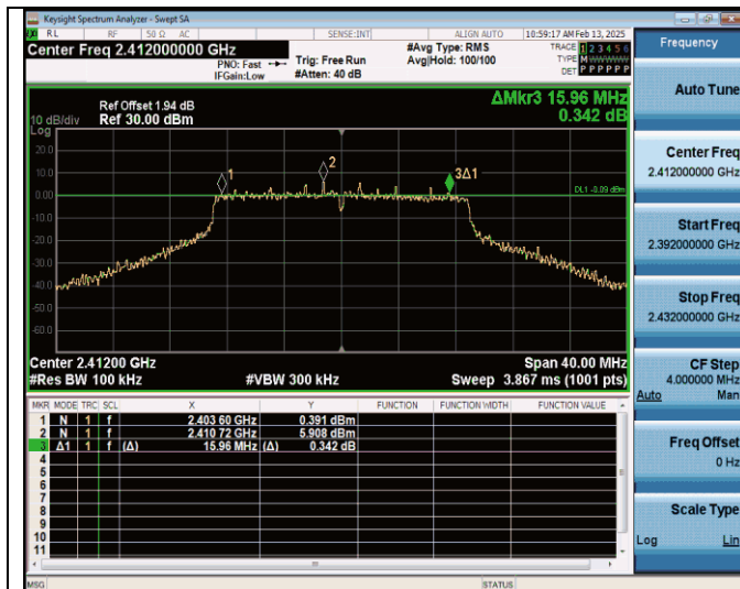
11n20SISO-Ant0-2412-PASS
