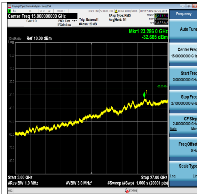
Band41-20MHz-QPSK-40620-1RB#0-3000~27000-PASS
