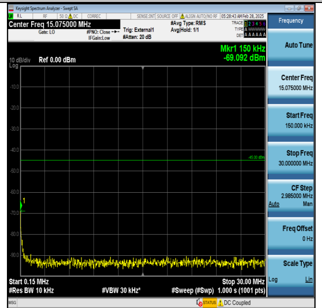
Band41-20MHz-QPSK-41490-1RB#0-0.15~30-PASS
