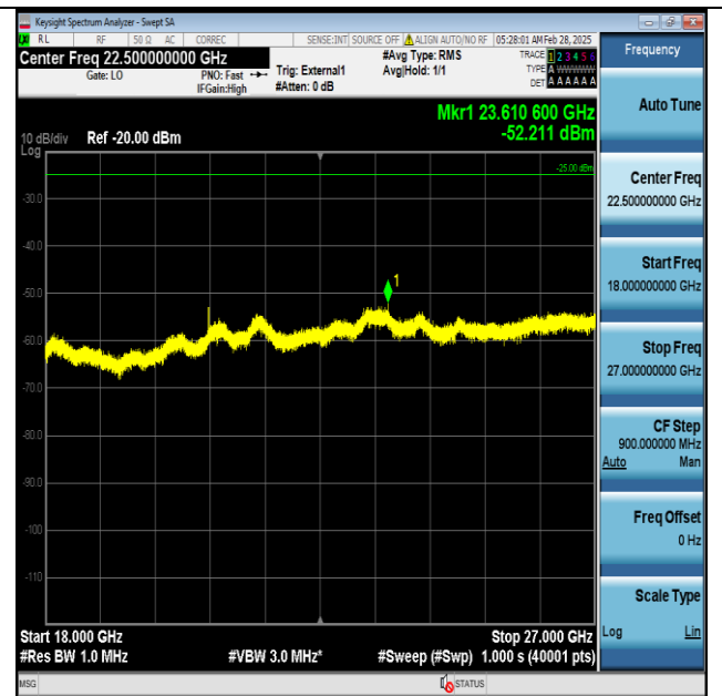
Band41-20MHz-QPSK-40620-1RB#0-18000~27000-PASS
