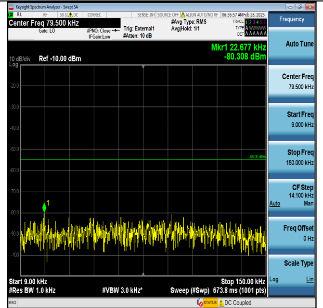
Band41-20MHz-QPSK-40620-1RB#0-0.009~0.15-PASS
