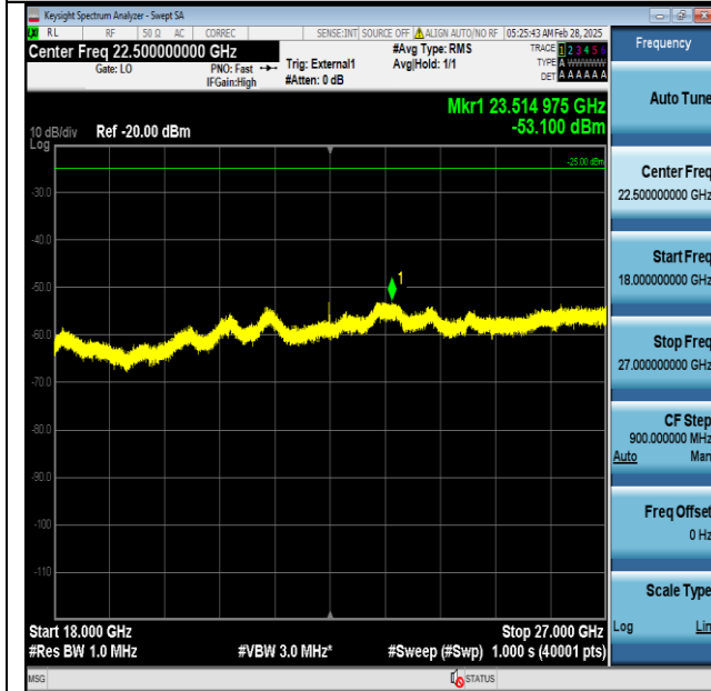
Band41-20MHz-QPSK-39750-1RB#0-18000~27000-PASS
