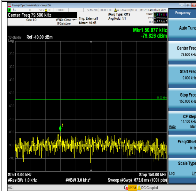
Band41-20MHz-QPSK-41490-1RB#0-0.009~0.15-PASS
