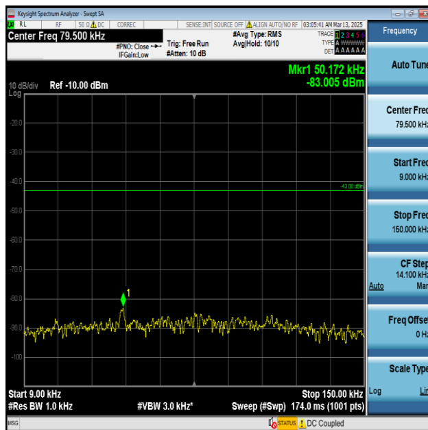
Band25-20MHz-QPSK-26590-1RB#0-0.009~0.15-PASS
