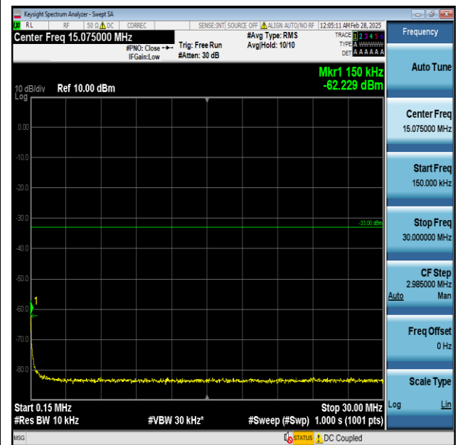
Band25-20MHz-QPSK-26590-1RB#0-0.15~30-PASS
