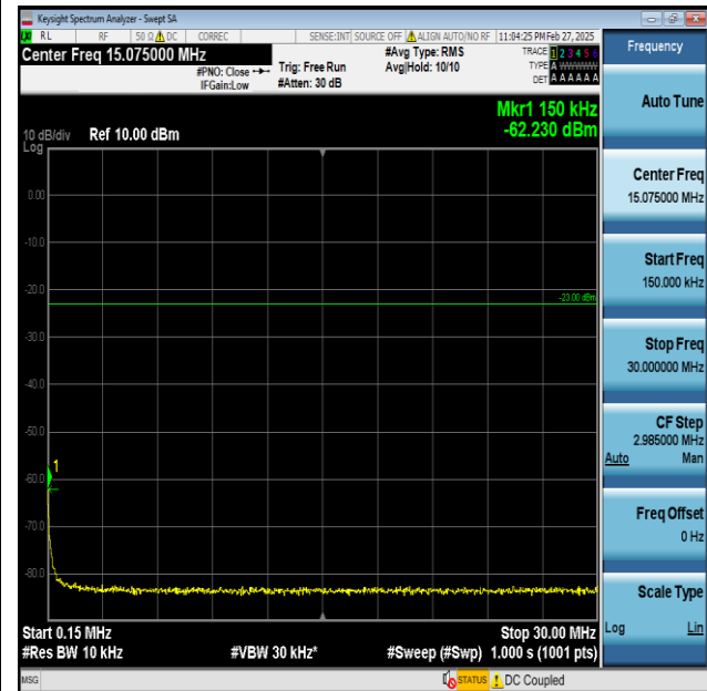
Band12-10MHz-QPSK-23130-1RB#0-0.15~30-PASS
