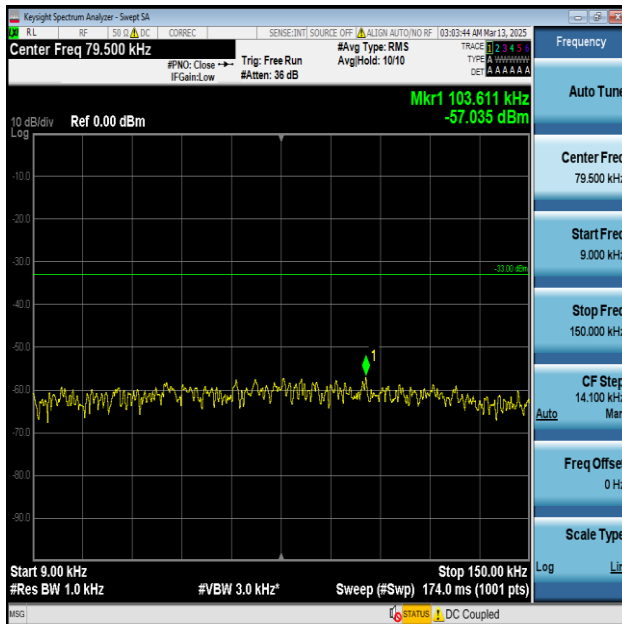
Band12-10MHz-QPSK-23130-1RB#0-0.009~0.15-PASS
