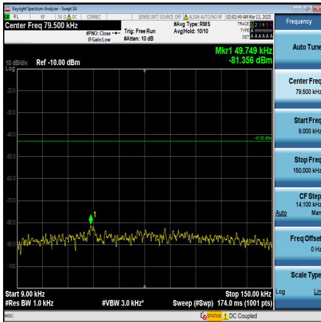
Band4-20MHz-QPSK-20300-1RB#0-0.009~0.15-PASS
