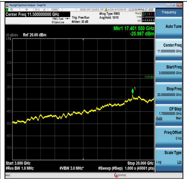
Band2-20MHz-QPSK-18900-1RB#0-3000~20000-PASS
