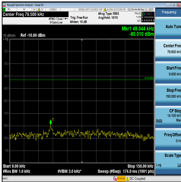
Band2-20MHz-QPSK-19100-1RB#0-0.009~0.15-PASS
