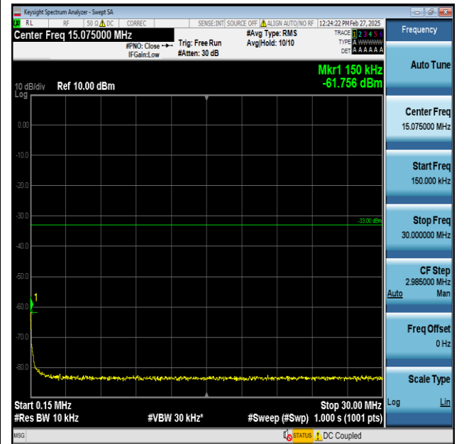
Band2-20MHz-QPSK-19100-1RB#0-0.15~30-PASS
