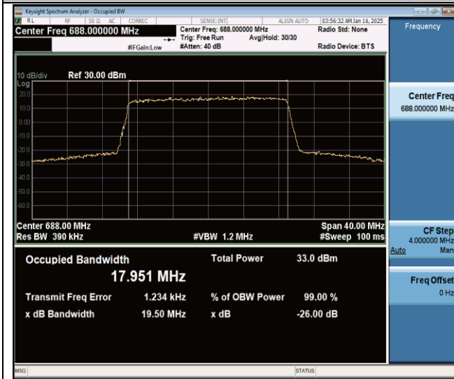
Band71-20MHz-QPSK-133372-100RB#0-PASS
