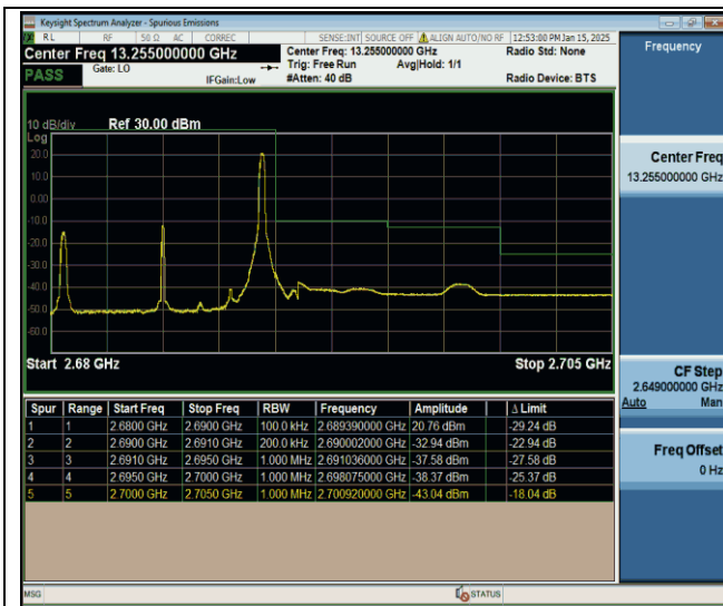
Band41-10MHz-QPSK-41540-1RB#49-PASS
