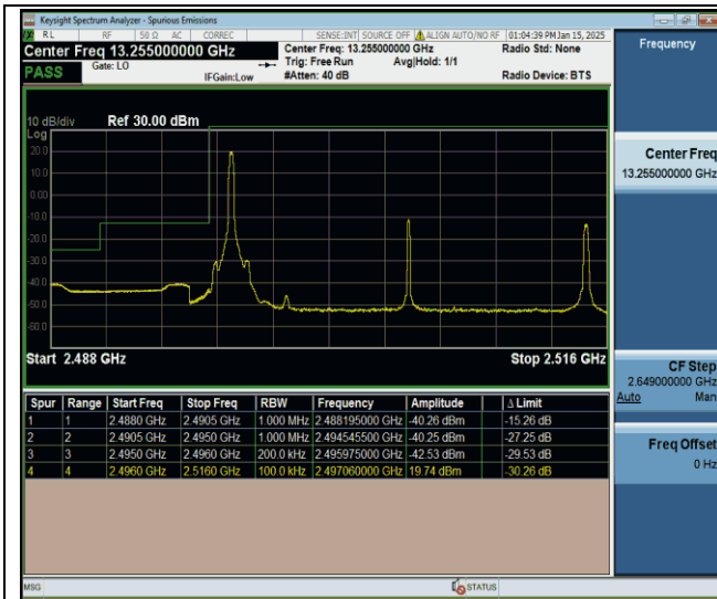
Band41-20MHz-QPSK-39750-1RB#0-PASS
