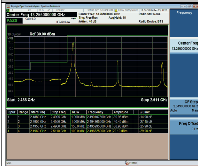
Band41-15MHz-QPSK-39725-1RB#0-PASS
