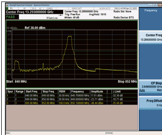
Band5-3MHz-QPSK-20635-1RB#14-PASS
