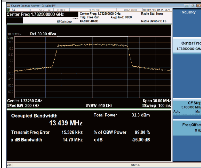
Band4-15MHz-QPSK-20175-75RB#0-PASS
