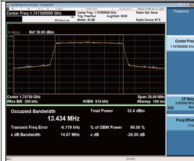
Band4-15MHz-QPSK-20325-75RB#0-PASS
