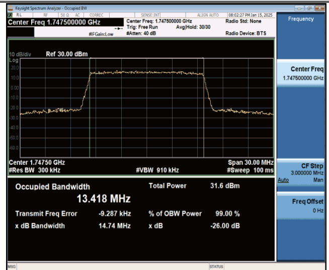
Band4-15MHz-16QAM-20325-75RB#0-PASS
