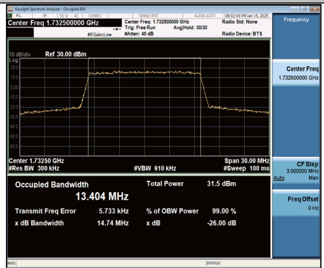
Band4-15MHz-16QAM-20175-75RB#0-PASS
