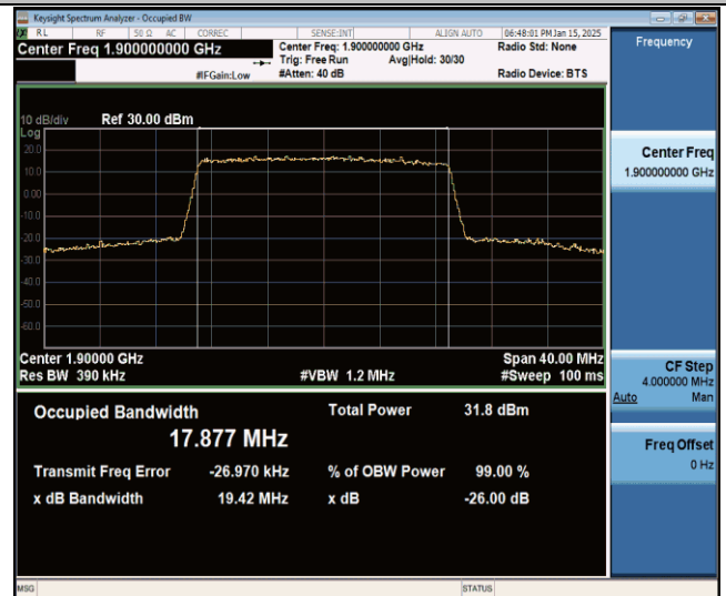
Band2-20MHz-16QAM-19100-100RB#0-PASS
