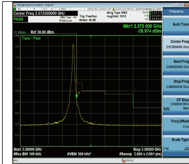
Band7-10MHz-QPSK-21400-1RB#49-PASS
