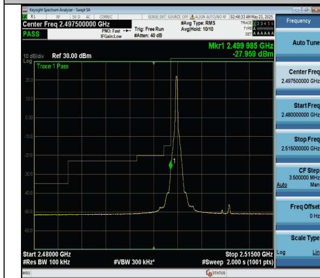
Band7-15MHz-QPSK-20825-1RB#0-PASS
