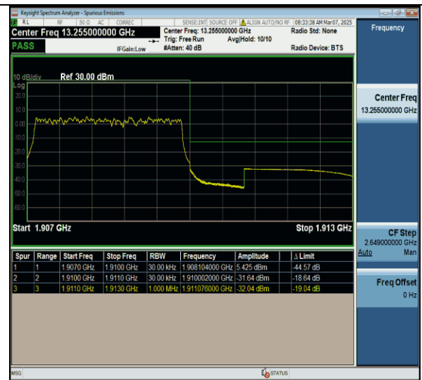
Band2-3MHz-QPSK-19185-15RB#0-PASS
