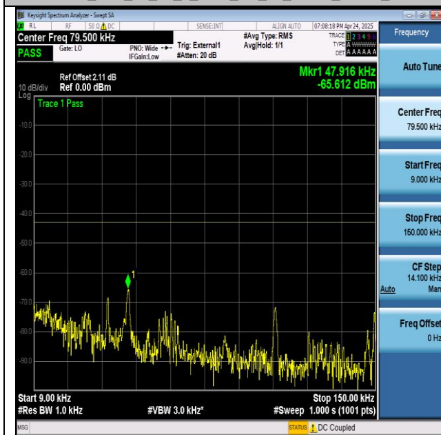
NTNV_N77-3700- 3980_PC2_30_20_M_TID1_NS_01_0.009_0.15_#1
