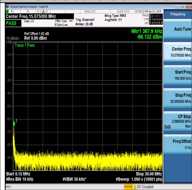
NTNV_N77-3700- 3980_PC2_30_20_M_TID1_NS_01_0.15_30_#1
