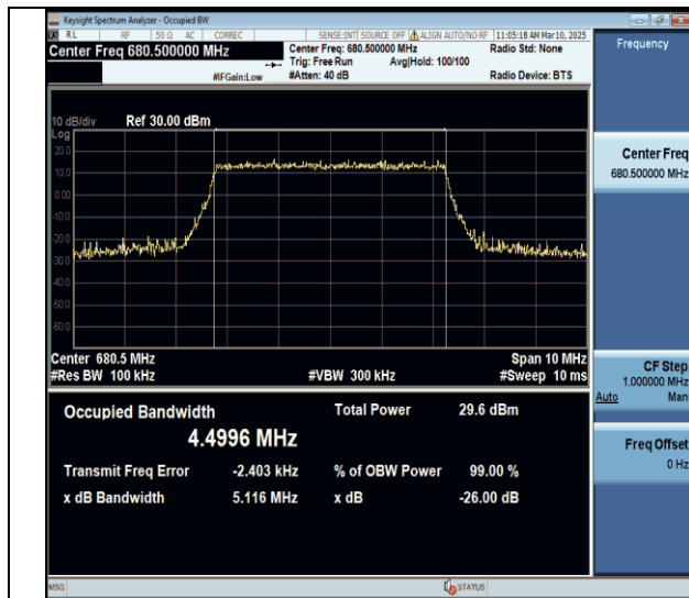
Band71-5MHz-64QAM-133297-25RB#0-PASS
