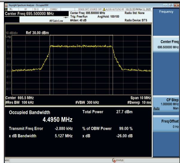
Band71-5MHz-256QAM-133447-25RB#0-PASS
