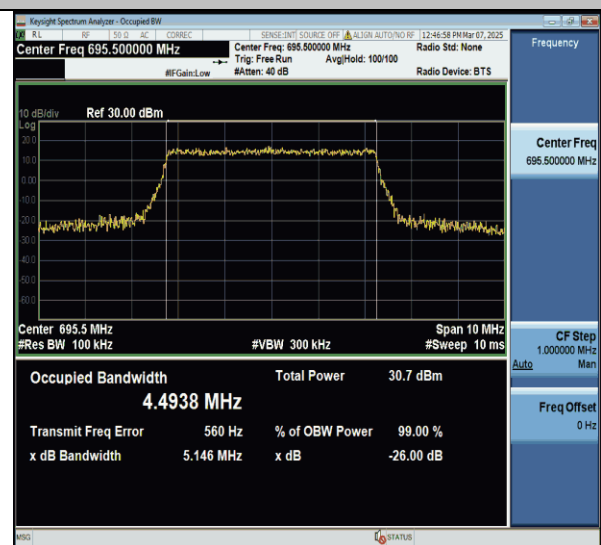
Band71-5MHz-16QAM-133447-25RB#0-PASS
