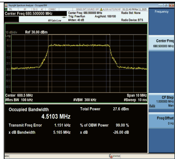
Band71-5MHz-256QAM-133297-25RB#0-PASS
