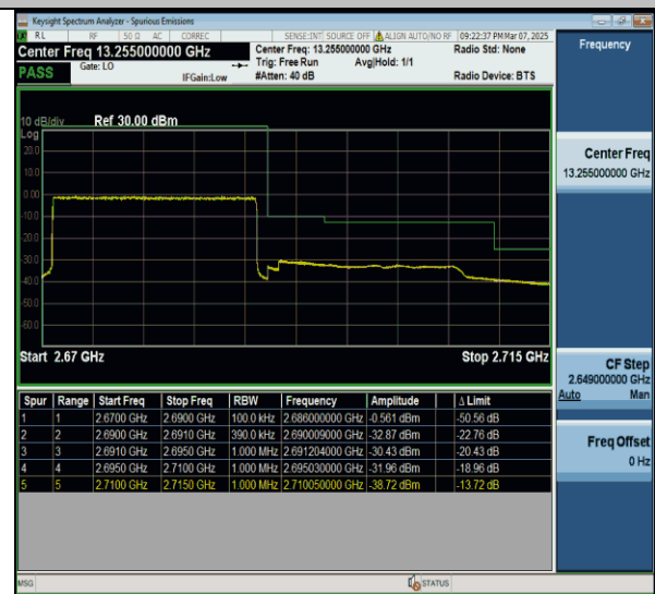
Band41-20MHz-QSPK-41490-100RB#0-PASS
