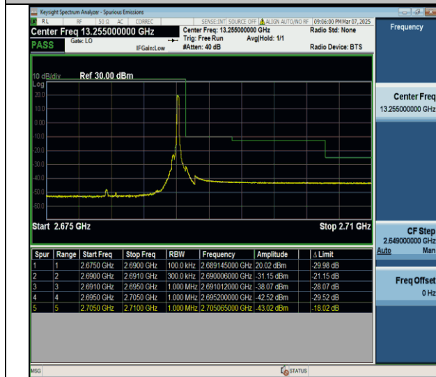
Band41-15MHz-QSPK-41515-1RB#74-PASS
