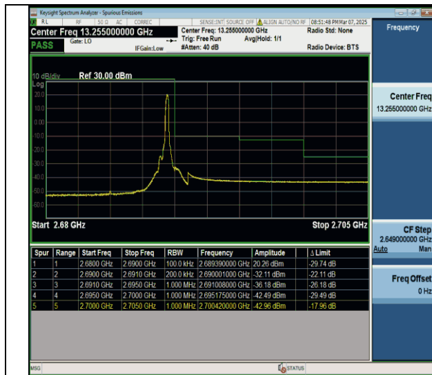
Band41-10MHz-QSPK-41540-1RB#49-PASS
