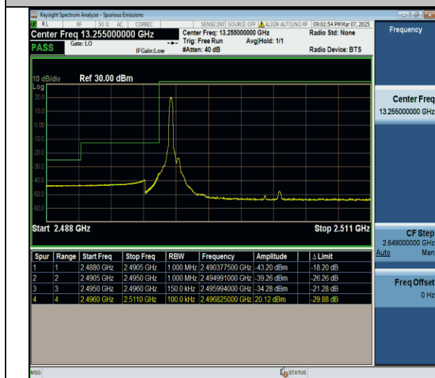
Band41-15MHz-QSPK-39725-1RB#0-PASS
