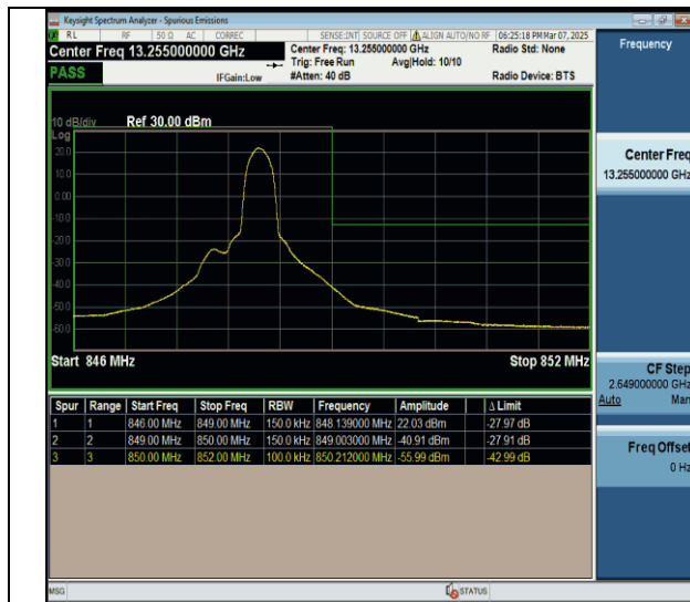
Band26(824-849)-15MHz-QSPK-26965-1RB#74-PASS
