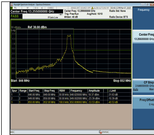
Band26(824-849)-3MHz-QSPK-27025-1RB#14-PASS
