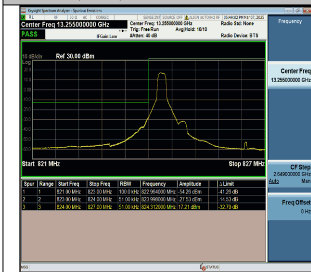
Band26(824-849)-5MHz-QSPK-26815-1RB#0-PASS
