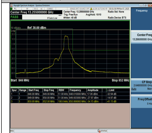
Band26(824-849)-5MHz-QSPK-27015-1RB#24-PASS
