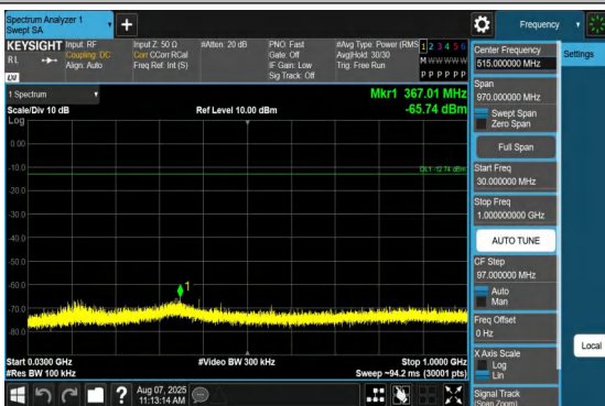
BLE_1M-Ant1-2480-0~Reference-PASS
