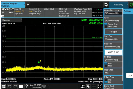
BLE_2M-Ant1-2440-0~Reference-PASS
