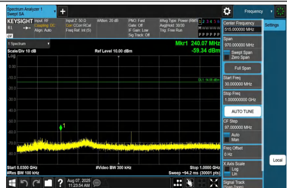
BLE_2M-Ant1-2480-0~Reference-PASS
