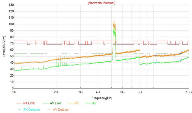
11AC_80M_5530
