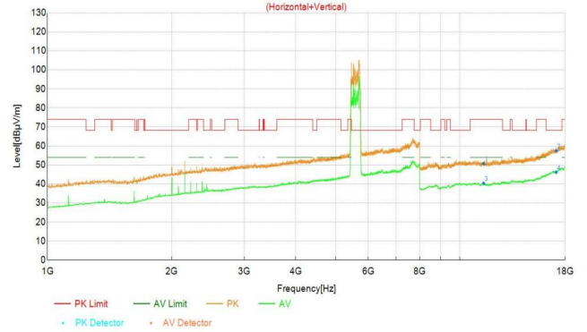
11N_40M_5795
