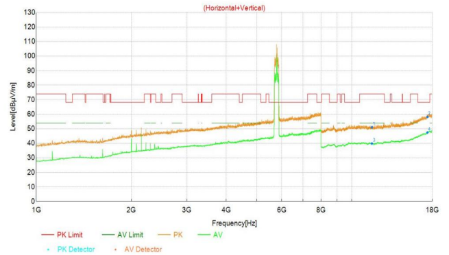
11AC_80M_5290
