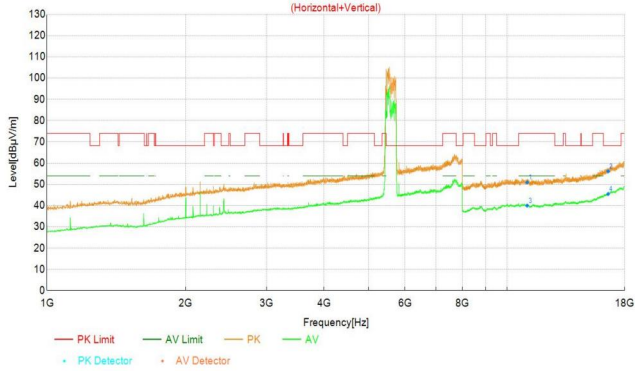
11AC_80M_5690
