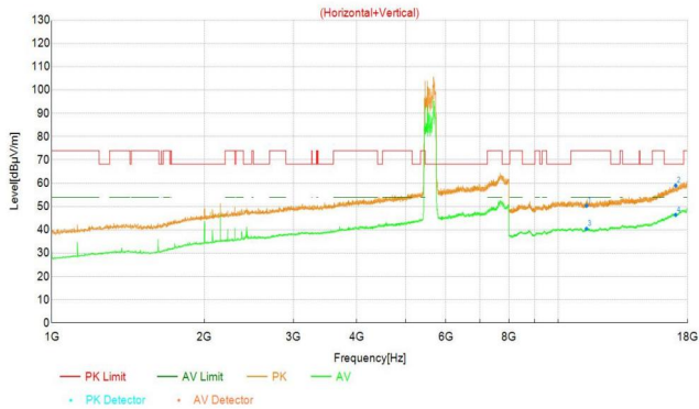
11AX_20M_5240
