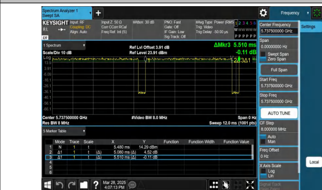
NTNV-11AX20MIMO-Ant2-5745-106Tone-RU53
