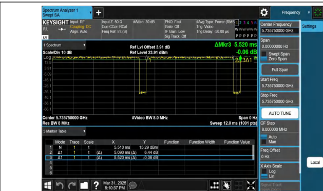
NTNV-11AX20MIMO-Ant2-5745-52Tone-RU37
