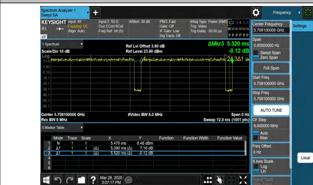
NTVN-11AX20MIMO-Ant2-5700-52Tone-RU40
