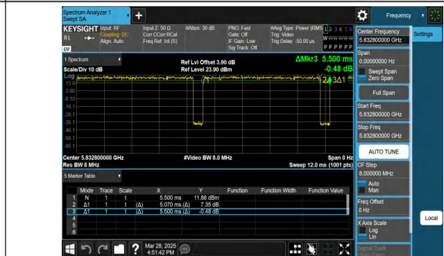
NTVN-11AX20MIMO-Ant2-5825-106Tone-RU54
