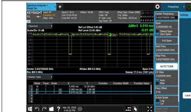
NTVN-11AX20MIMO-Ant1-5825-106Tone-RU54
