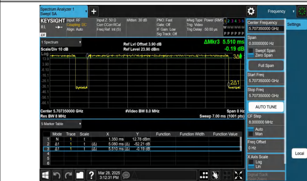
NTVN-11AX20MIMO-Ant2-5700-106Tone-RU54
