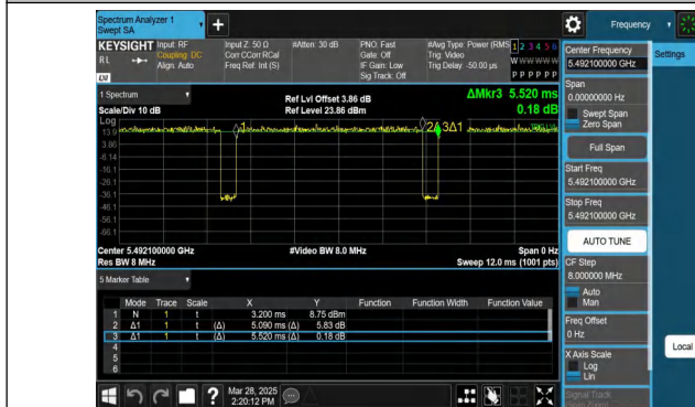
NTNV-11AX20MIMO-Ant1-5500-52Tone-RU37
