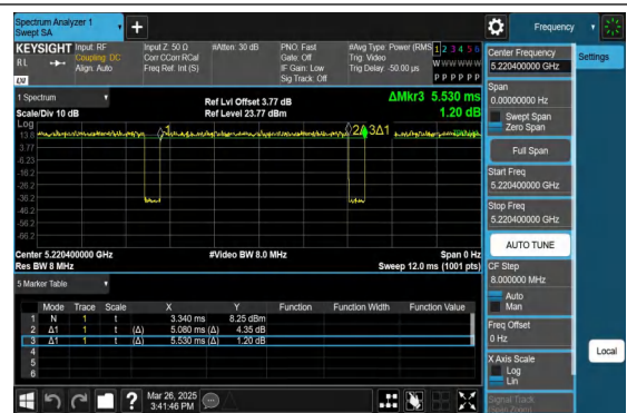
NTNV-11AX20MIMO-Ant2-5220-52Tone-RU39
