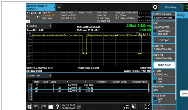
NTNV-11AX20MIMO-Ant1-5320-52Tone-RU40
