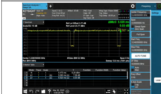
NTNV-11AX20MIMO-Ant1-5240-52Tone-RU40
