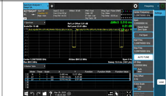
NTVN-11AX20MIMO-Ant2-5300-106Tone-RU53
