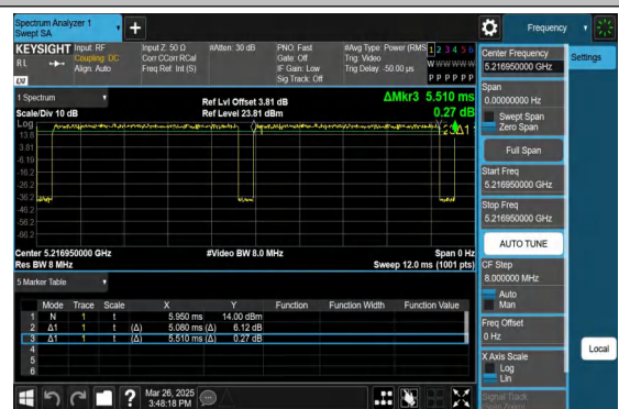
NTNV-11AX20MIMO-Ant2-5220-106Tone-RU53
