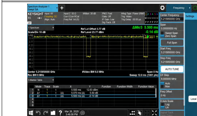
NTNV-11AX20MIMO-Ant1-5220-106Tone-RU53
