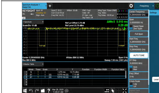
NTVN-11AX20MIMO-Ant1-5300-106Tone-RU53
