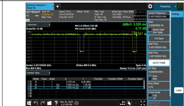
NTNV-11AX20MIMO-Ant2-5500-52Tone-RU37
