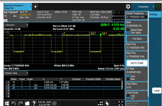
NTNV-11AX20MIMO-Ant2-5180
