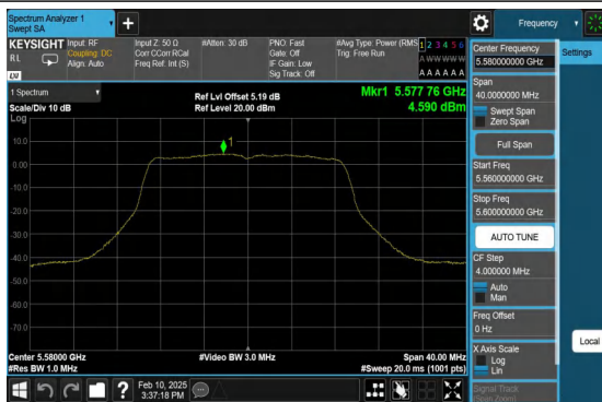
11AC20MIMO-Ant1-5700-PASS
