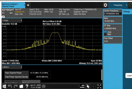
11AX20MIMO-Ant1-5785-52Tone-RU39-PASS
