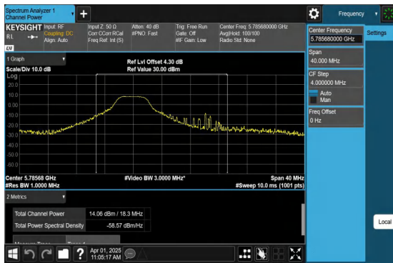
11AX20MIMO-Ant1-5785-106Tone-RU53-PASS
