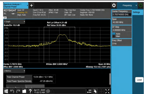
11AX20MIMO-Ant2-5785-52Tone-RU39-PASS
