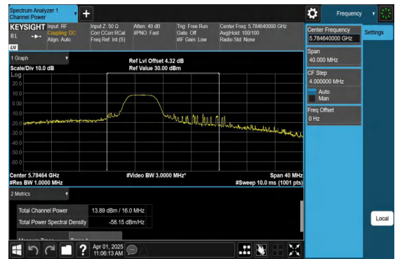
11AX20MIMO-Ant2-5785-106Tone-RU53-PASS
