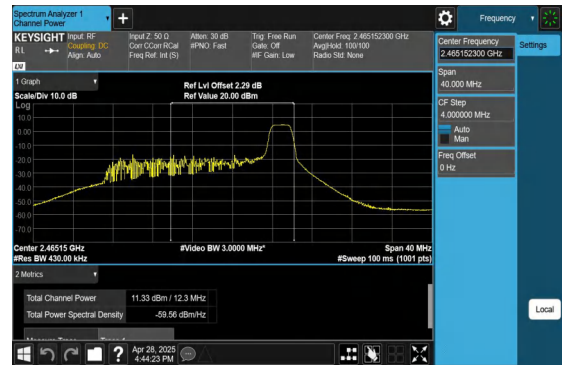
11AX20MIMO-Ant2-2462-52Tone-RU40-PASS
