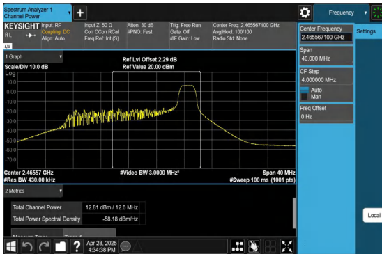
11AX20MIMO-Ant1-2462-52Tone-RU40-PASS
