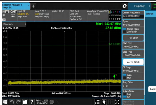
BLE_500K-Ant1-2480-30~1000-PASS
