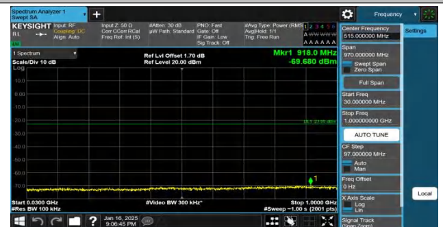
Band4-10MHz-QPSK-20000-50RB#0-30~1000-PASS
