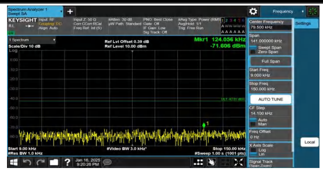
Band4-15MHz-QPSK-20175-75RB#0-0.009~0.15-PASS
