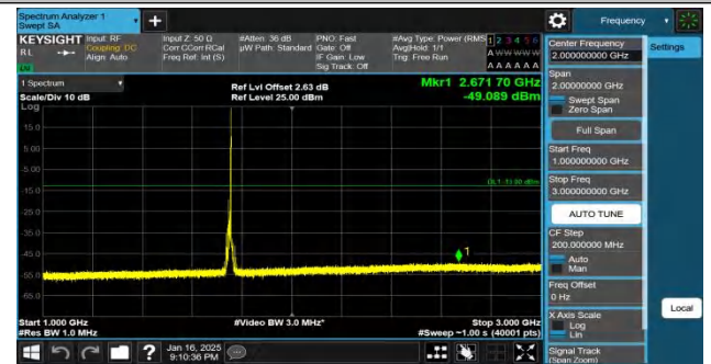
Band4-10MHz-QPSK-20350-1RB#49-1000~3000-PASS
