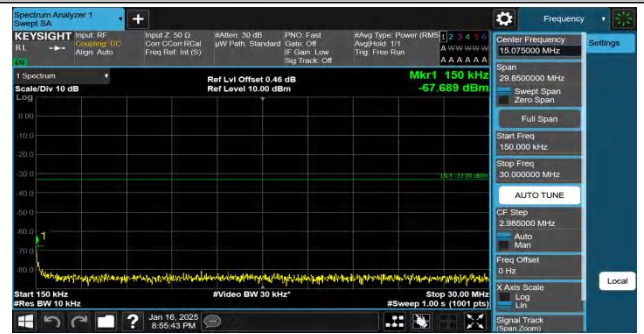
Band4-5MHz-QPSK-20175-1RB#0.15~30-PASS
