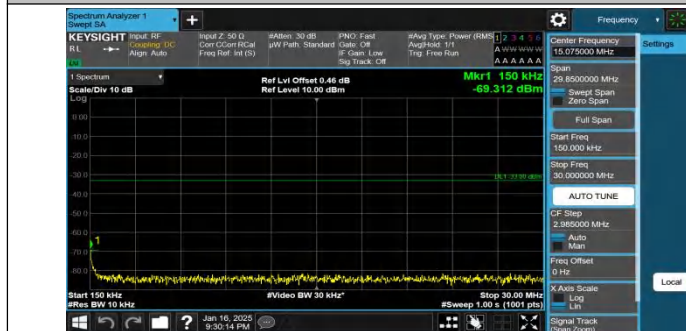
Band4-20MHz-QPSK-20175-1RB#99-0.15~30-PASS
