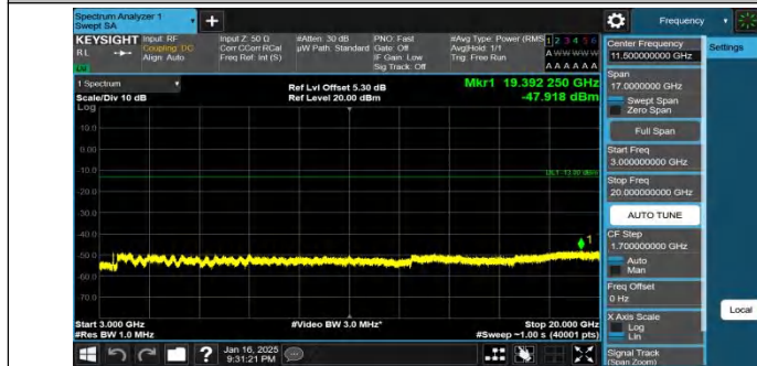
Band4-20MHz-QPSK-20175-100RB#0-3000~20000-PASS
