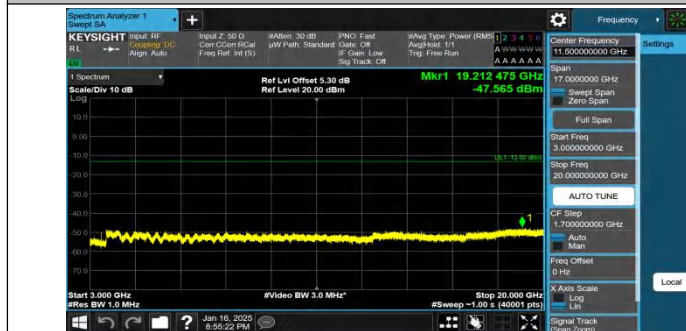
Band4-5MHz-QPSK-19975-25RB#0-3000~20000-PASS
