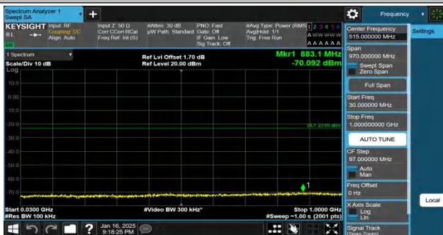
Band4-15MHz-QPSK-20025-75RB#0-30~1000-PASS
