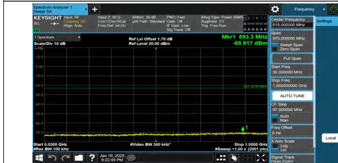
Band4-15MHz-QPSK-20325-75RB#0-30~1000-PASS
