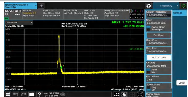
Band4-15MHz-QPSK-20025-75RB#0-1000~3000-PASS
