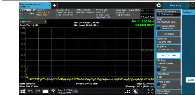
Band4-15MHz-QPSK-20175-75RB#0-0.15~30-PASS
