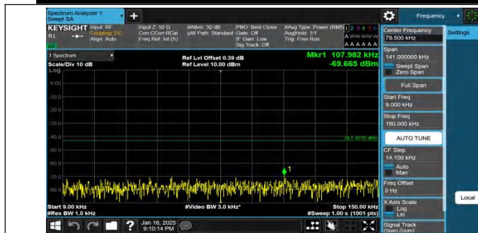
Band4-10MHz-QPSK-20350-1RB#49-0.009~0.15-PASS
