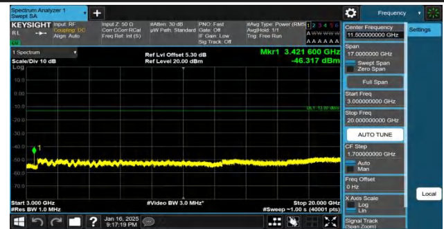
Band4-15MHz-QPSK-20025-1RB#0-3000~20000-PASS
