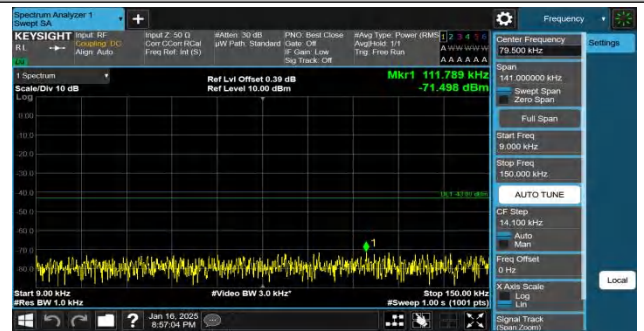
Band4-5MHz-QPSK-20175-25RB#0-0.009~0.15-PASS
