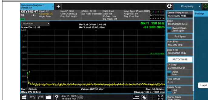
Band4-15MHz-QPSK-20025-1RB#0-0.15~30-PASS
