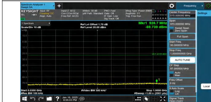
Band4-5MHz-QPSK-19975-25RB#0-30~1000-PASS
