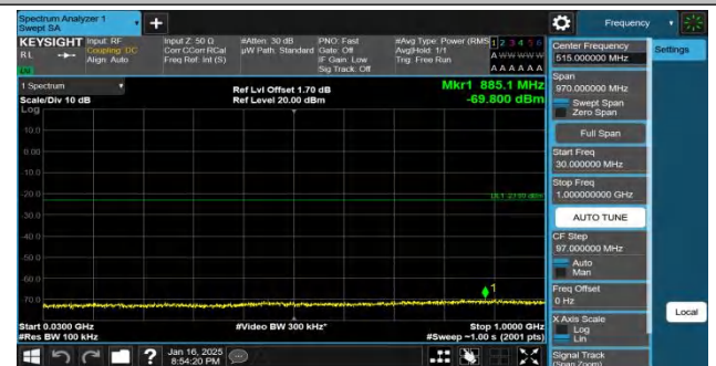
Band4-5MHz-QPSK-19975-1RB#24-30~1000-PASS
