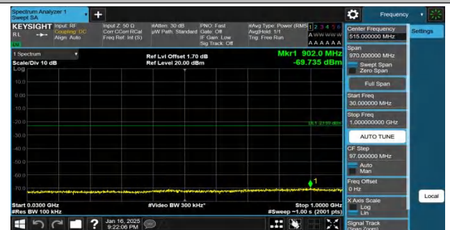
Band4-15MHz-QPSK-20325-1RB#74-30~1000-PASS
