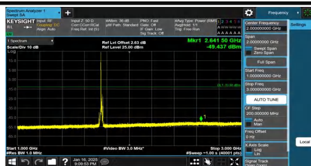
Band4-10MHz-QPSK-20350-1RB#0-1000~3000-PASS
