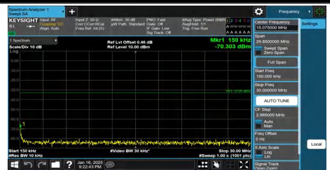
Band4-15MHz-QPSK-20325-75RB#0-0.15~30-PASS
