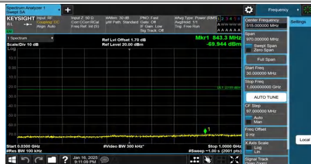
Band4-10MHz-QPSK-20350-50RB#0-30~1000-PASS
