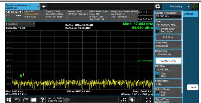
Band4-10MHz-QPSK-20175-1RB#0-0.009~0.15-PASS
