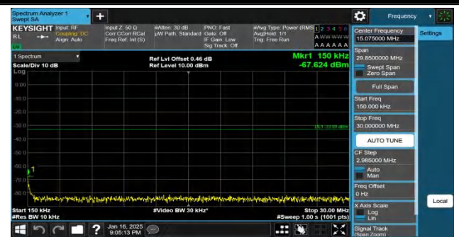
Band4-10MHz-QPSK-20000-1RB#0-0.15~30-PASS
