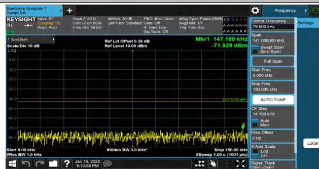
Band4-10MHz-QPSK-20350-50RB#0-0.009~0.15-PASS
