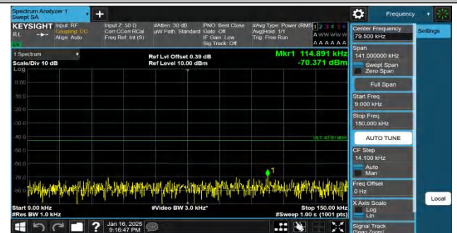
Band4-15MHz-QPSK-20025-1RB#0-0.009~0.15-PASS
