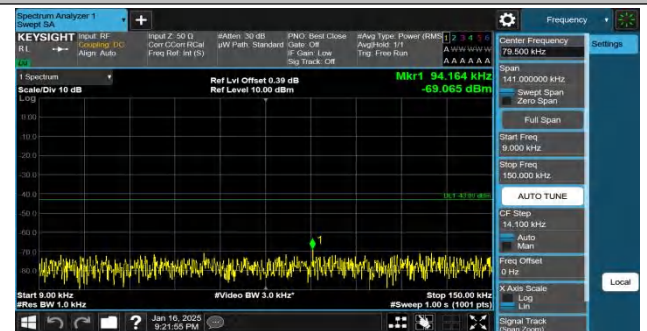
Band4-15MHz-QPSK-20325-1RB#74-0.009~0.15-PASS
