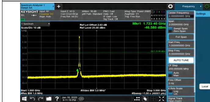
Band4-10MHz-QPSK-20350-50RB#0-1000~3000-PASS
