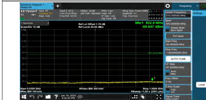
Band4-20MHz-QPSK-20300-1RB#99-30~1000-PASS
