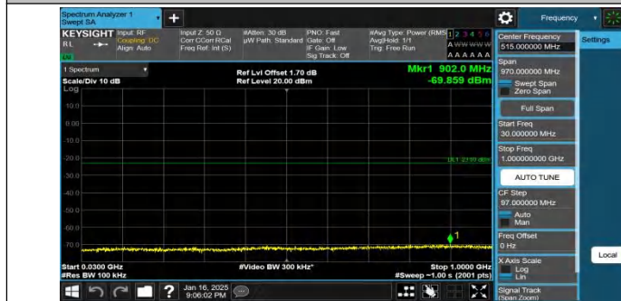
Band4-10MHz-QPSK-20000-1RB#49-30~1000-PASS
