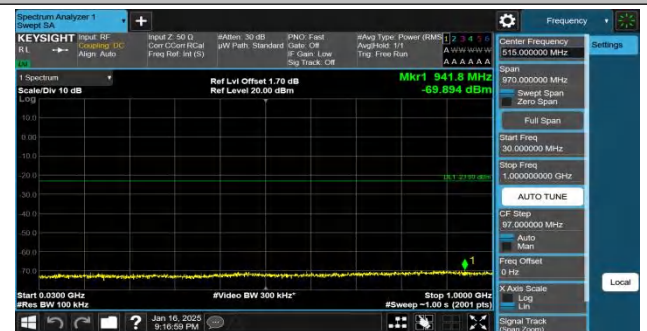
Band4-15MHz-QPSK-20025-1RB#0-30~1000-PASS
