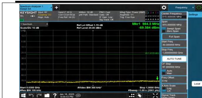
Band4-10MHz-QPSK-20350-1RB#0-30~1000-PASS
