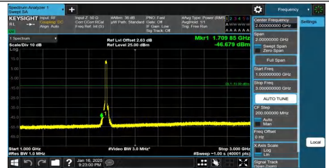
Band4-15MHz-QPSK-20325-75RB#0-1000~3000-PASS
