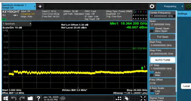
Band4-15MHz-QPSK-20025-75RB#0-3000~20000-PASS
