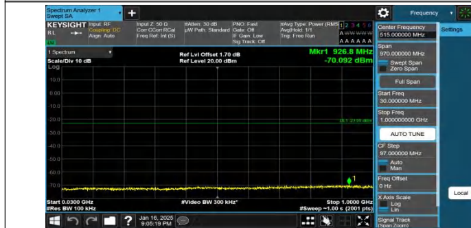
Band4-10MHz-QPSK-20000-1RB#0-30~1000-PASS
