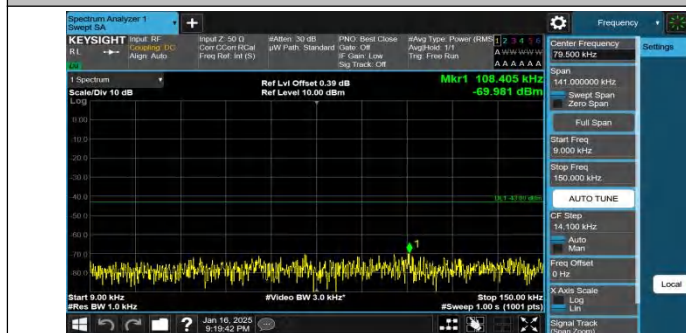
Band4-15MHz-QPSK-20175-1RB#74-0.009~0.15-PASS
