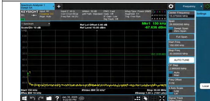
Band4-15MHz-QPSK-20325-1RB#74-0.15~30-PASS
