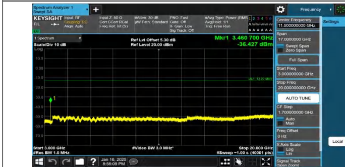
Band4-5MHz-QPSK-20175-1RB#0-3000~20000-PASS
