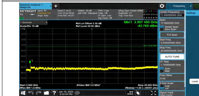
Band4-20MHz-QPSK-20300-1RB#99-3000~20000-PASS
