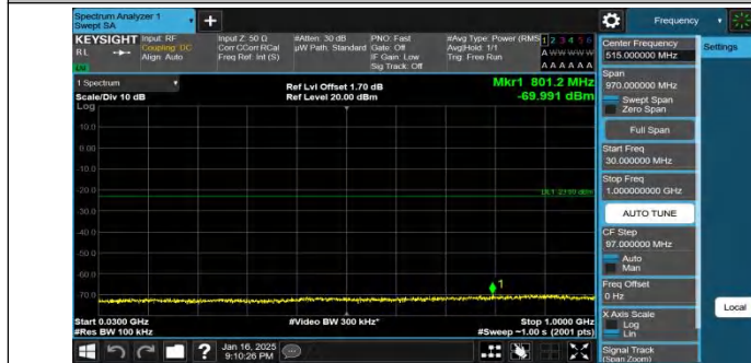
Band4-10MHz-QPSK-20350-1RB#49-30~1000-PASS
