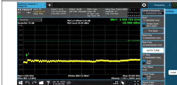
Band4-10MHz-QPSK-20350-1RB#49-3000~20000-PASS
