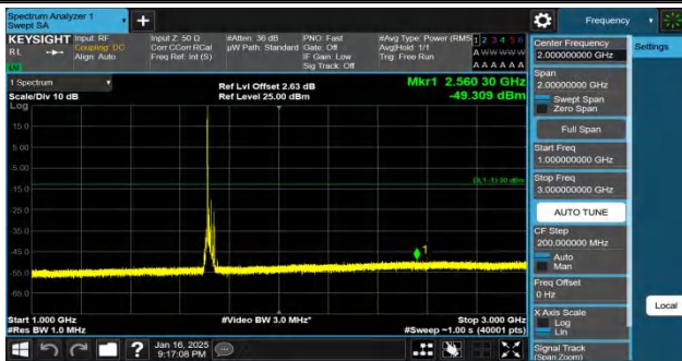
Band4-15MHz-QPSK-20025-1RB#0-1000~3000-PASS
