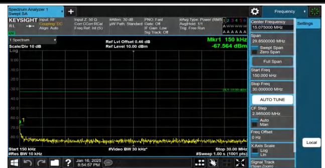
Band4-5MHz-QPSK-19975-25RB#0-0.15~30-PASS
