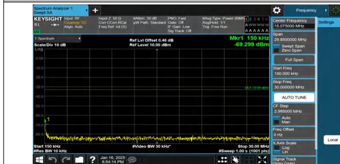
Band4-5MHz-QPSK-19975-1RB#24-0.15~30-PASS
