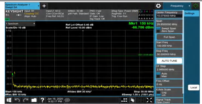
Band4-20MHz-QPSK-20300-1RB#99-0.15~30-PASS
