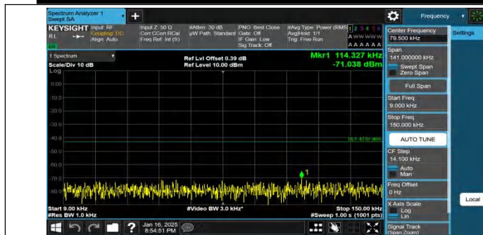
Band4-5MHz-QPSK-19975-25RB#0-0.009~0.15-PASS
