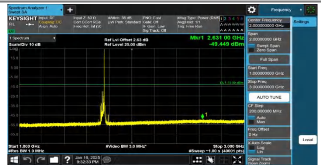
Band4-20MHz-QPSK-20300-1RB#99-1000~3000-PASS
