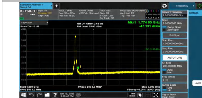
Band4-15MHz-QPSK-20175-75RB#0-1000~3000-PASS
