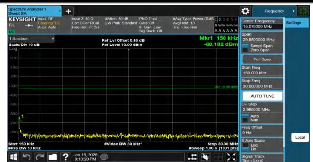
Band4-10MHz-QPSK-20350-1RB#49-0.15~30-PASS
