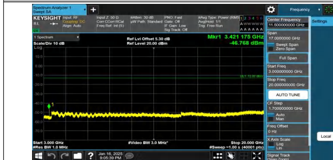
Band4-10MHz-QPSK-20000-1RB#0-3000~20000-PASS
