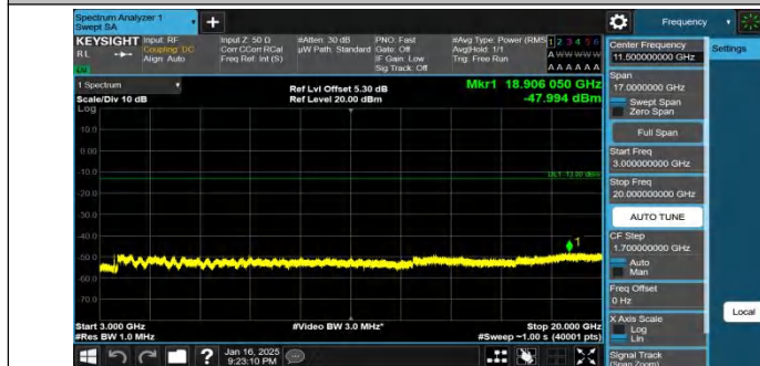
Band4-15MHz-QPSK-20325-75RB#0-3000~20000-PASS
