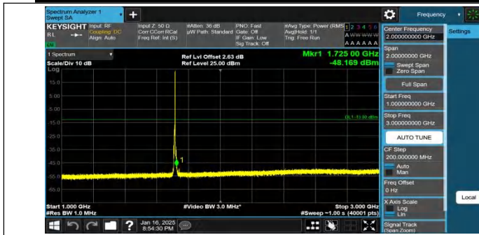
Band4-5MHz-QPSK-19975-1RB#24-1000~3000-PASS
