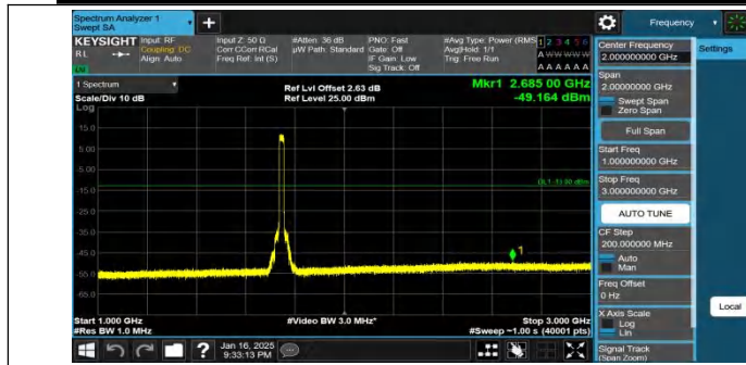
Band4-20MHz-QPSK-20300-100RB#0-1000~3000-PASS
