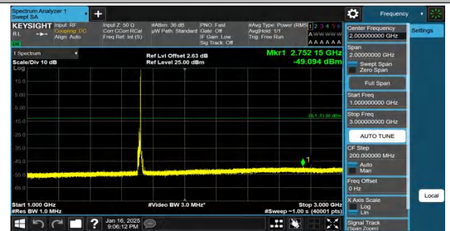
Band4-10MHz-QPSK-20000-1RB#49-1000~3000-PASS
