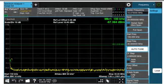
Band4-10MHz-QPSK-20000-1RB#49-0.15~30-PASS
