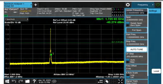
Band4-5MHz-QPSK-19975-25RB#0-1000~3000-PASS
