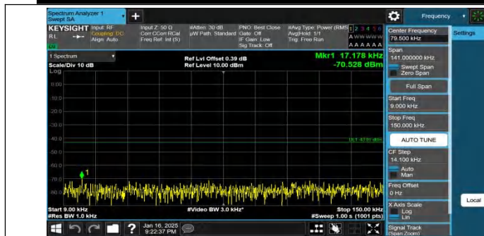
Band4-15MHz-QPSK-20325-75RB#0-0.009~0.15-PASS
