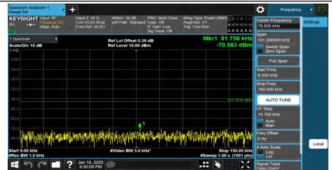
Band4-20MHz-QPSK-20175-1RB#99-0.009~0.15-PASS
