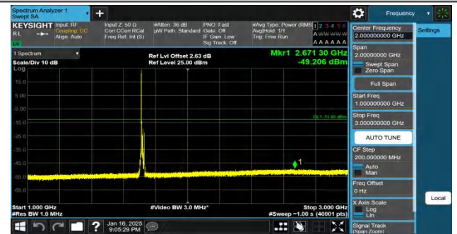
Band4-10MHz-QPSK-20000-1RB#0-1000~3000-PASS
