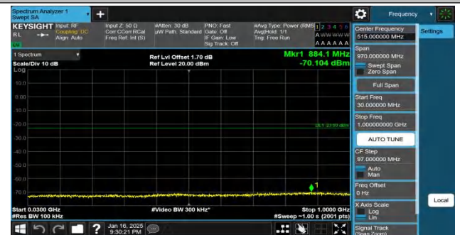
Band4-20MHz-QPSK-20175-1RB#99-30~1000-PASS
