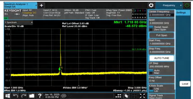
Band4-5MHz-QPSK-20175-1RB#0-1000~3000-PASS
