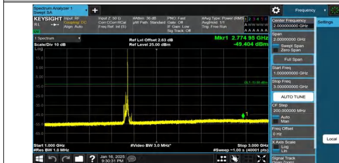
Band4-20MHz-QPSK-20175-1RB#99-1000~3000-PASS
