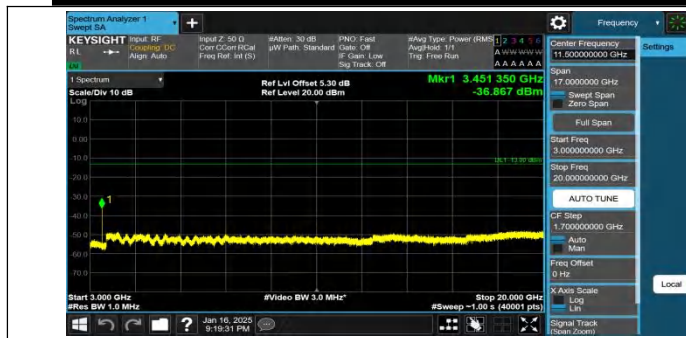
Band4-15MHz-QPSK-20175-1RB#0-3000~20000-PASS
