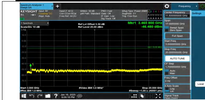
Band4-10MHz-QPSK-20175-50RB#0-3000~20000-PASS
