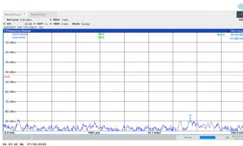
NTNV-DC_5A_n78A-PC2-30-5+100-M+L-QPSK-IDLE-DFT-QPSK-I nner_1RB_Left-0.009-0.15-PASS
