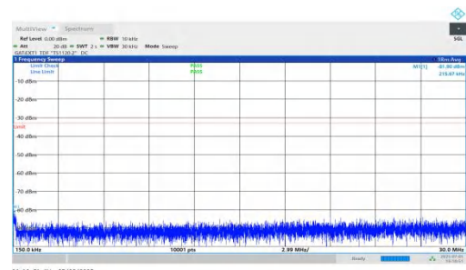
NTNV-DC_5A_n78A-PC2-30-5+90-M+L-QPSK-IDLE-DFT-QPSK-In ner_1RB_Left-0.15-30-PASS
