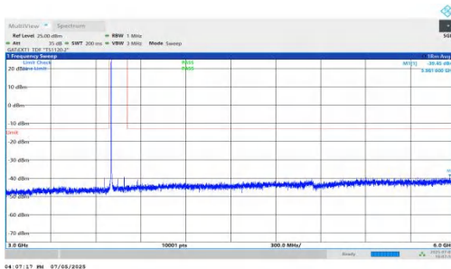
NTNV-DC_5A_n78A-PC2-30-5+90-M+L-QPSK-IDLE-DFT-BPSK-In ner_1RB_Left-3000-6000-PASS
