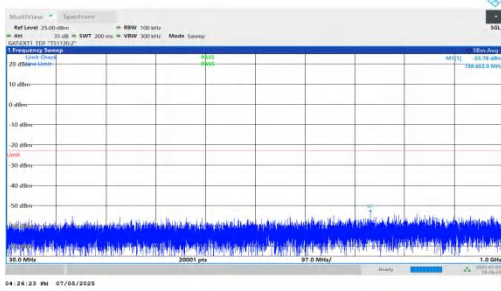
NTNV-DC_5A_n78A-PC2-30-5+90-M+H-QPSK-IDLE-DFT-QPSK-Inner_1RB_Left-30-1000-PASS
