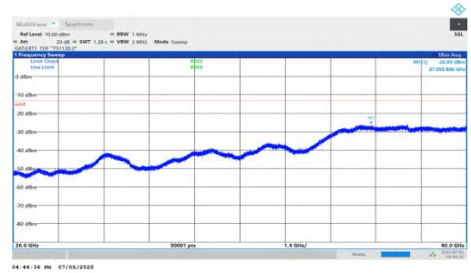
NTNV-DC_5A_n78A-PC2-30-5+100-M+M-QPSK-IDLE-DFT-QPSK-Inner_1RB_Right-26000-40000-PASS
