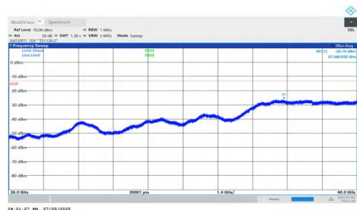
NTNV-DC_5A_n78A-PC2-30-5+90-M+M-QPSK-IDLE-DFT-QPSK-Inner_1RB_Right-26000-40000-PASS
