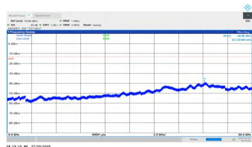
NTNV-DC_5A_n78A-PC2-30-5+90-M+M-QPSK-IDLE-DFT-QPSK-Inner_1RB_Left-6000-26000-PASS
