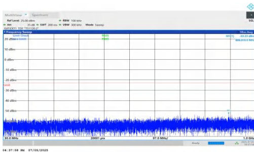
NTNV-DC_5A_n78A-PC2-30-5+100-M+M-QPSK-IDLE-DFT-BPSK-Inner_1RB_Left-30-1000-PASS
