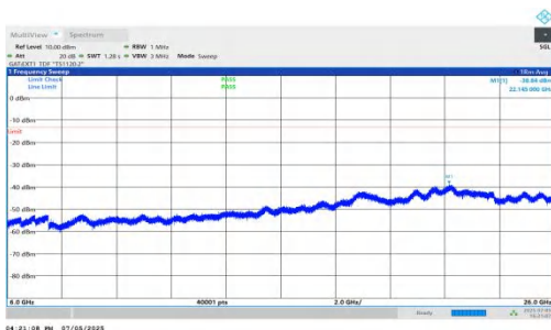
NTNV-DC_5A_n78A-PC2-30-5+90-M+M-QPSK-IDLE-DFT-QPSK-Inner_1RB_Right-6000-26000-PASS
