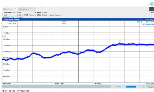
NTNV-DC_5A_n78A-PC2-30-5+100-M+M-QPSK-IDLE-DFT-BPSK-Inner_1RB_Left-26000-40000-PASS
