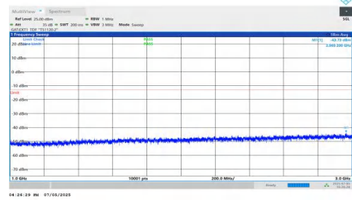
NTNV-DC_5A_n78A-PC2-30-5+90-M+H-QPSK-IDLE-DFT-QPSK-Inner_1RB_Left-1000-3000-PASS
