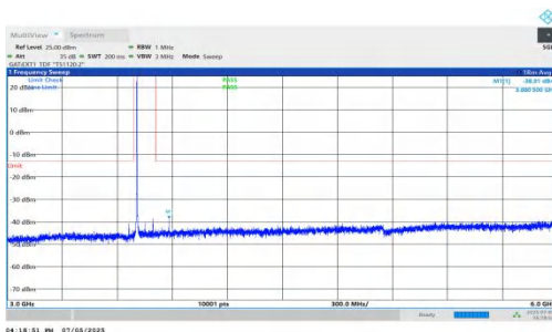
NTNV-DC_5A_n78A-PC2-30-5+90-M+M-QPSK-IDLE-DFT-QPSK-Inner_1RB_Left-3000-6000-PASS
