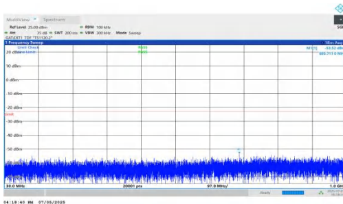
NTNV-DC_5A_n78A-PC2-30-5+90-M+M-QPSK-IDLE-DFT-QPSK-Inner_1RB_Left-30-1000-PASS
