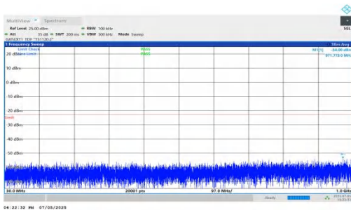
NTNV-DC_5A_n78A-PC2-30-5+90-M+H-QPSK-IDLE-DFT-BPSK-I nner_1RB_Left-30-1000-PASS
