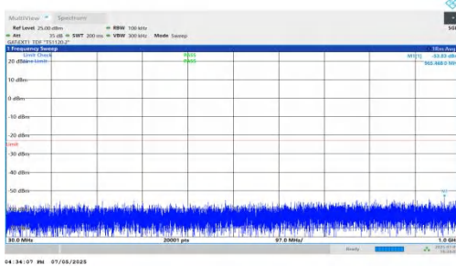
NTNV-DC_5A_n78A-PC2-30-5+100-M+L-QPSK-IDLE-DFT-QPSK-I nner_1RB_Left-30-1000-PASS
