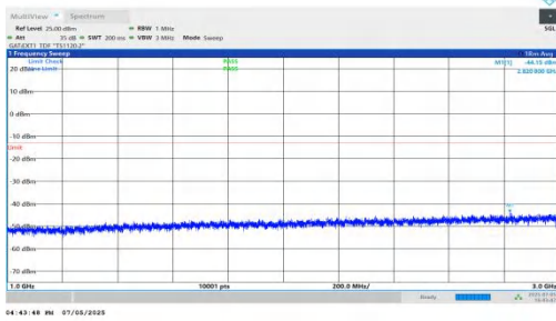
NTNV-DC_5A_n78A-PC2-30-5+100-M+M-QPSK-IDLE-DFT-QPSK-Inner_1RB_Right-1000-3000-PASS
