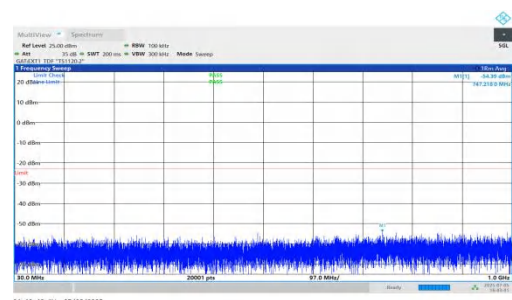
NTNV-DC_5A_n78A-PC2-30-5+100-M+M-QPSK-IDLE-DFT-QPSK-Inner_1RB_Right-30-1000-PASS
