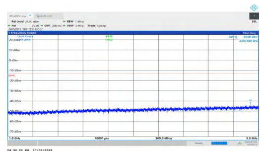
NTNV-DC_5A_n78A-PC2-30-5+100-M+L-QPSK-IDLE-DFT-BPSK-Inner_1RB_Left-1000-3000-PASS
