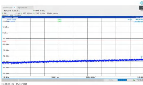
NTNV-DC_5A_n78A-PC2-30-5+90-M+L-QPSK-IDLE-DFT-BPSK-In ner_1RB_Right-1000-3000-PASS
