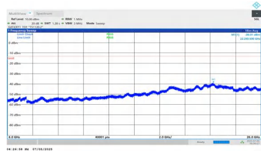
NTNV-DC_5A_n78A-PC2-30-5+90-M+H-QPSK-IDLE-DFT-QPSK-Inner_1RB_Left-6000-26000-PASS
