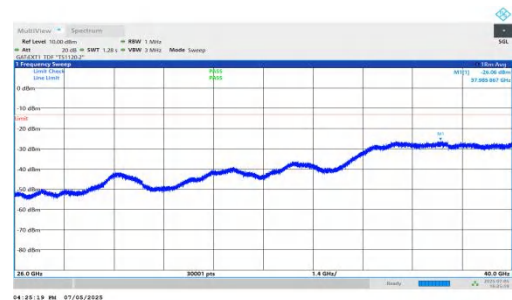
NTNV-DC_5A_n78A-PC2-30-5+90-M+H-QPSK-IDLE-DFT-BPSK-In ner_1RB_Right-26000-40000-PASS
