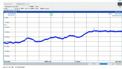
NTNV-DC_5A_n78A-PC2-30-5+90-M+M-QPSK-IDLE-DFT-BPSK-Inner_1RB_Right-26000-40000-PASS
