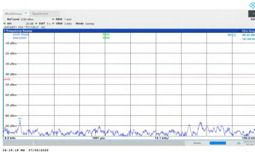
NTNV-DC_5A_n78A-PC2-30-5+90-M+M-QPSK-IDLE-DFT-QPSK-Inner_1RB_Left-0.009-0.15-PASS
