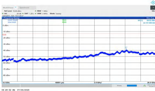
NTNV-DC_5A_n78A-PC2-30-5+90-M+H-QPSK-IDLE-DFT-QPSK-Inner_1RB_Right-6000-26000-PASS
