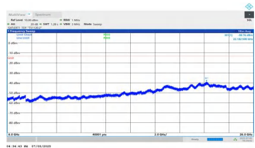
NTNV-DC_5A_n78A-PC2-30-5+100-M+L-QPSK-IDLE-DFT-QPSK-I nner_1RB_Left-6000-26000-PASS
