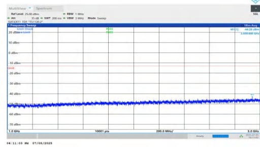
NTNV-DC_5A_n78A-PC2-30-5+90-M+L-QPSK-IDLE-DFT-QPSK-In ner_1RB_Left-1000-3000-PASS
