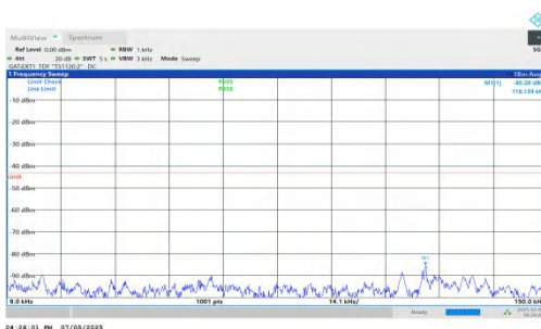
NTNV-DC_5A_n78A-PC2-30-5+90-M+H-QPSK-IDLE-DFT-QPSK-I nner_1RB_Left-0.009-0.15-PASS
