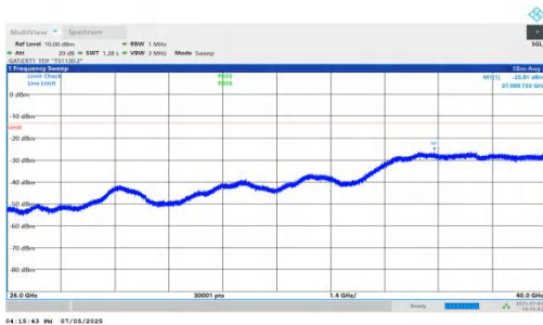
NTNV-DC_5A_n78A-PC2-30-5+90-M+M-QPSK-IDLE-DFT-BPSK-I nner_1RB_Left-26000-40000-PASS
