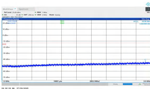
NTNV-DC_5A_n78A-PC2-30-5+100-M+L-QPSK-IDLE-DFT-QPSK-I nner_1RB_Right-1000-3000-PASS
