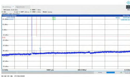
NTNV-DC_5A_n78A-PC2-30-5+100-M+M-QPSK-IDLE-DFT-QPSK-Inner_1RB_Left-3000-6000-PASS
