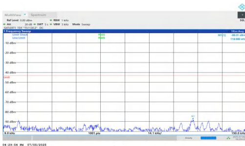
NTNV-DC_5A_n78A-PC2-30-5+100-M+L-QPSK-IDLE-DFT-BPSK-Inner_1RB_Left-0.009-0.15-PASS
