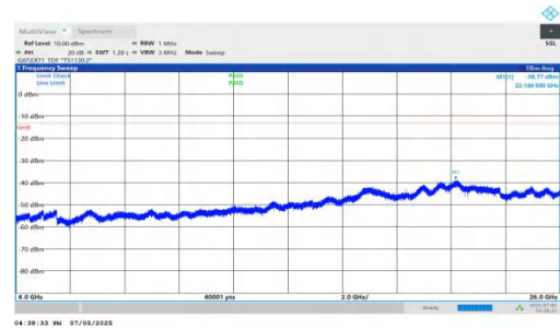
NTNV-DC_5A_n78A-PC2-30-5+100-M+M-QPSK-IDLE-DFT-BPSK-Inner_1RB_Left-6000-26000-PASS
