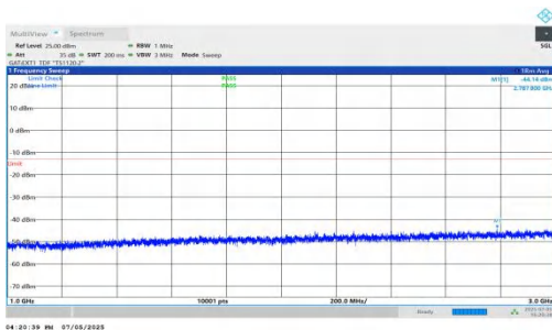
NTNV-DC_5A_n78A-PC2-30-5+90-M+M-QPSK-IDLE-DFT-QPSK-Inner_1RB_Right-1000-3000-PASS
