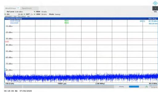
NTNV-DC_5A_n78A-PC2-30-5+90-M+M-QPSK-IDLE-DFT-QPSK-Inner_1RB_Left-0.15-30-PASS
