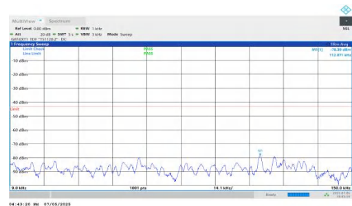
NTNV-DC_5A_n78A-PC2-30-5+100-M+M-QPSK-IDLE-DFT-QPSK-Inner_1RB_Right-0.009-0.15-PASS
