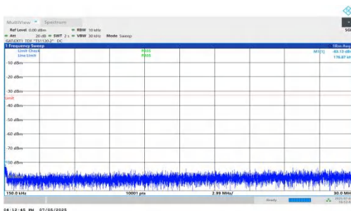
NTNV-DC_5A_n78A-PC2-30-5+90-M+L-QPSK-IDLE-DFT-QPSK-In ner_1RB_Right-0.15-30-PASS
