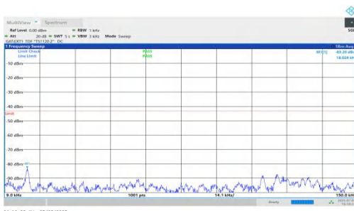
NTNV-DC_5A_n78A-PC2-30-5+90-M+L-QPSK-IDLE-DFT-QPSK-In ner_1RB_Left-0.009-0.15-PASS
