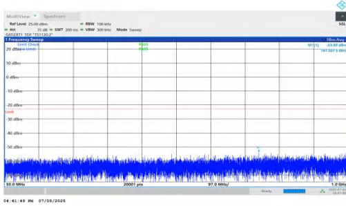
NTNV-DC_5A_n78A-PC2-30-5+100-M+M-QPSK-IDLE-DFT-QPSK-Inner_1RB_Left-30-1000-PASS
