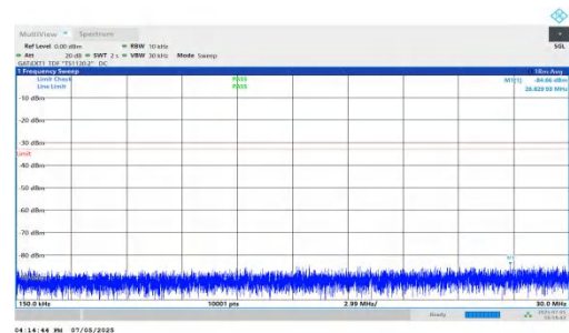
NTNV-DC_5A_n78A-PC2-30-5+90-M+M-QPSK-IDLE-DFT-BPSK-Inner_1RB_Left-0.15-30-PASS
