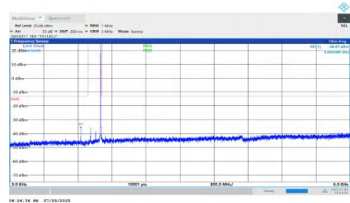
NTNV-DC_5A_n78A-PC2-30-5+90-M+H-QPSK-IDLE-DFT-BPSK-In ner_1RB_Right-3000-6000-PASS
