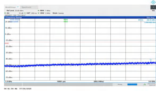
NTNV-DC_5A_n78A-PC2-30-5+100-M+M-QPSK-IDLE-DFT-QPSK-Inner_1RB_Left-1000-3000-PASS
