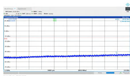
NTNV-DC_5A_n78A-PC2-30-5+90-M+M-QPSK-IDLE-DFT-BPSK-Inner_1RB_Left-1000-3000-PASS
