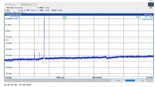
NTNV-DC_5A_n78A-PC2-30-5+100-M+M-QPSK-IDLE-DFT-QPSK-Inner_1RB_Right-3000-6000-PASS
