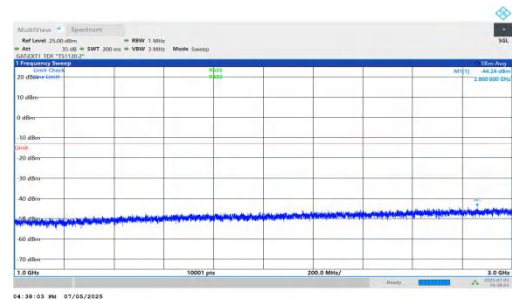
NTNV-DC_5A_n78A-PC2-30-5+100-M+M-QPSK-IDLE-DFT-BPSK-Inner_1RB_Left-1000-3000-PASS
