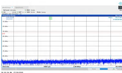
NTNV-DC_5A_n78A-PC2-30-5+100-M+L-QPSK-IDLE-DFT-BPSK-I nner_1RB_Right-0.15-30-PASS
