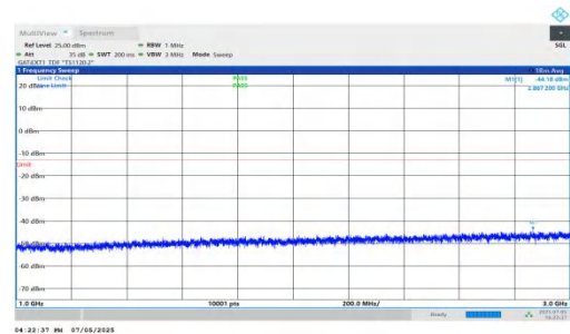
NTNV-DC_5A_n78A-PC2-30-5+90-M+H-QPSK-IDLE-DFT-BPSK-In ner_1RB_Left-1000-3000-PASS
