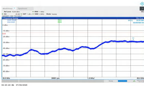
NTNV-DC_5A_n78A-PC2-30-5+90-M+H-QPSK-IDLE-DFT-BPSK-I nner_1RB_Left-26000-40000-PASS
