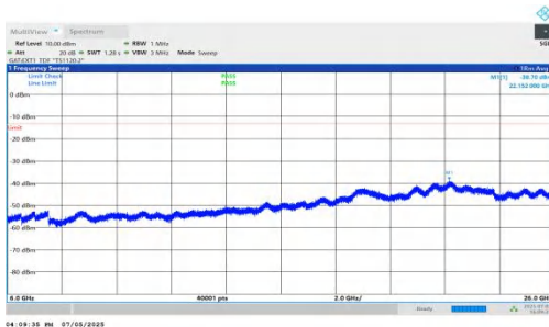
NTNV-DC_5A_n78A-PC2-30-5+90-M+L-QPSK-IDLE-DFT-BPSK-In ner_1RB_Right-6000-26000-PASS
