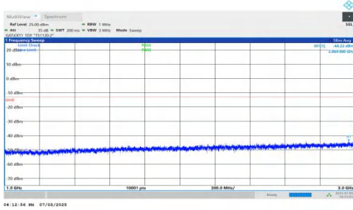
NTNV-DC_5A_n78A-PC2-30-5+90-M+L-QPSK-IDLE-DFT-QPSK-Inner_1RB_Right-1000-3000-PASS
