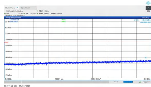
NTNV-DC_5A_n78A-PC2-30-5+90-M+L-QPSK-IDLE-DFT-BPSK-In ner_1RB_Left-1000-3000-PASS
