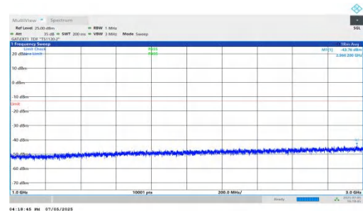
NTNV-DC_5A_n78A-PC2-30-5+90-M+M-QPSK-IDLE-DFT-QPSK-Inner_1RB_Left-1000-3000-PASS
