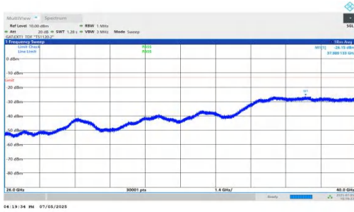
NTNV-DC_5A_n78A-PC2-30-5+90-M+M-QPSK-IDLE-DFT-QPSK-Inner_1RB_Left-26000-40000-PASS
