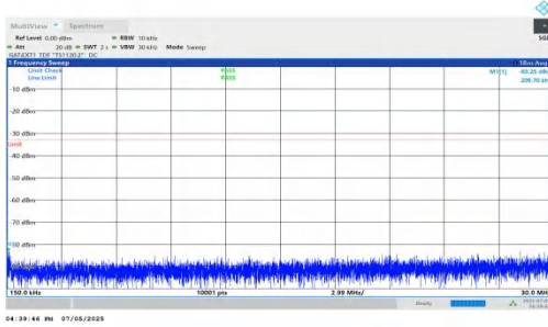
NTNV-DC_5A_n78A-PC2-30-5+100-M+M-QPSK-IDLE-DFT-BPSK-Inner_1RB_Right-0.15-30-PASS
