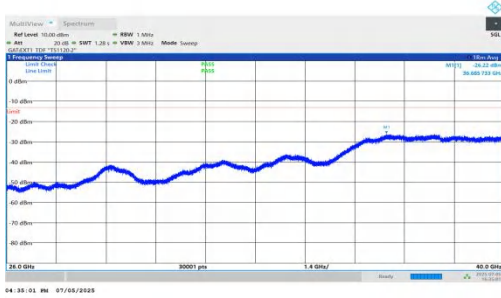
NTNV-DC_5A_n78A-PC2-30-5+100-M+L-QPSK-IDLE-DFT-QPSK-I nner_1RB_Left-26000-40000-PASS
