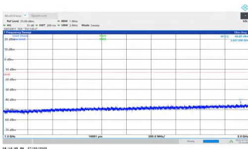
NTNV-DC_5A_n78A-PC2-30-5+90-M+M-QPSK-IDLE-DFT-BPSK-I nner_1RB_Right-1000-3000-PASS
