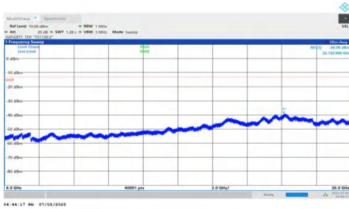
NTNV-DC_5A_n78A-PC2-30-5+100-M+M-QPSK-IDLE-DFT-QPSK-Inner_1RB_Right-6000-26000-PASS
