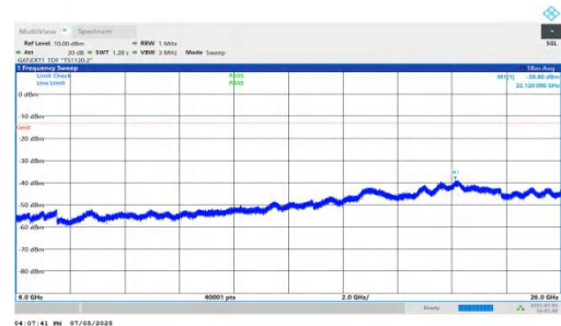
NTNV-DC_5A_n78A-PC2-30-5+90-M+L-QPSK-IDLE-DFT-BPSK-In ner_1RB_Left-6000-26000-PASS
