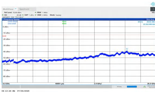
NTNV-DC_5A_n78A-PC2-30-5+90-M+L-QPSK-IDLE-DFT-QPSK-Inner_1RB_Right-6000-26000-PASS
