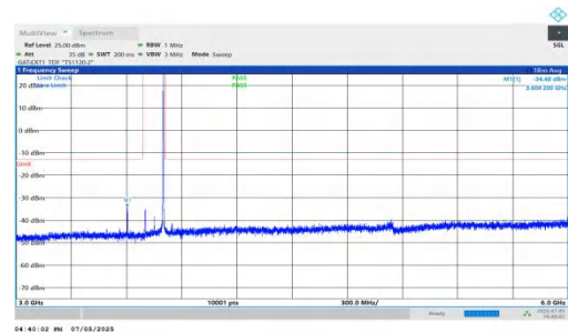
NTNV-DC_5A_n78A-PC2-30-5+100-M+M-QPSK-IDLE-DFT-BPSK-I nner_1RB_Right-3000-6000-PASS
