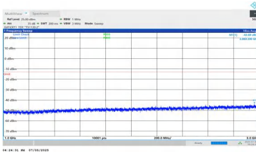
NTNV-DC_5A_n78A-PC2-30-5+90-M+H-QPSK-IDLE-DFT-BPSK-I nner_1RB_Right-1000-3000-PASS
