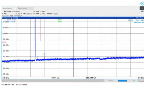
NTNV-DC_5A_n78A-PC2-30-5+100-M+M-QPSK-IDLE-DFT-BPSK-Inner_1RB_Left-3000-6000-PASS
