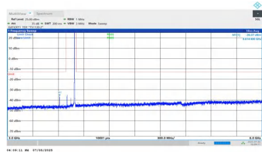
NTNV-DC_5A_n78A-PC2-30-5+90-M+L-QPSK-IDLE-DFT-BPSK-In ner_1RB_Right-3000-6000-PASS
