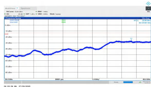
NTNV-DC_5A_n78A-PC2-30-5+90-M+L-QPSK-IDLE-DFT-BPSK-In ner_1RB_Right-26000-40000-PASS
