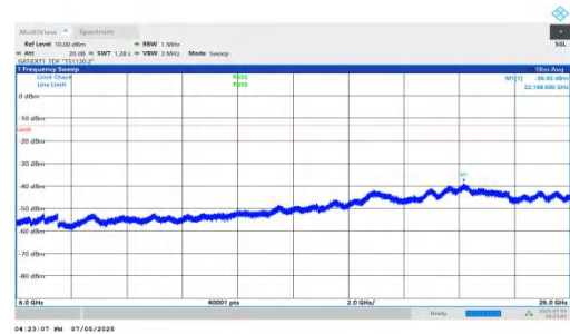
NTNV-DC_5A_n78A-PC2-30-5+90-M+H-QPSK-IDLE-DFT-BPSK-In ner_1RB_Left-6000-26000-PASS
