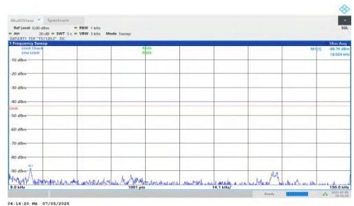
NTNV-DC_5A_n78A-PC2-30-5+90-M+M-QPSK-IDLE-DFT-BPSK-In ner_1RB_Right-0.009-0.15-PASS
