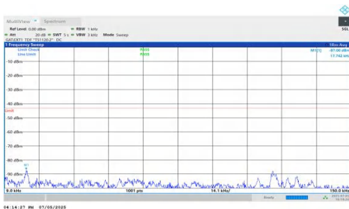
NTNV-DC_5A_n78A-PC2-30-5+90-M+M-QPSK-IDLE-DFT-BPSK-Inner_1RB_Left-0.009-0.15-PASS
