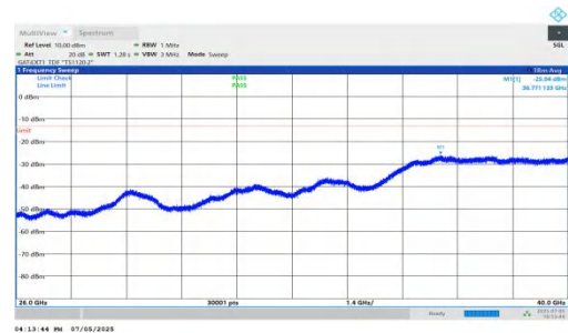
NTNV-DC_5A_n78A-PC2-30-5+90-M+L-QPSK-IDLE-DFT-QPSK-Inner_1RB_Right-26000-40000-PASS
