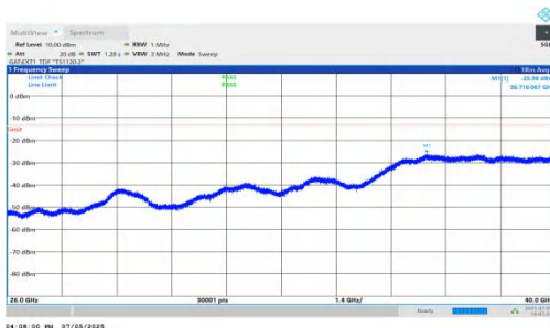
NTNV-DC_5A_n78A-PC2-30-5+90-M+L-QPSK-IDLE-DFT-BPSK-In ner_1RB_Left-26000-40000-PASS
