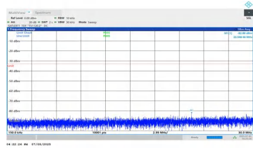
NTNV-DC_5A_n78A-PC2-30-5+90-M+H-QPSK-IDLE-DFT-BPSK-In ner_1RB_Left-0.15-30-PASS
