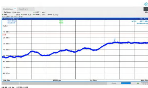
NTNV-DC_5A_n78A-PC2-30-5+100-M+M-QPSK-IDLE-DFT-QPSK-Inner_1RB_Left-26000-40000-PASS
