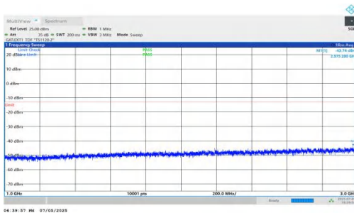
NTNV-DC_5A_n78A-PC2-30-5+100-M+M-QPSK-IDLE-DFT-BPSK-Inner_1RB_Right-1000-3000-PASS
