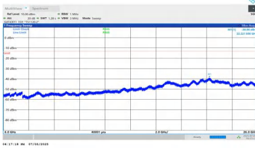
NTNV-DC_5A_n78A-PC2-30-5+90-M+M-QPSK-IDLE-DFT-BPSK-Inner_1RB_Right-6000-26000-PASS
