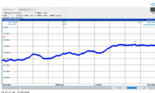
NTNV-DC_5A_n78A-PC2-30-5+90-M+H-QPSK-IDLE-DFT-QPSK-Inner_1RB_Left-26000-40000-PASS
