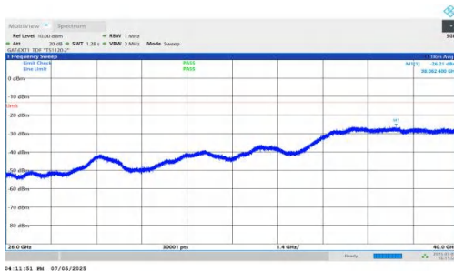
NTNV-DC_5A_n78A-PC2-30-5+90-M+L-QPSK-IDLE-DFT-QPSK-In ner_1RB_Left-26000-40000-PASS
