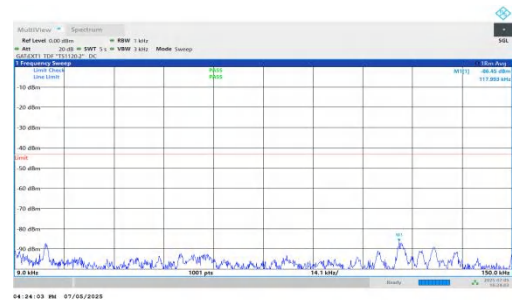
NTNV-DC_5A_n78A-PC2-30-5+90-M+H-QPSK-IDLE-DFT-BPSK-In ner_1RB_Right-0.009-0.15-PASS
