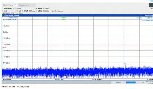
NTNV-DC_5A_n78A-PC2-30-5+90-M+L-QPSK-IDLE-DFT-QPSK-In ner_1RB_Left-30-1000-PASS
