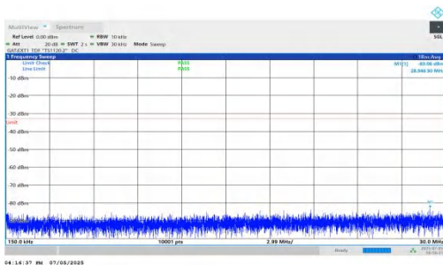
NTNV-DC_5A_n78A-PC2-30-5+90-M+M-QPSK-IDLE-DFT-BPSK-I nner_1RB_Right-0.15-30-PASS
