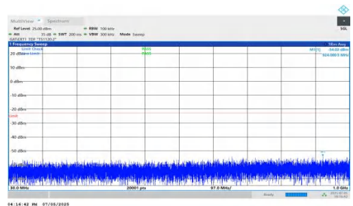
NTNV-DC_5A_n78A-PC2-30-5+90-M+M-QPSK-IDLE-DFT-BPSK-In ner_1RB_Right-30-1000-PASS
