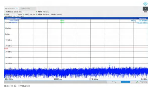
NTNV-DC_5A_n78A-PC2-30-5+100-M+L-QPSK-IDLE-DFT-QPSK-I nner_1RB_Right-30-1000-PASS
