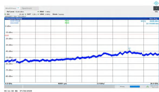
NTNV-DC_5A_n78A-PC2-30-5+90-M+L-QPSK-IDLE-DFT-QPSK-In ner_1RB_Left-6000-26000-PASS
