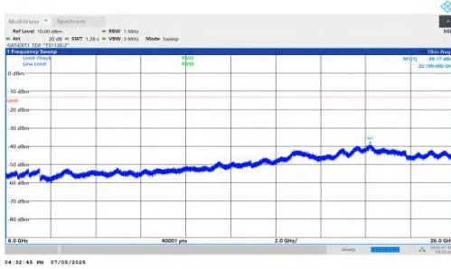
NTNV-DC_5A_n78A-PC2-30-5+100-M+L-QPSK-IDLE-DFT-BPSK-I nner_1RB_Right-6000-26000-PASS
