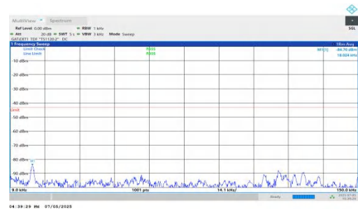
NTNV-DC_5A_n78A-PC2-30-5+100-M+M-QPSK-IDLE-DFT-BPSK-Inner_1RB_Right-0.009-0.15-PASS
