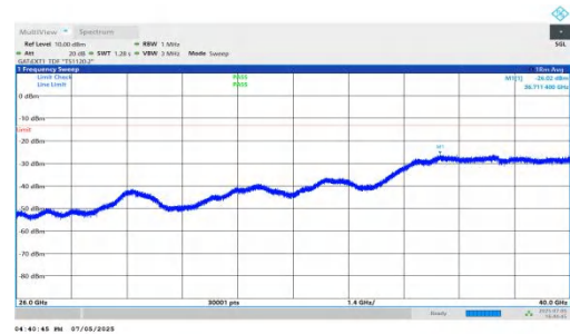
NTNV-DC_5A_n78A-PC2-30-5+100-M+M-QPSK-IDLE-DFT-BPSK-I nner_1RB_Right-26000-40000-PASS
