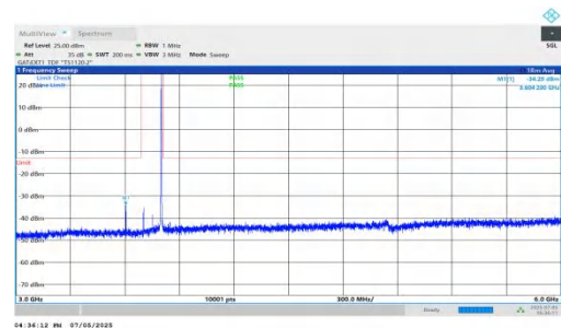
NTNV-DC_5A_n78A-PC2-30-5+100-M+L-QPSK-IDLE-DFT-QPSK-I nner_1RB_Right-3000-6000-PASS
