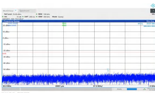
NTNV-DC_5A_n78A-PC2-30-5+90-M+M-QPSK-IDLE-DFT-BPSK-Inner_1RB_Left-30-1000-PASS
