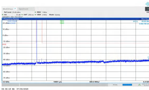
NTNV-DC_5A_n78A-PC2-30-5+100-M+L-QPSK-IDLE-DFT-QPSK-I nner_1RB_Left-3000-6000-PASS
