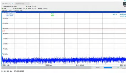
NTNV-DC_5A_n78A-PC2-30-5+90-M+H-QPSK-IDLE-DFT-BPSK-I nner_1RB_Right-0.15-30-PASS
