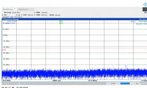
NTNV-DC_5A_n78A-PC2-30-5+100-M+L-QPSK-IDLE-DFT-BPSK-Inner_1RB_Left-30-1000-PASS
