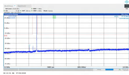
NTNV-DC_5A_n78A-PC2-30-5+90-M+L-QPSK-IDLE-DFT-QPSK-Inner_1RB_Right-3000-6000-PASS
