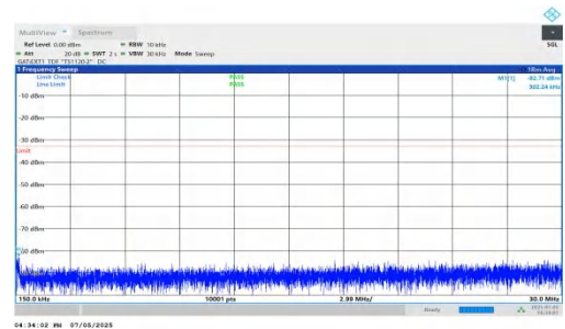
NTNV-DC_5A_n78A-PC2-30-5+100-M+L-QPSK-IDLE-DFT-QPSK-I nner_1RB_Left-0.15-30-PASS
