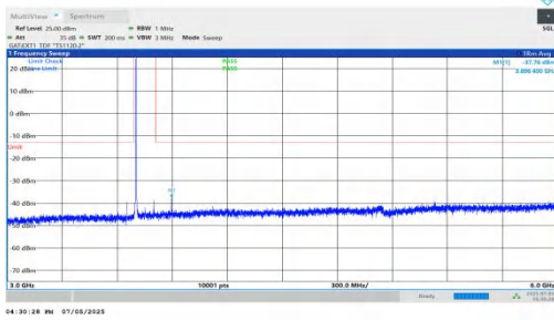
NTNV-DC_5A_n78A-PC2-30-5+100-M+L-QPSK-IDLE-DFT-BPSK-I nner_1RB_Left-3000-6000-PASS
