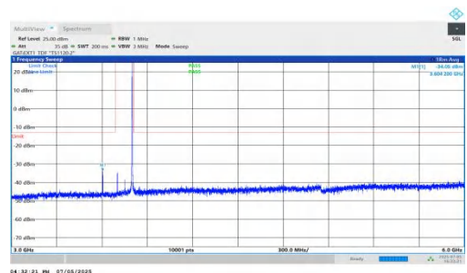
NTNV-DC_5A_n78A-PC2-30-5+100-M+L-QPSK-IDLE-DFT-BPSK-I nner_1RB_Right-3000-6000-PASS
