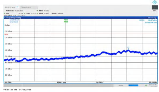
NTNV-DC_5A_n78A-PC2-30-5+90-M+M-QPSK-IDLE-DFT-BPSK-In ner_1RB_Left-6000-26000-PASS
