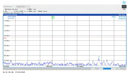
NTNV-DC_5A_n78A-PC2-30-5+100-M+L-QPSK-IDLE-DFT-BPSK-I nner_1RB_Right-0.009-0.15-PASS
