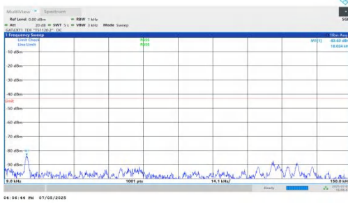
NTNV-DC_5A_n78A-PC2-30-5+90-M+L-QPSK-IDLE-DFT-BPSK-In ner_1RB_Left-0.009-0.15-PASS
