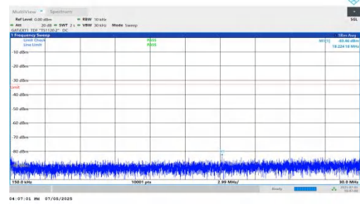
NTNV-DC_5A_n78A-PC2-30-5+90-M+L-QPSK-IDLE-DFT-BPSK-In ner_1RB_Left-0.15-30-PASS
