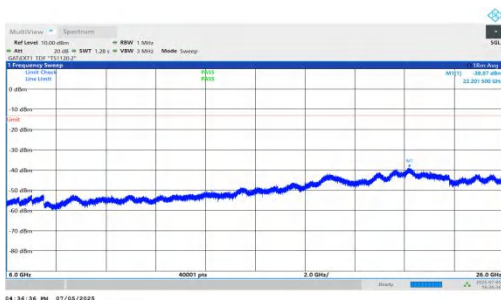
NTNV-DC_5A_n78A-PC2-30-5+100-M+L-QPSK-IDLE-DFT-QPSK-I nner_1RB_Right-6000-26000-PASS
