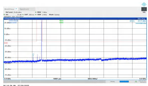
NTNV-DC_5A_n78A-PC2-30-5+90-M+M-QPSK-IDLE-DFT-BPSK-In ner_1RB_Right-3000-6000-PASS
