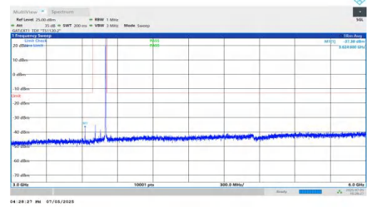
NTNV-DC_5A_n78A-PC2-30-5+90-M+H-QPSK-IDLE-DFT-QPSK-Inner_1RB_Right-3000-6000-PASS
