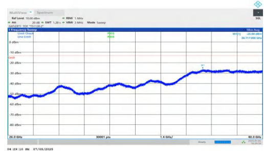
NTNV-DC_5A_n78A-PC2-30-5+90-M+H-QPSK-IDLE-DFT-QPSK-Inner_1RB_Right-26000-40000-PASS
