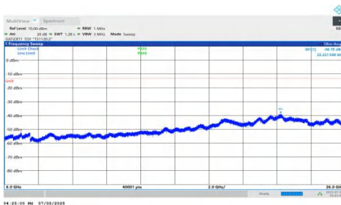
NTNV-DC_5A_n78A-PC2-30-5+90-M+H-QPSK-IDLE-DFT-BPSK-I nner_1RB_Right-6000-26000-PASS
