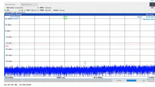
NTNV-DC_5A_n78A-PC2-30-5+90-M+H-QPSK-IDLE-DFT-BPSK-In ner_1RB_Right-30-1000-PASS
