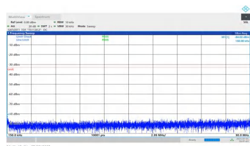
NTNV-DC_5A_n78A-PC2-30-5+100-M+M-QPSK-IDLE-DFT-QPSK-I nner_1RB_Left-0.15-30-PASS
