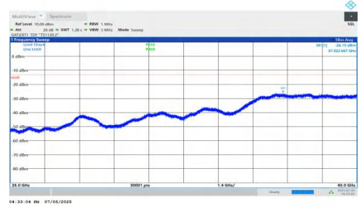
NTNV-DC_5A_n78A-PC2-30-5+100-M+L-QPSK-IDLE-DFT-BPSK-I nner_1RB_Right-26000-40000-PASS
