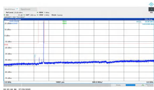
NTNV-DC_5A_n78A-PC2-30-5+90-M+M-QPSK-IDLE-DFT-QPSK-Inner_1RB_Right-3000-6000-PASS
