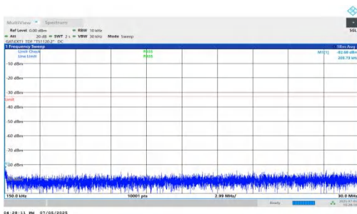
NTNV-DC_5A_n78A-PC2-30-5+90-M+H-QPSK-IDLE-DFT-QPSK-Inner_1RB_Right-0.15-30-PASS
