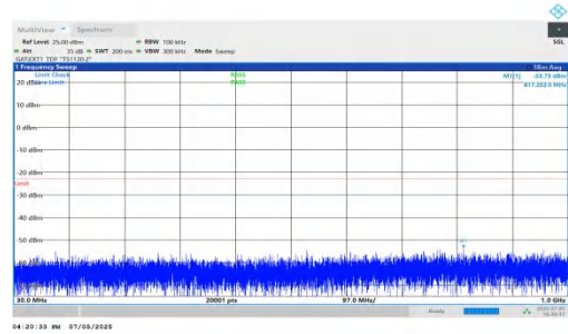
NTNV-DC_5A_n78A-PC2-30-5+90-M+M-QPSK-IDLE-DFT-QPSK-Inner_1RB_Right-30-1000-PASS
