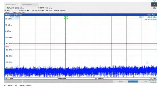
NTNV-DC_5A_n78A-PC2-30-5+90-M+L-QPSK-IDLE-DFT-BPSK-In ner_1RB_Right-30-1000-PASS
