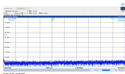
NTNV-DC_5A_n78A-PC2-30-5+90-M+H-QPSK-IDLE-DFT-QPSK-In ner_1RB_Left-0.15-30-PASS
