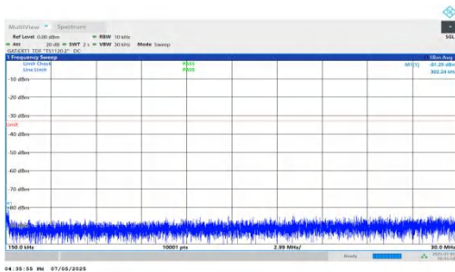
NTNV-DC_5A_n78A-PC2-30-5+100-M+L-QPSK-IDLE-DFT-QPSK-I nner_1RB_Right-0.15-30-PASS
