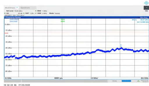
NTNV-DC_5A_n78A-PC2-30-5+100-M+M-QPSK-IDLE-DFT-QPSK-Inner_1RB_Left-6000-26000-PASS
