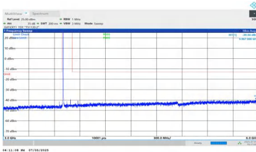
NTNV-DC_5A_n78A-PC2-30-5+90-M+L-QPSK-IDLE-DFT-QPSK-In ner_1RB_Left-3000-6000-PASS
