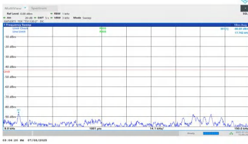
NTNV-DC_5A_n78A-PC2-30-5+70-M+L-QPSK-IDLE-DFT-BPSK-In ner_1RB_Left-0.009-0.15-PASS
