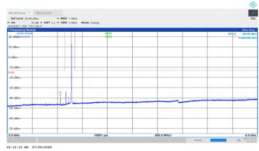
NTNV-DC_5A_n78A-PC2-30-5+70-M+L-QPSK-IDLE-DFT-QPSK-Inner_1RB_Right-3000-6000-PASS
