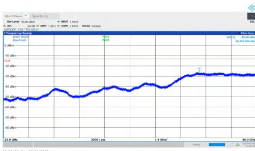
NTNV-DC_5A_n78A-PC2-30-5+80-M+M-QPSK-IDLE-DFT-BPSK-I nner_1RB_Left-26000-40000-PASS
