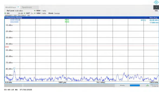
NTNV-DC_5A_n78A-PC2-30-5+80-M+L-QPSK-IDLE-DFT-QPSK-In ner_1RB_Right-0.009-0.15-PASS
