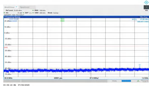
NTNV-DC_5A_n78A-PC2-30-5+60-M+H-QPSK-IDLE-DFT-QPSK-Inner_1RB_Right-30-1000-PASS
