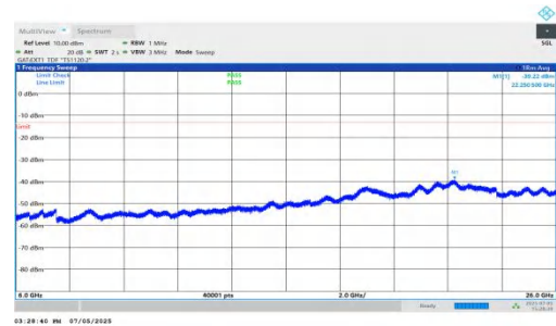
NTNV-DC_5A_n78A-PC2-30-5+70-M+H-QPSK-IDLE-DFT-BPSK-In ner_1RB_Left-6000-26000-PASS
