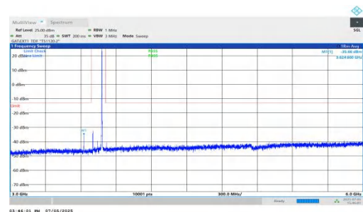
NTNV-DC_5A_n78A-PC2-30-5+80-M+L-QPSK-IDLE-DFT-BPSK-In ner_1RB_Right-3000-6000-PASS
