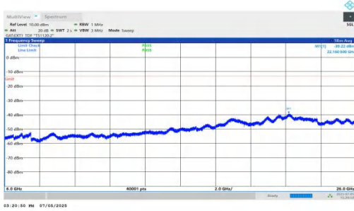
NTNV-DC_5A_n78A-PC2-30-5+70-M+M-QPSK-IDLE-DFT-BPSK-Inner_1RB_Right-6000-26000-PASS
