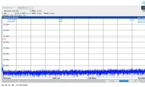
NTNV-DC_5A_n78A-PC2-30-5+80-M+H-QPSK-IDLE-DFT-QPSK-Inner_1RB_Right-0.15-30-PASS
