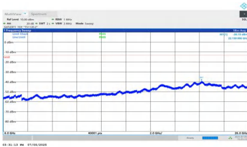
NTNV-DC_5A_n78A-PC2-30-5+70-M+H-QPSK-IDLE-DFT-BPSK-Inner_1RB_Right-6000-26000-PASS
