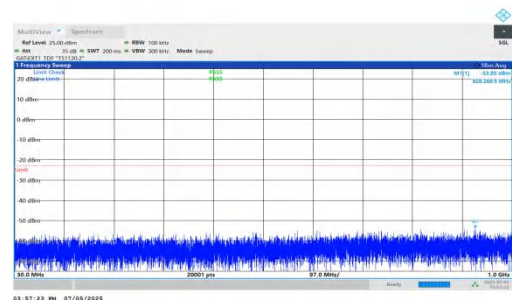
NTNV-DC_5A_n78A-PC2-30-5+80-M+M-QPSK-IDLE-DFT-QPSK-In ner_1RB_Right-30-1000-PASS
