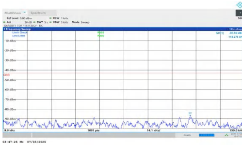
NTNV-DC_5A_n78A-PC2-30-5+80-M+L-QPSK-IDLE-DFT-QPSK-In ner_1RB_Left-0.009-0.15-PASS
