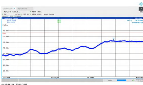
NTNV-DC_5A_n78A-PC2-30-5+70-M+L-QPSK-IDLE-DFT-QPSK-In ner_1RB_Left-26000-40000-PASS
