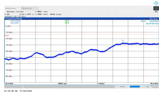
NTNV-DC_5A_n78A-PC2-30-5+70-M+H-QPSK-IDLE-DFT-QPSK-Inner_1RB_Right-26000-40000-PASS
