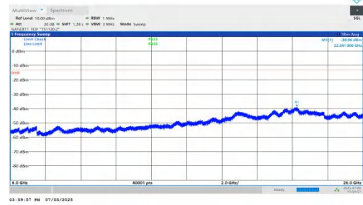
NTNV-DC_5A_n78A-PC2-30-5+80-M+H-QPSK-IDLE-DFT-BPSK-In ner_1RB_Left-6000-26000-PASS
