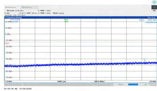
NTNV-DC_5A_n78A-PC2-30-5+80-M+M-QPSK-IDLE-DFT-QPSK-In ner_1RB_Left-1000-3000-PASS
