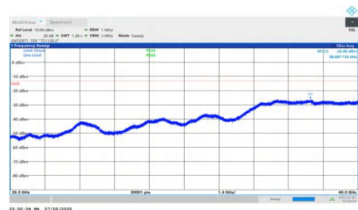
NTNV-DC_5A_n78A-PC2-30-5+80-M+L-QPSK-IDLE-DFT-QPSK-In ner_1RB_Right-26000-40000-PASS
