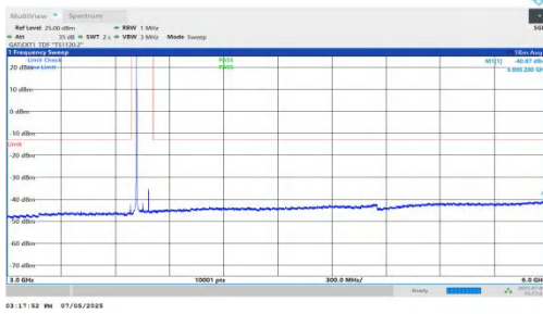
NTNV-DC_5A_n78A-PC2-30-5+70-M+M-QPSK-IDLE-DFT-BPSK-Inner_1RB_Left-3000-6000-PASS
