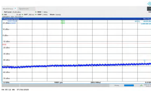
NTNV-DC_5A_n78A-PC2-30-5+80-M+H-QPSK-IDLE-DFT-QPSK-Inner_1RB_Right-1000-3000-PASS
