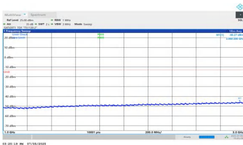
NTNV-DC_5A_n78A-PC2-30-5+70-M+M-QPSK-IDLE-DFT-QPSK-Inner_1RB_Right-1000-3000-PASS
