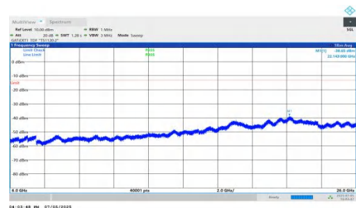
NTNV-DC_5A_n78A-PC2-30-5+80-M+H-QPSK-IDLE-DFT-QPSK-Inner_1RB_Left-6000-26000-PASS
