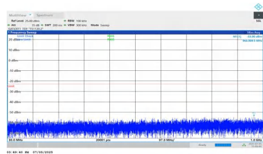
NTNV-DC_5A_n78A-PC2-30-5+80-M+L-QPSK-IDLE-DFT-QPSK-In ner_1RB_Right-30-1000-PASS
