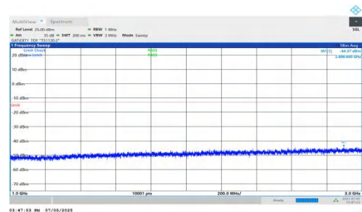
NTNV-DC_5A_n78A-PC2-30-5+80-M+L-QPSK-IDLE-DFT-QPSK-In ner_1RB_Left-1000-3000-PASS
