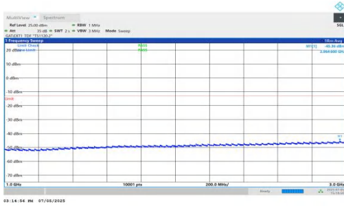
NTNV-DC_5A_n78A-PC2-30-5+70-M+L-QPSK-IDLE-DFT-QPSK-Inner_1RB_Right-1000-3000-PASS
