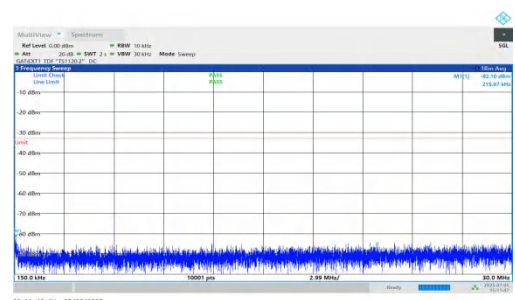
NTNV-DC_5A_n78A-PC2-30-5+70-M+L-QPSK-IDLE-DFT-QPSK-In ner_1RB_Left-0.15-30-PASS
