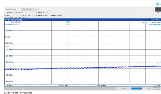
NTNV-DC_5A_n78A-PC2-30-5+70-M+H-QPSK-IDLE-DFT-BPSK-In ner_1RB_Left-1000-3000-PASS
