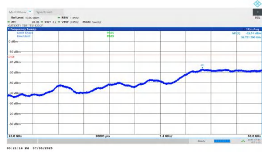
NTNV-DC_5A_n78A-PC2-30-5+70-M+M-QPSK-IDLE-DFT-BPSK-Inner_1RB_Right-26000-40000-PASS
