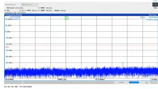
NTNV-DC_5A_n78A-PC2-30-5+80-M+M-QPSK-IDLE-DFT-BPSK-In ner_1RB_Right-30-1000-PASS
