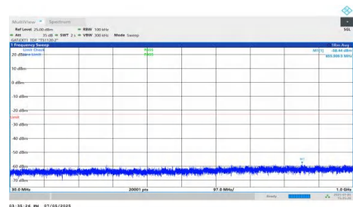
NTNV-DC_5A_n78A-PC2-30-5+70-M+H-QPSK-IDLE-DFT-QPSK-Inner_1RB_Right-30-1000-PASS
