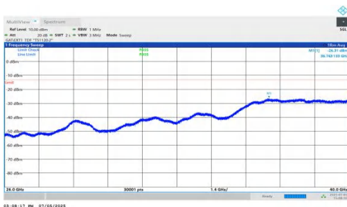
NTNV-DC_5A_n78A-PC2-30-5+70-M+L-QPSK-IDLE-DFT-BPSK-In ner_1RB_Left-26000-40000-PASS
