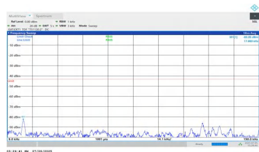
NTNV-DC_5A_n78A-PC2-30-5+70-M+H-QPSK-IDLE-DFT-BPSK-In ner_1RB_Right-0.009-0.15-PASS
