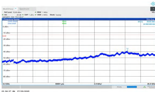
NTNV-DC_5A_n78A-PC2-30-5+80-M+M-QPSK-IDLE-DFT-BPSK-I nner_1RB_Right-6000-26000-PASS
