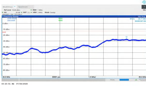
NTNV-DC_5A_n78A-PC2-30-5+70-M+M-QPSK-IDLE-DFT-QPSK-Inner_1RB_Left-26000-40000-PASS
