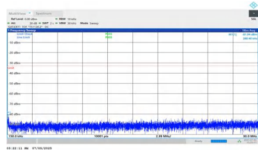
NTNV-DC_5A_n78A-PC2-30-5+70-M+M-QPSK-IDLE-DFT-QPSK-Inner_1RB_Left-0.15-30-PASS
