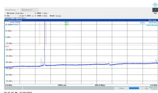
NTNV-DC_5A_n78A-PC2-30-5+70-M+M-QPSK-IDLE-DFT-BPSK-Inner_1RB_Right-3000-6000-PASS
