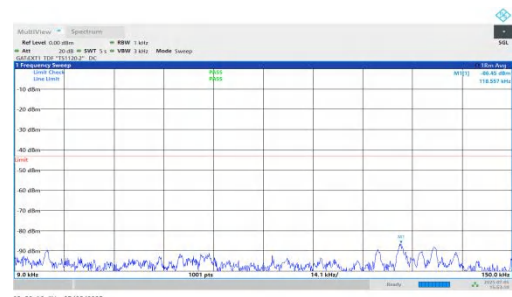
NTNV-DC_5A_n78A-PC2-30-5+80-M+M-QPSK-IDLE-DFT-BPSK-In ner_1RB_Right-0.009-0.15-PASS
