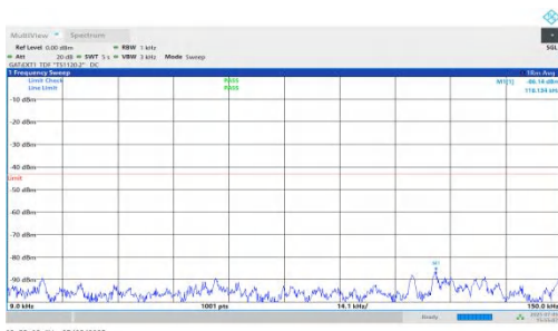
NTNV-DC_5A_n78A-PC2-30-5+80-M+M-QPSK-IDLE-DFT-QPSK-I nner_1RB_Left-0.009-0.15-PASS
