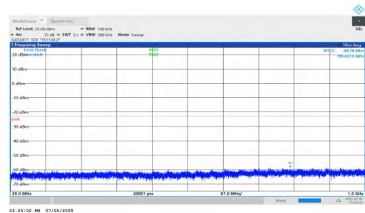
NTNV-DC_5A_n78A-PC2-30-5+70-M+M-QPSK-IDLE-DFT-QPSK-Inner_1RB_Right-30-1000-PASS
