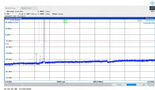
NTNV-DC_5A_n78A-PC2-30-5+80-M+M-QPSK-IDLE-DFT-BPSK-In ner_1RB_Right-3000-6000-PASS
