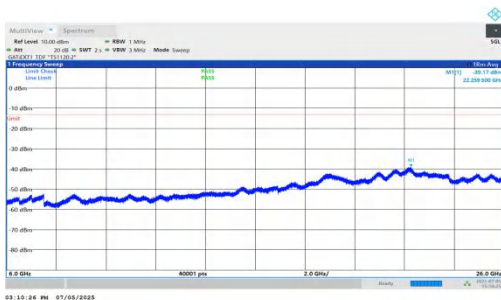
NTNV-DC_5A_n78A-PC2-30-5+70-M+L-QPSK-IDLE-DFT-BPSK-In ner_1RB_Right-6000-26000-PASS
