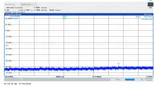
NTNV-DC_5A_n78A-PC2-30-5+70-M+L-QPSK-IDLE-DFT-BPSK-In ner_1RB_Right-30-1000-PASS
