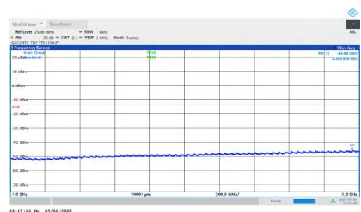
NTNV-DC_5A_n78A-PC2-30-5+70-M+M-QPSK-IDLE-DFT-BPSK-Inner_1RB_Left-1000-3000-PASS
