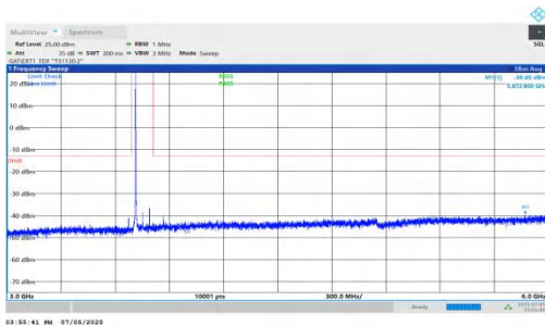
NTNV-DC_5A_n78A-PC2-30-5+80-M+M-QPSK-IDLE-DFT-QPSK-I nner_1RB_Left-3000-6000-PASS
