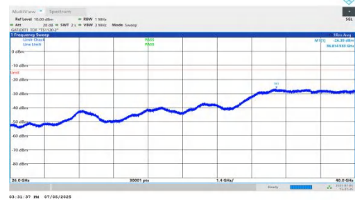
NTNV-DC_5A_n78A-PC2-30-5+70-M+H-QPSK-IDLE-DFT-BPSK-Inner_1RB_Right-26000-40000-PASS
