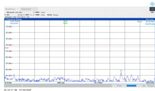
NTNV-DC_5A_n78A-PC2-30-5+70-M+M-QPSK-IDLE-DFT-BPSK-Inner_1RB_Right-0.009-0.15-PASS
