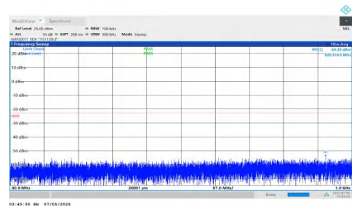
NTNV-DC_5A_n78A-PC2-30-5+80-M+L-QPSK-IDLE-DFT-BPSK-In ner_1RB_Right-30-1000-PASS
