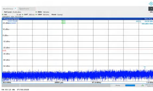
NTNV-DC_5A_n78A-PC2-30-5+80-M+H-QPSK-IDLE-DFT-QPSK-Inner_1RB_Left-30-1000-PASS
