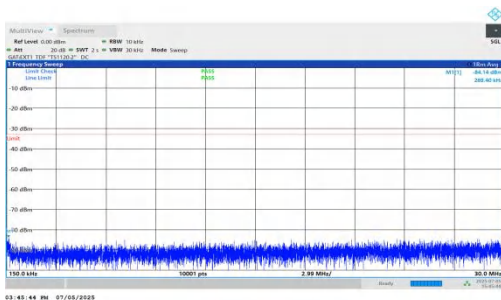
NTNV-DC_5A_n78A-PC2-30-5+80-M+L-QPSK-IDLE-DFT-BPSK-In ner_1RB_Right-0.15-30-PASS
