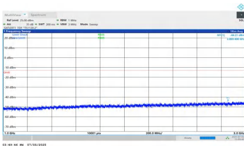
NTNV-DC_5A_n78A-PC2-30-5+80-M+L-QPSK-IDLE-DFT-QPSK-In ner_1RB_Right-1000-3000-PASS
