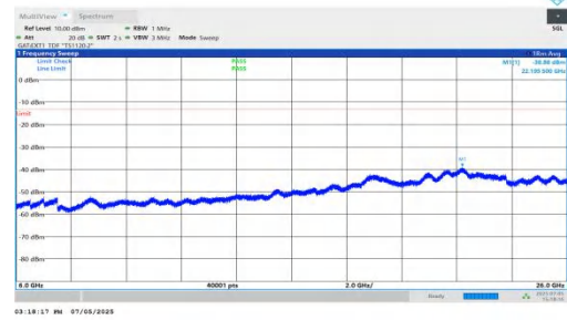
NTNV-DC_5A_n78A-PC2-30-5+70-M+M-QPSK-IDLE-DFT-BPSK-Inner_1RB_Left-6000-26000-PASS
