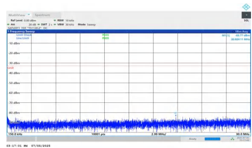
NTNV-DC_5A_n78A-PC2-30-5+70-M+M-QPSK-IDLE-DFT-BPSK-Inner_1RB_Left-0.15-30-PASS
