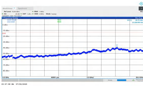
NTNV-DC_5A_n78A-PC2-30-5+80-M+M-QPSK-IDLE-DFT-QPSK-Inner_1RB_Right-6000-26000-PASS
