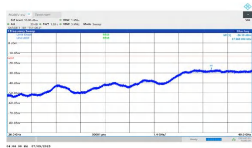
NTNV-DC_5A_n78A-PC2-30-5+80-M+H-QPSK-IDLE-DFT-QPSK-Inner_1RB_Right-26000-40000-PASS
