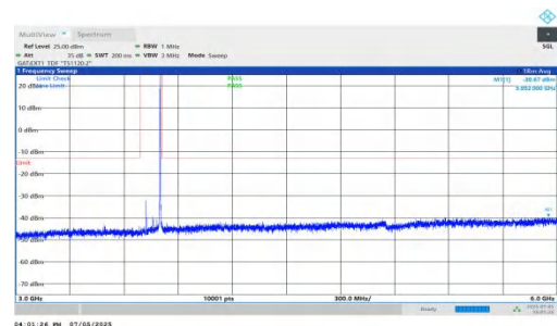
NTNV-DC_5A_n78A-PC2-30-5+80-M+H-QPSK-IDLE-DFT-BPSK-In ner_1RB_Right-3000-6000-PASS
