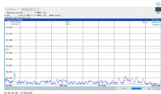
NTNV-DC_5A_n78A-PC2-30-5+80-M+L-QPSK-IDLE-DFT-BPSK-In ner_1RB_Right-0.009-0.15-PASS
