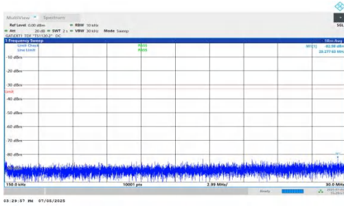
NTNV-DC_5A_n78A-PC2-30-5+70-M+H-QPSK-IDLE-DFT-BPSK-Inner_1RB_Right-0.15-30-PASS
