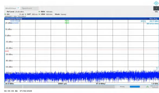
NTNV-DC_5A_n78A-PC2-30-5+80-M+H-QPSK-IDLE-DFT-QPSK-Inner_1RB_Right-30-1000-PASS
