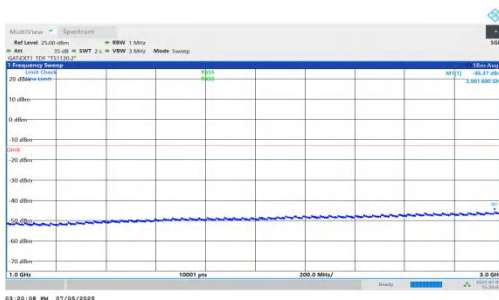
NTNV-DC_5A_n78A-PC2-30-5+70-M+M-QPSK-IDLE-DFT-BPSK-Inner_1RB_Right-1000-3000-PASS
