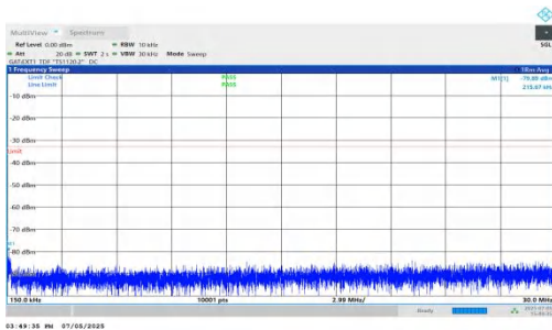
NTNV-DC_5A_n78A-PC2-30-5+80-M+L-QPSK-IDLE-DFT-QPSK-In ner_1RB_Right-0.15-30-PASS
