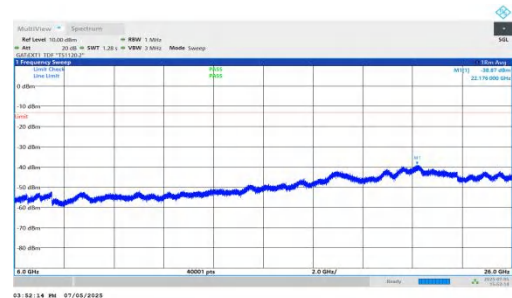
NTNV-DC_5A_n78A-PC2-30-5+80-M+M-QPSK-IDLE-DFT-BPSK-In ner_1RB_Left-6000-26000-PASS
