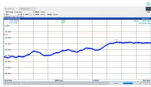
NTNV-DC_5A_n78A-PC2-30-5+60-M+H-QPSK-IDLE-DFT-QPSK-Inner_1RB_Right-26000-40000-PASS
