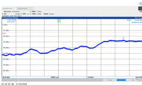
NTNV-DC_5A_n78A-PC2-30-5+70-M+M-QPSK-IDLE-DFT-BPSK-Inner_1RB_Left-26000-40000-PASS
