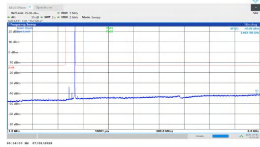
NTNV-DC_5A_n78A-PC2-30-5+70-M+H-QPSK-IDLE-DFT-QPSK-Inner_1RB_Right-3000-6000-PASS
