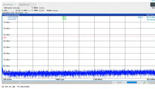
NTNV-DC_5A_n78A-PC2-30-5+70-M+L-QPSK-IDLE-DFT-BPSK-In ner_1RB_Right-0.15-30-PASS
