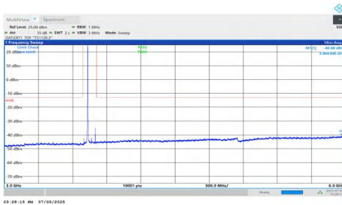
NTNV-DC_5A_n78A-PC2-30-5+70-M+H-QPSK-IDLE-DFT-BPSK-I nner_1RB_Left-3000-6000-PASS
