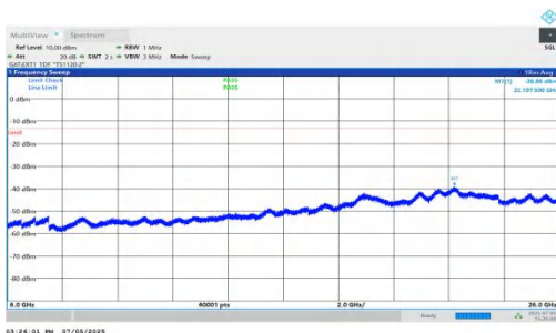
NTNV-DC_5A_n78A-PC2-30-5+70-M+M-QPSK-IDLE-DFT-QPSK-Inner_1RB_Right-6000-26000-PASS
