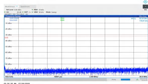
NTNV-DC_5A_n78A-PC2-30-5+70-M+H-QPSK-IDLE-DFT-QPSK-Inner_1RB_Left-0.15-30-PASS
