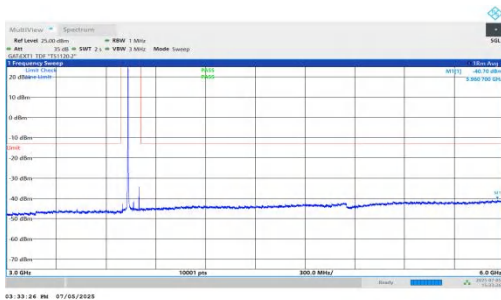
NTNV-DC_5A_n78A-PC2-30-5+70-M+H-QPSK-IDLE-DFT-QPSK-Inner_1RB_Left-3000-6000-PASS
