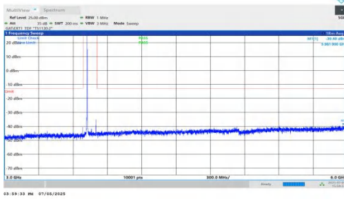
NTNV-DC_5A_n78A-PC2-30-5+80-M+H-QPSK-IDLE-DFT-BPSK-I nner_1RB_Left-3000-6000-PASS
