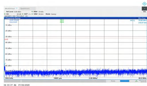
NTNV-DC_5A_n78A-PC2-30-5+80-M+H-QPSK-IDLE-DFT-QPSK-Inner_1RB_Left-0.15-30-PASS
