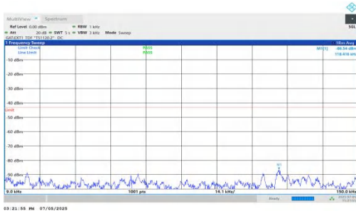
NTNV-DC_5A_n78A-PC2-30-5+70-M+M-QPSK-IDLE-DFT-QPSK-Inner_1RB_Left-0.009-0.15-PASS
