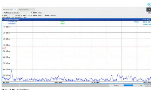
NTNV-DC_5A_n78A-PC2-30-5+70-M+H-QPSK-IDLE-DFT-QPSK-Inner_1RB_Left-0.009-0.15-PASS
