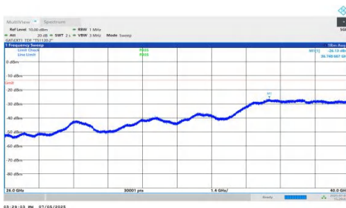
NTNV-DC_5A_n78A-PC2-30-5+70-M+H-QPSK-IDLE-DFT-BPSK-I nner_1RB_Left-26000-40000-PASS
