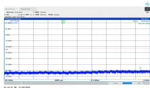
NTNV-DC_5A_n78A-PC2-30-5+70-M+M-QPSK-IDLE-DFT-BPSK-Inner_1RB_Right-30-1000-PASS
