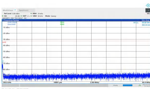
NTNV-DC_5A_n78A-PC2-30-5+70-M+L-QPSK-IDLE-DFT-QPSK-In ner_1RB_Right-0.15-30-PASS
