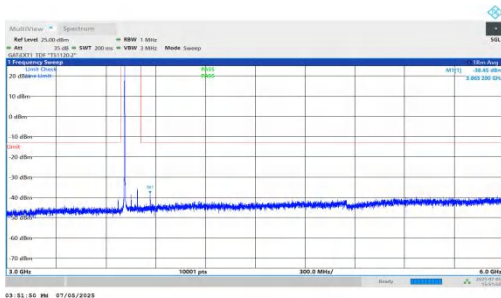
NTNV-DC_5A_n78A-PC2-30-5+80-M+M-QPSK-IDLE-DFT-BPSK-I nner_1RB_Left-3000-6000-PASS
