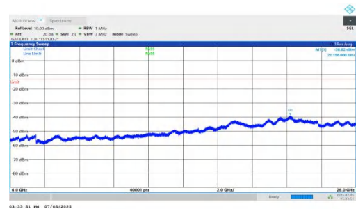
NTNV-DC_5A_n78A-PC2-30-5+70-M+H-QPSK-IDLE-DFT-QPSK-Inner_1RB_Left-6000-26000-PASS
