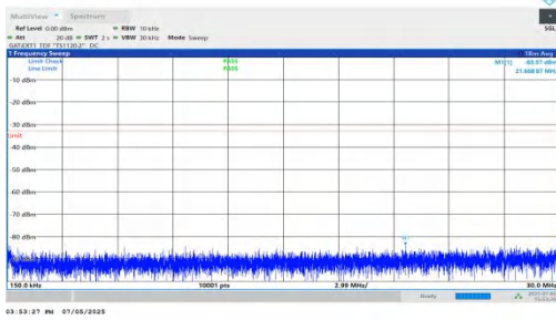
NTNV-DC_5A_n78A-PC2-30-5+80-M+M-QPSK-IDLE-DFT-BPSK-I nner_1RB_Right-0.15-30-PASS
