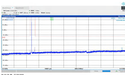
NTNV-DC_5A_n78A-PC2-30-5+80-M+H-QPSK-IDLE-DFT-QPSK-Inner_1RB_Left-3000-6000-PASS
