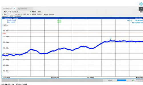
NTNV-DC_5A_n78A-PC2-30-5+70-M+H-QPSK-IDLE-DFT-QPSK-Inner_1RB_Left-26000-40000-PASS
