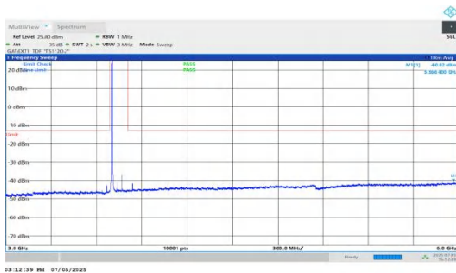
NTNV-DC_5A_n78A-PC2-30-5+70-M+L-QPSK-IDLE-DFT-QPSK-In ner_1RB_Left-3000-6000-PASS
