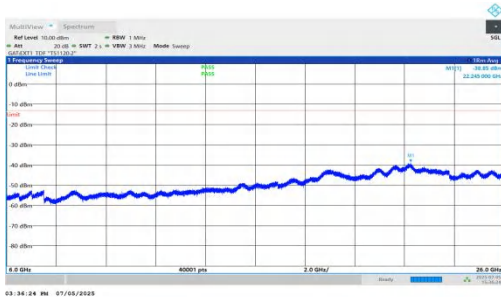
NTNV-DC_5A_n78A-PC2-30-5+70-M+H-QPSK-IDLE-DFT-QPSK-Inner_1RB_Right-6000-26000-PASS
