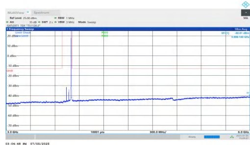
NTNV-DC_5A_n78A-PC2-30-5+60-M+H-QPSK-IDLE-DFT-QPSK-Inner_1RB_Right-3000-6000-PASS
