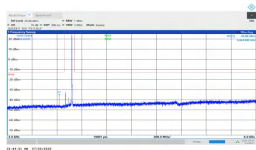
NTNV-DC_5A_n78A-PC2-30-5+80-M+L-QPSK-IDLE-DFT-QPSK-In ner_1RB_Right-3000-6000-PASS
