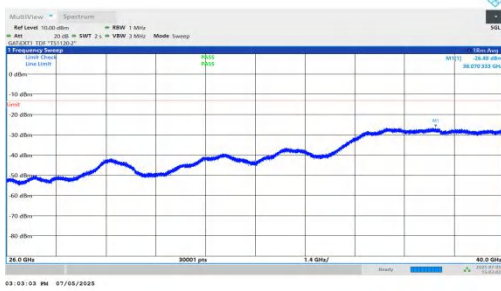
NTNV-DC_5A_n78A-PC2-30-5+60-M+H-QPSK-IDLE-DFT-QPSK-Inner_1RB_Left-26000-40000-PASS
