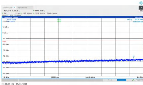
NTNV-DC_5A_n78A-PC2-30-5+80-M+M-QPSK-IDLE-DFT-BPSK-I nner_1RB_Right-1000-3000-PASS
