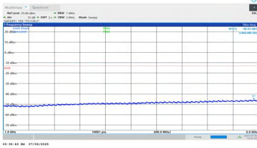
NTNV-DC_5A_n78A-PC2-30-5+70-M+H-QPSK-IDLE-DFT-QPSK-Inner_1RB_Right-1000-3000-PASS
