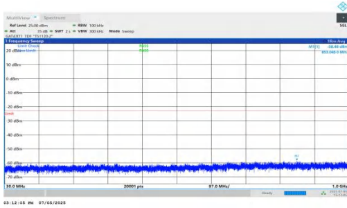
NTNV-DC_5A_n78A-PC2-30-5+70-M+L-QPSK-IDLE-DFT-QPSK-In ner_1RB_Left-30-1000-PASS
