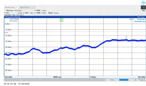
NTNV-DC_5A_n78A-PC2-30-5+80-M+H-QPSK-IDLE-DFT-BPSK-Inner_1RB_Right-26000-40000-PASS
