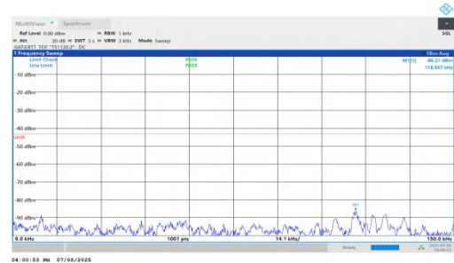
NTNV-DC_5A_n78A-PC2-30-5+80-M+H-QPSK-IDLE-DFT-BPSK-In ner_1RB_Right-0.009-0.15-PASS
