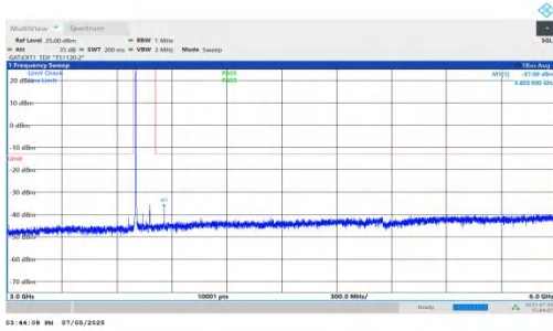
NTNV-DC_5A_n78A-PC2-30-5+80-M+L-QPSK-IDLE-DFT-BPSK-In ner_1RB_Left-3000-6000-PASS
