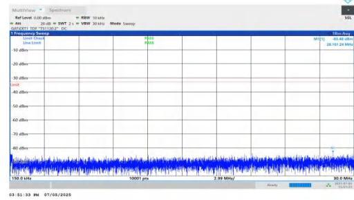
NTNV-DC_5A_n78A-PC2-30-5+80-M+M-QPSK-IDLE-DFT-BPSK-In ner_1RB_Left-0.15-30-PASS
