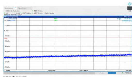
NTNV-DC_5A_n78A-PC2-30-5+80-M+L-QPSK-IDLE-DFT-BPSK-Inner_1RB_Left-1000-3000-PASS
