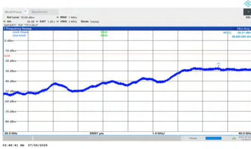
NTNV-DC_5A_n78A-PC2-30-5+80-M+L-QPSK-IDLE-DFT-QPSK-In ner_1RB_Left-26000-40000-PASS
