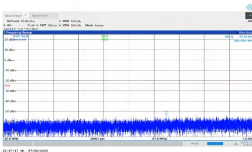
NTNV-DC_5A_n78A-PC2-30-5+80-M+L-QPSK-IDLE-DFT-QPSK-In ner_1RB_Left-30-1000-PASS
