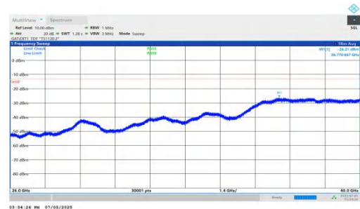
NTNV-DC_5A_n78A-PC2-30-5+80-M+M-QPSK-IDLE-DFT-BPSK-In ner_1RB_Right-26000-40000-PASS
