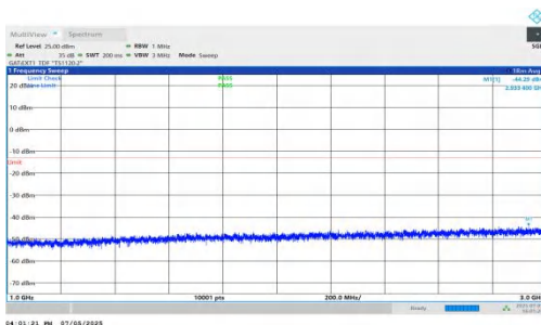
NTNV-DC_5A_n78A-PC2-30-5+80-M+H-QPSK-IDLE-DFT-BPSK-I nner_1RB_Right-1000-3000-PASS
