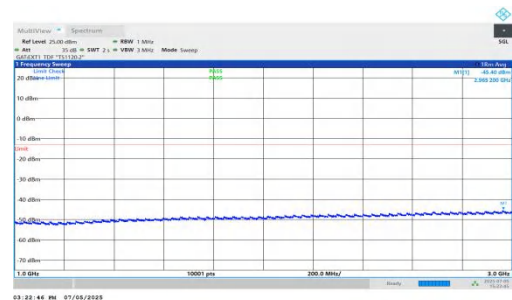
NTNV-DC_5A_n78A-PC2-30-5+70-M+M-QPSK-IDLE-DFT-QPSK-Inner_1RB_Left-1000-3000-PASS
