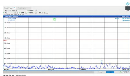
NTNV-DC_5A_n78A-PC2-30-5+70-M+L-QPSK-IDLE-DFT-BPSK-In ner_1RB_Right-0.009-0.15-PASS
