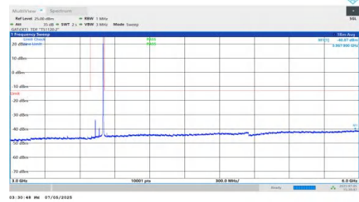
NTNV-DC_5A_n78A-PC2-30-5+70-M+H-QPSK-IDLE-DFT-BPSK-Inner_1RB_Right-3000-6000-PASS
