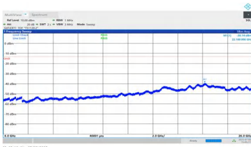
NTNV-DC_5A_n78A-PC2-30-5+60-M+H-QPSK-IDLE-DFT-QPSK-Inner_1RB_Right-6000-26000-PASS
