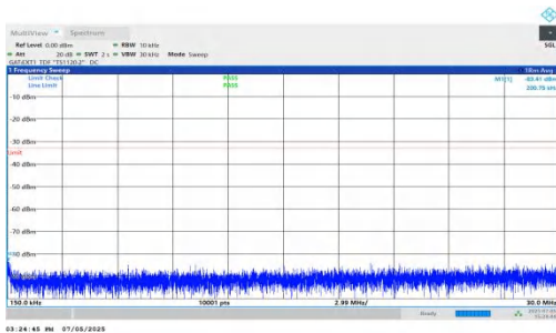
NTNV-DC_5A_n78A-PC2-30-5+70-M+M-QPSK-IDLE-DFT-QPSK-Inner_1RB_Right-0.15-30-PASS
