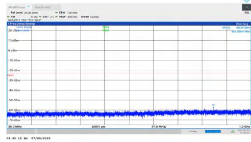
NTNV-DC_5A_n78A-PC2-30-5+70-M+H-QPSK-IDLE-DFT-BPSK-Inner_1RB_Right-30-1000-PASS
