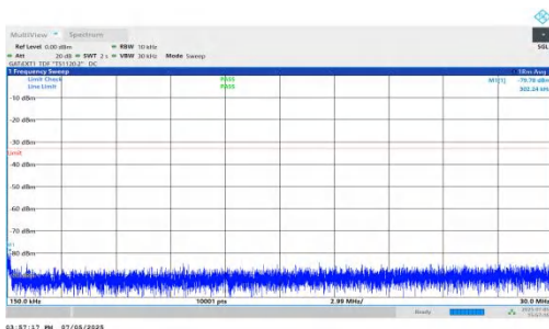
NTNV-DC_5A_n78A-PC2-30-5+80-M+M-QPSK-IDLE-DFT-QPSK-I nner_1RB_Right-0.15-30-PASS
