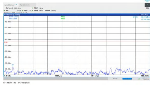
NTNV-DC_5A_n78A-PC2-30-5+60-M+H-QPSK-IDLE-DFT-QPSK-Inner_1RB_Right-0.009-0.15-PASS
