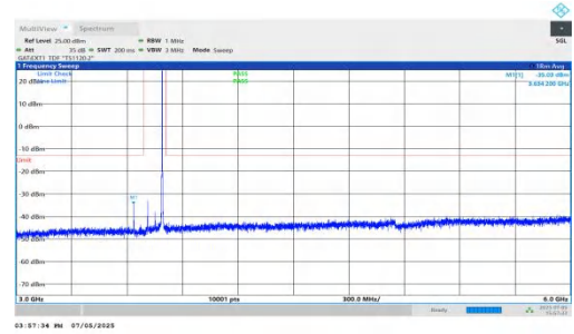
NTNV-DC_5A_n78A-PC2-30-5+80-M+M-QPSK-IDLE-DFT-QPSK-Inner_1RB_Right-3000-6000-PASS
