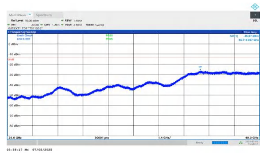
NTNV-DC_5A_n78A-PC2-30-5+80-M+M-QPSK-IDLE-DFT-QPSK-Inner_1RB_Right-26000-40000-PASS
