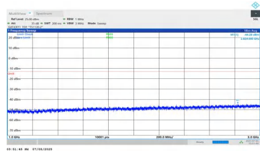
NTNV-DC_5A_n78A-PC2-30-5+80-M+M-QPSK-IDLE-DFT-BPSK-In ner_1RB_Left-1000-3000-PASS
