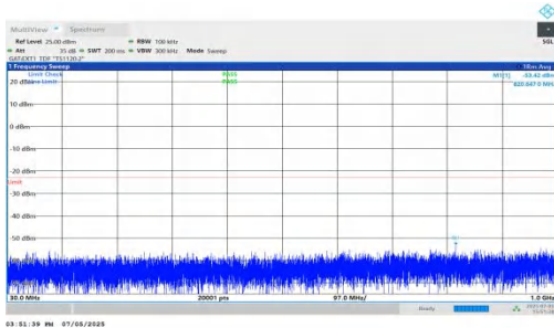
NTNV-DC_5A_n78A-PC2-30-5+80-M+M-QPSK-IDLE-DFT-BPSK-I nner_1RB_Left-30-1000-PASS
