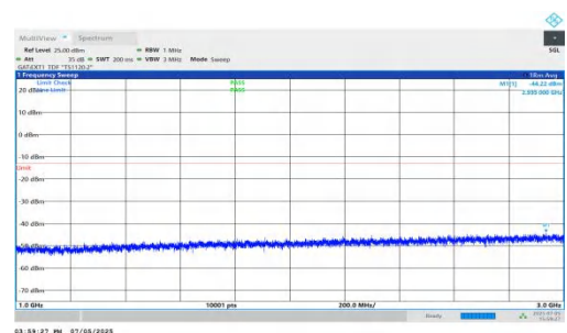
NTNV-DC_5A_n78A-PC2-30-5+80-M+H-QPSK-IDLE-DFT-BPSK-Inner_1RB_Left-1000-3000-PASS
