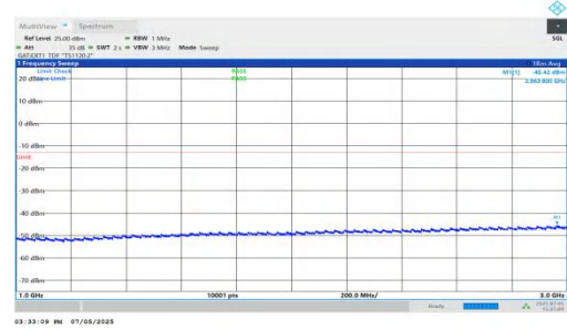
NTNV-DC_5A_n78A-PC2-30-5+70-M+H-QPSK-IDLE-DFT-QPSK-Inner_1RB_Left-1000-3000-PASS
