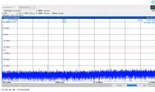
NTNV-DC_5A_n78A-PC2-30-5+80-M+M-QPSK-IDLE-DFT-QPSK-I nner_1RB_Left-30-1000-PASS
