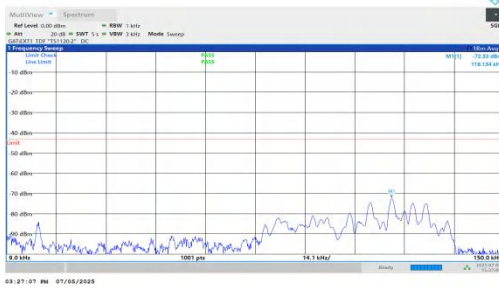
NTNV-DC_5A_n78A-PC2-30-5+70-M+H-QPSK-IDLE-DFT-BPSK-I nner_1RB_Left-0.009-0.15-PASS
