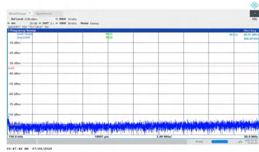
NTNV-DC_5A_n78A-PC2-30-5+80-M+L-QPSK-IDLE-DFT-QPSK-In ner_1RB_Left-0.15-30-PASS
