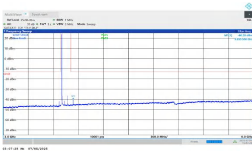
NTNV-DC_5A_n78A-PC2-30-5+70-M+L-QPSK-IDLE-DFT-BPSK-In ner_1RB_Left-3000-6000-PASS
