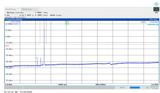
NTNV-DC_5A_n78A-PC2-30-5+70-M+L-QPSK-IDLE-DFT-BPSK-In ner_1RB_Right-3000-6000-PASS
