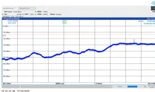
NTNV-DC_5A_n78A-PC2-30-5+80-M+H-QPSK-IDLE-DFT-BPSK-I nner_1RB_Left-26000-40000-PASS
