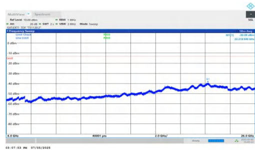
NTNV-DC_5A_n78A-PC2-30-5+70-M+L-QPSK-IDLE-DFT-BPSK-In ner_1RB_Left-6000-26000-PASS
