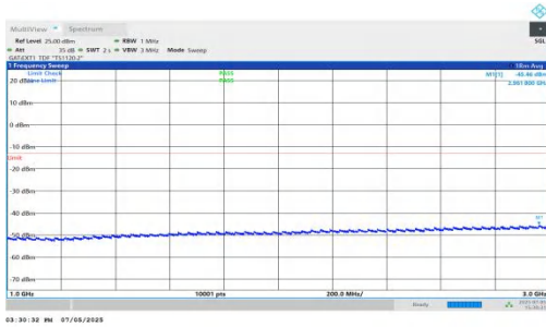
NTNV-DC_5A_n78A-PC2-30-5+70-M+H-QPSK-IDLE-DFT-BPSK-Inner_1RB_Right-1000-3000-PASS
