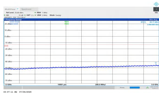
NTNV-DC_5A_n78A-PC2-30-5+70-M+L-QPSK-IDLE-DFT-BPSK-In ner_1RB_Left-1000-3000-PASS
