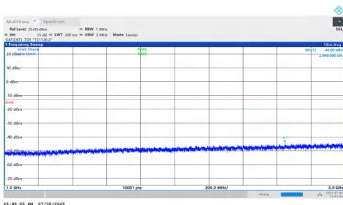
NTNV-DC_5A_n78A-PC2-30-5+80-M+L-QPSK-IDLE-DFT-BPSK-In ner_1RB_Right-1000-3000-PASS
