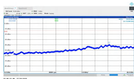
NTNV-DC_5A_n78A-PC2-30-5+80-M+L-QPSK-IDLE-DFT-QPSK-In ner_1RB_Left-6000-26000-PASS
