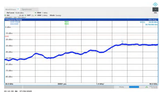
NTNV-DC_5A_n78A-PC2-30-5+70-M+L-QPSK-IDLE-DFT-BPSK-In ner_1RB_Right-26000-40000-PASS
