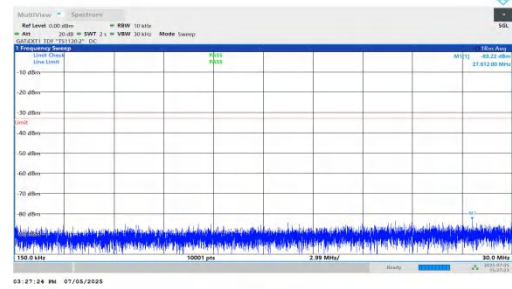
NTNV-DC_5A_n78A-PC2-30-5+70-M+H-QPSK-IDLE-DFT-BPSK-In ner_1RB_Left-0.15-30-PASS
