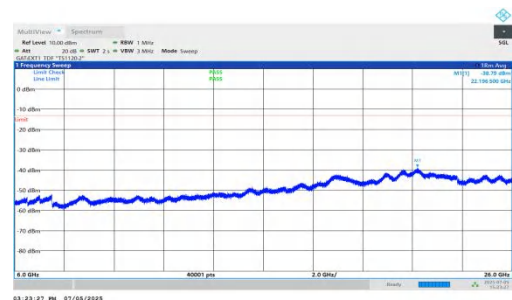
NTNV-DC_5A_n78A-PC2-30-5+70-M+M-QPSK-IDLE-DFT-QPSK-Inner_1RB_Left-6000-26000-PASS
