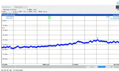
NTNV-DC_5A_n78A-PC2-30-5+80-M+H-QPSK-IDLE-DFT-QPSK-Inner_1RB_Right-6000-26000-PASS
