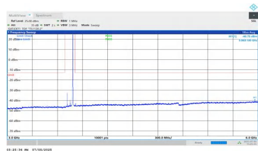
NTNV-DC_5A_n78A-PC2-30-5+70-M+M-QPSK-IDLE-DFT-QPSK-Inner_1RB_Right-3000-6000-PASS
