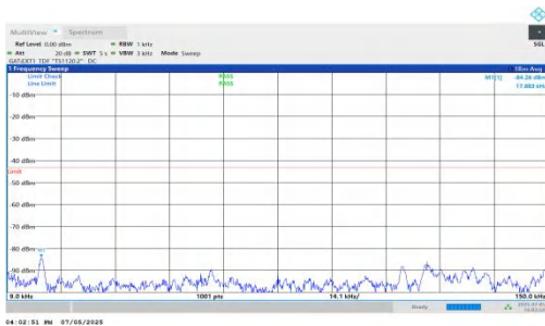
NTNV-DC_5A_n78A-PC2-30-5+80-M+H-QPSK-IDLE-DFT-QPSK-Inner_1RB_Left-0.009-0.15-PASS
