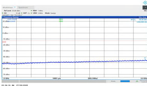
NTNV-DC_5A_n78A-PC2-30-5+60-M+H-QPSK-IDLE-DFT-QPSK-Inner_1RB_Right-1000-3000-PASS
