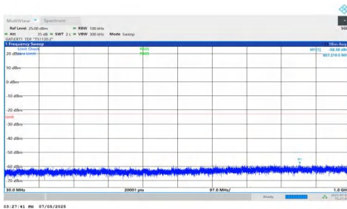
NTNV-DC_5A_n78A-PC2-30-5+70-M+H-QPSK-IDLE-DFT-BPSK-I nner_1RB_Left-30-1000-PASS
