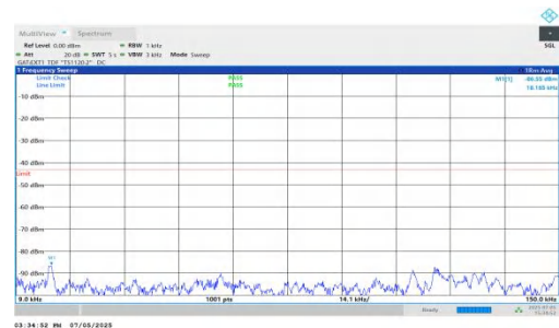
NTNV-DC_5A_n78A-PC2-30-5+70-M+H-QPSK-IDLE-DFT-QPSK-Inner_1RB_Right-0.009-0.15-PASS
