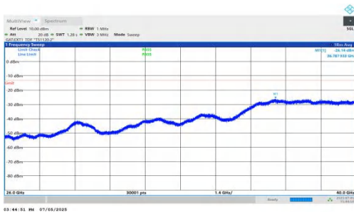
NTNV-DC_5A_n78A-PC2-30-5+80-M+L-QPSK-IDLE-DFT-BPSK-In ner_1RB_Left-26000-40000-PASS
