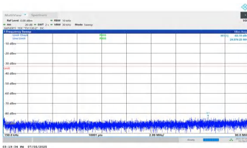
NTNV-DC_5A_n78A-PC2-30-5+70-M+M-QPSK-IDLE-DFT-BPSK-Inner_1RB_Right-0.15-30-PASS
