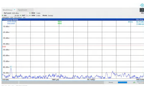
NTNV-DC_5A_n78A-PC2-30-5+70-M+L-QPSK-IDLE-DFT-QPSK-In ner_1RB_Left-0.009-0.15-PASS
