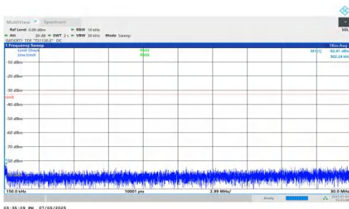
NTNV-DC_5A_n78A-PC2-30-5+70-M+H-QPSK-IDLE-DFT-QPSK-Inner_1RB_Right-0.15-30-PASS
