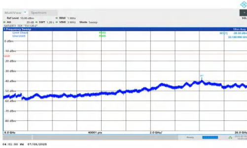
NTNV-DC_5A_n78A-PC2-30-5+80-M+H-QPSK-IDLE-DFT-BPSK-Inner_1RB_Right-6000-26000-PASS
