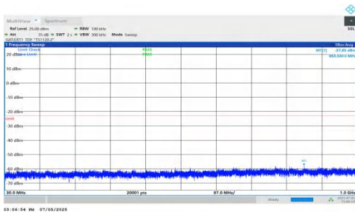
NTNV-DC_5A_n78A-PC2-30-5+70-M+L-QPSK-IDLE-DFT-BPSK-In ner_1RB_Left-30-1000-PASS
