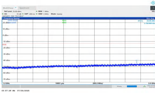
NTNV-DC_5A_n78A-PC2-30-5+80-M+M-QPSK-IDLE-DFT-QPSK-Inner_1RB_Right-1000-3000-PASS
