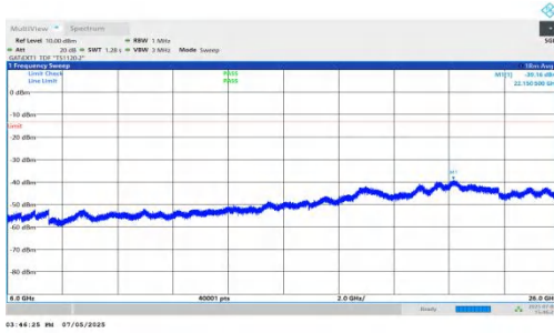
NTNV-DC_5A_n78A-PC2-30-5+80-M+L-QPSK-IDLE-DFT-BPSK-In ner_1RB_Right-6000-26000-PASS
