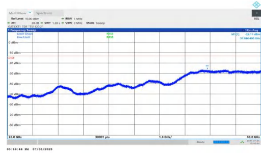
NTNV-DC_5A_n78A-PC2-30-5+80-M+L-QPSK-IDLE-DFT-BPSK-In ner_1RB_Right-26000-40000-PASS
