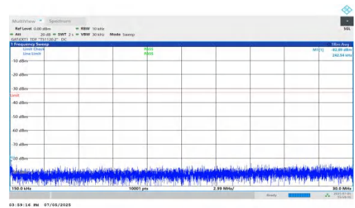
NTNV-DC_5A_n78A-PC2-30-5+80-M+H-QPSK-IDLE-DFT-BPSK-Inner_1RB_Left-0.15-30-PASS
