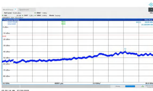
NTNV-DC_5A_n78A-PC2-30-5+80-M+L-QPSK-IDLE-DFT-QPSK-In ner_1RB_Right-6000-26000-PASS
