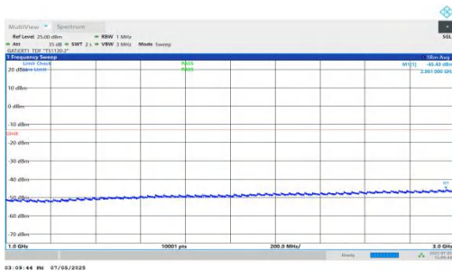
NTNV-DC_5A_n78A-PC2-30-5+70-M+L-QPSK-IDLE-DFT-BPSK-In ner_1RB_Right-1000-3000-PASS
