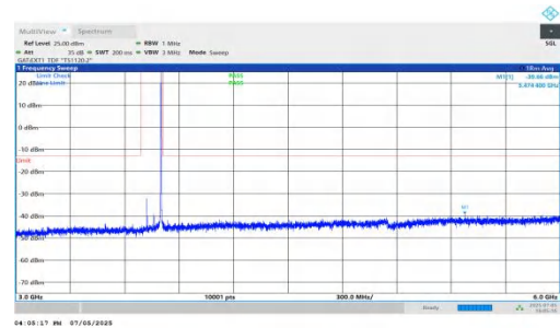
NTNV-DC_5A_n78A-PC2-30-5+80-M+H-QPSK-IDLE-DFT-QPSK-Inner_1RB_Right-3000-6000-PASS
