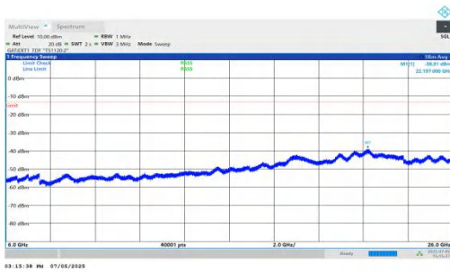
NTNV-DC_5A_n78A-PC2-30-5+70-M+L-QPSK-IDLE-DFT-QPSK-Inner_1RB_Right-6000-26000-PASS
