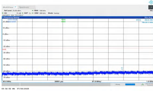
NTNV-DC_5A_n78A-PC2-30-5+70-M+H-QPSK-IDLE-DFT-QPSK-Inner_1RB_Left-30-1000-PASS
