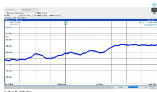
NTNV-DC_5A_n78A-PC2-30-5+70-M+M-QPSK-IDLE-DFT-QPSK-Inner_1RB_Right-26000-40000-PASS
