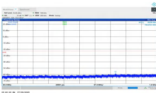
NTNV-DC_5A_n78A-PC2-30-5+70-M+M-QPSK-IDLE-DFT-QPSK-Inner_1RB_Left-30-1000-PASS
