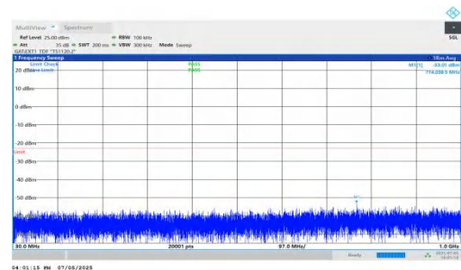
NTNV-DC_5A_n78A-PC2-30-5+80-M+H-QPSK-IDLE-DFT-BPSK-In ner_1RB_Right-30-1000-PASS
