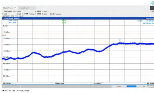
NTNV-DC_5A_n78A-PC2-30-5+80-M+H-QPSK-IDLE-DFT-QPSK-Inner_1RB_Left-26000-40000-PASS
