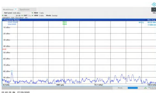
NTNV-DC_5A_n78A-PC2-30-5+80-M+L-QPSK-IDLE-DFT-BPSK-Inner_1RB_Left-0.009-0.15-PASS
