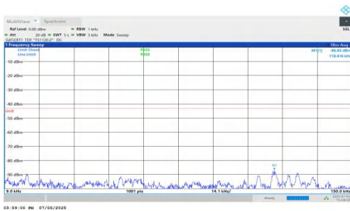
NTNV-DC_5A_n78A-PC2-30-5+80-M+H-QPSK-IDLE-DFT-BPSK-Inner_1RB_Left-0.009-0.15-PASS
