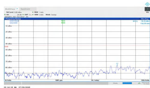
NTNV-DC_5A_n78A-PC2-30-5+70-M+L-QPSK-IDLE-DFT-QPSK-In ner_1RB_Right-0.009-0.15-PASS
