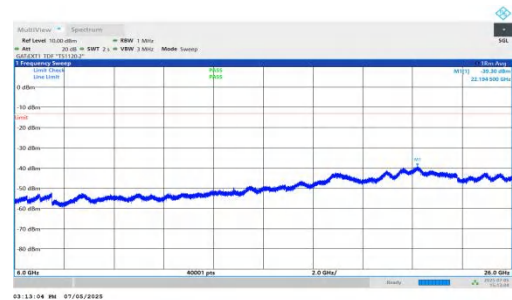
NTNV-DC_5A_n78A-PC2-30-5+70-M+L-QPSK-IDLE-DFT-QPSK-In ner_1RB_Left-6000-26000-PASS
