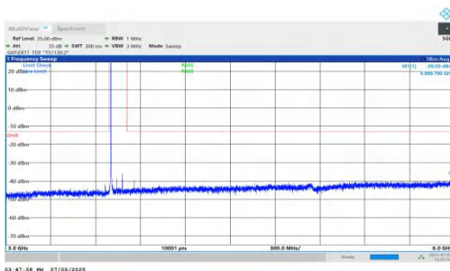
NTNV-DC_5A_n78A-PC2-30-5+80-M+L-QPSK-IDLE-DFT-QPSK-In ner_1RB_Left-3000-6000-PASS
