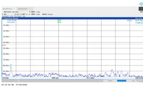
NTNV-DC_5A_n78A-PC2-30-5+70-M+M-QPSK-IDLE-DFT-BPSK-Inner_1RB_Left-0.009-0.15-PASS
