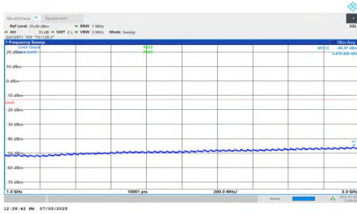
NTNV-DC_5A_n78A-PC2-30-5+20-M+H-QPSK-IDLE-DFT-QPSK-Inner_1RB_Right-1000-3000-PASS
