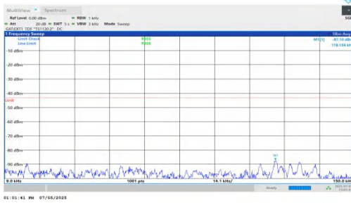
NTNV-DC_5A_n78A-PC2-30-5+30-M+L-QPSK-IDLE-DFT-BPSK-In ner_1RB_Left-0.009-0.15-PASS
