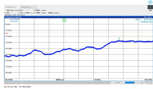
NTNV-DC_5A_n78A-PC2-30-5+20-M+M-QPSK-IDLE-DFT-BPSK-Inner_1RB_Right-26000-40000-PASS
