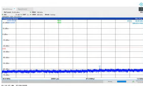
NTNV-DC_5A_n78A-PC2-30-5+30-M+M-QPSK-IDLE-DFT-BPSK-Inner_1RB_Left-30-1000-PASS
