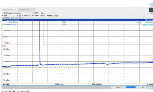
NTNV-DC_5A_n78A-PC2-30-5+30-M+M-QPSK-IDLE-DFT-QPSK-Inner_1RB_Left-3000-6000-PASS
