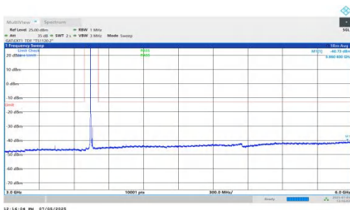
NTNV-DC_5A_n78A-PC2-30-5+20-M+M-QPSK-IDLE-DFT-QPSK-Inner_1RB_Left-3000-6000-PASS
