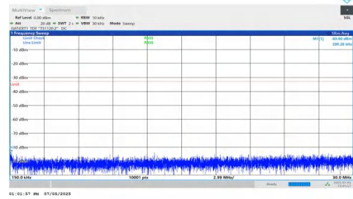
NTNV-DC_5A_n78A-PC2-30-5+30-M+L-QPSK-IDLE-DFT-BPSK-In ner_1RB_Left-0.15-30-PASS
