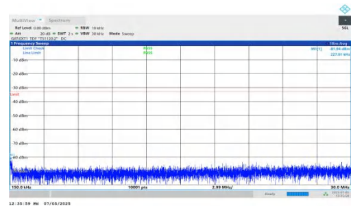
NTNV-DC_5A_n78A-PC2-30-5+25-M+L-QPSK-IDLE-DFT-QPSK-In ner_1RB_Left-0.15-30-PASS
