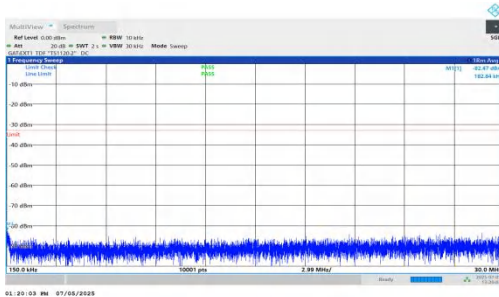
NTNV-DC_5A_n78A-PC2-30-5+30-M+M-QPSK-IDLE-DFT-QPSK-Inner_1RB_Right-0.15-30-PASS
