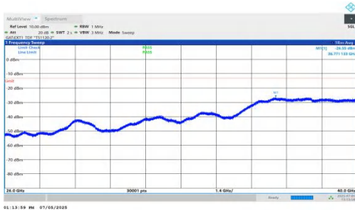
NTNV-DC_5A_n78A-PC2-30-5+30-M+M-QPSK-IDLE-DFT-BPSK-Inner_1RB_Left-26000-40000-PASS
