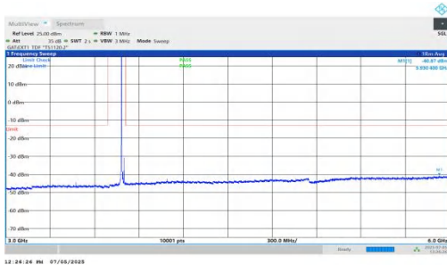
NTNV-DC_5A_n78A-PC2-30-5+20-M+H-QPSK-IDLE-DFT-QPSK-Inner_1RB_Left-3000-6000-PASS
