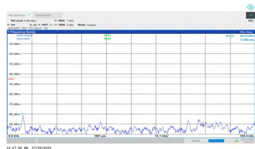
NTNV-DC_5A_n78A-PC2-30-5+20-M+H-QPSK-IDLE-DFT-QPSK-Inner_1RB_Right-0.009-0.15-PASS
