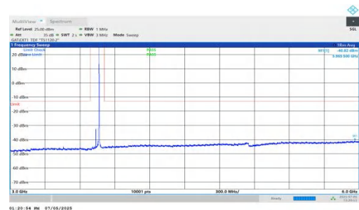
NTNV-DC_5A_n78A-PC2-30-5+30-M+M-QPSK-IDLE-DFT-QPSK-Inner_1RB_Right-3000-6000-PASS
