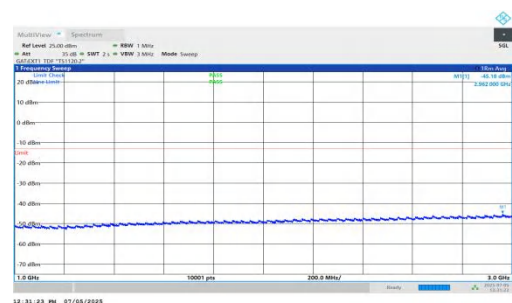
NTNV-DC_5A_n78A-PC2-30-5+25-M+L-QPSK-IDLE-DFT-BPSK-Inner_1RB_Left-1000-3000-PASS
