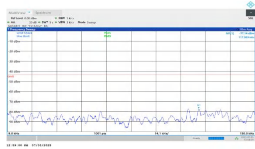
NTNV-DC_5A_n78A-PC2-30-5+25-M+H-QPSK-IDLE-DFT-QPSK-Inner_1RB_Right-0.009-0.15-PASS
