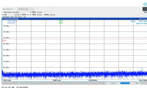
NTNV-DC_5A_n78A-PC2-30-5+20-M+M-QPSK-IDLE-DFT-BPSK-Inner_1RB_Right-0.15-30-PASS
