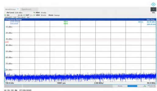
NTNV-DC_5A_n78A-PC2-30-5+25-M+H-QPSK-IDLE-DFT-BPSK-Inner_1RB_Left-0.15-30-PASS
