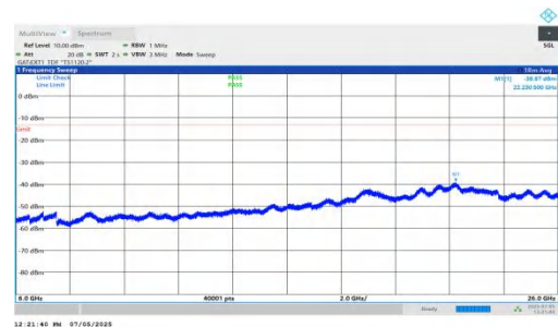
NTNV-DC_5A_n78A-PC2-30-5+20-M+H-QPSK-IDLE-DFT-BPSK-In ner_1RB_Left-6000-26000-PASS
