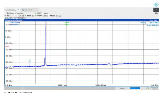
NTNV-DC_5A_n78A-PC2-30-5+25-M+H-QPSK-IDLE-DFT-BPSK-In ner_1RB_Right-3000-6000-PASS
