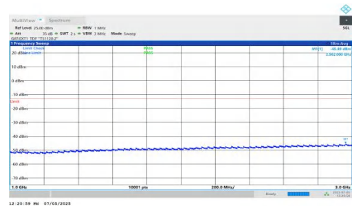
NTNV-DC_5A_n78A-PC2-30-5+20-M+H-QPSK-IDLE-DFT-BPSK-In ner_1RB_Left-1000-3000-PASS
