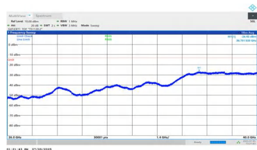
NTNV-DC_5A_n78A-PC2-30-5+30-M+M-QPSK-IDLE-DFT-QPSK-Inner_1RB_Right-26000-40000-PASS
