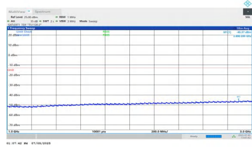
NTNV-DC_5A_n78A-PC2-30-5+30-M+L-QPSK-IDLE-DFT-QPSK-In ner_1RB_Left-1000-3000-PASS
