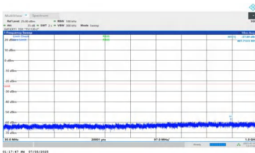
NTNV-DC_5A_n78A-PC2-30-5+30-M+M-QPSK-IDLE-DFT-QPSK-Inner_1RB_Left-30-1000-PASS
