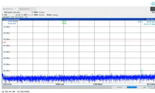
NTNV-DC_5A_n78A-PC2-30-5+25-M+H-QPSK-IDLE-DFT-BPSK-I nner_1RB_Right-0.15-30-PASS
