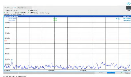
NTNV-DC_5A_n78A-PC2-30-5+30-M+H-QPSK-IDLE-DFT-QPSK-Inner_1RB_Right-0.009-0.15-PASS
