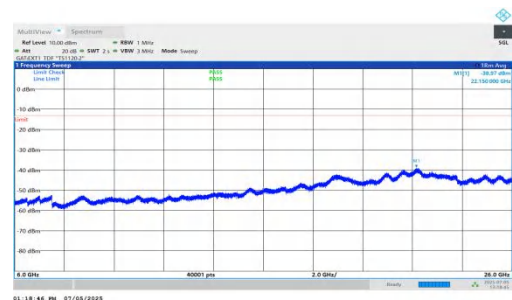
NTNV-DC_5A_n78A-PC2-30-5+30-M+M-QPSK-IDLE-DFT-QPSK-Inner_1RB_Left-6000-26000-PASS
