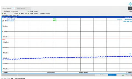
NTNV-DC_5A_n78A-PC2-30-5+25-M+H-QPSK-IDLE-DFT-BPSK-I nner_1RB_Right-1000-3000-PASS
