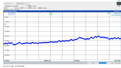
NTNV-DC_5A_n78A-PC2-30-5+20-M+M-QPSK-IDLE-DFT-BPSK-Inner_1RB_Left-6000-26000-PASS
