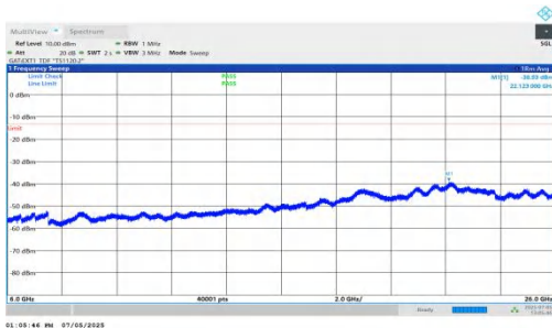
NTNV-DC_5A_n78A-PC2-30-5+30-M+L-QPSK-IDLE-DFT-BPSK-In ner_1RB_Right-6000-26000-PASS
