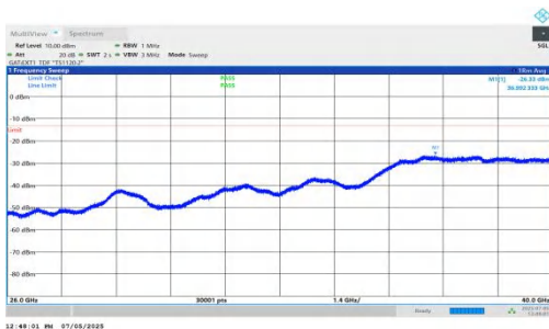
NTNV-DC_5A_n78A-PC2-30-5+25-M+M-QPSK-IDLE-DFT-QPSK-I nner_1RB_Left-26000-40000-PASS
