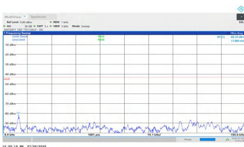
NTNV-DC_5A_n78A-PC2-30-5+20-M+H-QPSK-IDLE-DFT-QPSK-I nner_1RB_Left-0.009-0.15-PASS
