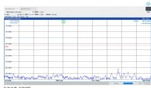
NTNV-DC_5A_n78A-PC2-30-5+30-M+L-QPSK-IDLE-DFT-BPSK-In ner_1RB_Right-0.009-0.15-PASS
