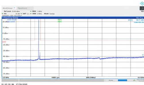
NTNV-DC_5A_n78A-PC2-30-5+30-M+H-QPSK-IDLE-DFT-BPSK-I nner_1RB_Left-3000-6000-PASS
