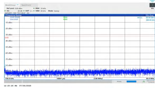
NTNV-DC_5A_n78A-PC2-30-5+20-M+H-QPSK-IDLE-DFT-BPSK-In ner_1RB_Left-0.15-30-PASS
