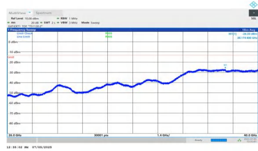
NTNV-DC_5A_n78A-PC2-30-5+25-M+L-QPSK-IDLE-DFT-BPSK-In ner_1RB_Right-26000-40000-PASS
