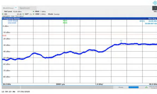
NTNV-DC_5A_n78A-PC2-30-5+25-M+H-QPSK-IDLE-DFT-QPSK-Inner_1RB_Left-26000-40000-PASS
