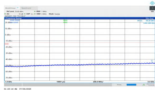
NTNV-DC_5A_n78A-PC2-30-5+30-M+H-QPSK-IDLE-DFT-BPSK-In ner_1RB_Left-1000-3000-PASS
