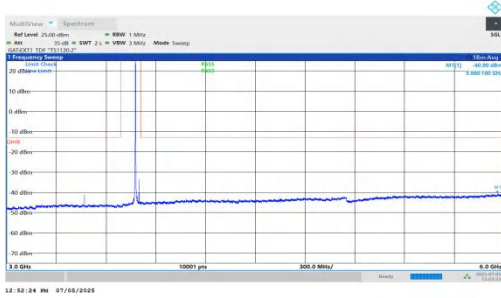
NTNV-DC_5A_n78A-PC2-30-5+25-M+H-QPSK-IDLE-DFT-BPSK-I nner_1RB_Left-3000-6000-PASS
