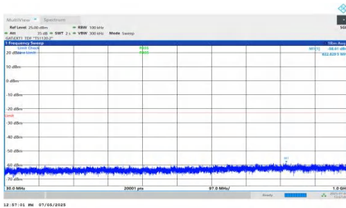
NTNV-DC_5A_n78A-PC2-30-5+25-M+H-QPSK-IDLE-DFT-QPSK-Inner_1RB_Left-30-1000-PASS
