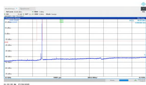
NTNV-DC_5A_n78A-PC2-30-5+25-M+H-QPSK-IDLE-DFT-QPSK-Inner_1RB_Right-3000-6000-PASS
