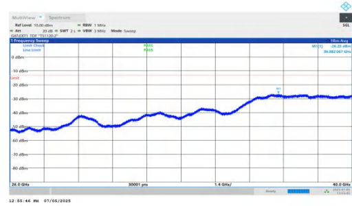
NTNV-DC_5A_n78A-PC2-30-5+25-M+H-QPSK-IDLE-DFT-BPSK-Inner_1RB_Right-26000-40000-PASS
