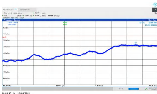
NTNV-DC_5A_n78A-PC2-30-5+30-M+L-QPSK-IDLE-DFT-QPSK-In ner_1RB_Left-26000-40000-PASS
