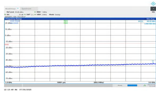
NTNV-DC_5A_n78A-PC2-30-5+20-M+M-QPSK-IDLE-DFT-QPSK-Inner_1RB_Left-1000-3000-PASS
