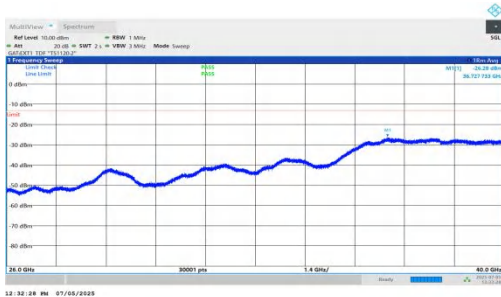
NTNV-DC_5A_n78A-PC2-30-5+25-M+L-QPSK-IDLE-DFT-BPSK-In ner_1RB_Left-26000-40000-PASS
