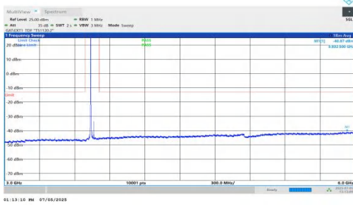
NTNV-DC_5A_n78A-PC2-30-5+30-M+M-QPSK-IDLE-DFT-BPSK-Inner_1RB_Left-3000-6000-PASS
