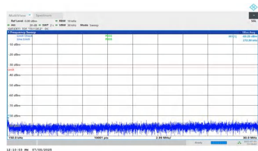
NTNV-DC_5A_n78A-PC2-30-5+20-M+M-QPSK-IDLE-DFT-BPSK-In ner_1RB_Left-0.15-30-PASS
