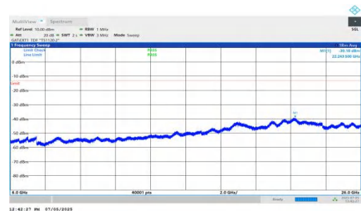
NTNV-DC_5A_n78A-PC2-30-5+25-M+M-QPSK-IDLE-DFT-BPSK-In ner_1RB_Left-6000-26000-PASS
