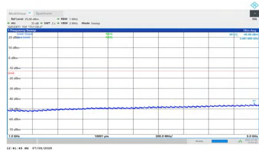
NTNV-DC_5A_n78A-PC2-30-5+25-M+M-QPSK-IDLE-DFT-BPSK-In ner_1RB_Left-1000-3000-PASS
