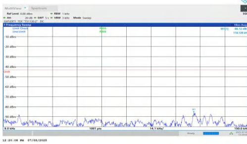
NTNV-DC_5A_n78A-PC2-30-5+20-M+H-QPSK-IDLE-DFT-BPSK-I nner_1RB_Left-0.009-0.15-PASS
