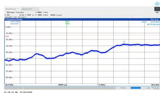
NTNV-DC_5A_n78A-PC2-30-5+30-M+L-QPSK-IDLE-DFT-BPSK-In ner_1RB_Right-26000-40000-PASS
