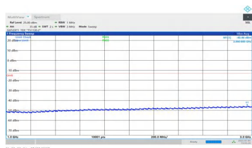
NTNV-DC_5A_n78A-PC2-30-5+40-M+L-QPSK-IDLE-DFT-BPSK-Inner_1RB_Left-1000-3000-PASS
