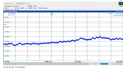
NTNV-DC_5A_n78A-PC2-30-5+25-M+L-QPSK-IDLE-DFT-BPSK-In ner_1RB_Left-6000-26000-PASS
