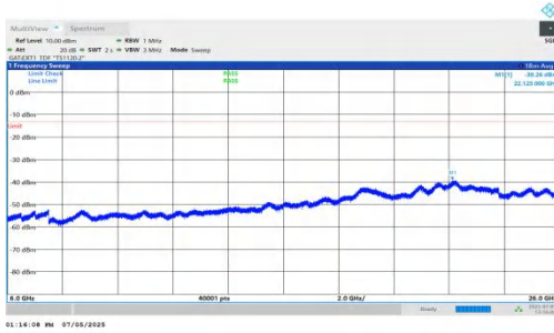
NTNV-DC_5A_n78A-PC2-30-5+30-M+M-QPSK-IDLE-DFT-BPSK-Inner_1RB_Right-6000-26000-PASS
