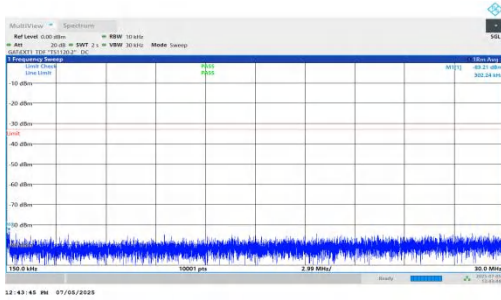
NTNV-DC_5A_n78A-PC2-30-5+25-M+M-QPSK-IDLE-DFT-BPSK-I nner_1RB_Right-0.15-30-PASS
