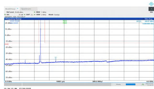
NTNV-DC_5A_n78A-PC2-30-5+25-M+L-QPSK-IDLE-DFT-BPSK-In ner_1RB_Right-3000-6000-PASS
