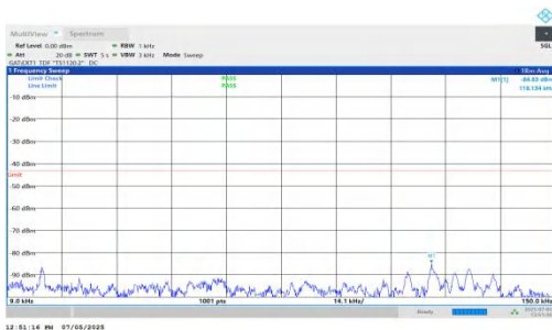
NTNV-DC_5A_n78A-PC2-30-5+25-M+H-QPSK-IDLE-DFT-BPSK-Inner_1RB_Left-0.009-0.15-PASS
