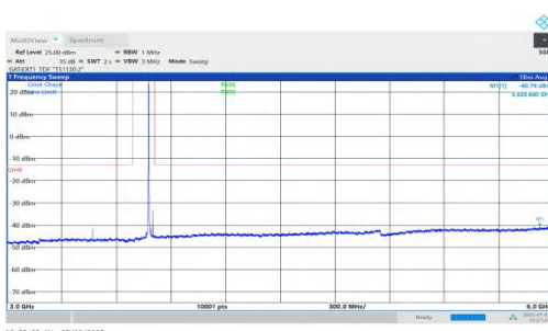
NTNV-DC_5A_n78A-PC2-30-5+25-M+H-QPSK-IDLE-DFT-QPSK-Inner_1RB_Left-3000-6000-PASS
