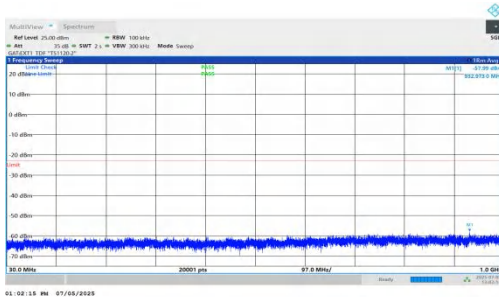
NTNV-DC_5A_n78A-PC2-30-5+30-M+L-QPSK-IDLE-DFT-BPSK-In ner_1RB_Left-30-1000-PASS
