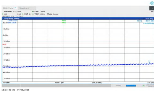
NTNV-DC_5A_n78A-PC2-30-5+20-M+H-QPSK-IDLE-DFT-BPSK-I nner_1RB_Right-1000-3000-PASS
