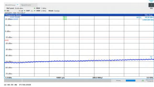
NTNV-DC_5A_n78A-PC2-30-5+25-M+M-QPSK-IDLE-DFT-QPSK-In ner_1RB_Left-1000-3000-PASS
