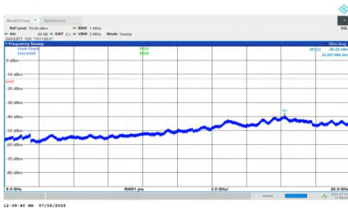
NTNV-DC_5A_n78A-PC2-30-5+20-M+L-QPSK-IDLE-DFT-QPSK-In ner_1RB_Right-6000-26000-PASS
