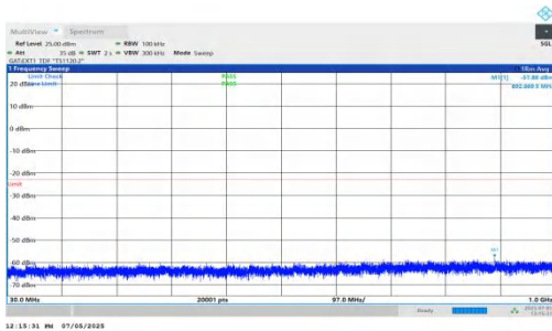
NTNV-DC_5A_n78A-PC2-30-5+20-M+M-QPSK-IDLE-DFT-QPSK-Inner_1RB_Left-30-1000-PASS
