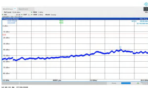
NTNV-DC_5A_n78A-PC2-30-5+25-M+M-QPSK-IDLE-DFT-BPSK-I nner_1RB_Right-6000-26000-PASS
