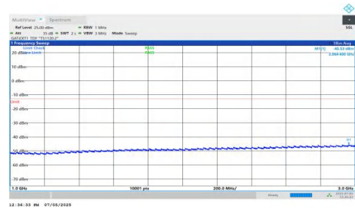
NTNV-DC_5A_n78A-PC2-30-5+25-M+L-QPSK-IDLE-DFT-QPSK-In ner_1RB_Left-1000-3000-PASS
