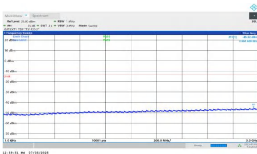
NTNV-DC_5A_n78A-PC2-30-5+25-M+H-QPSK-IDLE-DFT-QPSK-Inner_1RB_Right-1000-3000-PASS
