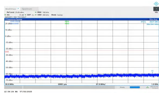
NTNV-DC_5A_n78A-PC2-30-5+25-M+H-QPSK-IDLE-DFT-BPSK-In ner_1RB_Right-30-1000-PASS
