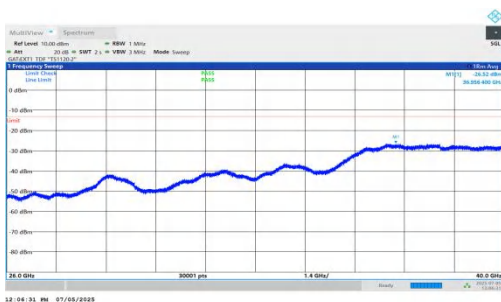
NTNV-DC_5A_n78A-PC2-30-5+20-M+L-QPSK-IDLE-DFT-QPSK-In ner_1RB_Left-26000-40000-PASS
