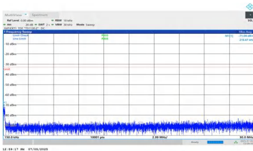
NTNV-DC_5A_n78A-PC2-30-5+25-M+H-QPSK-IDLE-DFT-QPSK-Inner_1RB_Right-0.15-30-PASS
