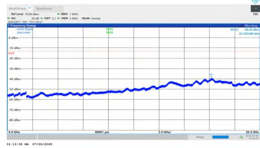
NTNV-DC_5A_n78A-PC2-30-5+30-M+M-QPSK-IDLE-DFT-BPSK-Inner_1RB_Left-6000-26000-PASS
