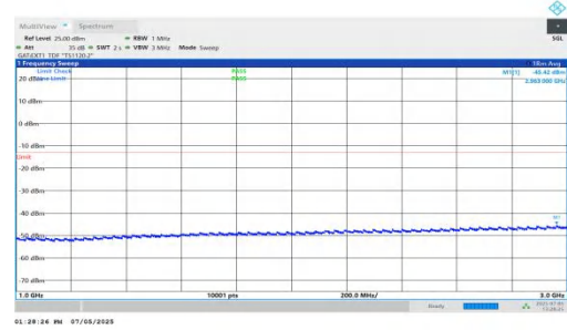
NTNV-DC_5A_n78A-PC2-30-5+30-M+H-QPSK-IDLE-DFT-QPSK-Inner_1RB_Left-1000-3000-PASS
