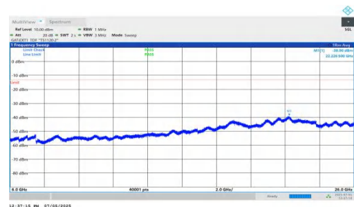
NTNV-DC_5A_n78A-PC2-30-5+25-M+L-QPSK-IDLE-DFT-QPSK-In ner_1RB_Left-6000-26000-PASS
