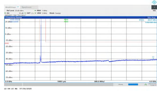
NTNV-DC_5A_n78A-PC2-30-5+20-M+L-QPSK-IDLE-DFT-QPSK-In ner_1RB_Right-3000-6000-PASS
