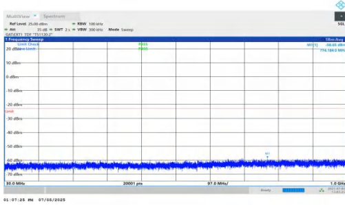
NTNV-DC_5A_n78A-PC2-30-5+30-M+L-QPSK-IDLE-DFT-QPSK-In ner_1RB_Left-30-1000-PASS
