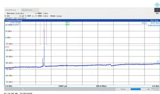
NTNV-DC_5A_n78A-PC2-30-5+30-M+M-QPSK-IDLE-DFT-BPSK-Inner_1RB_Right-3000-6000-PASS
