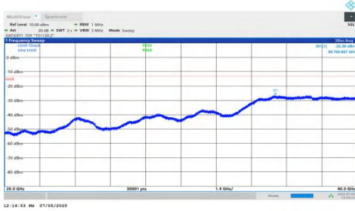
NTNV-DC_5A_n78A-PC2-30-5+20-M+M-QPSK-IDLE-DFT-QPSK-Inner_1RB_Left-26000-40000-PASS
