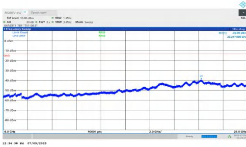
NTNV-DC_5A_n78A-PC2-30-5+25-M+L-QPSK-IDLE-DFT-BPSK-In ner_1RB_Right-6000-26000-PASS
