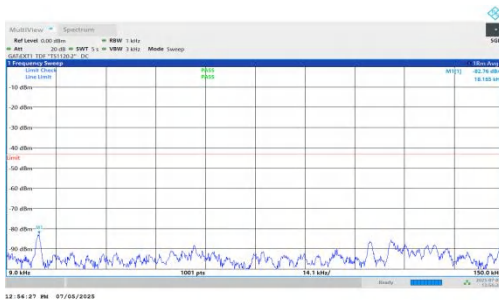
NTNV-DC_5A_n78A-PC2-30-5+25-M+H-QPSK-IDLE-DFT-QPSK-Inner_1RB_Left-0.009-0.15-PASS
