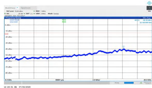
NTNV-DC_5A_n78A-PC2-30-5+20-M+H-QPSK-IDLE-DFT-QPSK-Inner_1RB_Left-6000-26000-PASS
