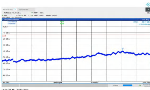
NTNV-DC_5A_n78A-PC2-30-5+25-M+L-QPSK-IDLE-DFT-QPSK-In ner_1RB_Right-6000-26000-PASS
