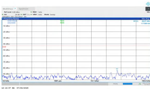
NTNV-DC_5A_n78A-PC2-30-5+20-M+M-QPSK-IDLE-DFT-QPSK-Inner_1RB_Left-0.009-0.15-PASS
