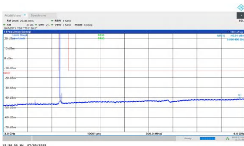
NTNV-DC_5A_n78A-PC2-30-5+25-M+L-QPSK-IDLE-DFT-QPSK-In ner_1RB_Left-3000-6000-PASS
