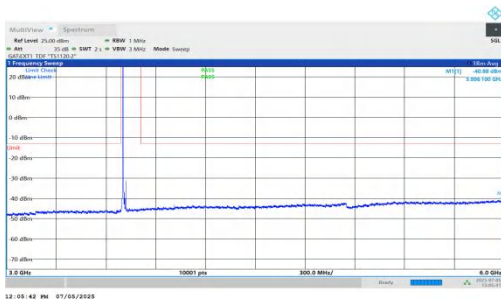
NTNV-DC_5A_n78A-PC2-30-5+20-M+L-QPSK-IDLE-DFT-QPSK-In ner_1RB_Left-3000-6000-PASS
