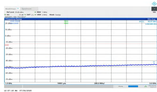
NTNV-DC_5A_n78A-PC2-30-5+25-M+H-QPSK-IDLE-DFT-QPSK-Inner_1RB_Left-1000-3000-PASS
