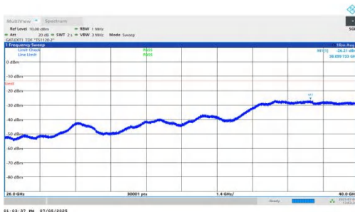
NTNV-DC_5A_n78A-PC2-30-5+30-M+L-QPSK-IDLE-DFT-BPSK-In ner_1RB_Left-26000-40000-PASS
