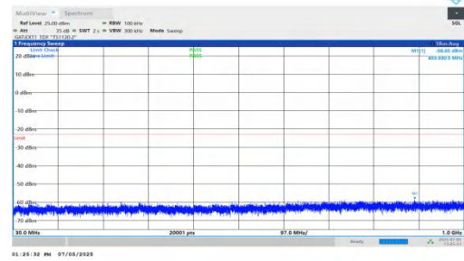
NTNV-DC_5A_n78A-PC2-30-5+30-M+H-QPSK-IDLE-DFT-BPSK-In ner_1RB_Right-30-1000-PASS
