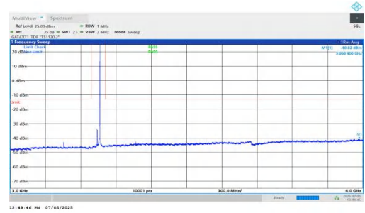
NTNV-DC_5A_n78A-PC2-30-5+25-M+M-QPSK-IDLE-DFT-QPSK-Inner_1RB_Right-3000-6000-PASS
