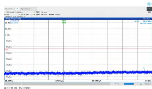
NTNV-DC_5A_n78A-PC2-30-5+25-M+H-QPSK-IDLE-DFT-QPSK-Inner_1RB_Right-30-1000-PASS
