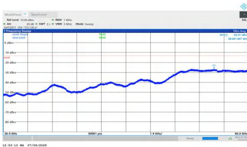
NTNV-DC_5A_n78A-PC2-30-5+25-M+H-QPSK-IDLE-DFT-BPSK-I nner_1RB_Left-26000-40000-PASS
