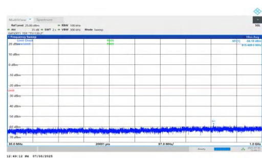
NTNV-DC_5A_n78A-PC2-30-5+25-M+M-QPSK-IDLE-DFT-QPSK-In ner_1RB_Right-30-1000-PASS
