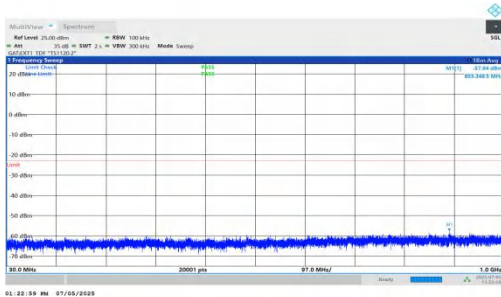
NTNV-DC_5A_n78A-PC2-30-5+30-M+H-QPSK-IDLE-DFT-BPSK-I nner_1RB_Left-30-1000-PASS
