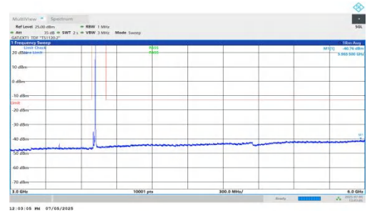
NTNV-DC_5A_n78A-PC2-30-5+20-M+L-QPSK-IDLE-DFT-BPSK-In ner_1RB_Right-3000-6000-PASS
