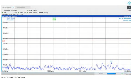
NTNV-DC_5A_n78A-PC2-30-5+10-M+L-QPSK-IDLE-DFT-BPSK-In ner_1RB_Left-0.009-0.15-PASS
