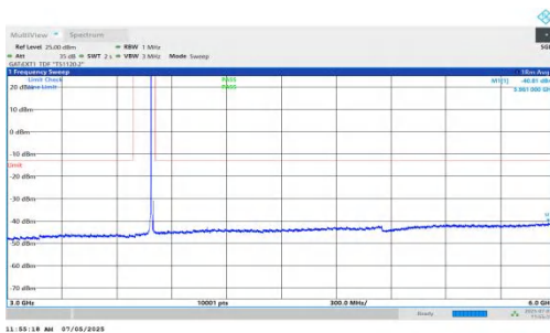
NTNV-DC_5A_n78A-PC2-30-5+15-M+H-QPSK-IDLE-DFT-QPSK-Inner_1RB_Left-3000-6000-PASS
