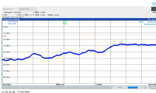
NTNV-DC_5A_n78A-PC2-30-5+10-M+L-QPSK-IDLE-DFT-BPSK-In ner_1RB_Left-26000-40000-PASS
