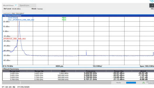
NTNV-DC_5A_n78A-PC2-30-5+90-M+L-QPSK-IDLE-DFT-QPSK-Edg e_1RB_Left-PASS
