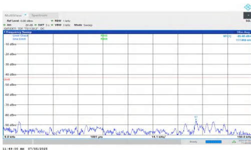
NTNV-DC_5A_n78A-PC2-30-5+15-M+H-QPSK-IDLE-DFT-BPSK-Inner_1RB_Left-0.009-0.15-PASS
