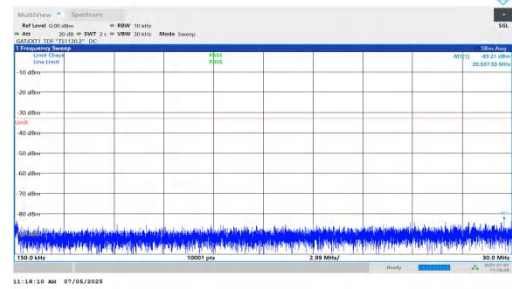
NTNV-DC_5A_n78A-PC2-30-5+10-M+H-QPSK-IDLE-DFT-BPSK-In ner_1RB_Left-0.15-30-PASS
