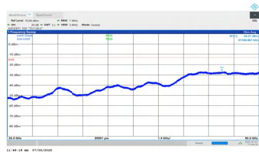
NTNV-DC_5A_n78A-PC2-30-5+15-M+M-QPSK-IDLE-DFT-QPSK-Inner_1RB_Right-26000-40000-PASS
