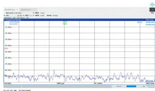
NTNV-DC_5A_n78A-PC2-30-5+20-M+L-QPSK-IDLE-DFT-BPSK-In ner_1RB_Right-0.009-0.15-PASS
