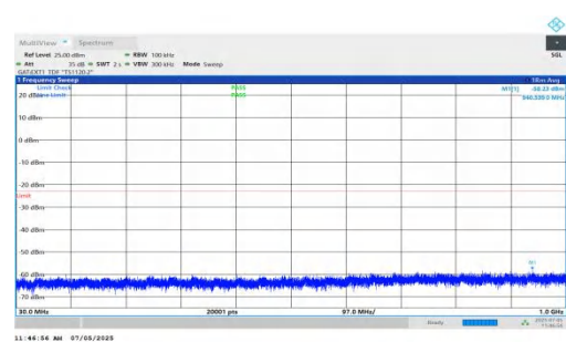
NTNV-DC_5A_n78A-PC2-30-5+15-M+M-QPSK-IDLE-DFT-QPSK-Inner_1RB_Right-30-1000-PASS
