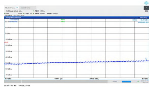
NTNV-DC_5A_n78A-PC2-30-5+10-M+L-QPSK-IDLE-DFT-BPSK-In ner_1RB_Left-1000-3000-PASS
