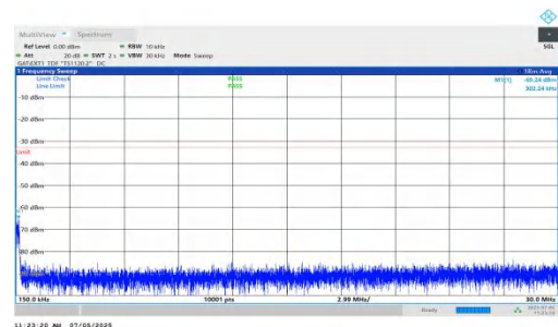
NTNV-DC_5A_n78A-PC2-30-5+10-M+H-QPSK-IDLE-DFT-QPSK-In ner_1RB_Left-0.15-30-PASS
