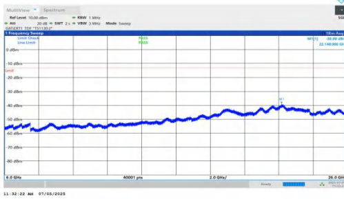
NTNV-DC_5A_n78A-PC2-30-5+15-M+L-QPSK-IDLE-DFT-BPSK-In ner_1RB_Right-6000-26000-PASS
