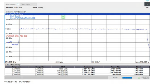
NTNV-DC_5A_n78A-PC2-30-5+100-M+L-QPSK-IDLE-DFT-BPS K-Outer_Full-PASS
