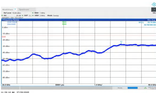
NTNV-DC_5A_n78A-PC2-30-5+10-M+L-QPSK-IDLE-DFT-QPSK-In ner_1RB_Left-26000-40000-PASS
