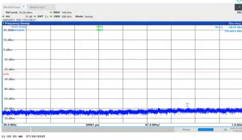
NTNV-DC_5A_n78A-PC2-30-5+10-M+L-QPSK-IDLE-DFT-QPSK-In ner_1RB_Left-30-1000-PASS
