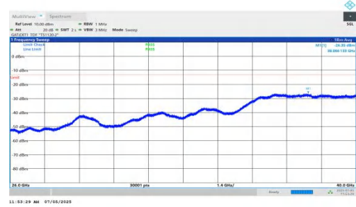
NTNV-DC_5A_n78A-PC2-30-5+15-M+H-QPSK-IDLE-DFT-BPSK-Inner_1RB_Right-26000-40000-PASS
