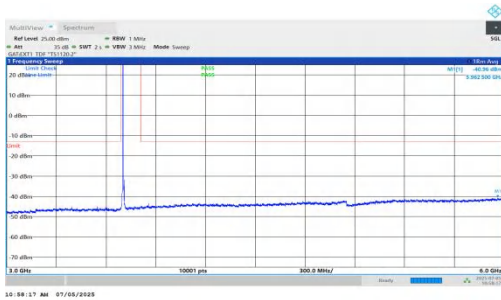
NTNV-DC_5A_n78A-PC2-30-5+10-M+L-QPSK-IDLE-DFT-BPSK-In ner_1RB_Left-3000-6000-PASS
