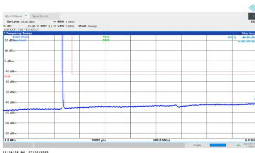
NTNV-DC_5A_n78A-PC2-30-5+15-M+L-QPSK-IDLE-DFT-QPSK-In ner_1RB_Left-3000-6000-PASS
