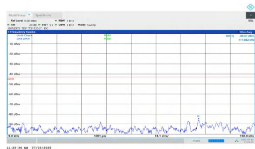
NTNV-DC_5A_n78A-PC2-30-5+10-M+H-QPSK-IDLE-DFT-QPSK-Inner_1RB_Right-0.009-0.15-PASS
