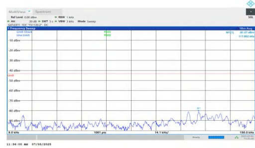
NTNV-DC_5A_n78A-PC2-30-5+15-M+L-QPSK-IDLE-DFT-QPSK-In ner_1RB_Right-0.009-0.15-PASS
