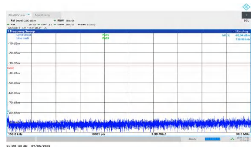
NTNV-DC_5A_n78A-PC2-30-5+15-M+L-QPSK-IDLE-DFT-BPSK-Inner_1RB_Left-0.15-30-PASS
