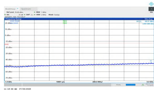
NTNV-DC_5A_n78A-PC2-30-5+10-M+H-QPSK-IDLE-DFT-BPSK-In ner_1RB_Left-1000-3000-PASS
