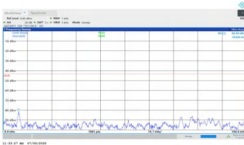
NTNV-DC_5A_n78A-PC2-30-5+15-M+L-QPSK-IDLE-DFT-QPSK-In ner_1RB_Left-0.009-0.15-PASS
