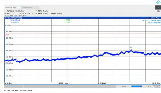
NTNV-DC_5A_n78A-PC2-30-5+15-M+L-QPSK-IDLE-DFT-BPSK-In ner_1RB_Left-6000-26000-PASS
