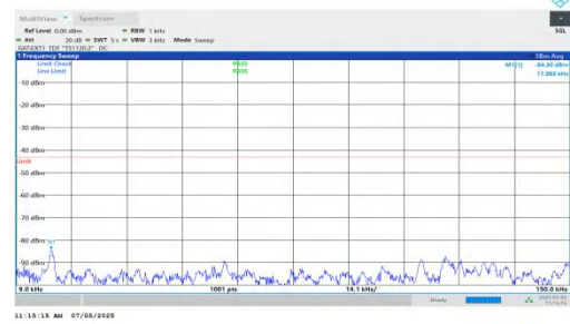
NTNV-DC_5A_n78A-PC2-30-5+10-M+M-QPSK-IDLE-DFT-QPSK-Inner_1RB_Right-0.009-0.15-PASS
