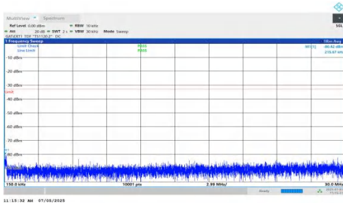
NTNV-DC_5A_n78A-PC2-30-5+10-M+M-QPSK-IDLE-DFT-QPSK-Inner_1RB_Right-0.15-30-PASS
