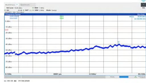
NTNV-DC_5A_n78A-PC2-30-5+10-M+M-QPSK-IDLE-DFT-BPSK-Inner_1RB_Left-6000-26000-PASS
