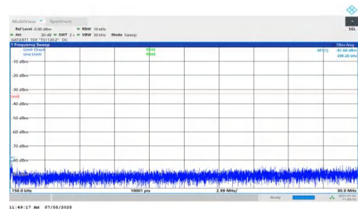
NTNV-DC_5A_n78A-PC2-30-5+15-M+H-QPSK-IDLE-DFT-BPSK-Inner_1RB_Left-0.15-30-PASS
