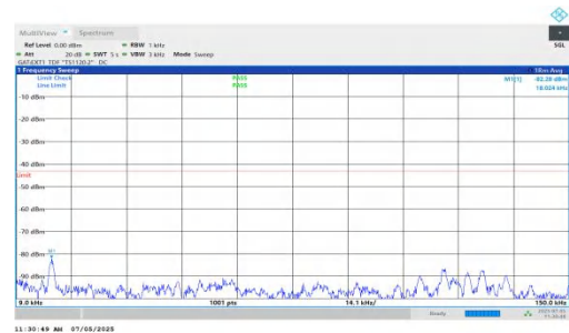
NTNV-DC_5A_n78A-PC2-30-5+15-M+L-QPSK-IDLE-DFT-BPSK-In ner_1RB_Right-0.009-0.15-PASS
