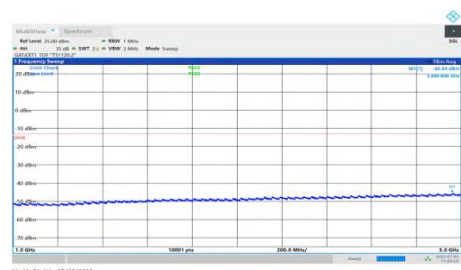
NTNV-DC_5A_n78A-PC2-30-5+15-M+H-QPSK-IDLE-DFT-BPSK-Inner_1RB_Left-1000-3000-PASS
