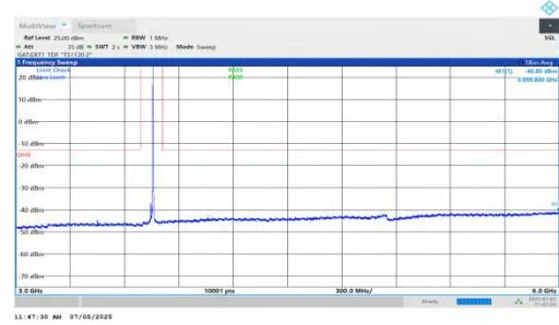
NTNV-DC_5A_n78A-PC2-30-5+15-M+M-QPSK-IDLE-DFT-QPSK-Inner_1RB_Right-3000-6000-PASS
