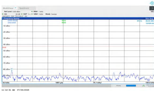
NTNV-DC_5A_n78A-PC2-30-5+10-M+M-QPSK-IDLE-DFT-QPSK-Inner_1RB_Left-0.009-0.15-PASS
