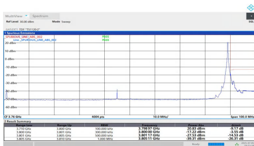
NTNV-DC_5A_n78A-PC2-30-5+90-M+H-QPSK-IDLE-DFT-QPSK-Edg e_1RB_Right-PASS
