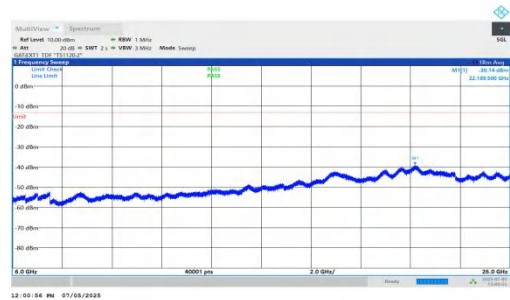
NTNV-DC_5A_n78A-PC2-30-5+20-M+L-QPSK-IDLE-DFT-BPSK-In ner_1RB_Left-6000-26000-PASS
