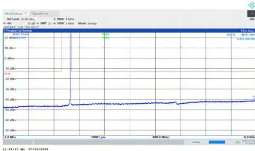
NTNV-DC_5A_n78A-PC2-30-5+10-M+H-QPSK-IDLE-DFT-QPSK-Inner_1RB_Left-3000-6000-PASS
