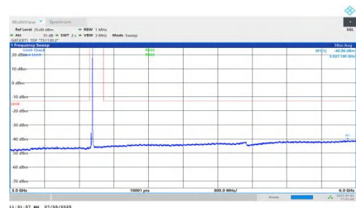
NTNV-DC_5A_n78A-PC2-30-5+15-M+L-QPSK-IDLE-DFT-BPSK-In ner_1RB_Right-3000-6000-PASS
