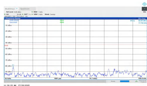
NTNV-DC_5A_n78A-PC2-30-5+10-M+L-QPSK-IDLE-DFT-QPSK-In ner_1RB_Right-0.009-0.15-PASS
