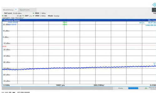
NTNV-DC_5A_n78A-PC2-30-5+10-M+M-QPSK-IDLE-DFT-BPSK-Inner_1RB_Right-1000-3000-PASS
