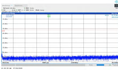
NTNV-DC_5A_n78A-PC2-30-5+10-M+L-QPSK-IDLE-DFT-BPSK-In ner_1RB_Right-0.15-30-PASS
