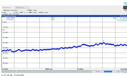
NTNV-DC_5A_n78A-PC2-30-5+15-M+M-QPSK-IDLE-DFT-QPSK-Inner_1RB_Right-6000-26000-PASS
