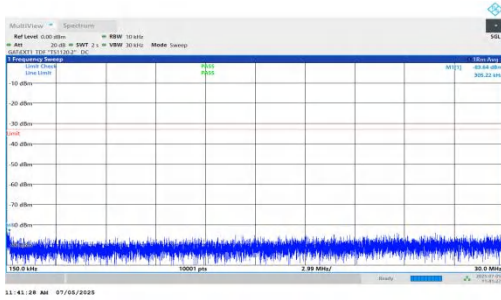
NTNV-DC_5A_n78A-PC2-30-5+15-M+M-QPSK-IDLE-DFT-BPSK-I nner_1RB_Right-0.15-30-PASS
