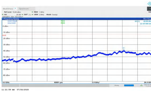
NTNV-DC_5A_n78A-PC2-30-5+10-M+H-QPSK-IDLE-DFT-BPSK-I nner_1RB_Right-6000-26000-PASS
