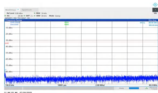
NTNV-DC_5A_n78A-PC2-30-5+15-M+M-QPSK-IDLE-DFT-QPSK-In ner_1RB_Left-0.15-30-PASS
