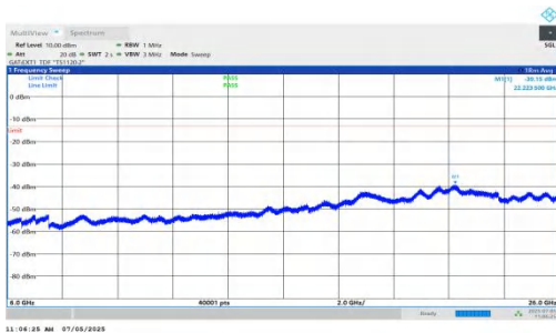
NTNV-DC_5A_n78A-PC2-30-5+10-M+L-QPSK-IDLE-DFT-QPSK-In ner_1RB_Right-6000-26000-PASS
