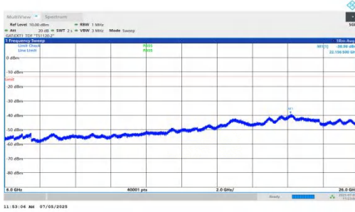
NTNV-DC_5A_n78A-PC2-30-5+15-M+H-QPSK-IDLE-DFT-BPSK-Inner_1RB_Right-6000-26000-PASS
