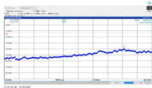
NTNV-DC_5A_n78A-PC2-30-5+10-M+L-QPSK-IDLE-DFT-QPSK-In ner_1RB_Left-6000-26000-PASS
