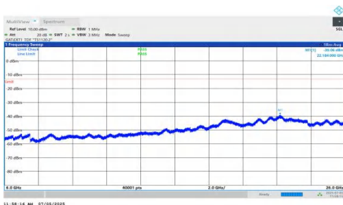
NTNV-DC_5A_n78A-PC2-30-5+15-M+H-QPSK-IDLE-DFT-QPSK-Inner_1RB_Right-6000-26000-PASS
