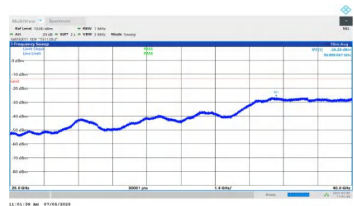
NTNV-DC_5A_n78A-PC2-30-5+10-M+L-QPSK-IDLE-DFT-BPSK-In ner_1RB_Right-26000-40000-PASS
