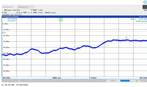
NTNV-DC_5A_n78A-PC2-30-5+15-M+L-QPSK-IDLE-DFT-QPSK-In ner_1RB_Left-26000-40000-PASS
