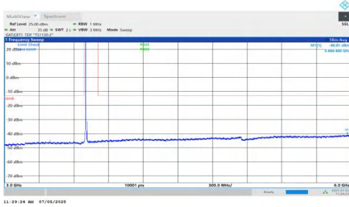
NTNV-DC_5A_n78A-PC2-30-5+15-M+L-QPSK-IDLE-DFT-BPSK-In ner_1RB_Left-3000-6000-PASS
