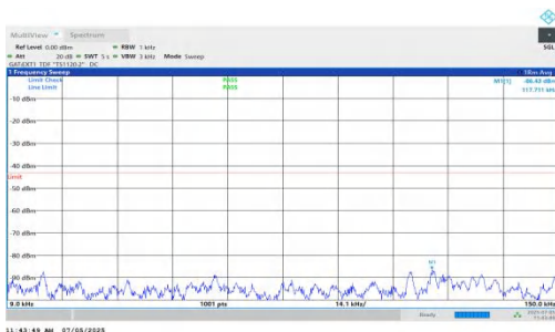
NTNV-DC_5A_n78A-PC2-30-5+15-M+M-QPSK-IDLE-DFT-QPSK-I nner_1RB_Left-0.009-0.15-PASS
