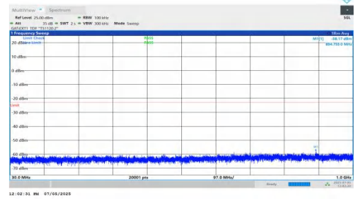
NTNV-DC_5A_n78A-PC2-30-5+20-M+L-QPSK-IDLE-DFT-BPSK-In ner_1RB_Right-30-1000-PASS
