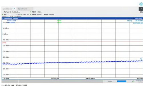
NTNV-DC_5A_n78A-PC2-30-5+15-M+H-QPSK-IDLE-DFT-QPSK-Inner_1RB_Right-1000-3000-PASS
