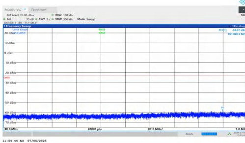
NTNV-DC_5A_n78A-PC2-30-5+15-M+H-QPSK-IDLE-DFT-QPSK-Inner_1RB_Left-30-1000-PASS
