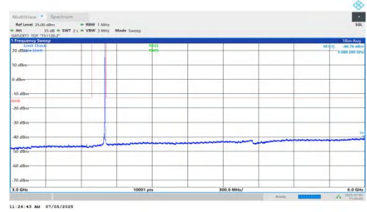
NTNV-DC_5A_n78A-PC2-30-5+10-M+H-QPSK-IDLE-DFT-QPSK-Inner_1RB_Right-3000-6000-PASS
