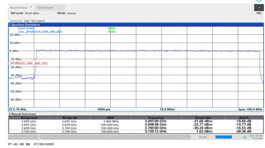
NTNV-DC_5A_n78A-PC2-30-5+90-M+L-QPSK-IDLE-DFT-BPSK-Outer_Full-PASS
