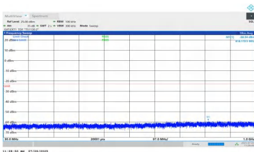
NTNV-DC_5A_n78A-PC2-30-5+15-M+L-QPSK-IDLE-DFT-BPSK-Inner_1RB_Left-30-1000-PASS
