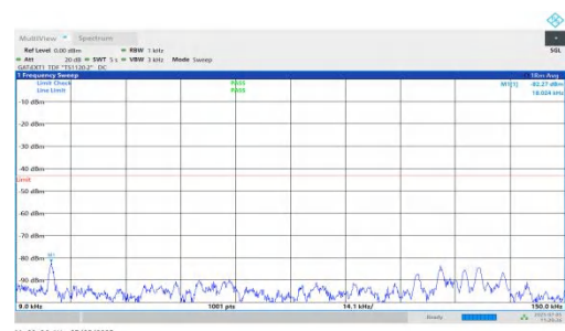
NTNV-DC_5A_n78A-PC2-30-5+10-M+H-QPSK-IDLE-DFT-BPSK-In ner_1RB_Right-0.009-0.15-PASS
