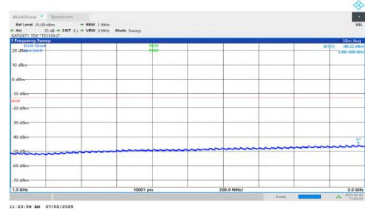
NTNV-DC_5A_n78A-PC2-30-5+10-M+H-QPSK-IDLE-DFT-QPSK-Inner_1RB_Left-1000-3000-PASS
