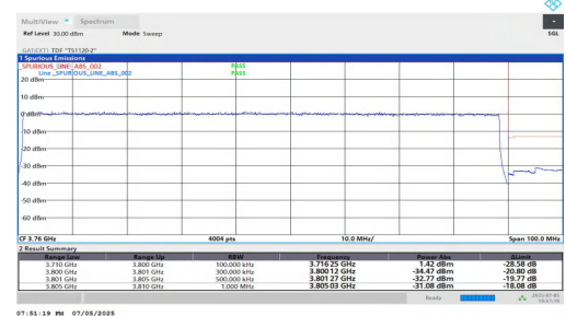
NTNV-DC_5A_n78A-PC2-30-5+90-M+H-QPSK-IDLE-DFT-BPSK-Outer_Full-PASS
