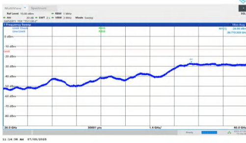
NTNV-DC_5A_n78A-PC2-30-5+10-M+M-QPSK-IDLE-DFT-QPSK-Inner_1RB_Left-26000-40000-PASS
