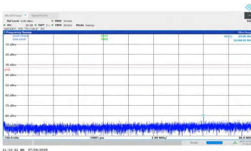
NTNV-DC_5A_n78A-PC2-30-5+10-M+M-QPSK-IDLE-DFT-BPSK-Inner_1RB_Right-0.15-30-PASS
