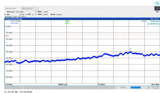
NTNV-DC_5A_n78A-PC2-30-5+10-M+H-QPSK-IDLE-DFT-QPSK-Inner_1RB_Left-6000-26000-PASS
