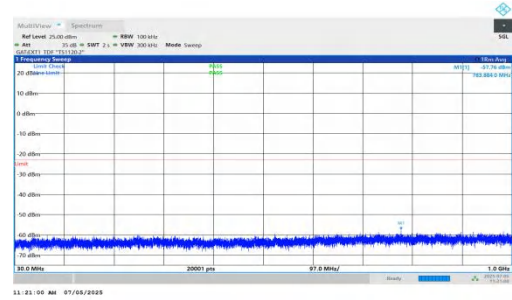
NTNV-DC_5A_n78A-PC2-30-5+10-M+H-QPSK-IDLE-DFT-BPSK-In ner_1RB_Right-30-1000-PASS
