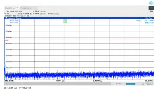
NTNV-DC_5A_n78A-PC2-30-5+10-M+M-QPSK-IDLE-DFT-QPSK-Inner_1RB_Left-0.15-30-PASS
