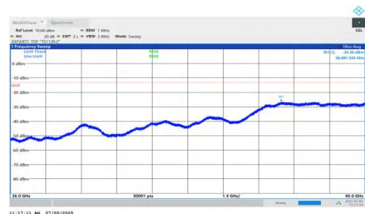
NTNV-DC_5A_n78A-PC2-30-5+10-M+M-QPSK-IDLE-DFT-QPSK-Inner_1RB_Right-26000-40000-PASS
