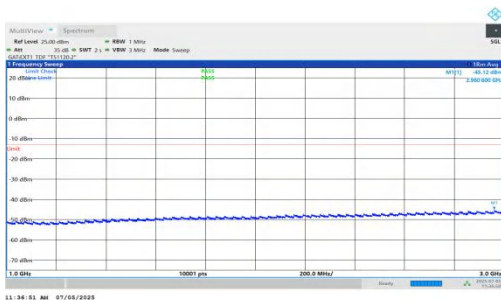
NTNV-DC_5A_n78A-PC2-30-5+15-M+L-QPSK-IDLE-DFT-QPSK-In ner_1RB_Right-1000-3000-PASS
