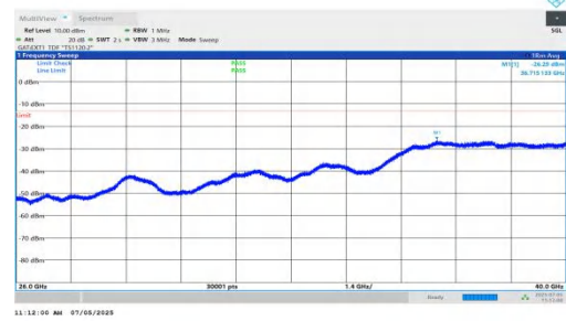
NTNV-DC_5A_n78A-PC2-30-5+10-M+M-QPSK-IDLE-DFT-BPSK-Inner_1RB_Right-26000-40000-PASS
