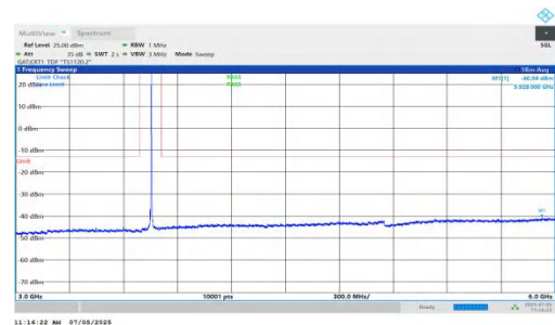
NTNV-DC_5A_n78A-PC2-30-5+10-M+M-QPSK-IDLE-DFT-QPSK-Inner_1RB_Right-3000-6000-PASS
