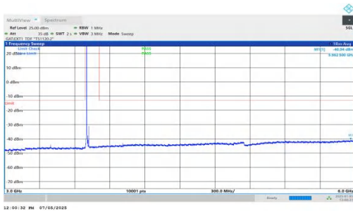
NTNV-DC_5A_n78A-PC2-30-5+20-M+L-QPSK-IDLE-DFT-BPSK-In ner_1RB_Left-3000-6000-PASS
