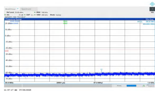
NTNV-DC_5A_n78A-PC2-30-5+15-M+H-QPSK-IDLE-DFT-QPSK-Inner_1RB_Right-30-1000-PASS
