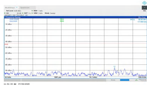
NTNV-DC_5A_n78A-PC2-30-5+15-M+H-QPSK-IDLE-DFT-BPSK-In ner_1RB_Right-0.009-0.15-PASS
