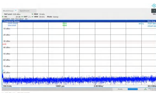
NTNV-DC_5A_n78A-PC2-30-5+10-M+H-QPSK-IDLE-DFT-QPSK-Inner_1RB_Right-0.15-30-PASS
