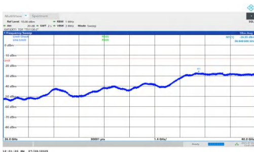
NTNV-DC_5A_n78A-PC2-30-5+20-M+L-QPSK-IDLE-DFT-BPSK-In ner_1RB_Left-26000-40000-PASS
