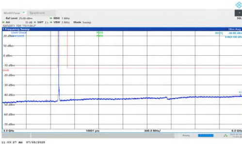
NTNV-DC_5A_n78A-PC2-30-5+10-M+L-QPSK-IDLE-DFT-QPSK-In ner_1RB_Left-3000-6000-PASS
