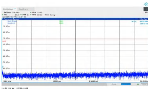
NTNV-DC_5A_n78A-PC2-30-5+15-M+H-QPSK-IDLE-DFT-BPSK-I nner_1RB_Right-0.15-30-PASS
