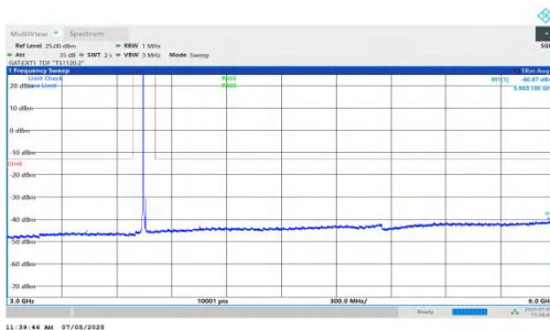
NTNV-DC_5A_n78A-PC2-30-5+15-M+M-QPSK-IDLE-DFT-BPSK-I nner_1RB_Left-3000-6000-PASS
