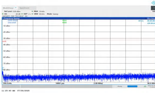
NTNV-DC_5A_n78A-PC2-30-5+10-M+H-QPSK-IDLE-DFT-BPSK-I nner_1RB_Right-0.15-30-PASS
