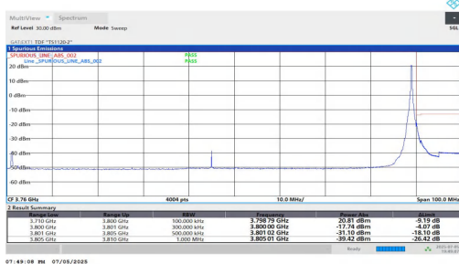
NTNV-DC_5A_n78A-PC2-30-5+90-M+H-QPSK-IDLE-DFT-BPSK-Edg e_1RB_Right-PASS
