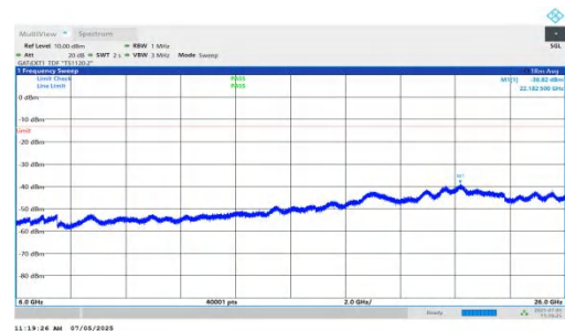
NTNV-DC_5A_n78A-PC2-30-5+10-M+H-QPSK-IDLE-DFT-BPSK-In ner_1RB_Left-6000-26000-PASS
