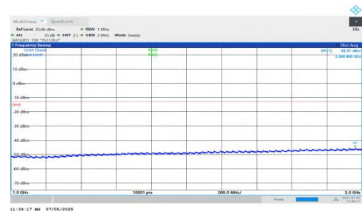
NTNV-DC_5A_n78A-PC2-30-5+15-M+L-QPSK-IDLE-DFT-QPSK-In ner_1RB_Left-1000-3000-PASS
