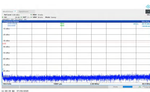
NTNV-DC_5A_n78A-PC2-30-5+15-M+M-QPSK-IDLE-DFT-QPSK-Inner_1RB_Right-0.15-30-PASS
