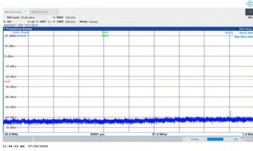
NTNV-DC_5A_n78A-PC2-30-5+15-M+M-QPSK-IDLE-DFT-QPSK-Inner_1RB_Left-30-1000-PASS
