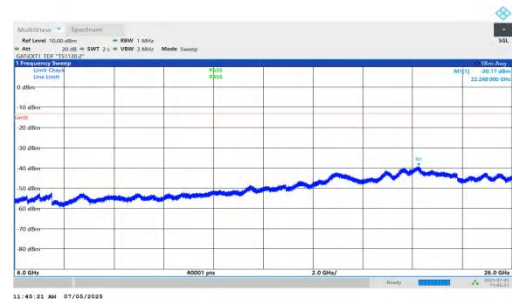
NTNV-DC_5A_n78A-PC2-30-5+15-M+M-QPSK-IDLE-DFT-QPSK-Inner_1RB_Left-6000-26000-PASS
