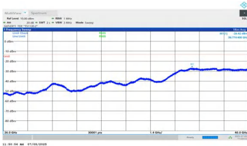
NTNV-DC_5A_n78A-PC2-30-5+15-M+H-QPSK-IDLE-DFT-BPSK-I nner_1RB_Left-26000-40000-PASS
