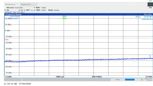
NTNV-DC_5A_n78A-PC2-30-5+10-M+L-QPSK-IDLE-DFT-QPSK-In ner_1RB_Left-1000-3000-PASS
