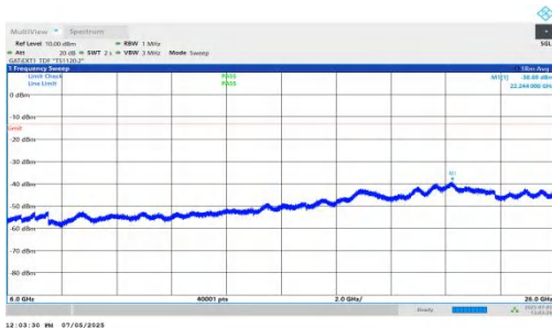
NTNV-DC_5A_n78A-PC2-30-5+20-M+L-QPSK-IDLE-DFT-BPSK-In ner_1RB_Right-6000-26000-PASS
