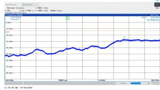
NTNV-DC_5A_n78A-PC2-30-5+15-M+L-QPSK-IDLE-DFT-BPSK-In ner_1RB_Right-26000-40000-PASS
