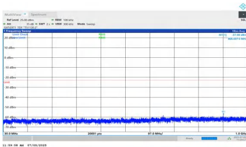
NTNV-DC_5A_n78A-PC2-30-5+20-M+L-QPSK-IDLE-DFT-BPSK-In ner_1RB_Left-30-1000-PASS
