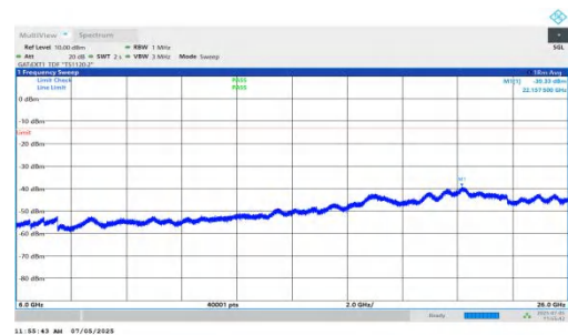
NTNV-DC_5A_n78A-PC2-30-5+15-M+H-QPSK-IDLE-DFT-QPSK-Inner_1RB_Left-6000-26000-PASS
