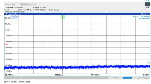
NTNV-DC_5A_n78A-PC2-30-5+10-M+L-QPSK-IDLE-DFT-BPSK-In ner_1RB_Right-30-1000-PASS
