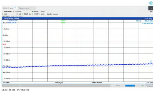
NTNV-DC_5A_n78A-PC2-30-5+20-M+L-QPSK-IDLE-DFT-BPSK-In ner_1RB_Right-1000-3000-PASS
