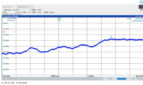
NTNV-DC_5A_n78A-PC2-30-5+15-M+H-QPSK-IDLE-DFT-QPSK-Inner_1RB_Left-26000-40000-PASS
