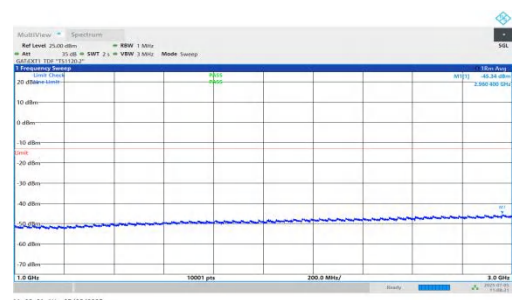
NTNV-DC_5A_n78A-PC2-30-5+10-M+M-QPSK-IDLE-DFT-BPSK-In ner_1RB_Left-1000-3000-PASS
