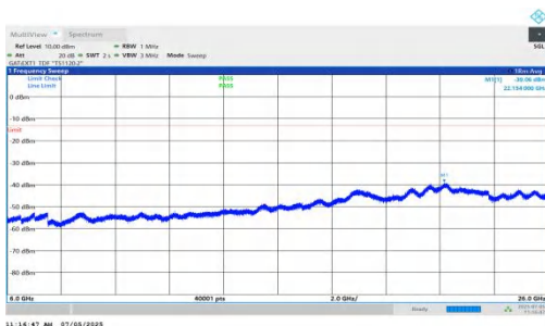
NTNV-DC_5A_n78A-PC2-30-5+10-M+M-QPSK-IDLE-DFT-QPSK-Inner_1RB_Right-6000-26000-PASS
