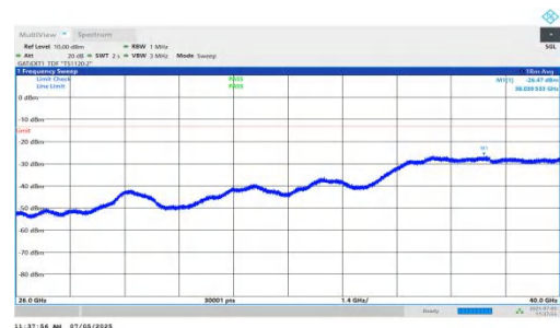
NTNV-DC_5A_n78A-PC2-30-5+15-M+L-QPSK-IDLE-DFT-QPSK-In ner_1RB_Right-26000-40000-PASS
