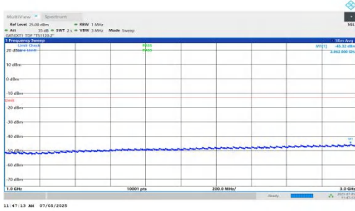
NTNV-DC_5A_n78A-PC2-30-5+15-M+M-QPSK-IDLE-DFT-QPSK-Inner_1RB_Right-1000-3000-PASS
