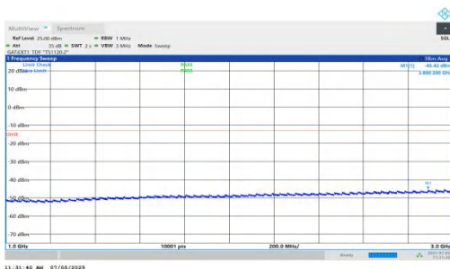
NTNV-DC_5A_n78A-PC2-30-5+15-M+L-QPSK-IDLE-DFT-BPSK-In ner_1RB_Right-1000-3000-PASS
