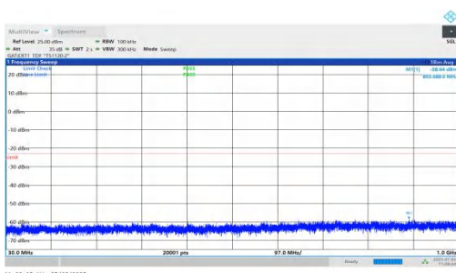
NTNV-DC_5A_n78A-PC2-30-5+10-M+M-QPSK-IDLE-DFT-BPSK-I nner_1RB_Left-30-1000-PASS
