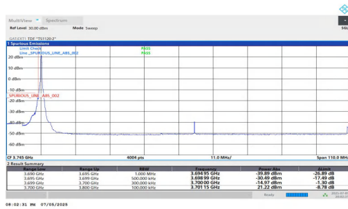
NTNV-DC_5A_n78A-PC2-30-5+100-M+L-QPSK-IDLE-DFT-QPSK-Ed ge_1RB_Left-PASS
