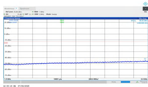
NTNV-DC_5A_n78A-PC2-30-5+20-M+L-QPSK-IDLE-DFT-BPSK-In ner_1RB_Left-1000-3000-PASS
