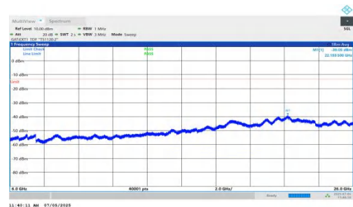
NTNV-DC_5A_n78A-PC2-30-5+15-M+M-QPSK-IDLE-DFT-BPSK-In ner_1RB_Left-6000-26000-PASS
