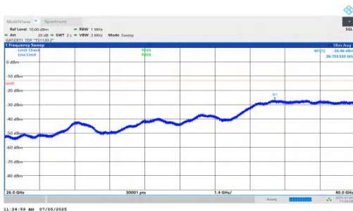
NTNV-DC_5A_n78A-PC2-30-5+10-M+H-QPSK-IDLE-DFT-QPSK-Inner_1RB_Left-26000-40000-PASS
