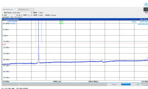
NTNV-DC_5A_n78A-PC2-30-5+10-M+M-QPSK-IDLE-DFT-QPSK-Inner_1RB_Left-3000-6000-PASS
