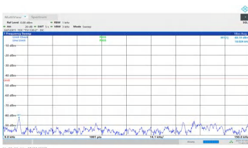
NTNV-DC_5A_n78A-PC2-30-5+10-M+L-QPSK-IDLE-DFT-QPSK-In ner_1RB_Left-0.009-0.15-PASS
