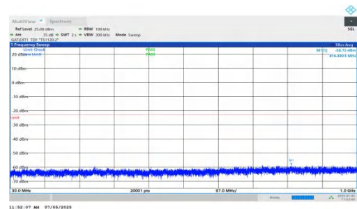
NTNV-DC_5A_n78A-PC2-30-5+15-M+H-QPSK-IDLE-DFT-BPSK-In ner_1RB_Right-30-1000-PASS
