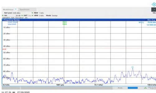
NTNV-DC_5A_n78A-PC2-30-5+10-M+M-QPSK-IDLE-DFT-BPSK-I nner_1RB_Left-0.009-0.15-PASS
