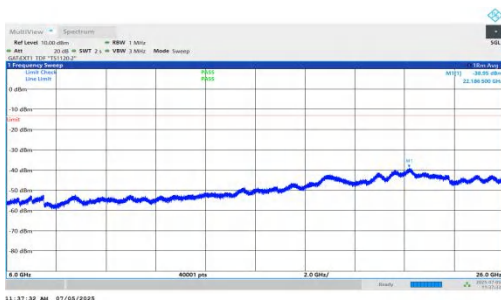
NTNV-DC_5A_n78A-PC2-30-5+15-M+L-QPSK-IDLE-DFT-QPSK-In ner_1RB_Right-6000-26000-PASS
