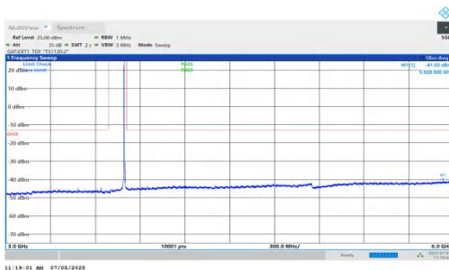
NTNV-DC_5A_n78A-PC2-30-5+10-M+H-QPSK-IDLE-DFT-BPSK-I nner_1RB_Left-3000-6000-PASS
