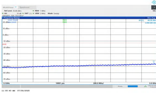
NTNV-DC_5A_n78A-PC2-30-5+10-M+L-QPSK-IDLE-DFT-QPSK-In ner_1RB_Right-1000-3000-PASS
