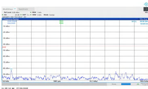
NTNV-DC_5A_n78A-PC2-30-5+15-M+L-QPSK-IDLE-DFT-BPSK-Inner_1RB_Left-0.009-0.15-PASS
