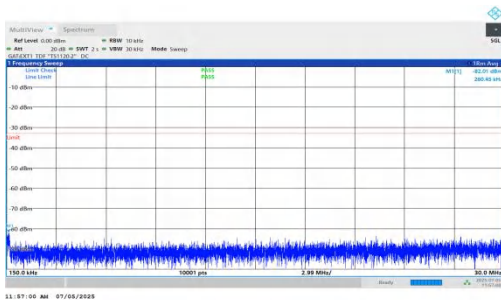
NTNV-DC_5A_n78A-PC2-30-5+15-M+H-QPSK-IDLE-DFT-QPSK-Inner_1RB_Right-0.15-30-PASS
