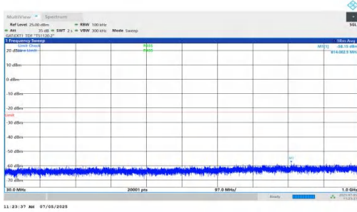
NTNV-DC_5A_n78A-PC2-30-5+10-M+H-QPSK-IDLE-DFT-QPSK-Inner_1RB_Left-30-1000-PASS
