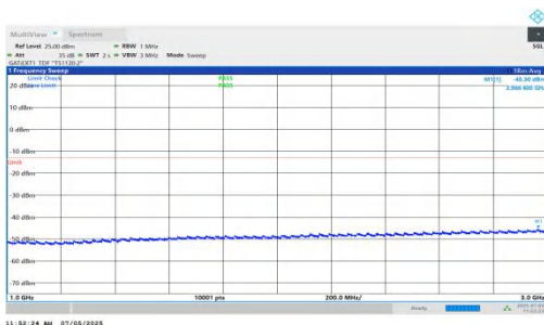
NTNV-DC_5A_n78A-PC2-30-5+15-M+H-QPSK-IDLE-DFT-BPSK-I nner_1RB_Right-1000-3000-PASS
