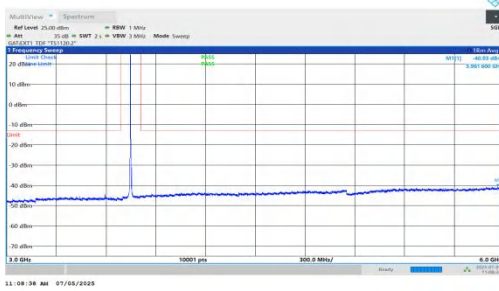
NTNV-DC_5A_n78A-PC2-30-5+10-M+M-QPSK-IDLE-DFT-BPSK-Inner_1RB_Left-3000-6000-PASS
