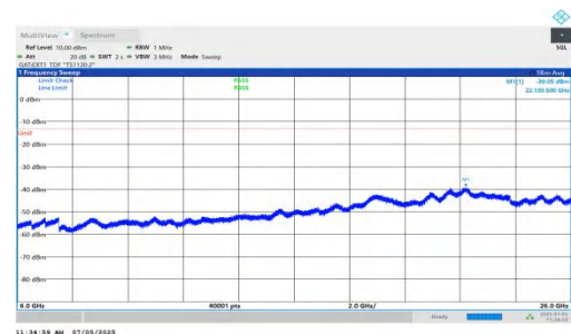
NTNV-DC_5A_n78A-PC2-30-5+15-M+L-QPSK-IDLE-DFT-QPSK-In ner_1RB_Left-6000-26000-PASS
