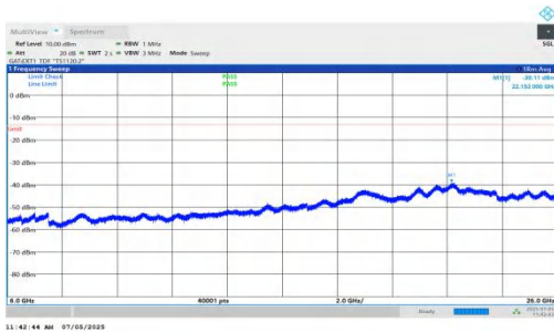
NTNV-DC_5A_n78A-PC2-30-5+15-M+M-QPSK-IDLE-DFT-BPSK-I nner_1RB_Right-6000-26000-PASS
