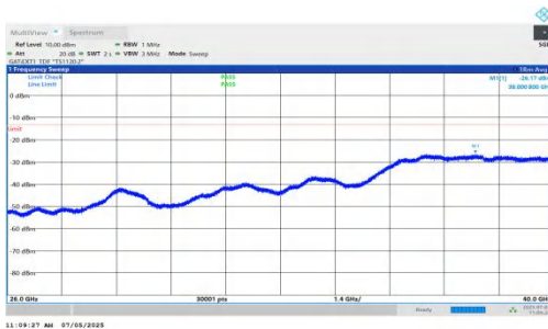
NTNV-DC_5A_n78A-PC2-30-5+10-M+M-QPSK-IDLE-DFT-BPSK-Inner_1RB_Left-26000-40000-PASS
