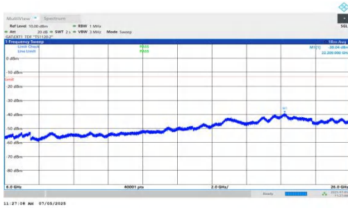
NTNV-DC_5A_n78A-PC2-30-5+10-M+H-QPSK-IDLE-DFT-QPSK-Inner_1RB_Right-6000-26000-PASS
