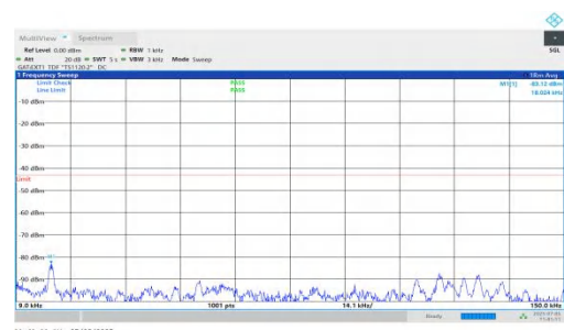
NTNV-DC_5A_n78A-PC2-30-5+15-M+M-QPSK-IDLE-DFT-BPSK-In ner_1RB_Right-0.009-0.15-PASS
