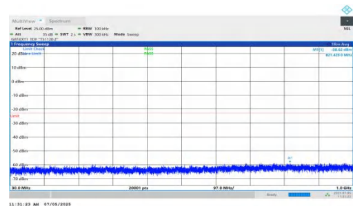
NTNV-DC_5A_n78A-PC2-30-5+15-M+L-QPSK-IDLE-DFT-BPSK-In ner_1RB_Right-30-1000-PASS
