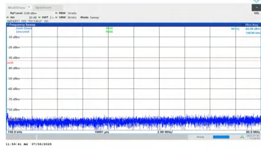
NTNV-DC_5A_n78A-PC2-30-5+20-M+L-QPSK-IDLE-DFT-BPSK-In ner_1RB_Left-0.15-30-PASS
