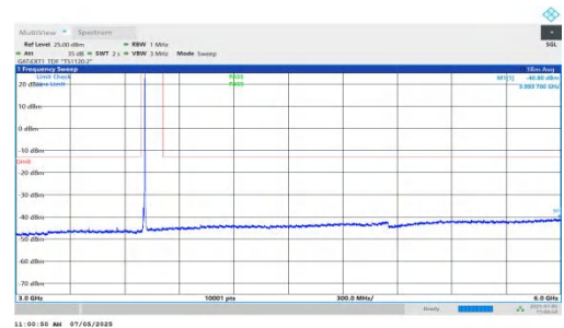
NTNV-DC_5A_n78A-PC2-30-5+10-M+L-QPSK-IDLE-DFT-BPSK-In ner_1RB_Right-3000-6000-PASS
