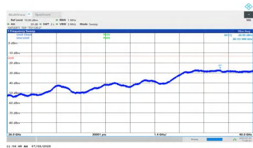
NTNV-DC_5A_n78A-PC2-30-5+10-M+L-QPSK-IDLE-DFT-QPSK-In ner_1RB_Right-26000-40000-PASS
