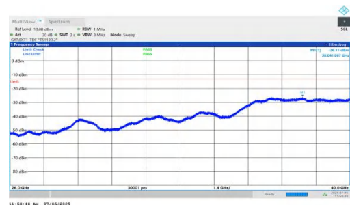
NTNV-DC_5A_n78A-PC2-30-5+15-M+H-QPSK-IDLE-DFT-QPSK-Inner_1RB_Right-26000-40000-PASS
