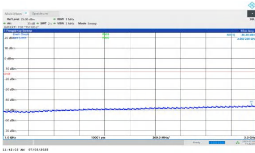
NTNV-DC_5A_n78A-PC2-30-5+15-M+M-QPSK-IDLE-DFT-BPSK-I nner_1RB_Right-1000-3000-PASS
