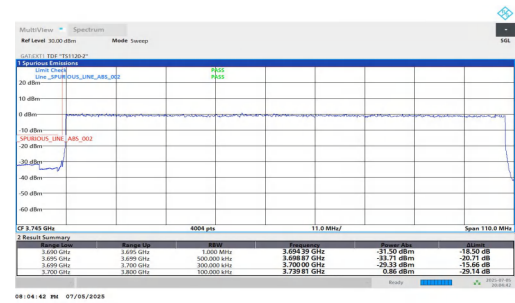
NTNV-DC_5A_n78A-PC2-30-5+100-M+L-QPSK-IDLE-DFT-QPS K-Outer_Full-PASS
