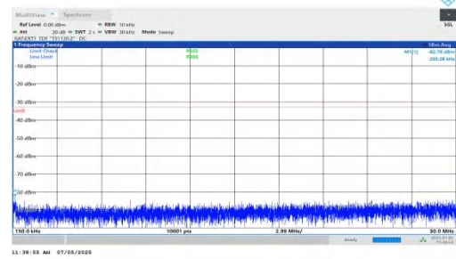
NTNV-DC_5A_n78A-PC2-30-5+15-M+M-QPSK-IDLE-DFT-BPSK-In ner_1RB_Left-0.15-30-PASS
