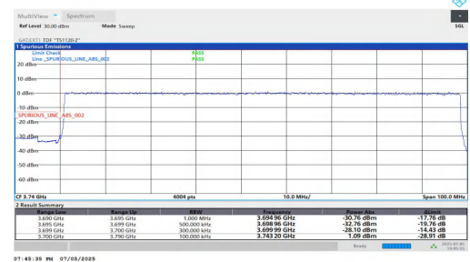
NTNV-DC_5A_n78A-PC2-30-5+90-M+L-QPSK-IDLE-DFT-QPSK-Outer_Full-PASS
