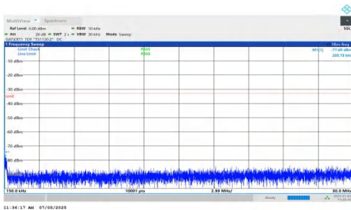
NTNV-DC_5A_n78A-PC2-30-5+15-M+L-QPSK-IDLE-DFT-QPSK-In ner_1RB_Right-0.15-30-PASS
