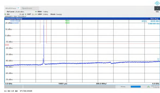
NTNV-DC_5A_n78A-PC2-30-5+15-M+M-QPSK-IDLE-DFT-BPSK-In ner_1RB_Right-3000-6000-PASS
