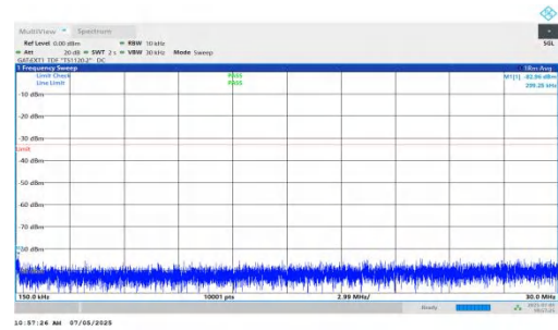
NTNV-DC_5A_n78A-PC2-30-5+10-M+L-QPSK-IDLE-DFT-BPSK-In ner_1RB_Left-0.15-30-PASS
