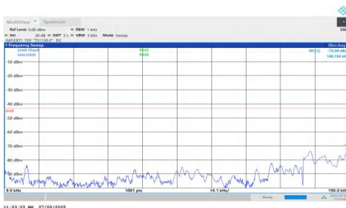
NTNV-DC_5A_n78A-PC2-30-5+10-M+H-QPSK-IDLE-DFT-QPSK-I nner_1RB_Left-0.009-0.15-PASS
