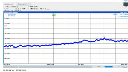
NTNV-DC_5A_n78A-PC2-30-5+15-M+H-QPSK-IDLE-DFT-BPSK-In ner_1RB_Left-6000-26000-PASS
