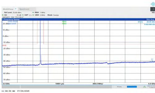
NTNV-DC_5A_n78A-PC2-30-5+15-M+M-QPSK-IDLE-DFT-QPSK-Inner_1RB_Left-3000-6000-PASS
