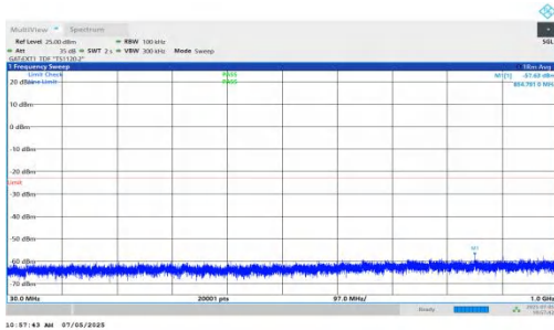
NTNV-DC_5A_n78A-PC2-30-5+10-M+L-QPSK-IDLE-DFT-BPSK-In ner_1RB_Left-30-1000-PASS
