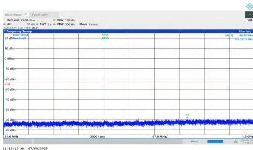
NTNV-DC_5A_n78A-PC2-30-5+10-M+M-QPSK-IDLE-DFT-QPSK-Inner_1RB_Left-30-1000-PASS
