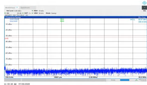
NTNV-DC_5A_n78A-PC2-30-5+15-M+L-QPSK-IDLE-DFT-QPSK-In ner_1RB_Left-0.15-30-PASS
