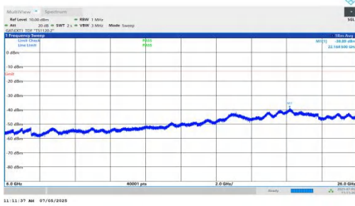
NTNV-DC_5A_n78A-PC2-30-5+10-M+M-QPSK-IDLE-DFT-BPSK-Inner_1RB_Right-6000-26000-PASS
