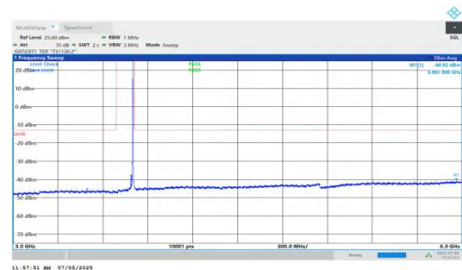
NTNV-DC_5A_n78A-PC2-30-5+15-M+H-QPSK-IDLE-DFT-QPSK-Inner_1RB_Right-3000-6000-PASS
