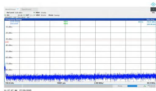
NTNV-DC_5A_n78A-PC2-30-5+10-M+M-QPSK-IDLE-DFT-BPSK-In ner_1RB_Left-0.15-30-PASS
