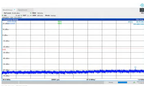
NTNV-DC_5A_n78A-PC2-30-5+15-M+H-QPSK-IDLE-DFT-BPSK-Inner_1RB_Left-30-1000-PASS
