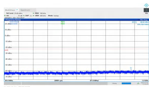
NTNV-DC_5A_n78A-PC2-30-5+10-M+H-QPSK-IDLE-DFT-QPSK-Inner_1RB_Right-30-1000-PASS
