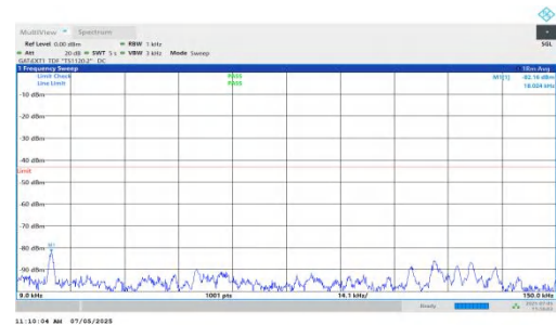
NTNV-DC_5A_n78A-PC2-30-5+10-M+M-QPSK-IDLE-DFT-BPSK-Inner_1RB_Right-0.009-0.15-PASS
