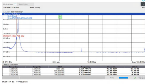
NTNV-DC_5A_n78A-PC2-30-5+90-M+L-QPSK-IDLE-DFT-BPSK-Edg e_1RB_Left-PASS
