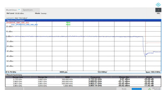
NTNV-DC_5A_n78A-PC2-30-5+90-M+H-QPSK-IDLE-DFT-QPSK-Outer_Full-PASS
