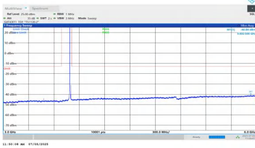
NTNV-DC_5A_n78A-PC2-30-5+15-M+H-QPSK-IDLE-DFT-BPSK-I nner_1RB_Left-3000-6000-PASS
