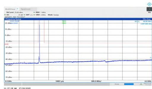
NTNV-DC_5A_n78A-PC2-30-5+15-M+L-QPSK-IDLE-DFT-QPSK-In ner_1RB_Right-3000-6000-PASS
