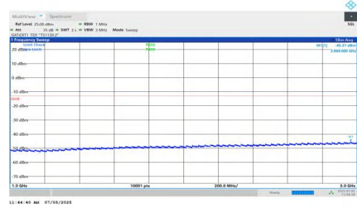
NTNV-DC_5A_n78A-PC2-30-5+15-M+M-QPSK-IDLE-DFT-QPSK-Inner_1RB_Left-1000-3000-PASS
