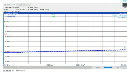
NTNV-DC_5A_n78A-PC2-30-5+15-M+H-QPSK-IDLE-DFT-QPSK-Inner_1RB_Left-1000-3000-PASS
