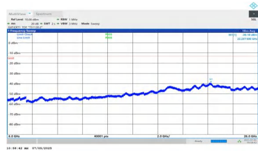
NTNV-DC_5A_n78A-PC2-30-5+10-M+L-QPSK-IDLE-DFT-BPSK-In ner_1RB_Left-6000-26000-PASS
