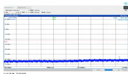
NTNV-DC_5A_n78A-PC2-30-5+10-M+M-QPSK-IDLE-DFT-BPSK-Inner_1RB_Right-30-1000-PASS
