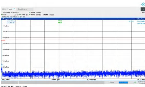
NTNV-DC_5A_n78A-PC2-30-5+10-M+L-QPSK-IDLE-DFT-QPSK-In ner_1RB_Right-0.15-30-PASS
