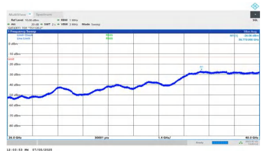
NTNV-DC_5A_n78A-PC2-30-5+20-M+L-QPSK-IDLE-DFT-BPSK-In ner_1RB_Right-26000-40000-PASS
