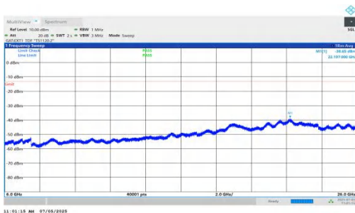
NTNV-DC_5A_n78A-PC2-30-5+10-M+L-QPSK-IDLE-DFT-BPSK-In ner_1RB_Right-6000-26000-PASS
