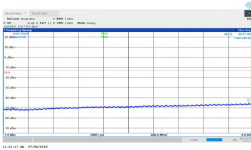
NTNV-DC_5A_n78A-PC2-30-5+10-M+H-QPSK-IDLE-DFT-BPSK-I nner_1RB_Right-1000-3000-PASS
