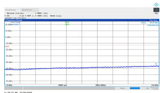
NTNV-DC_5A_n78A-PC2-30-5+15-M+L-QPSK-IDLE-DFT-BPSK-Inner_1RB_Left-1000-3000-PASS
