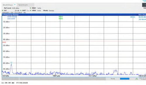
NTNV-DC_5A_n78A-PC2-30-5+15-M+M-QPSK-IDLE-DFT-BPSK-I nner_1RB_Left-0.009-0.15-PASS
