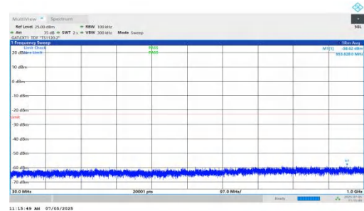
NTNV-DC_5A_n78A-PC2-30-5+10-M+M-QPSK-IDLE-DFT-QPSK-Inner_1RB_Right-30-1000-PASS
