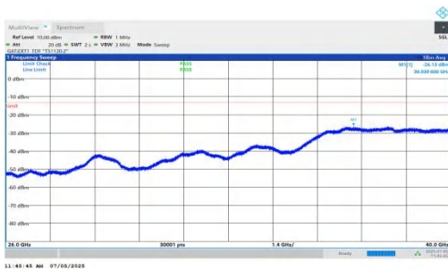
NTNV-DC_5A_n78A-PC2-30-5+15-M+M-QPSK-IDLE-DFT-QPSK-Inner_1RB_Left-26000-40000-PASS
