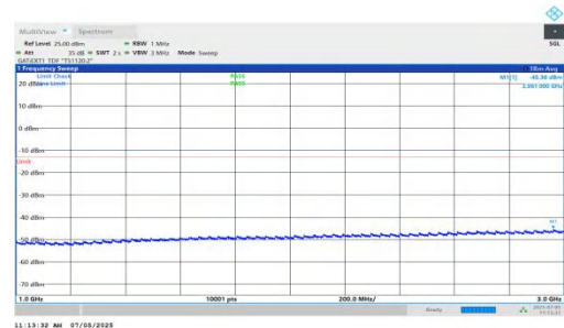
NTNV-DC_5A_n78A-PC2-30-5+10-M+M-QPSK-IDLE-DFT-QPSK-Inner_1RB_Left-1000-3000-PASS
