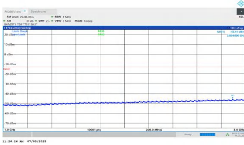
NTNV-DC_5A_n78A-PC2-30-5+10-M+H-QPSK-IDLE-DFT-QPSK-Inner_1RB_Right-1000-3000-PASS
