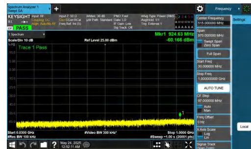
NTNV-DC_5A_n78A-PC2-30-5+90-M+M-QPSK-IDLE-DFT-QPSK-In ner_1RB_Right-30-1000-PASS
