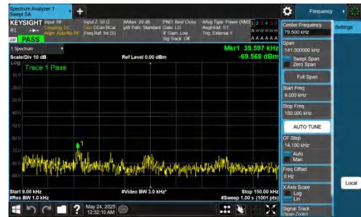
NTNV-DC_5A_n78A-PC2-30-5+80-M+H-QPSK-IDLE-DFT-QPSK-Inner_1RB_Right-0.009-0.15-PASS
