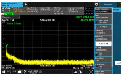
NTNV-DC_5A_n78A-PC2-30-5+100-M+M-QPSK-IDLE-DFT-QPSK- Inner_1RB_Right-0.15-30-PASS
