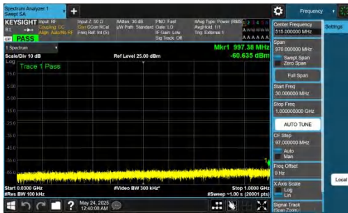
NTNV-DC_5A_n78A-PC2-30-5+90-M+L-QPSK-IDLE-DFT-QPSK-In ner_1RB_Left-30-1000-PASS
