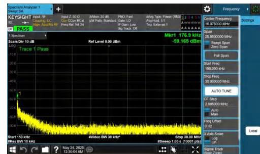
NTNV-DC_5A_n78A-PC2-30-5+80-M+H-QPSK-IDLE-DFT-QPSK-Inner_1RB_Left-0.15-30-PASS
