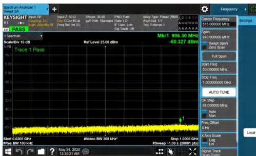
NTNV-DC_5A_n78A-PC2-30-5+90-M+L-QPSK-IDLE-DFT-BPSK-In ner_1RB_Left-30-1000-PASS
