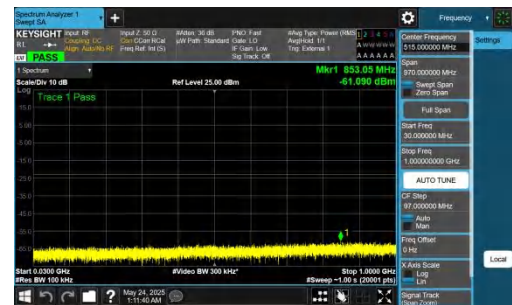
NTNV-DC_5A_n78A-PC2-30-5+100-M+M-QPSK-IDLE-DFT-QPSK-I nner_1RB_Right-30-1000-PASS
