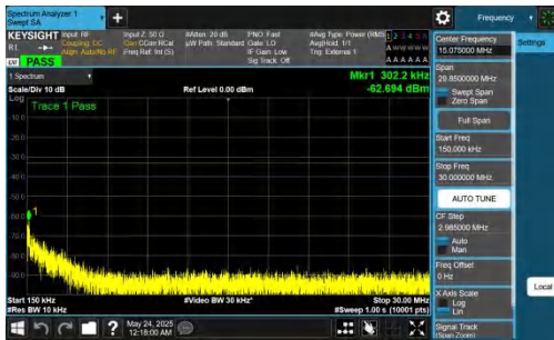
NTNV-DC_5A_n78A-PC2-30-5+80-M+M-QPSK-IDLE-DFT-BPSK-I nner_1RB_Right-0.15-30-PASS
