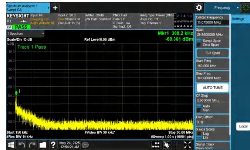
NTNV-DC_5A_n78A-PC2-30-5+90-M+H-QPSK-IDLE-DFT-BPSK-Inner_1RB_Left-0.15-30-PASS
