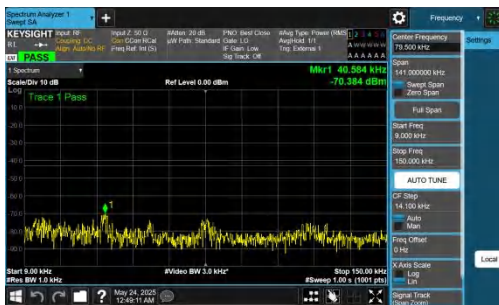
NTNV-DC_5A_n78A-PC2-30-5+90-M+M-QPSK-IDLE-DFT-QPSK-I nner_1RB_Left-0.009-0.15-PASS
