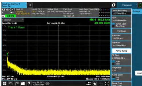
NTNV-DC_5A_n78A-PC2-30-5+90-M+M-QPSK-IDLE-DFT-QPSK-I nner_1RB_Right-0.15-30-PASS
