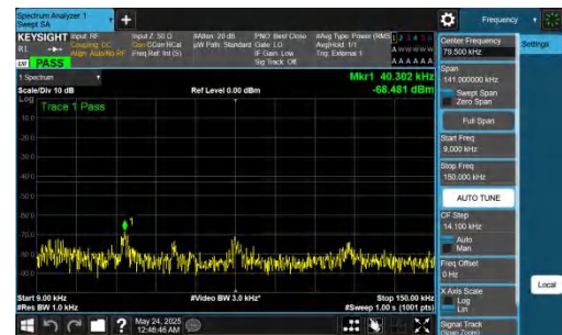
NTVN-DC_5A_n78A-PC2-30-5+90-M+M-QPSK-IDLE-DFT-BPSK-Inner_1RB_Right-0.009-0.15-PASS
