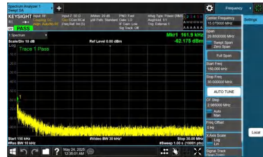
NTNV-DC_5A_n78A-PC2-30-5+90-M+L-QPSK-IDLE-DFT-BPSK-In ner_1RB_Left-0.15-30-PASS
