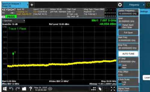
NTNV-DC_5A_n78A-PC2-30-5+80-M+H-QPSK-IDLE-DFT-BPSK-Inner_1RB_Right-6000-26000-PASS
