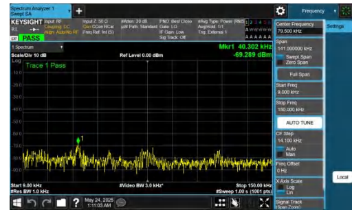
NTNV-DC_5A_n78A-PC2-30-5+100-M+M-QPSK-IDLE-DFT-QPSK-I nner_1RB_Right-0.009-0.15-PASS
