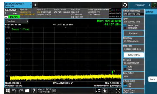
NTNV-DC_5A_n78A-PC2-30-5+90-M+L-QPSK-IDLE-DFT-BPSK-In ner_1RB_Right-30-1000-PASS
