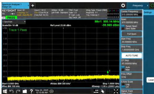
NTNV-DC_5A_n78A-PC2-30-5+80-M+M-QPSK-IDLE-DFT-BPSK-In nner_1RB_Left-30-1000-PASS
