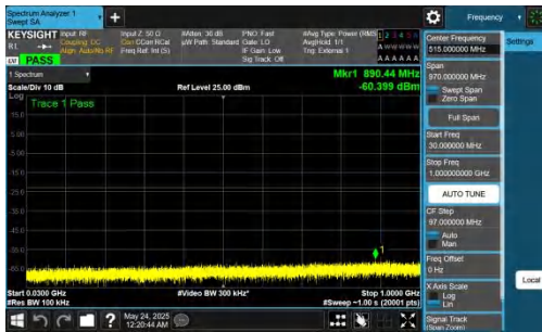
NTNV-DC_5A_n78A-PC2-30-5+80-M+M-QPSK-IDLE-DFT-QPSK-I nner_1RB_Left-30-1000-PASS
