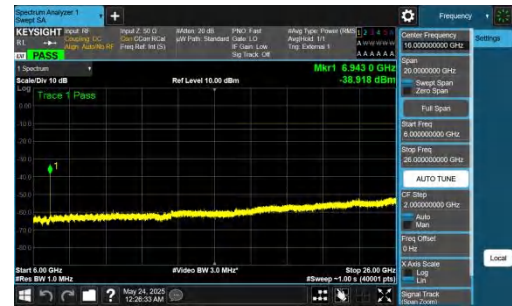
NTNV-DC_5A_n78A-PC2-30-5+80-M+H-QPSK-IDLE-DFT-BPSK-In ner_1RB_Left-6000-26000-PASS
