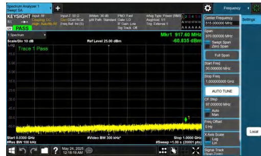
NTNV-DC_5A_n78A-PC2-30-5+80-M+M-QPSK-IDLE-DFT-BPSK-In ner_1RB_Right-30-1000-PASS
