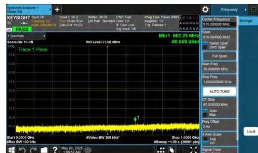
NTNV-DC_5A_n78A-PC2-30-5+100-M+M-QPSK-IDLE-DFT-BPSK-I- nner_1RB_Right-30-1000-PASS
