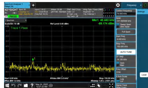
NTNV-DC_5A_n78A-PC2-30-5+80-M+H-QPSK-IDLE-DFT-BPSK-In ner_1RB_Right-0.009-0.15-PASS
