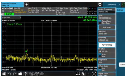
NTNV-DC_5A_n78A-PC2-30-5+100-M+M-QPSK-IDLE-DFT-QPSK- Inner_1RB_Left-0.009-0.15-PASS
