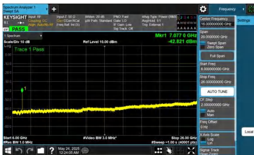
NTVN-DC_5A_n78A-PC2-30-5+80-M+M-QPSK-IDLE-DFT-QPSK-Inner_1RB_Right-6000-26000-PASS
