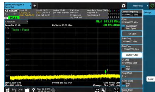
NTVN-DC_5A_n78A-PC2-30-5+90-M+M-QPSK-IDLE-DFT-BPSK-Inner_1RB_Right-30-1000-PASS
