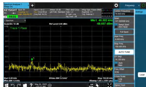
NTNV-DC_5A_n78A-PC2-30-5+90-M+H-QPSK-IDLE-DFT-QPSK-In ner_1RB_Right-0.009-0.15-PASS
