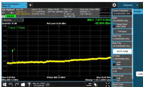
NTNV-DC_5A_n78A-PC2-30-5+90-M+L-QPSK-IDLE-DFT-QPSK-In ner_1RB_Right-6000-26000-PASS
