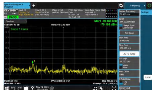
NTNV-DC_5A_n78A-PC2-30-5+90-M+L-QPSK-IDLE-DFT-QPSK-In ner_1RB_Right-0.009-0.15-PASS
