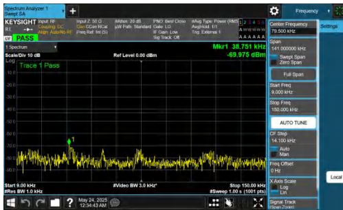
NTNV-DC_5A_n78A-PC2-30-5+90-M+L-QPSK-IDLE-DFT-BPSK-In ner_1RB_Left-0.009-0.15-PASS
