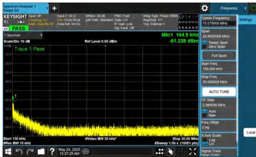
NTNV-DC_5A_n78A-PC2-30-5+90-M+L-QPSK-IDLE-DFT-BPSK-In ner_1RB_Right-0.15-30-PASS
