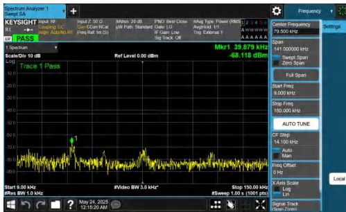
NTNV-DC_5A_n78A-PC2-30-5+80-M+M-QPSK-IDLE-DFT-BPSK-In nner_1RB_Left-0.009-0.15-PASS
