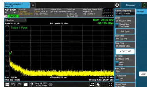
NTNV-DC_5A_n78A-PC2-30-5+90-M+M-QPSK-IDLE-DFT-QPSK-In ner_1RB_Left-0.15-30-PASS
