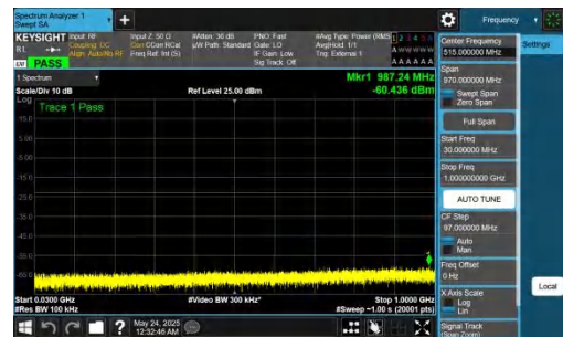
NTNV-DC_5A_n78A-PC2-30-5+80-M+H-QPSK-IDLE-DFT-QPSK-Inner_1RB_Right-30-1000-PASS
