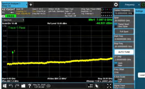
NTNV-DC_5A_n78A-PC2-30-5+100-M+M-QPSK-IDLE-DFT-BPSK- Inner_1RB_Right-6000-26000-PASS
