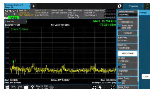
NTNV-DC_5A_n78A-PC2-30-5+80-M+M-QPSK-IDLE-DFT-BPSK-In ner_1RB_Right-0.009-0.15-PASS
