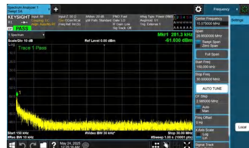
NTVN-DC_5A_n78A-PC2-30-5+80-M+H-QPSK-IDLE-DFT-BPSK-Inner_1RB_Left-0.15-30-PASS
