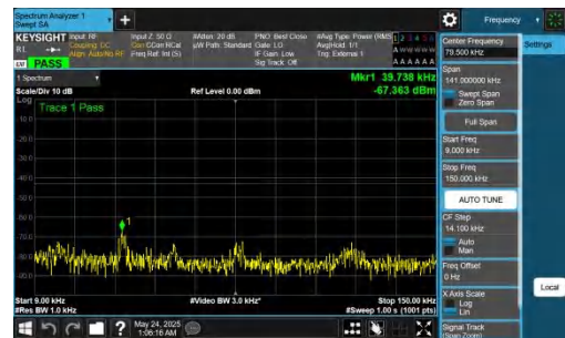
NTNV-DC_5A_n78A-PC2-30-5+100-M+M-QPSK-IDLE-DFT-BPSK-I- nner_1RB_Right-0.009-0.15-PASS
