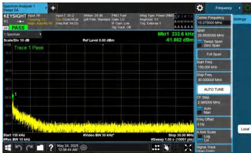
NTNV-DC_5A_n78A-PC2-30-5+90-M+H-QPSK-IDLE-DFT-BPSK-In nner_1RB_Right-0.15-30-PASS
