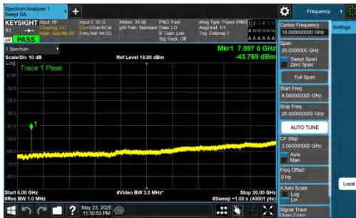
NTNV-DC_5A_n78A-PC2-30-5+60-M+H-QPSK-IDLE-DFT-BPSK-Inner_1RB_Right-6000-26000-PASS
