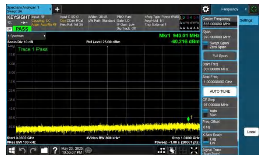
NTNV-DC_5A_n78A-PC2-30-5+50-M+M-QPSK-IDLE-DFT-QPSK-In ner_1RB_Right-30-1000-PASS
