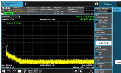
NTNV-DC_5A_n78A-PC2-30-5+80-M+L-QPSK-IDLE-DFT-BPSK-In ner_1RB_Right-0.15-30-PASS
