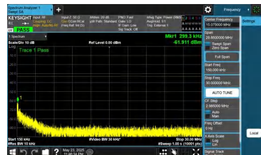
NTNV-DC_5A_n78A-PC2-30-5+70-M+M-QPSK-IDLE-DFT-BPSK-In ner_1RB_Left-0.15-30-PASS
