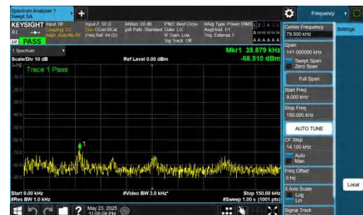
NTNV-DC_5A_n78A-PC2-30-5+50-M+H-QPSK-IDLE-DFT-QPSK-In ner_1RB_Right-0.009-0.15-PASS
