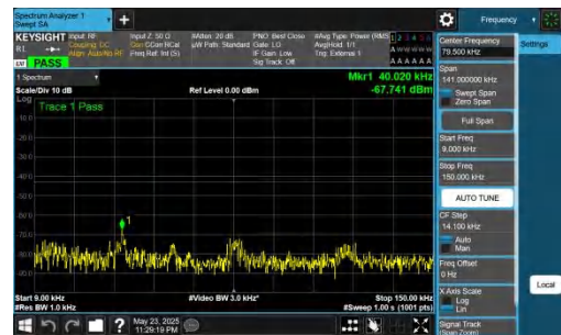
NTNV-DC_5A_n78A-PC2-30-5+60-M+H-QPSK-IDLE-DFT-BPSK-In ner_1RB_Right-0.009-0.15-PASS
