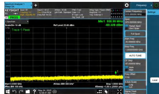
NTNV-DC_5A_n78A-PC2-30-5+80-M+L-QPSK-IDLE-DFT-BPSK-In ner_1RB_Right-30-1000-PASS
