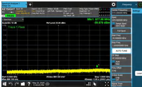
NTNV-DC_5A_n78A-PC2-30-5+50-M+H-QPSK-IDLE-DFT-QPSK-I nner_1RB_Left-30-1000-PASS
