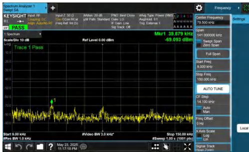
NTVN-DC_5A_n78A-PC2-30-5+60-M+M-QPSK-IDLE-DFT-BPSK-Inner_1RB_Left-0.009-0.15-PASS
