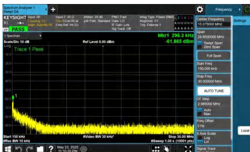
NTNV-DC_5A_n78A-PC2-30-5+60-M+L-QPSK-IDLE-DFT-BPSK-In ner_1RB_Right-0.15-30-PASS
