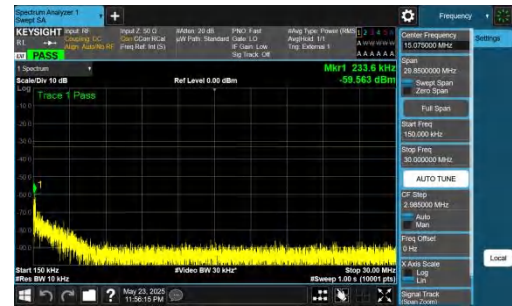
NTNV-DC_5A_n78A-PC2-30-5+70-M+H-QPSK-IDLE-DFT-BPSK-Inner_1RB_Left-0.15-30-PASS
