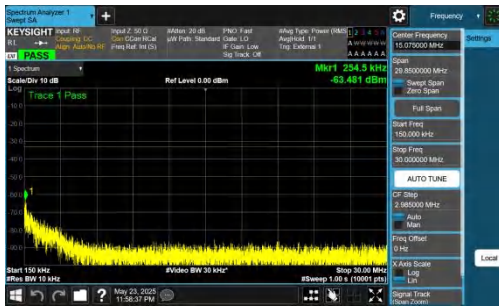
NTNV-DC_5A_n78A-PC2-30-5+70-M+H-QPSK-IDLE-DFT-BPSK-I nner_1RB_Right-0.15-30-PASS
