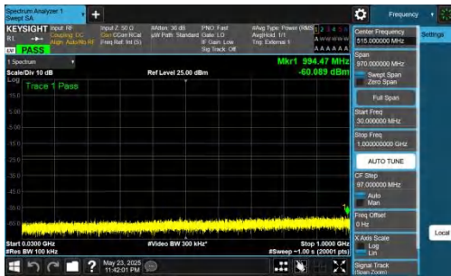
NTNV-DC_5A_n78A-PC2-30-5+70-M+L-QPSK-IDLE-DFT-QPSK-In ner_1RB_Left-30-1000-PASS
