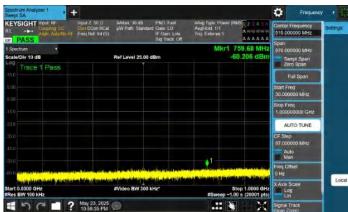
NTNV-DC_5A_n78A-PC2-30-5+50-M+H-QPSK-IDLE-DFT-BPSK-Inner_1RB_Left-30-1000-PASS
