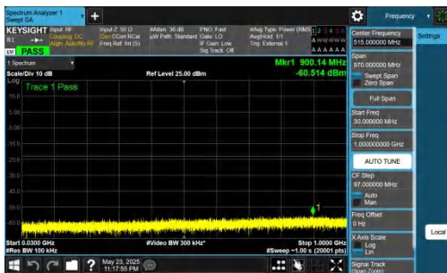
NTVN-DC_5A_n78A-PC2-30-5+60-M+M-QPSK-IDLE-DFT-BPSK-Inner_1RB_Left-30-1000-PASS
