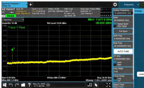
NTNV-DC_5A_n78A-PC2-30-5+60-M+L-QPSK-IDLE-DFT-BPSK-In ner_1RB_Right-6000-26000-PASS
