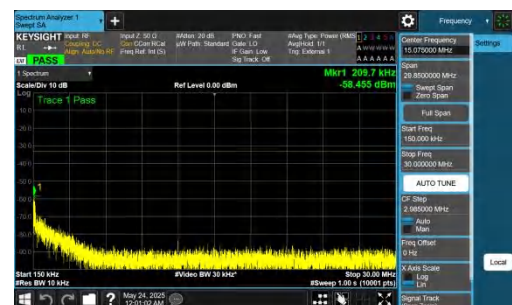
NTNV-DC_5A_n78A-PC2-30-5+70-M+H-QPSK-IDLE-DFT-QPSK-In ner_1RB_Left-0.15-30-PASS
