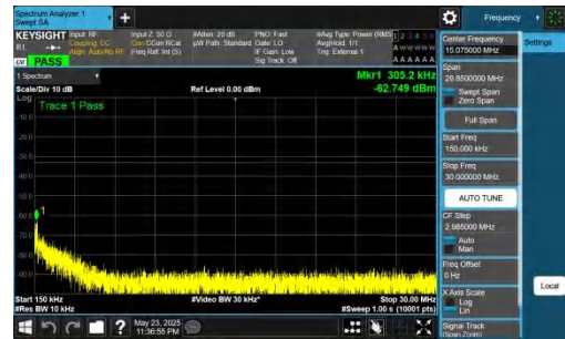
NTNV-DC_5A_n78A-PC2-30-5+70-M+L-QPSK-IDLE-DFT-BPSK-In ner_1RB_Left-0.15-30-PASS
