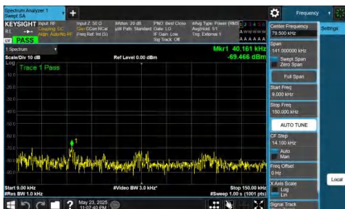
NTNV-DC_5A_n78A-PC2-30-5+60-M+L-QPSK-IDLE-DFT-BPSK-Inner_1RB_Left-0.009-0.15-PASS
