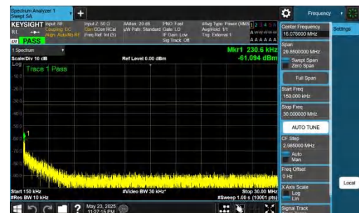
NTNV-DC_5A_n78A-PC2-30-5+60-M+H-QPSK-IDLE-DFT-BPSK-Inner_1RB_Left-0.15-30-PASS
