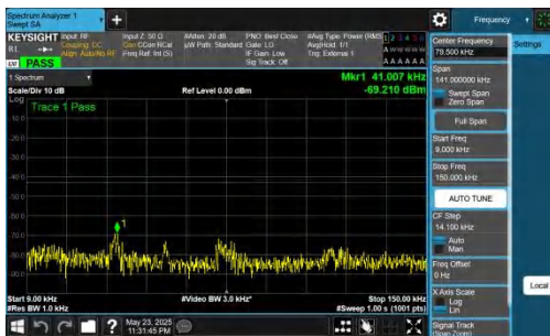
NTNV-DC_5A_n78A-PC2-30-5+60-M+H-QPSK-IDLE-DFT-QPSK-Inner_1RB_Left-0.009-0.15-PASS
