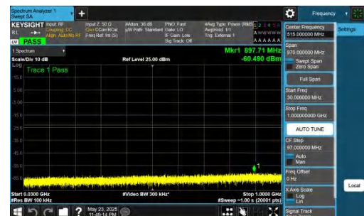
NTVN-DC_5A_n78A-PC2-30-5+70-M+M-QPSK-IDLE-DFT-BPSK-Inner_1RB_Right-30-1000-PASS
