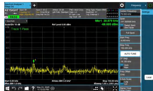
NTNV-DC_5A_n78A-PC2-30-5+60-M+L-QPSK-IDLE-DFT-BPSK-In ner_1RB_Right-0.009-0.15-PASS
