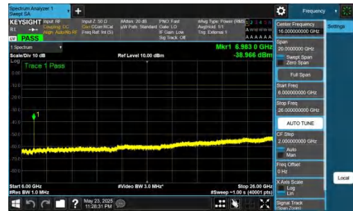
NTNV-DC_5A_n78A-PC2-30-5+60-M+H-QPSK-IDLE-DFT-BPSK-In ner_1RB_Left-6000-26000-PASS
