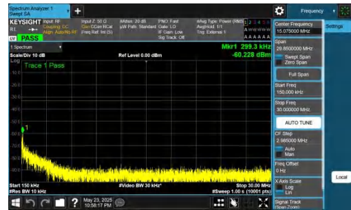
NTNV-DC_5A_n78A-PC2-30-5+50-M+H-QPSK-IDLE-DFT-BPSK-Inner_1RB_Left-0.15-30-PASS
