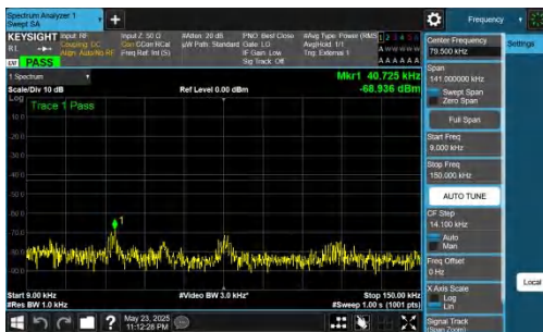
NTNV-DC_5A_n78A-PC2-30-5+60-M+L-QPSK-IDLE-DFT-QPSK-In ner_1RB_Left-0.009-0.15-PASS
