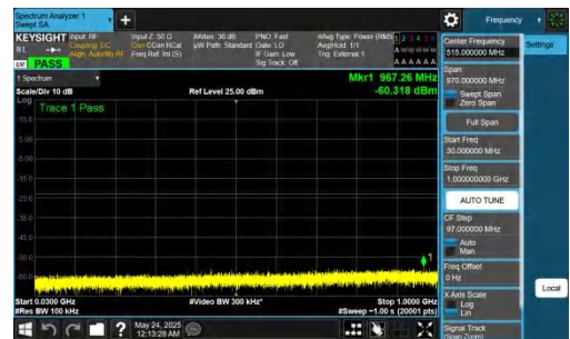
NTNV-DC_5A_n78A-PC2-30-5+80-M+L-QPSK-IDLE-DFT-QPSK-In ner_1RB_Right-30-1000-PASS
