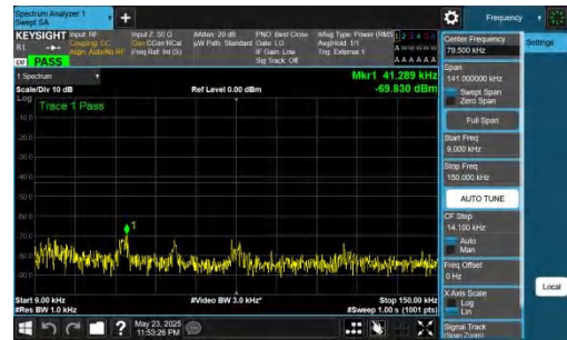
NTNV-DC_5A_n78A-PC2-30-5+70-M+M-QPSK-IDLE-DFT-QPSK-In ner_1RB_Right-0.009-0.15-PASS
