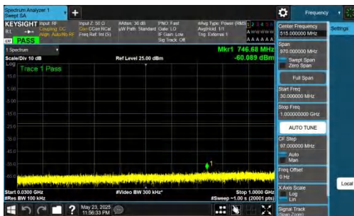
NTNV-DC_5A_n78A-PC2-30-5+70-M+H-QPSK-IDLE-DFT-BPSK-Inner_1RB_Left-30-1000-PASS
