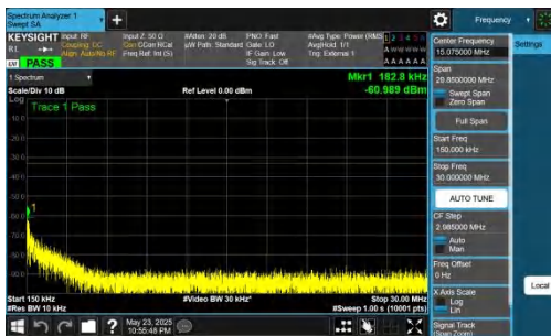
NTNV-DC_5A_n78A-PC2-30-5+50-M+M-QPSK-IDLE-DFT-QPSK-I nner_1RB_Right-0.15-30-PASS
