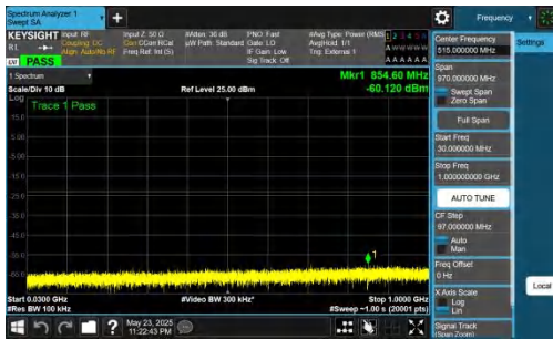
NTNV-DC_5A_n78A-PC2-30-5+60-M+M-QPSK-IDLE-DFT-QPSK-I nner_1RB_Left-30-1000-PASS
