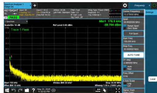
NTNV-DC_5A_n78A-PC2-30-5+60-M+H-QPSK-IDLE-DFT-QPSK-Inner_1RB_Left-0.15-30-PASS
