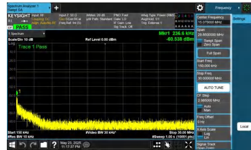
NTVN-DC_5A_n78A-PC2-30-5+60-M+M-QPSK-IDLE-DFT-BPSK-Inner_1RB_Left-0.15-30-PASS
