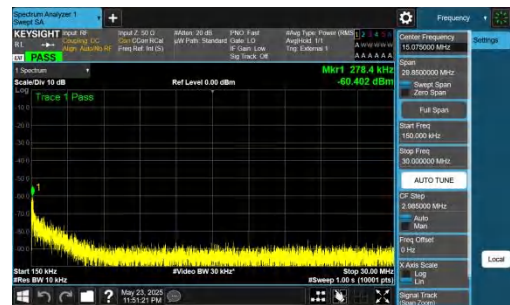
NTNV-DC_5A_n78A-PC2-30-5+70-M+M-QPSK-IDLE-DFT-QPSK-Inner_1RB_Left-0.15-30-PASS
