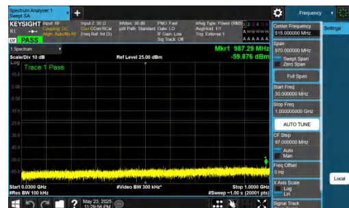
NTNV-DC_5A_n78A-PC2-30-5+60-M+H-QPSK-IDLE-DFT-BPSK-In ner_1RB_Right-30-1000-PASS
