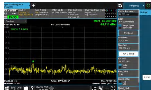
NTNV-DC_5A_n78A-PC2-30-5+60-M+M-QPSK-IDLE-DFT-QPSK-In ner_1RB_Right-0.009-0.15-PASS
