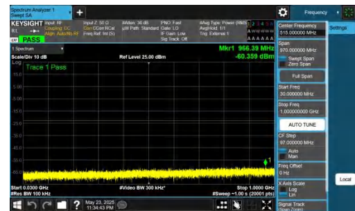
NTNV-DC_5A_n78A-PC2-30-5+60-M+H-QPSK-IDLE-DFT-QPSK-Inner_1RB_Right-30-1000-PASS
