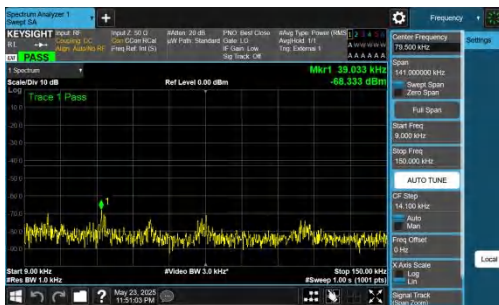
NTNV-DC_5A_n78A-PC2-30-5+70-M+M-QPSK-IDLE-DFT-QPSK-Inner_1RB_Left-0.009-0.15-PASS
