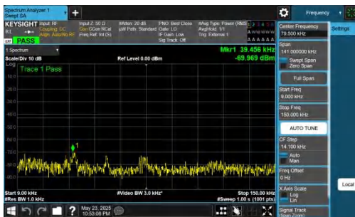
NTNV-DC_5A_n78A-PC2-30-5+50-M+M-QPSK-IDLE-DFT-QPSK-Inner_1RB_Left-0.009-0.15-PASS
