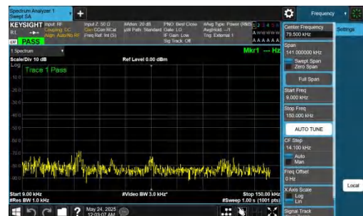
NTNV-DC_5A_n78A-PC2-30-5+70-M+H-QPSK-IDLE-DFT-QPSK-In ner_1RB_Right-0.009-0.15-PASS
