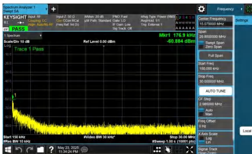
NTNV-DC_5A_n78A-PC2-30-5+60-M+H-QPSK-IDLE-DFT-QPSK-Inner_1RB_Right-0.15-30-PASS
