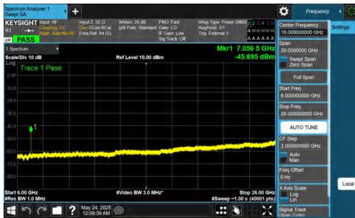
NTNV-DC_5A_n78A-PC2-30-5+80-M+L-QPSK-IDLE-DFT-BPSK-In ner_1RB_Right-6000-26000-PASS
