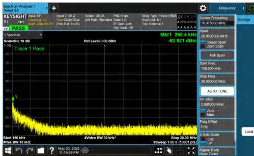
NTNV-DC_5A_n78A-PC2-30-5+60-M+M-QPSK-IDLE-DFT-BPSK-I nner_1RB_Right-0.15-30-PASS
