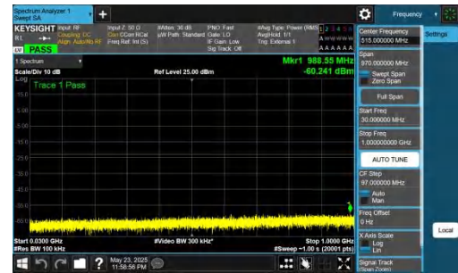
NTNV-DC_5A_n78A-PC2-30-5+70-M+H-QPSK-IDLE-DFT-BPSK-In ner_1RB_Right-30-1000-PASS
