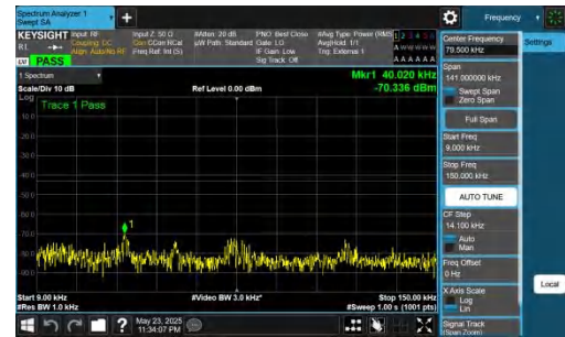
NTNV-DC_5A_n78A-PC2-30-5+60-M+H-QPSK-IDLE-DFT-QPSK-Inner_1RB_Right-0.009-0.15-PASS
