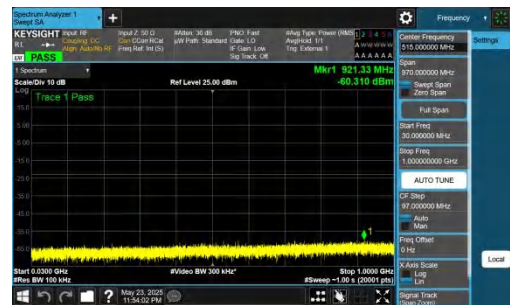
NTNV-DC_5A_n78A-PC2-30-5+70-M+M-QPSK-IDLE-DFT-QPSK-In ner_1RB_Right-30-1000-PASS
