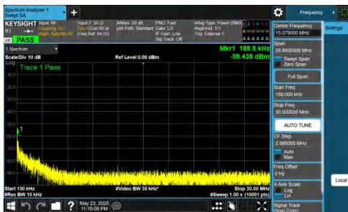
NTNV-DC_5A_n78A-PC2-30-5+60-M+L-QPSK-IDLE-DFT-QPSK-In ner_1RB_Right-0.15-30-PASS
