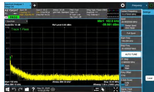
NTNV-DC_5A_n78A-PC2-30-5+50-M+M-QPSK-IDLE-DFT-QPSK-Inner_1RB_Left-0.15-30-PASS
