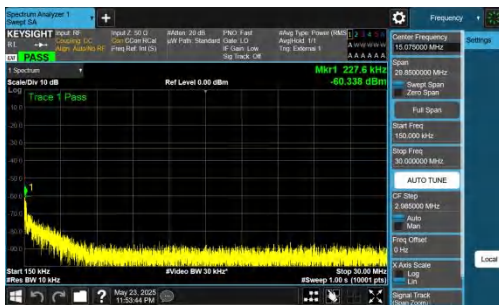
NTNV-DC_5A_n78A-PC2-30-5+70-M+M-QPSK-IDLE-DFT-QPSK-I nner_1RB_Right-0.15-30-PASS
