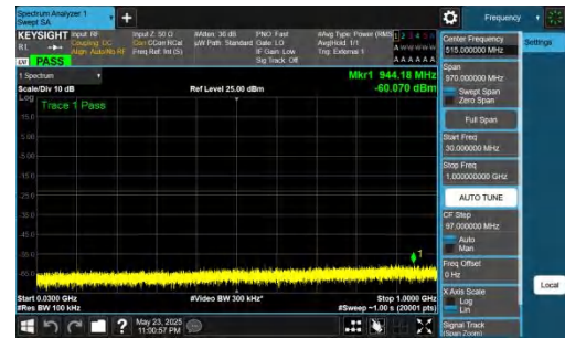
NTNV-DC_5A_n78A-PC2-30-5+50-M+H-QPSK-IDLE-DFT-BPSK-In ner_1RB_Right-30-1000-PASS
