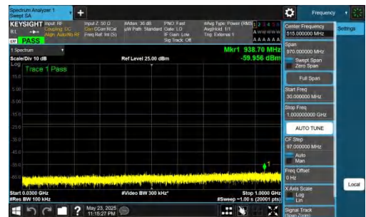
NTNV-DC_5A_n78A-PC2-30-5+60-M+L-QPSK-IDLE-DFT-QPSK-In ner_1RB_Right-30-1000-PASS
