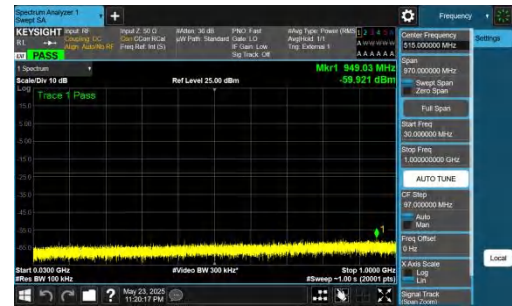
NTNV-DC_5A_n78A-PC2-30-5+60-M+M-QPSK-IDLE-DFT-BPSK-In ner_1RB_Right-30-1000-PASS
