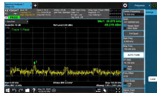
NTNV-DC_5A_n78A-PC2-30-5+50-M+M-QPSK-IDLE-DFT-BPSK-In ner_1RB_Right-0.009-0.15-PASS
