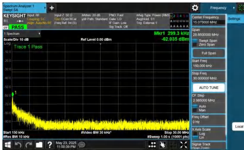
NTNV-DC_5A_n78A-PC2-30-5+50-M+H-QPSK-IDLE-DFT-BPSK-I nner_1RB_Right-0.15-30-PASS
