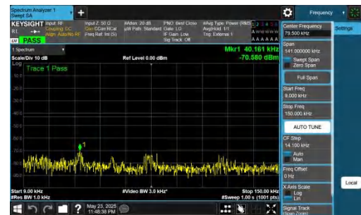
NTVN-DC_5A_n78A-PC2-30-5+70-M+M-QPSK-IDLE-DFT-BPSK-Inner_1RB_Right-0.009-0.15-PASS
