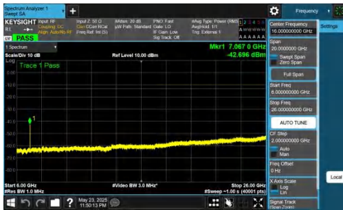
NTNV-DC_5A_n78A-PC2-30-5+70-M+M-QPSK-IDLE-DFT-BPSK-Inner_1RB_Right-6000-26000-PASS
