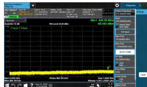
NTNV-DC_5A_n78A-PC2-30-5+60-M+L-QPSK-IDLE-DFT-BPSK-In ner_1RB_Right-30-1000-PASS
