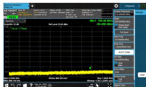
NTNV-DC_5A_n78A-PC2-30-5+70-M+H-QPSK-IDLE-DFT-QPSK-In ner_1RB_Right-30-1000-PASS
