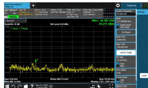
NTNV-DC_5A_n78A-PC2-30-5+70-M+L-QPSK-IDLE-DFT-QPSK-In ner_1RB_Right-0.009-0.15-PASS
