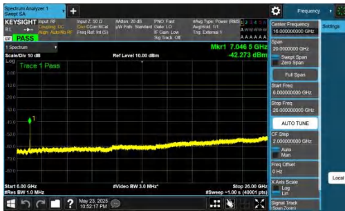
NTNV-DC_5A_n78A-PC2-30-5+50-M+M-QPSK-IDLE-DFT-BPSK-Inner_1RB_Right-6000-26000-PASS
