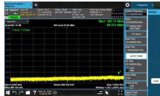
NTNV-DC_5A_n78A-PC2-30-5+70-M+L-QPSK-IDLE-DFT-BPSK-In ner_1RB_Right-30-1000-PASS
