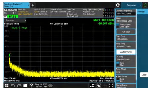
NTNV-DC_5A_n78A-PC2-30-5+80-M+L-QPSK-IDLE-DFT-QPSK-In ner_1RB_Left-0.15-30-PASS
