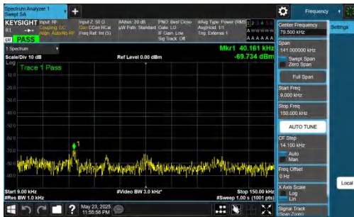
NTNV-DC_5A_n78A-PC2-30-5+70-M+H-QPSK-IDLE-DFT-BPSK-Inner_1RB_Left-0.009-0.15-PASS
