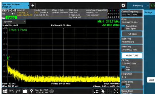
NTNV-DC_5A_n78A-PC2-30-5+80-M+L-QPSK-IDLE-DFT-QPSK-In ner_1RB_Right-0.15-30-PASS
