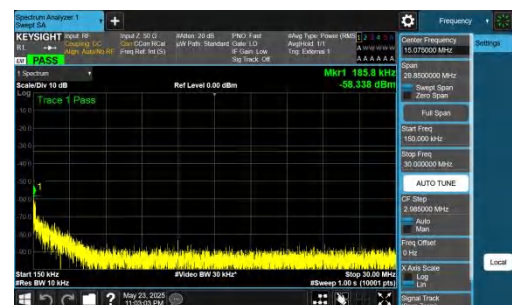
NTNV-DC_5A_n78A-PC2-30-5+50-M+H-QPSK-IDLE-DFT-QPSK-In ner_1RB_Left-0.15-30-PASS
