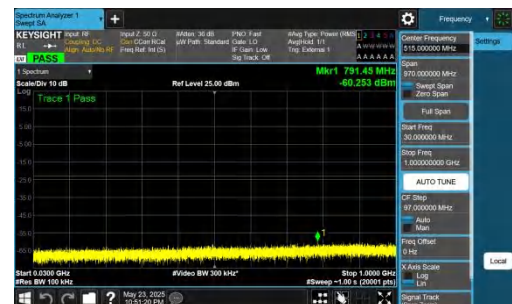
NTNV-DC_5A_n78A-PC2-30-5+50-M+M-QPSK-IDLE-DFT-BPSK-In ner_1RB_Right-30-1000-PASS
