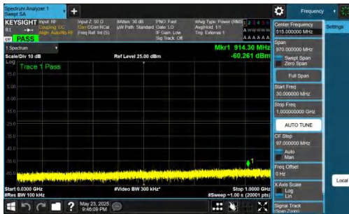
NTNV-DC_5A_n78A-PC2-30-5+30-M+L-QPSK-IDLE-DFT-QPSK-In ner_1RB_Left-30-1000-PASS
