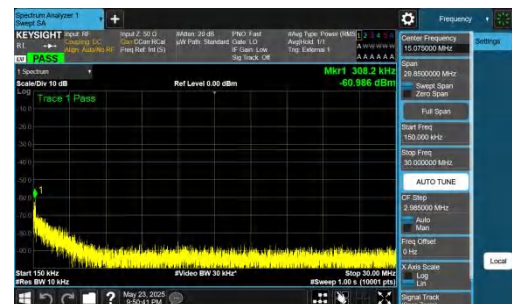
NTNV-DC_5A_n78A-PC2-30-5+30-M+M-QPSK-IDLE-DFT-BPSK-In ner_1RB_Left-0.15-30-PASS
