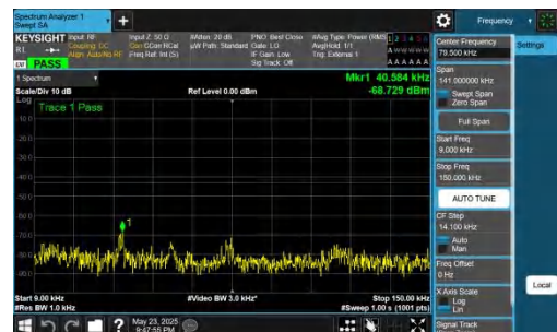
NTNV-DC_5A_n78A-PC2-30-5+30-M+L-QPSK-IDLE-DFT-QPSK-In ner_1RB_Right-0.009-0.15-PASS
