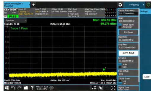
NTNV-DC_5A_n78A-PC2-30-5+30-M+L-QPSK-IDLE-DFT-BPSK-In ner_1RB_Right-30-1000-PASS
