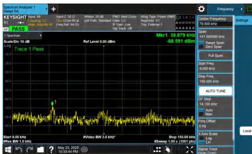
NTNV-DC_5A_n78A-PC2-30-5+40-M+H-QPSK-IDLE-DFT-QPSK-Inner_1RB_Left-0.009-0.15-PASS
