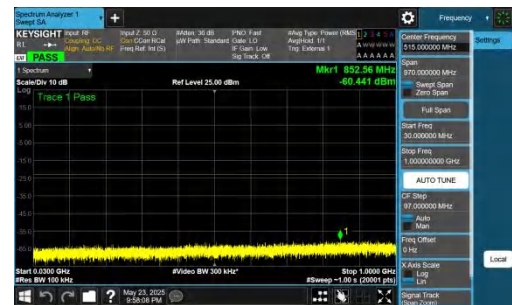
NTNV-DC_5A_n78A-PC2-30-5+30-M+M-QPSK-IDLE-DFT-QPSK-In ner_1RB_Right-30-1000-PASS
