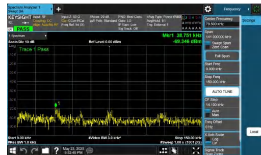
NTVN-DC_5A_n78A-PC2-30-5+30-M+M-QPSK-IDLE-DFT-BPSK-Inner_1RB_Right-0.009-0.15-PASS
