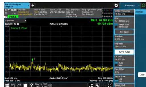
NTNV-DC_5A_n78A-PC2-30-5+30-M+H-QPSK-IDLE-DFT-QPSK-Inner_1RB_Right-0.009-0.15-PASS
