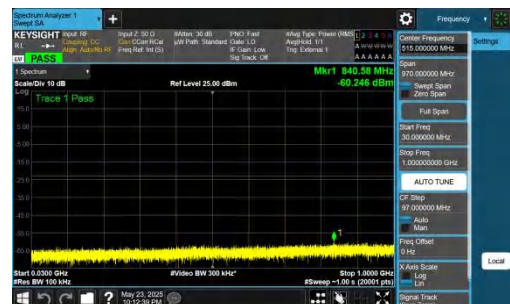
NTNV-DC_5A_n78A-PC2-30-5+40-M+L-QPSK-IDLE-DFT-BPSK-In ner_1RB_Right-30-1000-PASS
