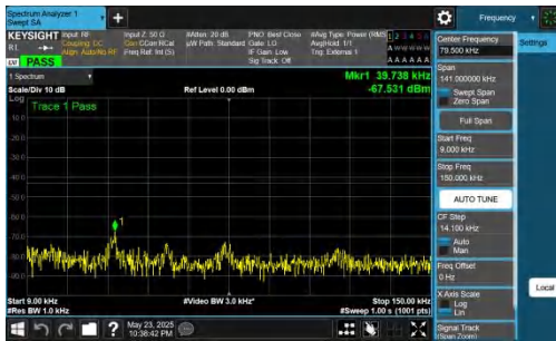
NTNV-DC_5A_n78A-PC2-30-5+50-M+L-QPSK-IDLE-DFT-BPSK-In ner_1RB_Left-0.009-0.15-PASS
