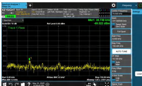
NTNV-DC_5A_n78A-PC2-30-5+40-M+L-QPSK-IDLE-DFT-BPSK-Inner_1RB_Left-0.009-0.15-PASS
