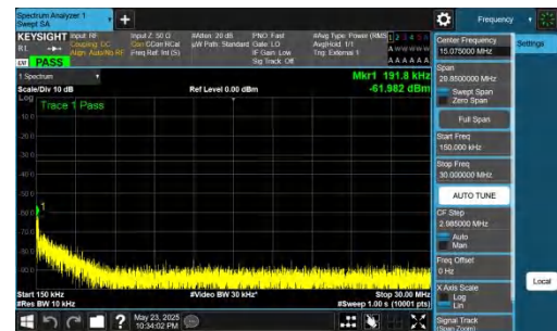
NTNV-DC_5A_n78A-PC2-30-5+40-M+H-QPSK-IDLE-DFT-QPSK-Inner_1RB_Left-0.15-30-PASS
