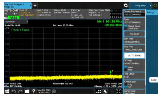
NTNV-DC_5A_n78A-PC2-30-5+25-M+H-QPSK-IDLE-DFT-QPSK-Inner_1RB_Right-30-1000-PASS
