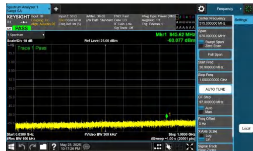
NTNV-DC_5A_n78A-PC2-30-5+40-M+L-QPSK-IDLE-DFT-QPSK-In_ner_1RB_Right-30-1000-PASS
