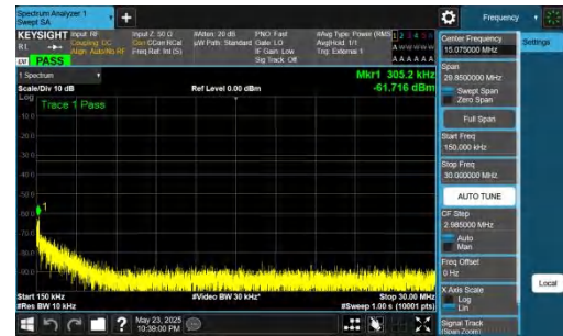
NTNV-DC_5A_n78A-PC2-30-5+50-M+L-QPSK-IDLE-DFT-BPSK-In ner_1RB_Left-0.15-30-PASS
