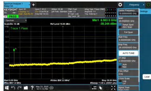
NTNV-DC_5A_n78A-PC2-30-5+40-M+L-QPSK-IDLE-DFT-BPSK-In ner_1RB_Left-6000-26000-PASS
