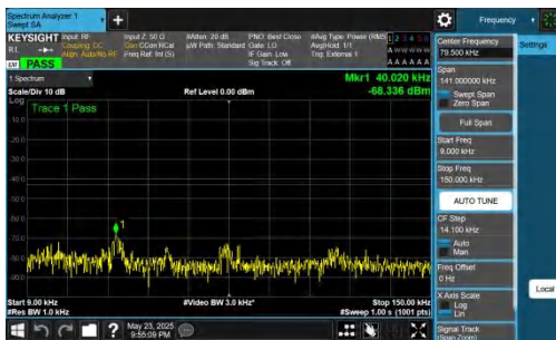
NTNV-DC_5A_n78A-PC2-30-5+30-M+M-QPSK-IDLE-DFT-QPSK-Inner_1RB_Left-0.009-0.15-PASS
