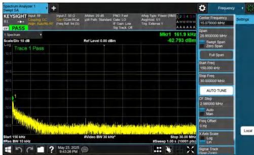
NTNV-DC_5A_n78A-PC2-30-5+30-M+L-QPSK-IDLE-DFT-BPSK-In ner_1RB_Right-0.15-30-PASS
