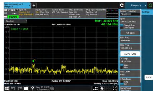
NTNV-DC_5A_n78A-PC2-30-5+40-M+L-QPSK-IDLE-DFT-BPSK-In ner_1RB_Right-0.009-0.15-PASS
