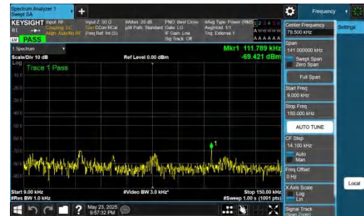
NTNV-DC_5A_n78A-PC2-30-5+30-M+M-QPSK-IDLE-DFT-QPSK-In ner_1RB_Right-0.009-0.15-PASS
