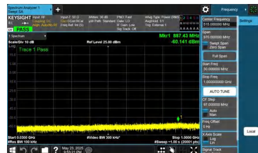
NTVN-DC_5A_n78A-PC2-30-5+30-M+M-QPSK-IDLE-DFT-BPSK-Inner_1RB_Right-30-1000-PASS
