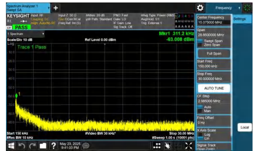
NTNV-DC_5A_n78A-PC2-30-5+30-M+L-QPSK-IDLE-DFT-BPSK-In ner_1RB_Left-0.15-30-PASS
