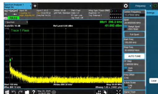
NTNV-DC_5A_n78A-PC2-30-5+40-M+L-QPSK-IDLE-DFT-BPSK-Inner_1RB_Left-0.15-30-PASS
