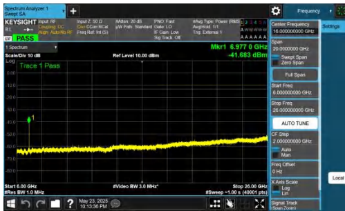
NTNV-DC_5A_n78A-PC2-30-5+40-M+L-QPSK-IDLE-DFT-BPSK-In ner_1RB_Right-6000-26000-PASS
