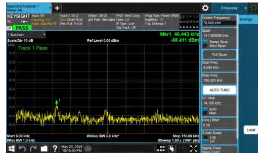
NTNV-DC_5A_n78A-PC2-30-5+40-M+L-QPSK-IDLE-DFT-QPSK-In_ner_1RB_Right-0.009-0.15-PASS
