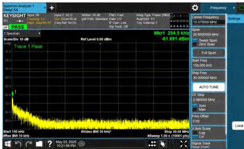
NTNV-DC_5A_n78A-PC2-30-5+40-M+M-QPSK-IDLE-DFT-BPSK-I nner_1RB_Right-0.15-30-PASS
