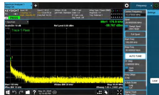
NTNV-DC_5A_n78A-PC2-30-5+40-M+L-QPSK-IDLE-DFT-QPSK-In ner_1RB_Left-0.15-30-PASS
