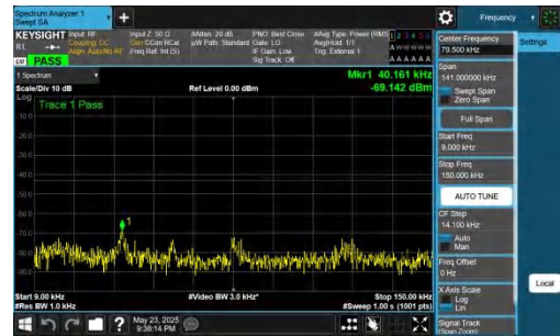
NTNV-DC_5A_n78A-PC2-30-5+25-M+H-QPSK-IDLE-DFT-QPSK-Inner_1RB_Right-0.009-0.15-PASS
