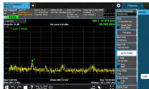
NTNV-DC_5A_n78A-PC2-30-5+25-M+M-QPSK-IDLE-DFT-QPSK-In ner_1RB_Right-0.009-0.15-PASS
