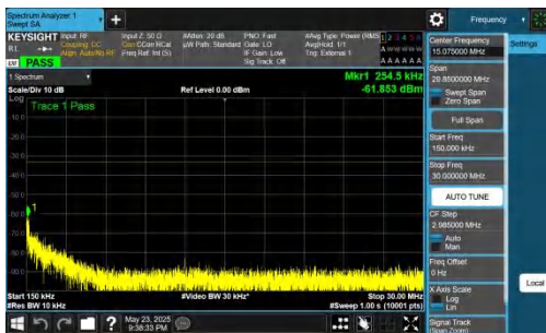
NTNV-DC_5A_n78A-PC2-30-5+25-M+H-QPSK-IDLE-DFT-QPSK-Inner_1RB_Right-0.15-30-PASS
