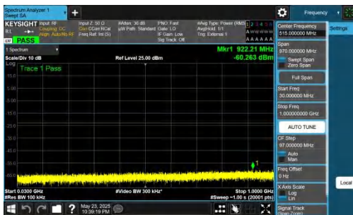
NTNV-DC_5A_n78A-PC2-30-5+50-M+L-QPSK-IDLE-DFT-BPSK-In ner_1RB_Left-30-1000-PASS
