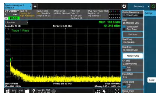
NTNV-DC_5A_n78A-PC2-30-5+50-M+L-QPSK-IDLE-DFT-QPSK-In ner_1RB_Left-0.15-30-PASS
