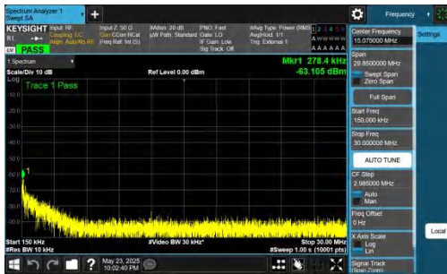
NTVN-DC_5A_n78A-PC2-30-5+30-M+H-QPSK-IDLE-DFT-BPSK-Inner_1RB_Right-0.15-30-PASS
