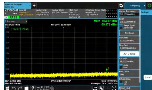
NTNV-DC_5A_n78A-PC2-30-5+40-M+H-QPSK-IDLE-DFT-BPSK-Inner_1RB_Right-30-1000-PASS
