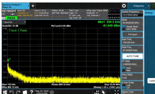
NTVN-DC_5A_n78A-PC2-30-5+30-M+M-QPSK-IDLE-DFT-BPSK-Inner_1RB_Right-0.15-30-PASS
