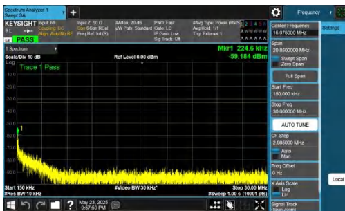
NTNV-DC_5A_n78A-PC2-30-5+30-M+M-QPSK-IDLE-DFT-QPSK-I nner_1RB_Right-0.15-30-PASS
