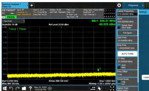
NTNV-DC_5A_n78A-PC2-30-5+30-M+H-QPSK-IDLE-DFT-BPSK-In nner_1RB_Left-30-1000-PASS
