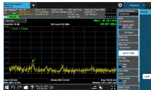
NTNV-DC_5A_n78A-PC2-30-5+25-M+H-QPSK-IDLE-DFT-BPSK-In ner_1RB_Right-0.009-0.15-PASS
