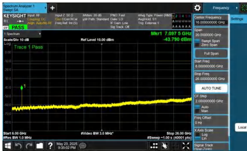
NTNV-DC_5A_n78A-PC2-30-5+25-M+H-QPSK-IDLE-DFT-BPSK-Inner_1RB_Right-6000-26000-PASS
