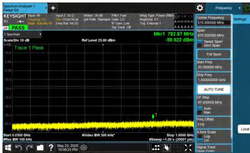
NTNV-DC_5A_n78A-PC2-30-5+30-M+H-QPSK-IDLE-DFT-QPSK-Inner_1RB_Left-30-1000-PASS
