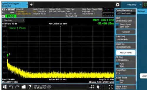
NTNV-DC_5A_n78A-PC2-30-5+50-M+L-QPSK-IDLE-DFT-BPSK-In ner_1RB_Right-0.15-30-PASS
