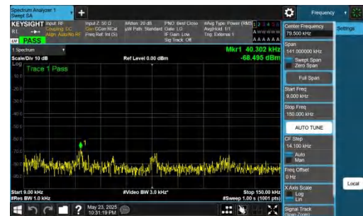
NTNV-DC_5A_n78A-PC2-30-5+40-M+H-QPSK-IDLE-DFT-BPSK-Inner_1RB_Right-0.009-0.15-PASS
