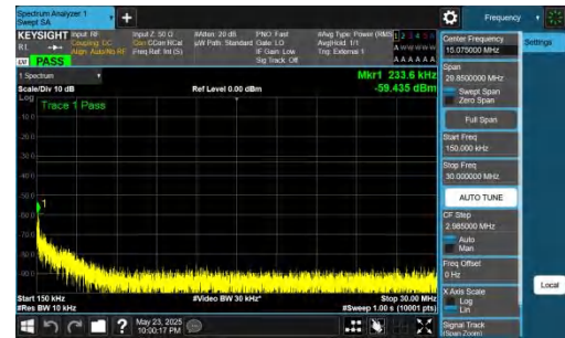
NTNV-DC_5A_n78A-PC2-30-5+30-M+H-QPSK-IDLE-DFT-BPSK-In ner_1RB_Left-0.15-30-PASS
