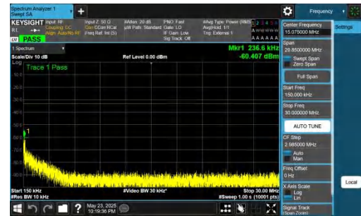
NTNV-DC_5A_n78A-PC2-30-5+40-M+M-QPSK-IDLE-DFT-BPSK-Inner_1RB_Left-0.15-30-PASS
