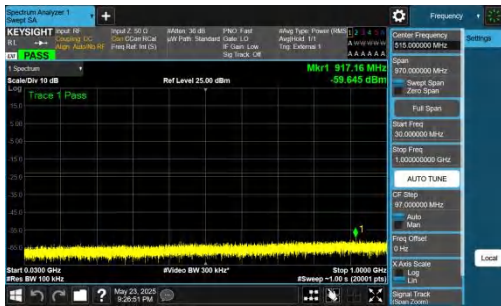
NTNV-DC_5A_n78A-PC2-30-5+25-M+M-QPSK-IDLE-DFT-QPSK-I nner_1RB_Left-30-1000-PASS
