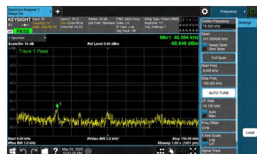
NTNV-DC_5A_n78A-PC2-30-5+50-M+L-QPSK-IDLE-DFT-BPSK-In ner_1RB_Right-0.009-0.15-PASS
