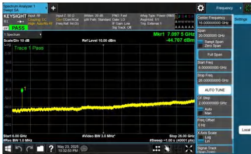
NTNV-DC_5A_n78A-PC2-30-5+40-M+H-QPSK-IDLE-DFT-BPSK-Inner_1RB_Right-6000-26000-PASS
