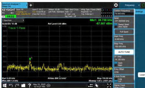
NTNV-DC_5A_n78A-PC2-30-5+40-M+L-QPSK-IDLE-DFT-QPSK-In ner_1RB_Left-0.009-0.15-PASS
