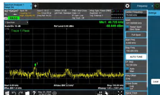
NTNV-DC_5A_n78A-PC2-30-5+40-M+M-QPSK-IDLE-DFT-QPSK-In ner_1RB_Right-0.009-0.15-PASS
