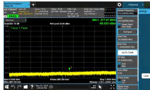
NTNV-DC_5A_n78A-PC2-30-5+20-M+H-QPSK-IDLE-DFT-BPSK-Inner_1RB_Right-30-1000-PASS
