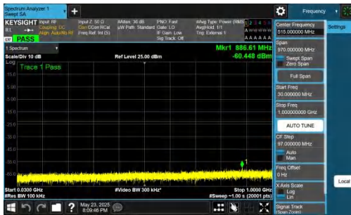
NTNV-DC_5A_n78A-PC2-30-5+10-M+H-QPSK-IDLE-DFT-QPSK-Inner_1RB_Left-30-1000-PASS
