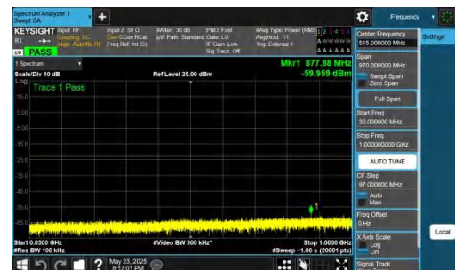
NTNV-DC_5A_n78A-PC2-30-5+15-M+L-QPSK-IDLE-DFT-BPSK-In ner_1RB_Right-30-1000-PASS
