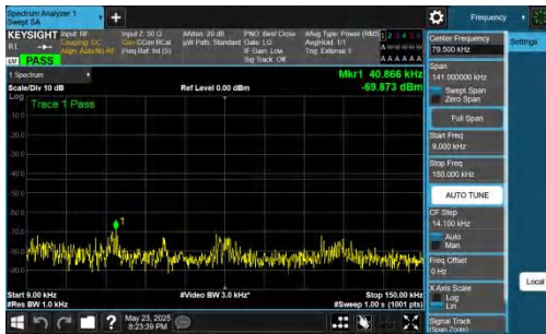
NTNV-DC_5A_n78A-PC2-30-5+15-M+M-QPSK-IDLE-DFT-BPSK-Inner_1RB_Left-0.009-0.15-PASS
