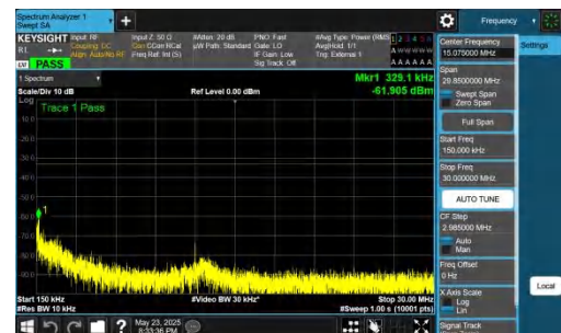
NTNV-DC_5A_n78A-PC2-30-5+15-M+H-QPSK-IDLE-DFT-BPSK-Inner_1RB_Left-0.15-30-PASS
