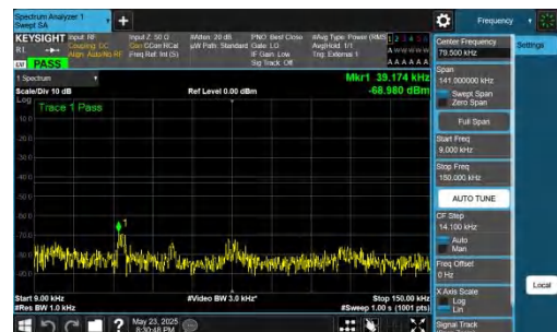
NTNV-DC_5A_n78A-PC2-30-5+15-M+M-QPSK-IDLE-DFT-QPSK-In ner_1RB_Right-0.009-0.15-PASS
