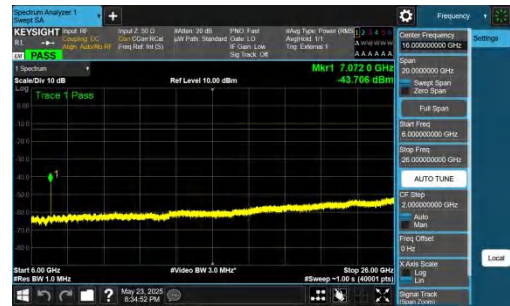
NTNV-DC_5A_n78A-PC2-30-5+15-M+H-QPSK-IDLE-DFT-BPSK-In ner_1RB_Left-6000-26000-PASS
