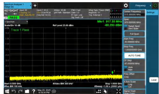
NTNV-DC_5A_n78A-PC2-30-5+25-M+L-QPSK-IDLE-DFT-QPSK-In_ner_1RB_Right-30-1000-PASS
