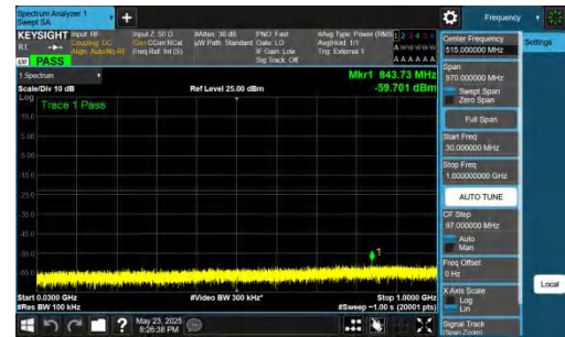
NTNV-DC_5A_n78A-PC2-30-5+15-M+M-QPSK-IDLE-DFT-BPSK-In ner_1RB_Right-30-1000-PASS
