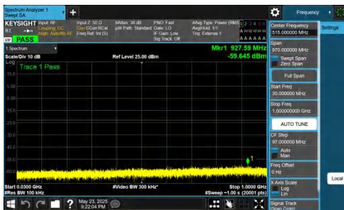
NTNV-DC_5A_n78A-PC2-30-5+25-M+M-QPSK-IDLE-DFT-BPSK-I nner_1RB_Left-30-1000-PASS
