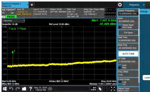
NTVN-DC_5A_n78A-PC2-30-5+10-M+M-QPSK-IDLE-DFT-BPSK-Inner_1RB_Right-6000-26000-PASS
