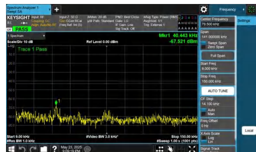
NTNV-DC_5A_n78A-PC2-30-5+20-M+H-QPSK-IDLE-DFT-QPSK-Inner_1RB_Right-0.009-0.15-PASS
