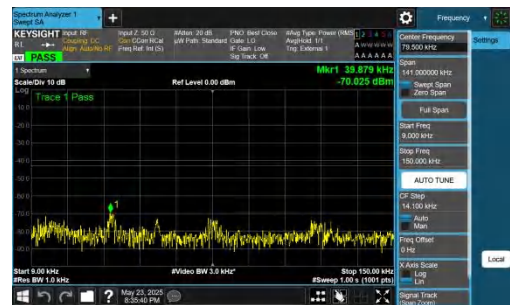
NTNV-DC_5A_n78A-PC2-30-5+15-M+H-QPSK-IDLE-DFT-BPSK-In ner_1RB_Right-0.009-0.15-PASS
