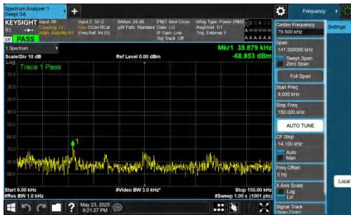
NTNV-DC_5A_n78A-PC2-30-5+25-M+M-QPSK-IDLE-DFT-BPSK-I nner_1RB_Left-0.009-0.15-PASS
