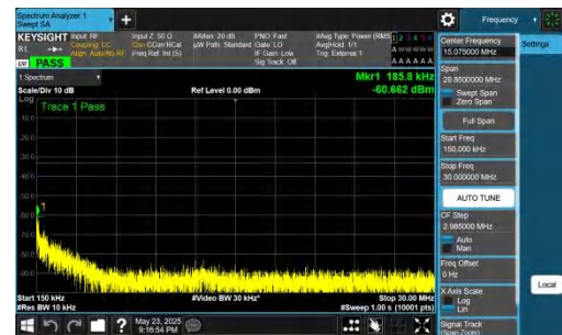
NTNV-DC_5A_n78A-PC2-30-5+25-M+L-QPSK-IDLE-DFT-QPSK-In ner_1RB_Left-0.15-30-PASS
