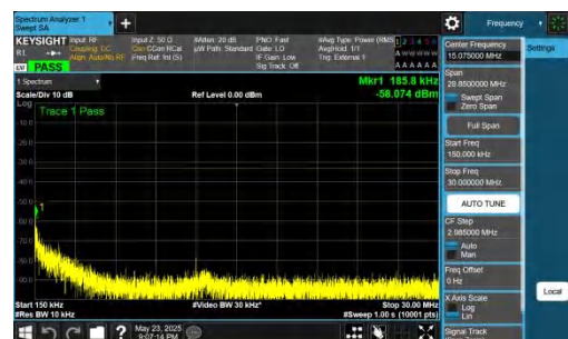
NTNV-DC_5A_n78A-PC2-30-5+20-M+H-QPSK-IDLE-DFT-QPSK-Inner_1RB_Left-0.15-30-PASS
