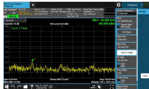
NTNV-DC_5A_n78A-PC2-30-5+20-M+L-QPSK-IDLE-DFT-QPSK-In ner_1RB_Right-0.009-0.15-PASS
