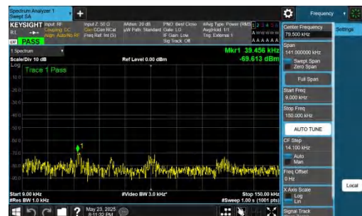
NTNV-DC_5A_n78A-PC2-30-5+10-M+H-QPSK-IDLE-DFT-QPSK-Inner_1RB_Right-0.009-0.15-PASS
