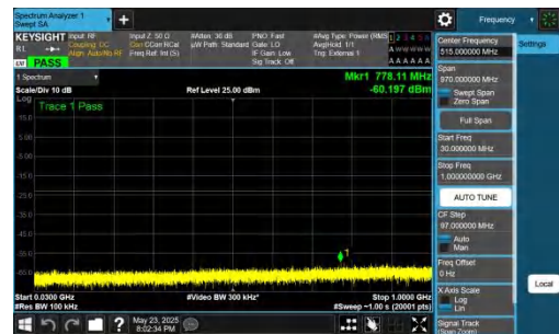
NTNV-DC_5A_n78A-PC2-30-5+10-M+M-QPSK-IDLE-DFT-QPSK-In ner_1RB_Right-30-1000-PASS
