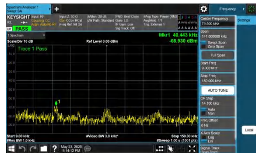
NTNV-DC_5A_n78A-PC2-30-5+25-M+L-QPSK-IDLE-DFT-BPSK-In ner_1RB_Right-0.009-0.15-PASS
