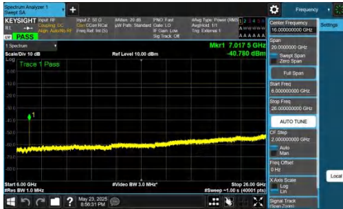
NTNV-DC_5A_n78A-PC2-30-5+20-M+M-QPSK-IDLE-DFT-BPSK-Inner_1RB_Right-6000-26000-PASS
