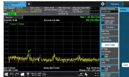
NTNV-DC_5A_n78A-PC2-30-5+15-M+L-QPSK-IDLE-DFT-QPSK-In ner_1RB_Right-0.009-0.15-PASS
