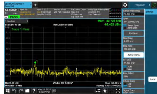
NTVN-DC_5A_n78A-PC2-30-5+15-M+H-QPSK-IDLE-DFT-QPSK-Inner_1RB_Right-0.009-0.15-PASS
