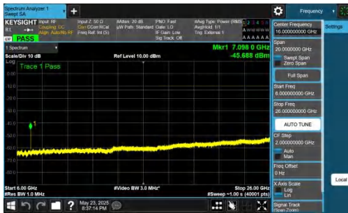
NTNV-DC_5A_n78A-PC2-30-5+15-M+H-QPSK-IDLE-DFT-BPSK-Inner_1RB_Right-6000-26000-PASS
