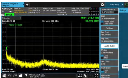
NTNV-DC_5A_n78A-PC2-30-5+15-M+L-QPSK-IDLE-DFT-QPSK-In ner_1RB_Right-0.15-30-PASS
