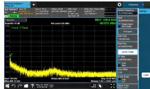
NTNV-DC_5A_n78A-PC2-30-5+15-M+M-QPSK-IDLE-DFT-BPSK-Inner_1RB_Left-0.15-30-PASS
