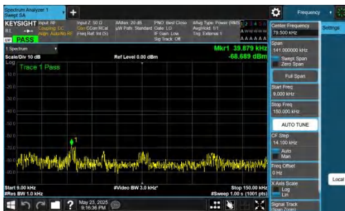
NTNV-DC_5A_n78A-PC2-30-5+25-M+L-QPSK-IDLE-DFT-QPSK-In ner_1RB_Left-0.009-0.15-PASS
