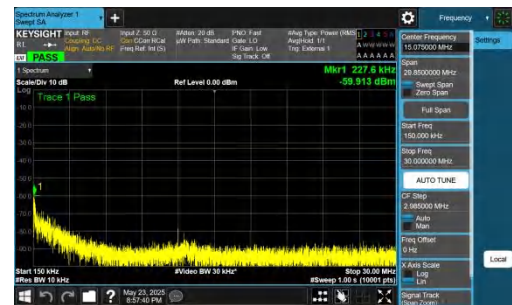
NTNV-DC_5A_n78A-PC2-30-5+20-M+M-QPSK-IDLE-DFT-QPSK-Inner_1RB_Left-0.15-30-PASS
