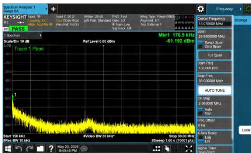
NTVN-DC_5A_n78A-PC2-30-5+15-M+H-QPSK-IDLE-DFT-QPSK-Inner_1RB_Right-0.15-30-PASS
