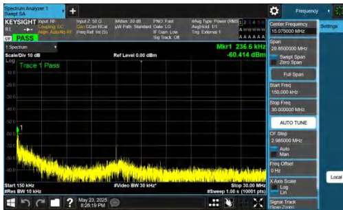
NTNV-DC_5A_n78A-PC2-30-5+15-M+M-QPSK-IDLE-DFT-BPSK-I nner_1RB_Right-0.15-30-PASS
