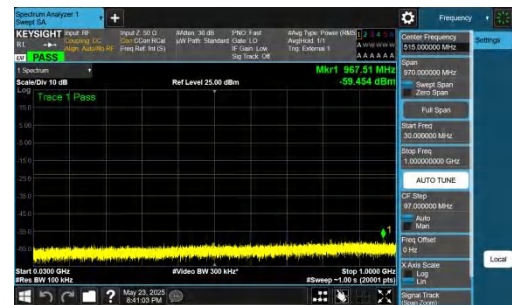
NTVN-DC_5A_n78A-PC2-30-5+15-M+H-QPSK-IDLE-DFT-QPSK-Inner_1RB_Right-30-1000-PASS
