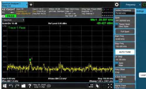
NTNV-DC_5A_n78A-PC2-30-5+20-M+H-QPSK-IDLE-DFT-BPSK-Inner_1RB_Left-0.009-0.15-PASS
