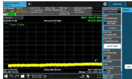
NTNV-DC_5A_n78A-PC2-30-5+10-M+H-QPSK-IDLE-DFT-BPSK-In ner_1RB_Right-30-1000-PASS
