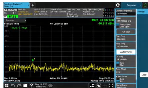
NTVN-DC_5A_n78A-PC2-30-5+20-M+M-QPSK-IDLE-DFT-BPSK-Inner_1RB_Right-0.009-0.15-PASS
