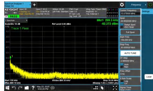
NTNV-DC_5A_n78A-PC2-30-5+20-M+H-QPSK-IDLE-DFT-BPSK-Inner_1RB_Left-0.15-30-PASS
