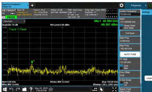
NTVN-DC_5A_n78A-PC2-30-5+10-M+M-QPSK-IDLE-DFT-QPSK-Inner_1RB_Left-0.009-0.15-PASS
