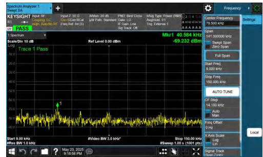
NTNV-DC_5A_n78A-PC2-30-5+25-M+L-QPSK-IDLE-DFT-QPSK-In_ner_1RB_Right-0.009-0.15-PASS
