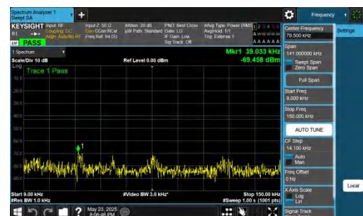
NTNV-DC_5A_n78A-PC2-30-5+10-M+H-QPSK-IDLE-DFT-BPSK-In ner_1RB_Right-0.009-0.15-PASS
