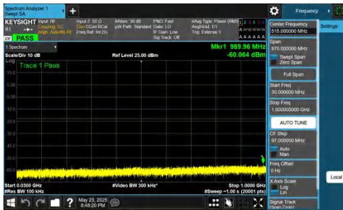
NTNV-DC_5A_n78A-PC2-30-5+20-M+L-QPSK-IDLE-DFT-QPSK-In ner_1RB_Left-30-1000-PASS
