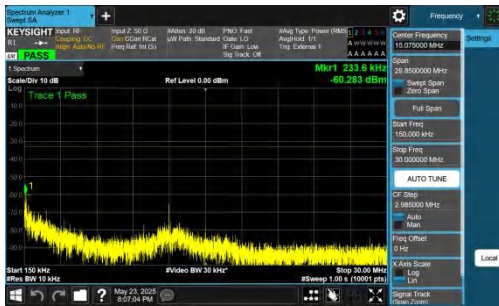
NTNV-DC_5A_n78A-PC2-30-5+10-M+H-QPSK-IDLE-DFT-BPSK-I nner_1RB_Right-0.15-30-PASS
