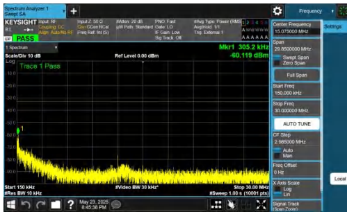
NTNV-DC_5A_n78A-PC2-30-5+20-M+L-QPSK-IDLE-DFT-BPSK-In ner_1RB_Right-0.15-30-PASS
