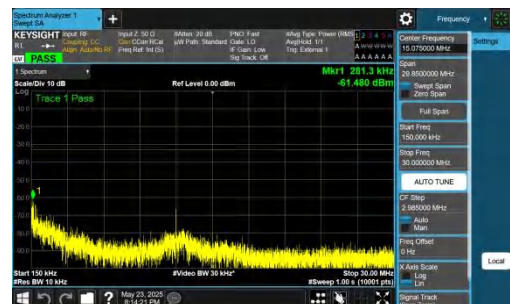
NTNV-DC_5A_n78A-PC2-30-5+15-M+L-QPSK-IDLE-DFT-BPSK-Inner_1RB_Left-0.15-30-PASS
