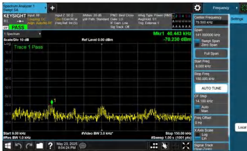
NTNV-DC_5A_n78A-PC2-30-5+10-M+H-QPSK-IDLE-DFT-BPSK-I nner_1RB_Left-0.009-0.15-PASS
