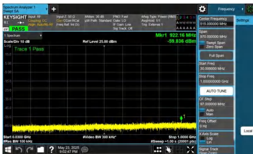
NTNV-DC_5A_n78A-PC2-30-5+20-M+H-QPSK-IDLE-DFT-BPSK-Inner_1RB_Left-30-1000-PASS
