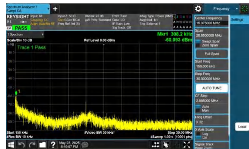
NTNV-DC_5A_n78A-PC2-30-5+15-M+L-QPSK-IDLE-DFT-QPSK-In ner_1RB_Left-0.15-30-PASS
