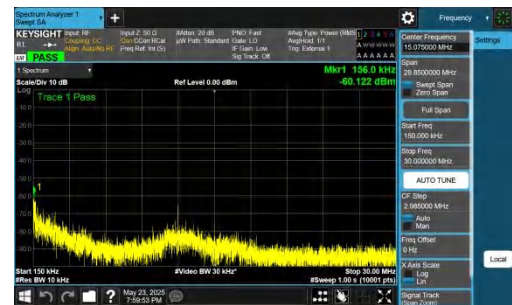
NTVN-DC_5A_n78A-PC2-30-5+10-M+M-QPSK-IDLE-DFT-QPSK-Inner_1RB_Left-0.15-30-PASS
