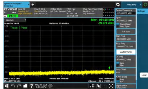
NTNV-DC_5A_n78A-PC2-30-5+20-M+L-QPSK-IDLE-DFT-BPSK-In ner_1RB_Right-30-1000-PASS
