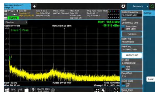
NTNV-DC_5A_n78A-PC2-30-5+10-M+H-QPSK-IDLE-DFT-QPSK-In ner_1RB_Left-0.15-30-PASS
