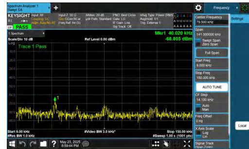
NTNV-DC_5A_n78A-PC2-30-5+20-M+M-QPSK-IDLE-DFT-QPSK-In ner_1RB_Right-0.009-0.15-PASS
