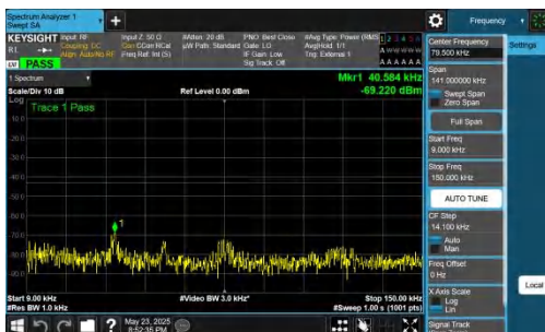
NTNV-DC_5A_n78A-PC2-30-5+20-M+M-QPSK-IDLE-DFT-BPSK-In nner_1RB_Left-0.009-0.15-PASS
