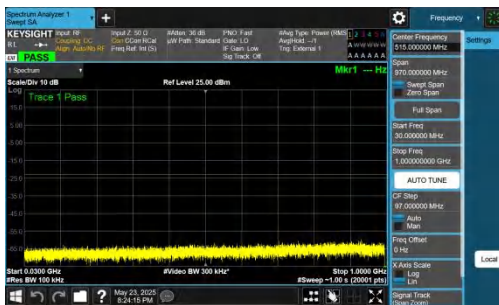
NTNV-DC_5A_n78A-PC2-30-5+15-M+M-QPSK-IDLE-DFT-BPSK-Inner_1RB_Left-30-1000-PASS
