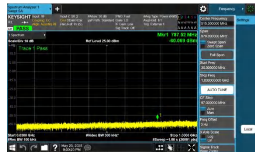
NTNV-DC_5A_n78A-PC2-30-5+20-M+M-QPSK-IDLE-DFT-QPSK-In ner_1RB_Right-30-1000-PASS
