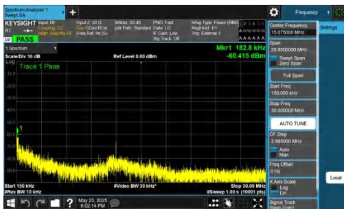
NTNV-DC_5A_n78A-PC2-30-5+10-M+M-QPSK-IDLE-DFT-QPSK-I nner_1RB_Right-0.15-30-PASS
