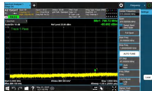
NTNV-DC_5A_n78A-PC2-30-5+15-M+L-QPSK-IDLE-DFT-QPSK-In ner_1RB_Right-30-1000-PASS
