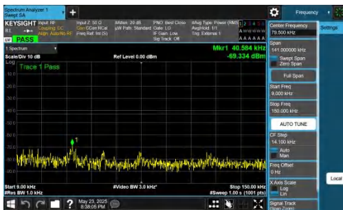
NTNV-DC_5A_n78A-PC2-30-5+15-M+H-QPSK-IDLE-DFT-QPSK-Inner_1RB_Left-0.009-0.15-PASS
