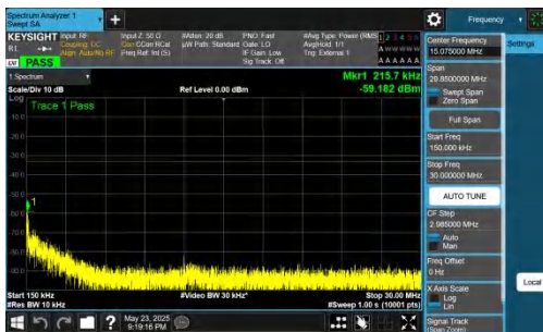
NTNV-DC_5A_n78A-PC2-30-5+25-M+L-QPSK-IDLE-DFT-QPSK-In_ner_1RB_Right-0.15-30-PASS
