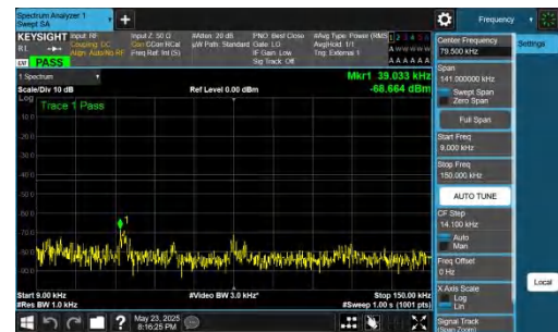
NTNV-DC_5A_n78A-PC2-30-5+15-M+L-QPSK-IDLE-DFT-BPSK-In ner_1RB_Right-0.009-0.15-PASS
