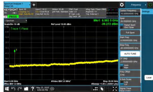
NTVN-DC_5A_n78A-PC2-30-5+20-M+M-QPSK-IDLE-DFT-BPSK-Inner_1RB_Left-6000-26000-PASS
