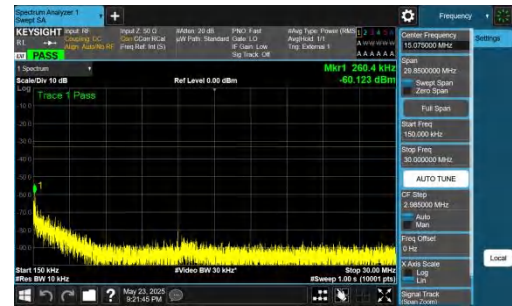
NTNV-DC_5A_n78A-PC2-30-5+25-M+M-QPSK-IDLE-DFT-BPSK-In ner_1RB_Left-0.15-30-PASS
