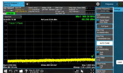
NTNV-DC_5A_n78A-PC2-30-5+25-M+L-QPSK-IDLE-DFT-BPSK-In ner_1RB_Right-30-1000-PASS
