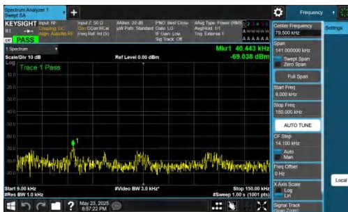
NTNV-DC_5A_n78A-PC2-30-5+20-M+M-QPSK-IDLE-DFT-QPSK-Inner_1RB_Left-0.009-0.15-PASS
