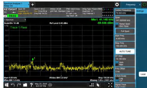
NTNV-DC_5A_n78A-PC2-30-5+10-M+M-QPSK-IDLE-DFT-QPSK-In ner_1RB_Right-0.009-0.15-PASS
