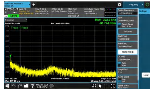
NTNV-DC_5A_n78A-PC2-30-5+10-M+H-QPSK-IDLE-DFT-BPSK-In ner_1RB_Left-0.15-30-PASS
