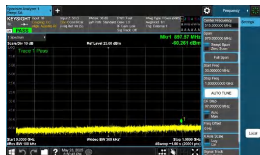
NTNV-DC_5A_n78A-PC2-30-5+20-M+L-QPSK-IDLE-DFT-QPSK-In ner_1RB_Right-30-1000-PASS
