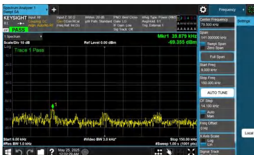
NTNV-DC_5A_n77A-PC2-30-5+80-M+H-QPSK-IDLE-DFT-BPSK-Inner_1RB_Left-0.009-0.15-PASS
