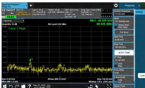
NTNV-DC_5A_n77A-PC2-30-5+90-M+M-QPSK-IDLE-DFT-BPSK-In_ner_1RB_Left-0.009-0.15-PASS
