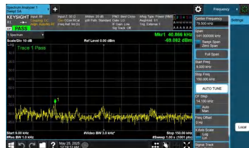
NTNV-DC_5A_n77A-PC2-30-5+90-M+L-QPSK-IDLE-DFT-QPSK-In ner_1RB_Right-0.009-0.15-PASS
