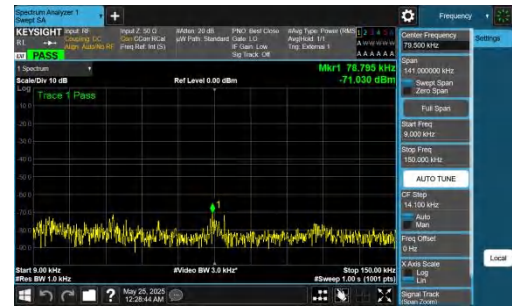
NTNV-DC_5A_n77A-PC2-30-5+90-M+M-QPSK-IDLE-DFT-QPSK-In ner_1RB_Right-0.009-0.15-PASS
