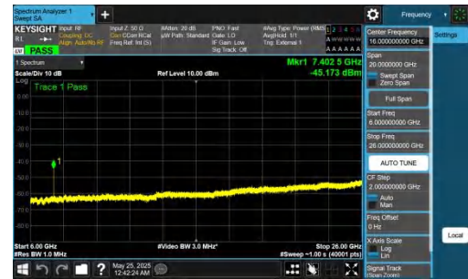
NTNV-DC_5A_n77A-PC2-30-5+100-M+L-QPSK-IDLE-DFT-BPSK-I nner_1RB_Left-6000-26000-PASS
