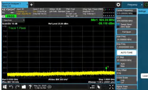
NTNV-DC_5A_n77A-PC2-30-5+80-M+M-QPSK-IDLE-DFT-QPSK-I nner_1RB_Left-30-1000-PASS
