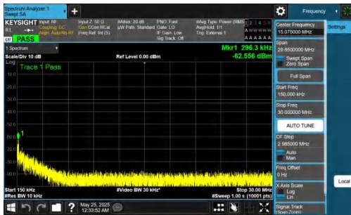
NTNV-DC_5A_n77A-PC2-30-5+90-M+H-QPSK-IDLE-DFT-BPSK-In nner_1RB_Right-0.15-30-PASS
