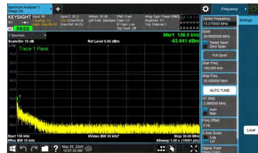
NTNV-DC_5A_n77A-PC2-30-5+80-M+H-QPSK-IDLE-DFT-QPSK-Inner_1RB_Left-0.15-30-PASS
