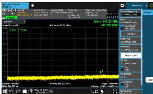
NTNV-DC_5A_n77A-PC2-30-5+90-M+H-QPSK-IDLE-DFT-BPSK-Inner_1RB_Left-30-1000-PASS
