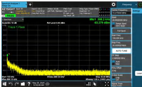
NTNV-DC_5A_n77A-PC2-30-5+100-M+M-QPSK-IDLE-DFT-BPSK- Inner_1RB_Right-0.15-30-PASS
