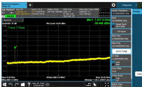
NTNV-DC_5A_n77A-PC2-30-5+90-M+L-QPSK-IDLE-DFT-QPSK-In_ner_1RB_Right-6000-26000-PASS
