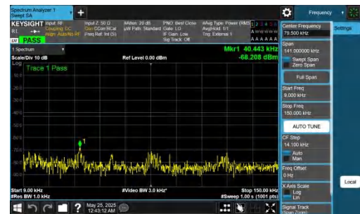
NTNV-DC_5A_n77A-PC2-30-5+100-M+L-QPSK-IDLE-DFT-BPSK-I nner_1RB_Right-0.009-0.15-PASS
