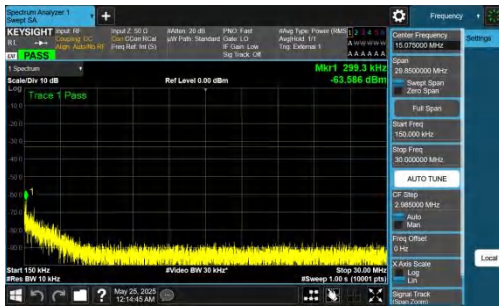
NTNV-DC_5A_n77A-PC2-30-5+90-M+L-QPSK-IDLE-DFT-BPSK-In ner_1RB_Right-0.15-30-PASS
