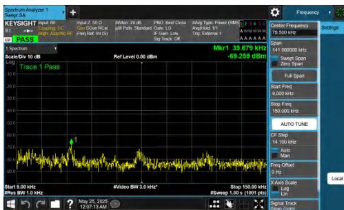
NTNV-DC_5A_n77A-PC2-30-5+80-M+H-QPSK-IDLE-DFT-QPSK-Inner_1RB_Left-0.009-0.15-PASS
