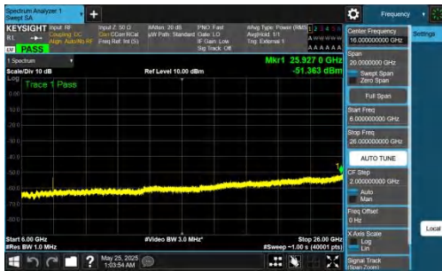
NTNV-DC_5A_n77A-PC2-30-5+100-M+H-QPSK-IDLE-DFT-BPSK- Inner_1RB_Right-6000-26000-PASS
