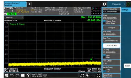
NTNV-DC_5A_n77A-PC2-30-5+90-M+H-QPSK-IDLE-DFT-BPSK-In ner_1RB_Right-30-1000-PASS
