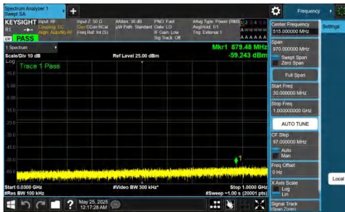
NTNV-DC_5A_n77A-PC2-30-5+90-M+L-QPSK-IDLE-DFT-QPSK-In ner_1RB_Left-30-1000-PASS
