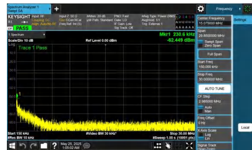
NTNV-DC_5A_n77A-PC2-30-5+100-M+H-QPSK-IDLE-DFT-QPSK-I nner_1RB_Left-0.15-30-PASS
