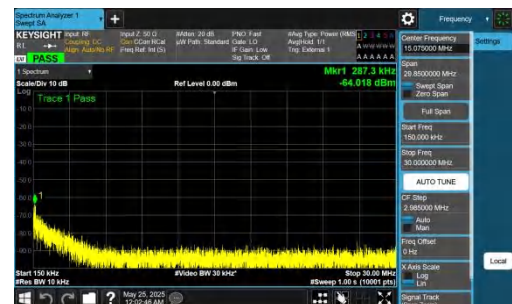
NTNV-DC_5A_n77A-PC2-30-5+80-M+H-QPSK-IDLE-DFT-BPSK-Inner_1RB_Left-0.15-30-PASS
