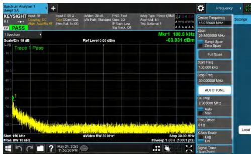
NTNV-DC_5A_n77A-PC2-30-5+80-M+M-QPSK-IDLE-DFT-BPSK-I nner_1RB_Right-0.15-30-PASS
