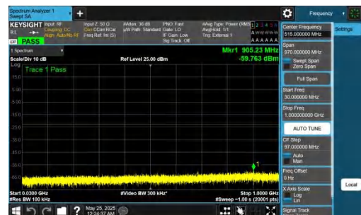
NTNV-DC_5A_n77A-PC2-30-5+90-M+M-QPSK-IDLE-DFT-BPSK-In ner_1RB_Right-30-1000-PASS
