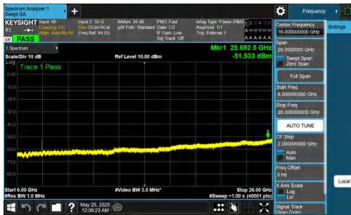
NTNV-DC_5A_n77A-PC2-30-5+80-M+H-QPSK-IDLE-DFT-BPSK-Inner_1RB_Right-6000-26000-PASS
