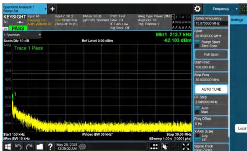
NTNV-DC_5A_n77A-PC2-30-5+90-M+M-QPSK-IDLE-DFT-QPSK-I nner_1RB_Right-0.15-30-PASS
