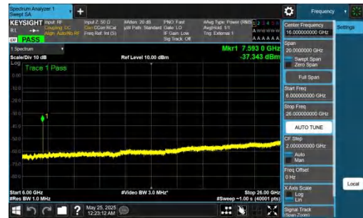
NTNV-DC_5A_n77A-PC2-30-5+90-M+M-QPSK-IDLE-DFT-BPSK-In ner_1RB_Left-6000-26000-PASS
