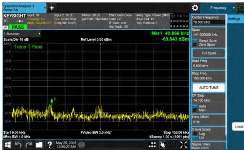
NTNV-DC_5A_n77A-PC2-30-5+100-M+M-QPSK-IDLE-DFT-BPSK- Inner_1RB_Left-0.009-0.15-PASS
