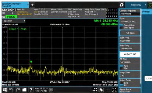
NTNV-DC_5A_n77A-PC2-30-5+90-M+H-QPSK-IDLE-DFT-BPSK-Inner_1RB_Left-0.009-0.15-PASS
