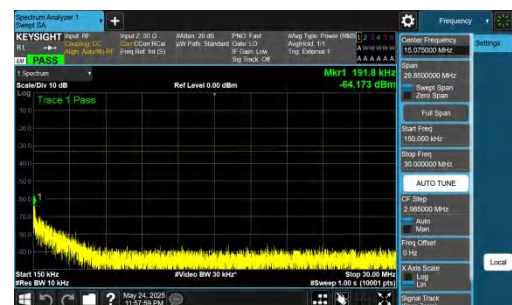
NTNV-DC_5A_n77A-PC2-30-5+80-M+M-QPSK-IDLE-DFT-QPSK-In ner_1RB_Left-0.15-30-PASS
