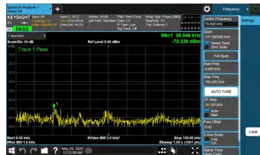
NTNV-DC_5A_n77A-PC2-30-5+90-M+M-QPSK-IDLE-DFT-BPSK-In ner_1RB_Right-0.009-0.15-PASS
