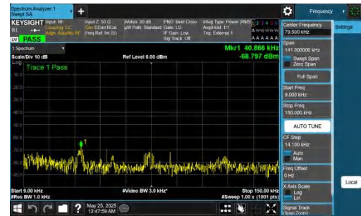
NTNV-DC_5A_n77A-PC2-30-5+100-M+L-QPSK-IDLE-DFT-QPSK-I nner_1RB_Right-0.009-0.15-PASS
