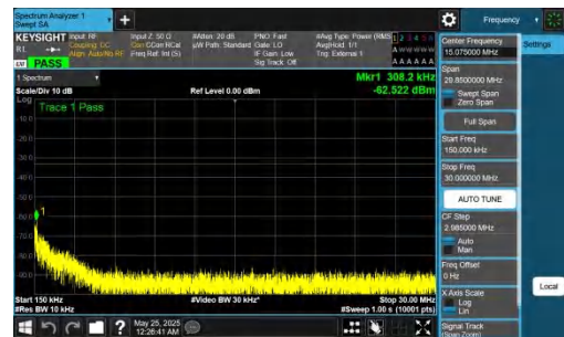
NTNV-DC_5A_n77A-PC2-30-5+90-M+M-QPSK-IDLE-DFT-QPSK-Inner_1RB_Left-0.15-30-PASS
