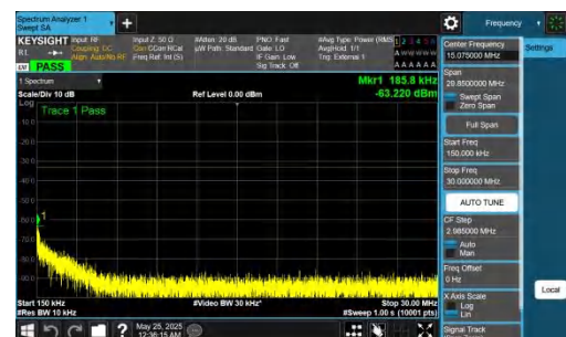
NTNV-DC_5A_n77A-PC2-30-5+90-M+H-QPSK-IDLE-DFT-QPSK-In ner_1RB_Left-0.15-30-PASS
