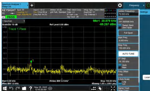
NTNV-DC_5A_n77A-PC2-30-5+100-M+L-QPSK-IDLE-DFT-QPSK-I nner_1RB_Left-0.009-0.15-PASS
