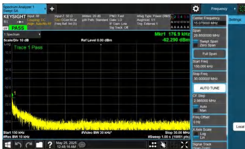
NTNV-DC_5A_n77A-PC2-30-5+100-M+L-QPSK-IDLE-DFT-QPSK-I nner_1RB_Right-0.15-30-PASS
