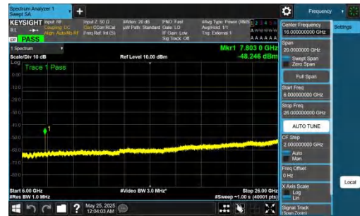
NTNV-DC_5A_n77A-PC2-30-5+80-M+H-QPSK-IDLE-DFT-BPSK-In ner_1RB_Left-6000-26000-PASS
