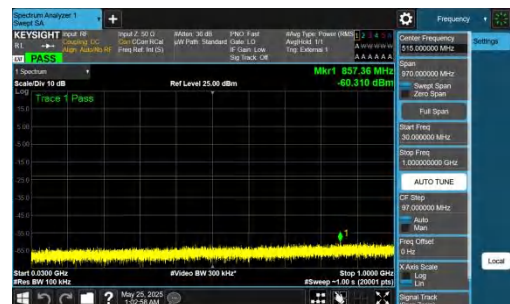
NTNV-DC_5A_n77A-PC2-30-5+100-M+H-QPSK-IDLE-DFT-BPSK-I nner_1RB_Right-30-1000-PASS
