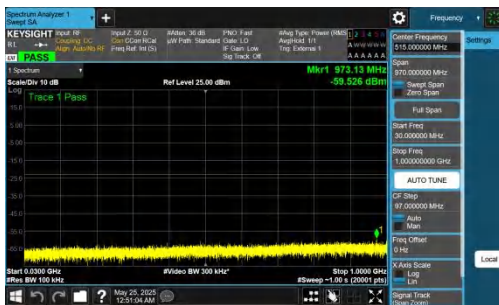
NTNV-DC_5A_n77A-PC2-30-5+100-M+M-QPSK-IDLE-DFT-BPSK- Inner_1RB_Left-30-1000-PASS
