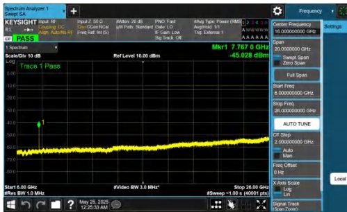
NTNV-DC_5A_n77A-PC2-30-5+90-M+M-QPSK-IDLE-DFT-BPSK-Inner_1RB_Right-6000-26000-PASS
