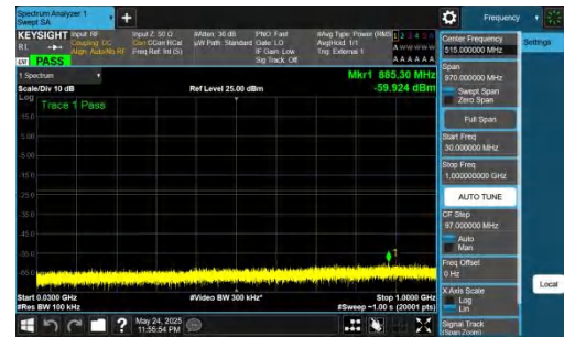
NTNV-DC_5A_n77A-PC2-30-5+80-M+M-QPSK-IDLE-DFT-BPSK-In ner_1RB_Right-30-1000-PASS
