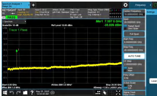
NTNV-DC_5A_n77A-PC2-30-5+100-M+L-QPSK-IDLE-DFT-BPSK-I nner_1RB_Right-6000-26000-PASS
