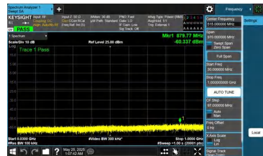
NTNV-DC_5A_n77A-PC2-30-5+100-M+H-QPSK-IDLE-DFT-QPSK-I-nner_1RB_Right-30-1000-PASS
