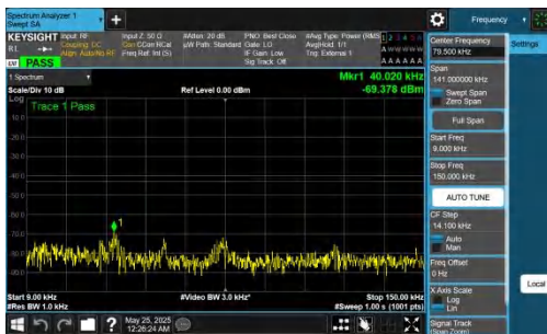
NTNV-DC_5A_n77A-PC2-30-5+90-M+M-QPSK-IDLE-DFT-QPSK-Inner_1RB_Left-0.009-0.15-PASS
