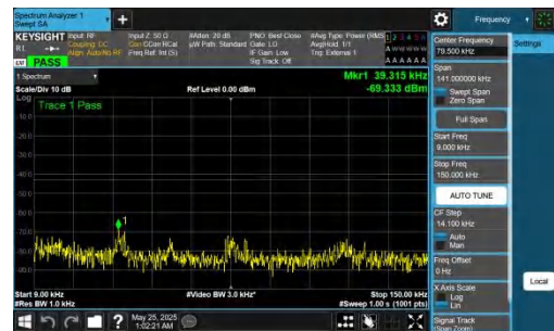
NTNV-DC_5A_n77A-PC2-30-5+100-M+H-QPSK-IDLE-DFT-BPSK-I nner_1RB_Right-0.009-0.15-PASS
