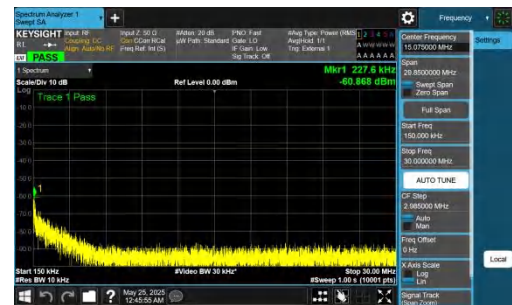
NTNV-DC_5A_n77A-PC2-30-5+100-M+L-QPSK-IDLE-DFT-QPSK-I nner_1RB_Left-0.15-30-PASS
