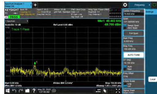
NTNV-DC_5A_n77A-PC2-30-5+100-M+H-QPSK-IDLE-DFT-QPSK-I-nner_1RB_Right-0.009-0.15-PASS
