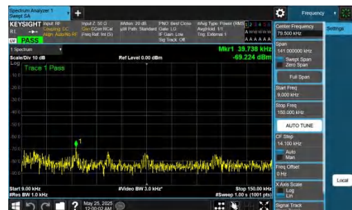
NTNV-DC_5A_n77A-PC2-30-5+80-M+M-QPSK-IDLE-DFT-QPSK-In ner_1RB_Right-0.009-0.15-PASS
