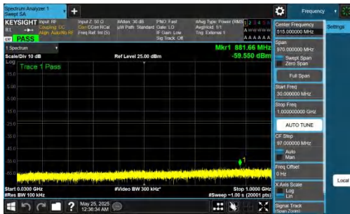
NTNV-DC_5A_n77A-PC2-30-5+90-M+H-QPSK-IDLE-DFT-QPSK-Inner_1RB_Left-30-1000-PASS
