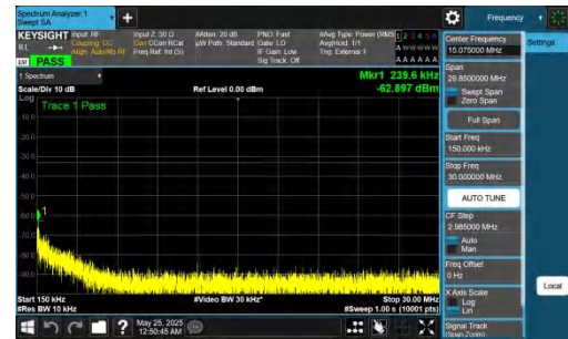
NTNV-DC_5A_n77A-PC2-30-5+100-M+M-QPSK-IDLE-DFT-BPSK-I nner_1RB_Left-0.15-30-PASS
