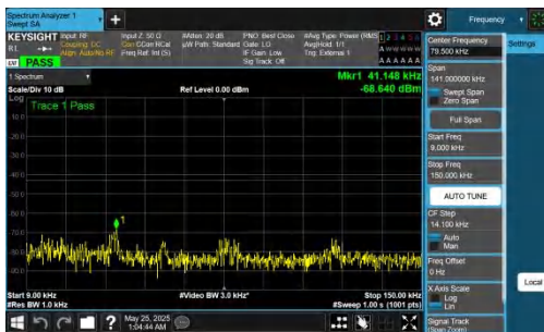
NTNV-DC_5A_n77A-PC2-30-5+100-M+H-QPSK-IDLE-DFT-QPSK- Inner_1RB_Left-0.009-0.15-PASS
