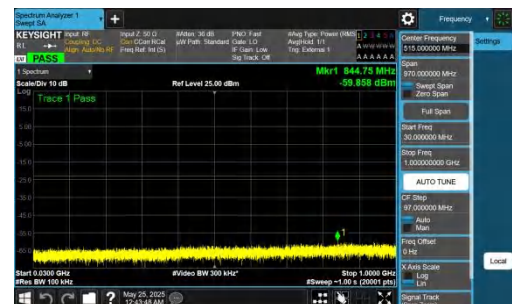
NTNV-DC_5A_n77A-PC2-30-5+100-M+L-QPSK-IDLE-DFT-BPSK-I nner_1RB_Right-30-1000-PASS
