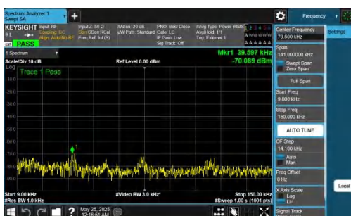
NTNV-DC_5A_n77A-PC2-30-5+90-M+L-QPSK-IDLE-DFT-QPSK-In ner_1RB_Left-0.009-0.15-PASS
