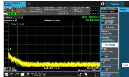
NTNV-DC_5A_n77A-PC2-30-5+90-M+L-QPSK-IDLE-DFT-BPSK-In ner_1RB_Left-0.15-30-PASS
