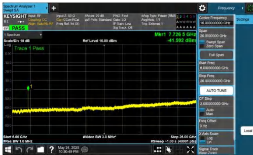
NTVN-DC_5A_n77A-PC2-30-5+50-M+M-QPSK-IDLE-DFT-BPSK-Inner_1RB_Right-6000-26000-PASS
