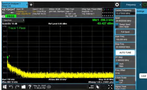
NTNV-DC_5A_n77A-PC2-30-5+70-M+H-QPSK-IDLE-DFT-BPSK-In nner_1RB_Right-0.15-30-PASS
