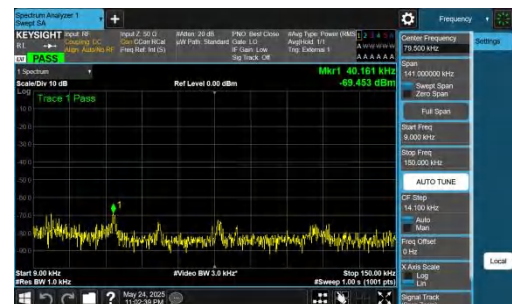
NTNV-DC_5A_n77A-PC2-30-5+60-M+M-QPSK-IDLE-DFT-QPSK-In ner_1RB_Right-0.009-0.15-PASS
