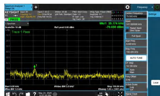
NTNV-DC_5A_n77A-PC2-30-5+60-M+M-QPSK-IDLE-DFT-BPSK-In ner_1RB_Right-0.009-0.15-PASS
