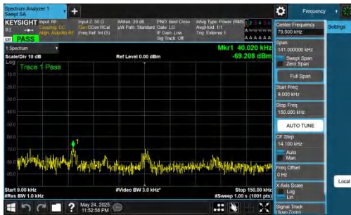
NTNV-DC_5A_n77A-PC2-30-5+80-M+M-QPSK-IDLE-DFT-BPSK-In nner_1RB_Left-0.009-0.15-PASS
