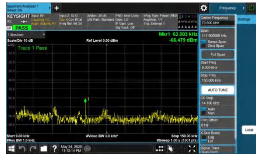
NTNV-DC_5A_n77A-PC2-30-5+60-M+H-QPSK-IDLE-DFT-QPSK-Inner_1RB_Right-0.009-0.15-PASS
