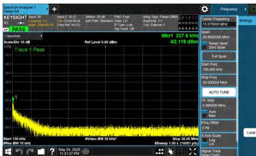
NTNV-DC_5A_n77A-PC2-30-5+70-M+M-QPSK-IDLE-DFT-QPSK-I nner_1RB_Right-0.15-30-PASS
