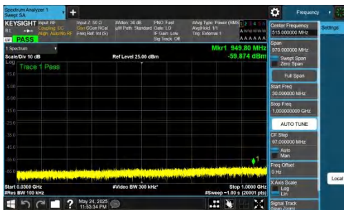
NTNV-DC_5A_n77A-PC2-30-5+80-M+M-QPSK-IDLE-DFT-BPSK-In nner_1RB_Left-30-1000-PASS
