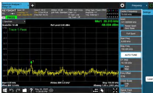
NTNV-DC_5A_n77A-PC2-30-5+70-M+M-QPSK-IDLE-DFT-QPSK-Inner_1RB_Left-0.009-0.15-PASS
