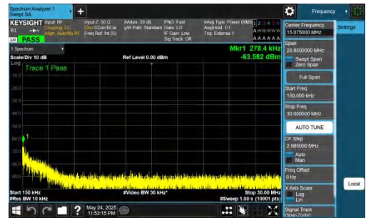
NTNV-DC_5A_n77A-PC2-30-5+80-M+M-QPSK-IDLE-DFT-BPSK-In ner_1RB_Left-0.15-30-PASS
