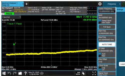
NTNV-DC_5A_n77A-PC2-30-5+70-M+M-QPSK-IDLE-DFT-BPSK-Inner_1RB_Right-6000-26000-PASS
