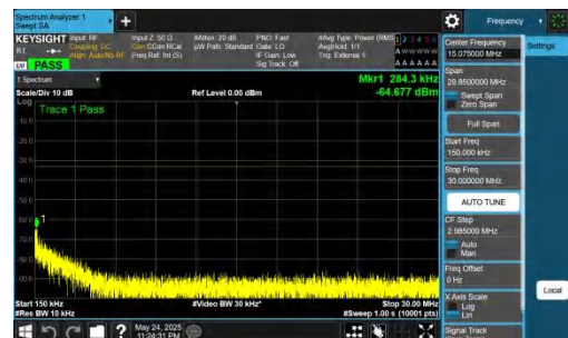
NTNV-DC_5A_n77A-PC2-30-5+70-M+M-QPSK-IDLE-DFT-BPSK-In ner_1RB_Left-0.15-30-PASS
