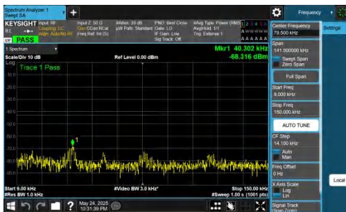
NTVN-DC_5A_n77A-PC2-30-5+50-M+M-QPSK-IDLE-DFT-QPSK-Inner_1RB_Left-0.009-0.15-PASS
