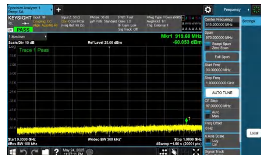
NTNV-DC_5A_n77A-PC2-30-5+70-M+M-QPSK-IDLE-DFT-BPSK-In ner_1RB_Right-30-1000-PASS
