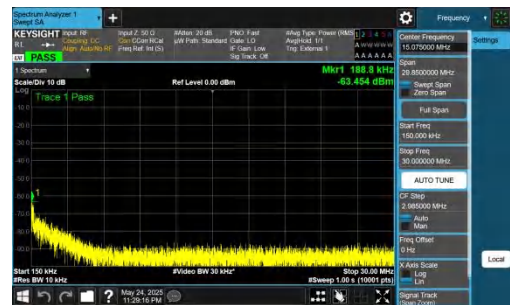
NTNV-DC_5A_n77A-PC2-30-5+70-M+M-QPSK-IDLE-DFT-QPSK-Inner_1RB_Left-0.15-30-PASS
