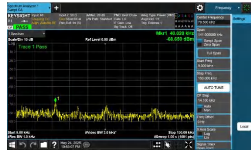
NTNV-DC_5A_n77A-PC2-30-5+60-M+L-QPSK-IDLE-DFT-QPSK-In_ner_1RB_Right-0.009-0.15-PASS
