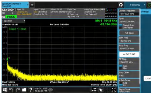
NTNV-DC_5A_n77A-PC2-30-5+50-M+H-QPSK-IDLE-DFT-BPSK-Inner_1RB_Right-0.15-30-PASS
