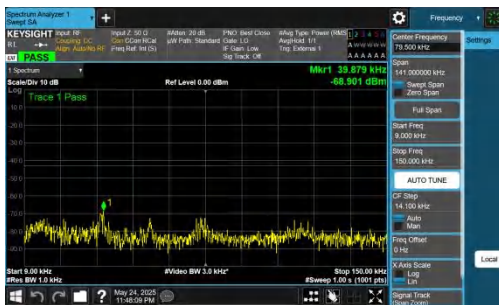
NTNV-DC_5A_n77A-PC2-30-5+80-M+L-QPSK-IDLE-DFT-QPSK-In ner_1RB_Left-0.009-0.15-PASS
