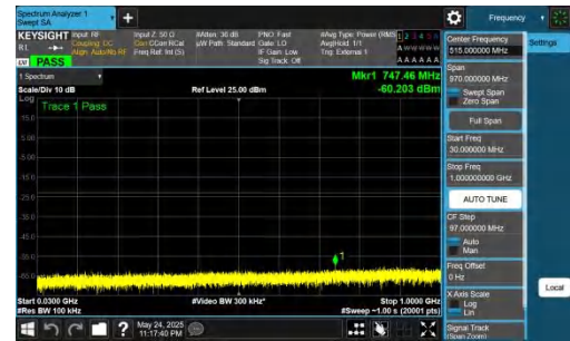
NTNV-DC_5A_n77A-PC2-30-5+70-M+L-QPSK-IDLE-DFT-BPSK-In ner_1RB_Right-30-1000-PASS
