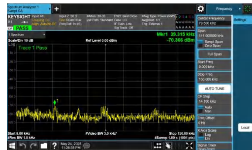
NTNV-DC_5A_n77A-PC2-30-5+70-M+M-QPSK-IDLE-DFT-BPSK-In ner_1RB_Right-0.009-0.15-PASS
