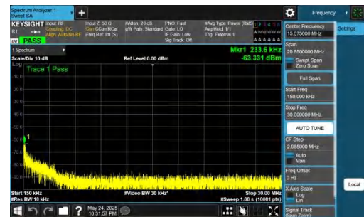
NTVN-DC_5A_n77A-PC2-30-5+50-M+M-QPSK-IDLE-DFT-QPSK-Inner_1RB_Left-0.15-30-PASS
