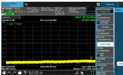
NTNV-DC_5A_n77A-PC2-30-5+60-M+M-QPSK-IDLE-DFT-BPSK-In nner_1RB_Left-30-1000-PASS
