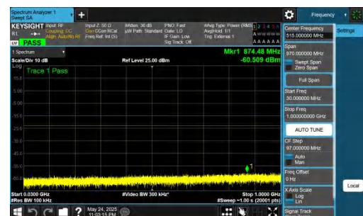
NTNV-DC_5A_n77A-PC2-30-5+60-M+M-QPSK-IDLE-DFT-QPSK-In ner_1RB_Right-30-1000-PASS
