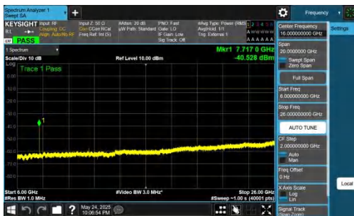
NTNV-DC_5A_n77A-PC2-30-5+40-M+M-QPSK-IDLE-DFT-QPSK-Inner_1RB_Right-6000-26000-PASS
