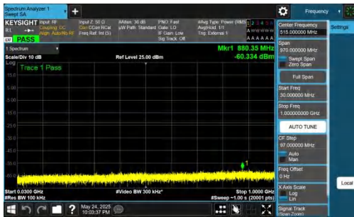
NTNV-DC_5A_n77A-PC2-30-5+40-M+M-QPSK-IDLE-DFT-QPSK-I nner_1RB_Left-30-1000-PASS
