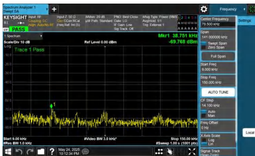
NTNV-DC_5A_n77A-PC2-30-5+40-M+H-QPSK-IDLE-DFT-QPSK-Inner_1RB_Left-0.009-0.15-PASS
