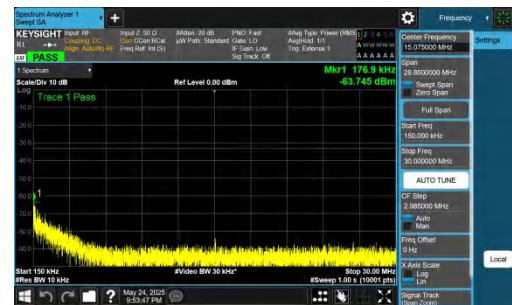
NTNV-DC_5A_n77A-PC2-30-5+40-M+L-QPSK-IDLE-DFT-QPSK-In ner_1RB_Left-0.15-30-PASS
