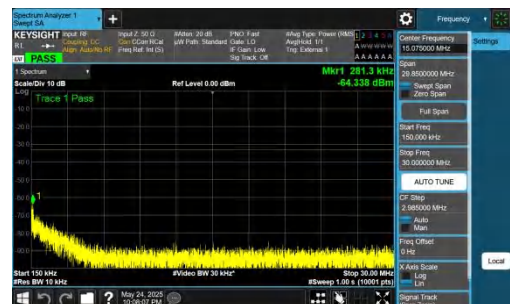
NTNV-DC_5A_n77A-PC2-30-5+40-M+H-QPSK-IDLE-DFT-BPSK-Inner_1RB_Left-0.15-30-PASS
