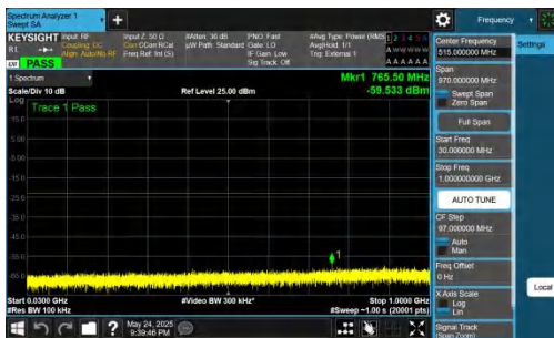
NTNV-DC_5A_n77A-PC2-30-5+30-M+H-QPSK-IDLE-DFT-BPSK-I nner_1RB_Left-30-1000-PASS
