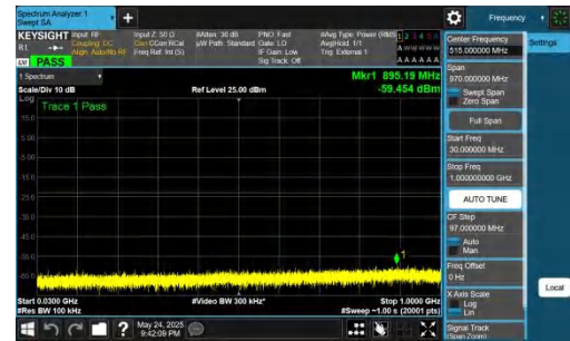
NTNV-DC_5A_n77A-PC2-30-5+30-M+H-QPSK-IDLE-DFT-BPSK-Inner_1RB_Right-30-1000-PASS
