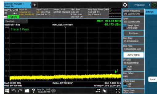
NTNV-DC_5A_n77A-PC2-30-5+50-M+L-QPSK-IDLE-DFT-BPSK-In ner_1RB_Right-30-1000-PASS
