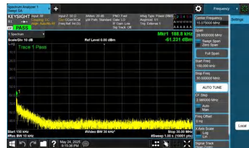
NTNV-DC_5A_n77A-PC2-30-5+25-M+H-QPSK-IDLE-DFT-QPSK-Inner_1RB_Left-0.15-30-PASS
