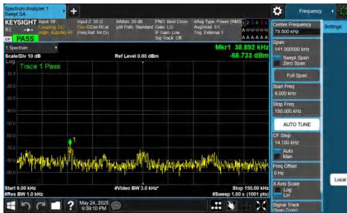
NTNV-DC_5A_n77A-PC2-30-5+30-M+H-QPSK-IDLE-DFT-BPSK-I nner_1RB_Left-0.009-0.15-PASS
