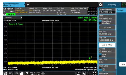
NTNV-DC_5A_n77A-PC2-30-5+40-M+L-QPSK-IDLE-DFT-BPSK-In ner_1RB_Right-30-1000-PASS
