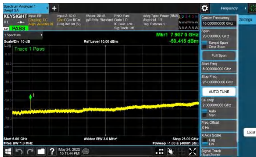
NTNV-DC_5A_n77A-PC2-30-5+40-M+H-QPSK-IDLE-DFT-BPSK-Inner_1RB_Right-6000-26000-PASS
