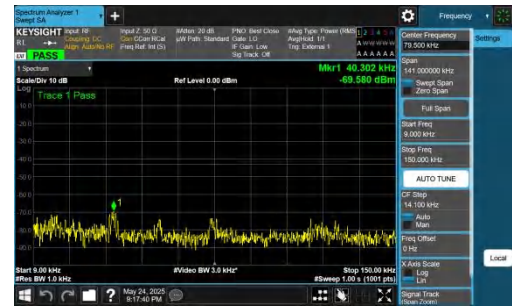
NTNV-DC_5A_n77A-PC2-30-5+25-M+H-QPSK-IDLE-DFT-QPSK-Inner_1RB_Right-0.009-0.15-PASS
