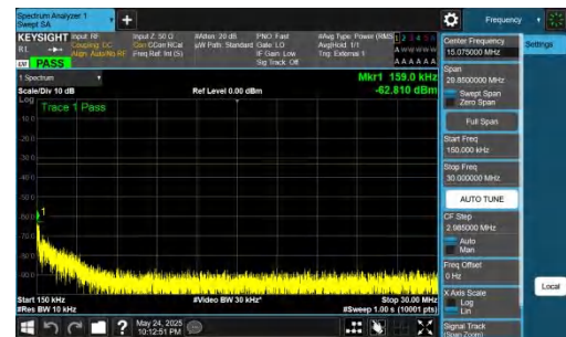
NTNV-DC_5A_n77A-PC2-30-5+40-M+H-QPSK-IDLE-DFT-QPSK-Inner_1RB_Left-0.15-30-PASS
