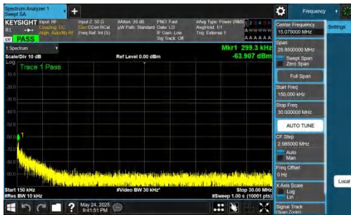
NTNV-DC_5A_n77A-PC2-30-5+30-M+H-QPSK-IDLE-DFT-BPSK-Inner_1RB_Right-0.15-30-PASS
