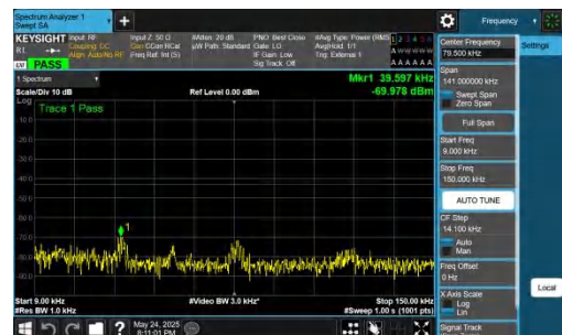
NTNV-DC_5A_n77A-PC2-30-5+15-M+M-QPSK-IDLE-DFT-QPSK-In ner_1RB_Right-0.009-0.15-PASS
