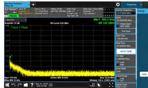
NTNV-DC_5A_n77A-PC2-30-5+15-M+M-QPSK-IDLE-DFT-BPSK-In ner_1RB_Left-0.15-30-PASS
