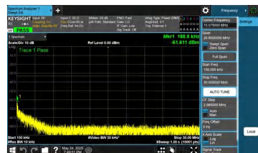
NTNV-DC_5A_n77A-PC2-30-5+10-M+H-QPSK-IDLE-DFT-QPSK-In ner_1RB_Left-0.15-30-PASS
