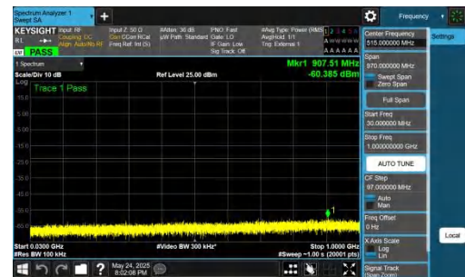
NTNV-DC_5A_n77A-PC2-30-5+15-M+L-QPSK-IDLE-DFT-QPSK-In_ner_1RB_Right-30-1000-PASS
