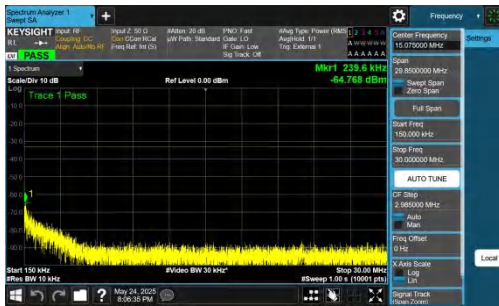
NTNV-DC_5A_n77A-PC2-30-5+15-M+M-QPSK-IDLE-DFT-BPSK-I nner_1RB_Right-0.15-30-PASS
