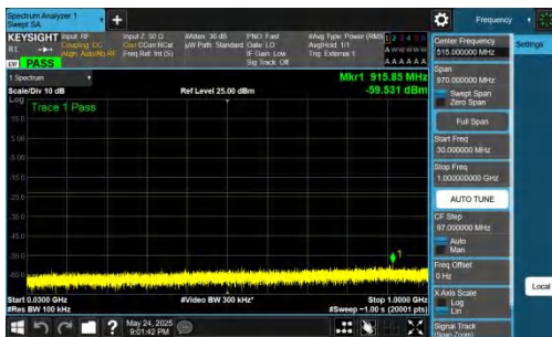
NTNV-DC_5A_n77A-PC2-30-5+25-M+M-QPSK-IDLE-DFT-BPSK-Inner_1RB_Left-30-1000-PASS
