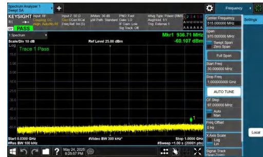
NTNV-DC_5A_n77A-PC2-30-5+20-M+L-QPSK-IDLE-DFT-BPSK-In ner_1RB_Right-30-1000-PASS
