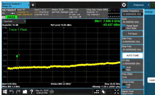
NTVN-DC_5A_n77A-PC2-30-5+20-M+M-QPSK-IDLE-DFT-BPSK-Inner_1RB_Right-6000-26000-PASS
