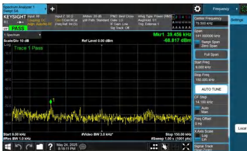
NTNV-DC_5A_n77A-PC2-30-5+15-M+H-QPSK-IDLE-DFT-QPSK-Inner_1RB_Left-0.009-0.15-PASS
