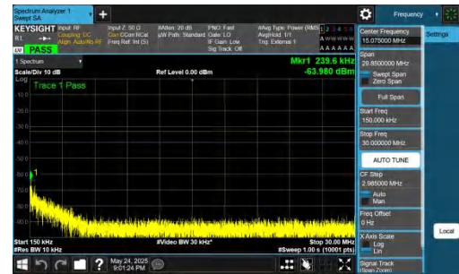
NTNV-DC_5A_n77A-PC2-30-5+25-M+M-QPSK-IDLE-DFT-BPSK-Inner_1RB_Left-0.15-30-PASS
