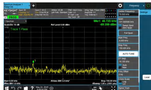
NTNV-DC_5A_n77A-PC2-30-5+20-M+H-QPSK-IDLE-DFT-QPSK-In ner_1RB_Right-0.009-0.15-PASS
