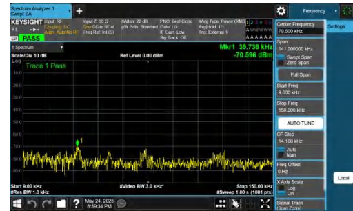
NTNV-DC_5A_n77A-PC2-30-5+20-M+M-QPSK-IDLE-DFT-QPSK-In ner_1RB_Right-0.009-0.15-PASS
