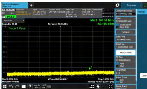
NTNV-DC_5A_n77A-PC2-30-5+15-M+M-QPSK-IDLE-DFT-BPSK-I nner_1RB_Left-30-1000-PASS
