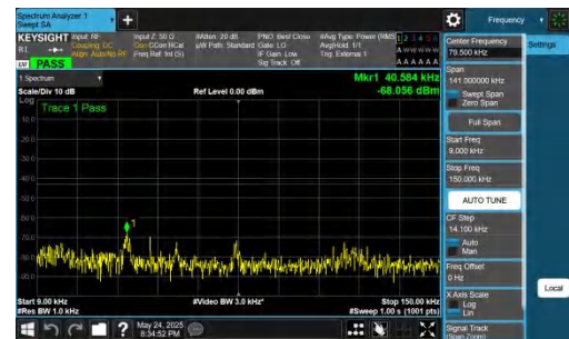
NTVN-DC_5A_n77A-PC2-30-5+20-M+M-QPSK-IDLE-DFT-BPSK-Inner_1RB_Right-0.009-0.15-PASS
