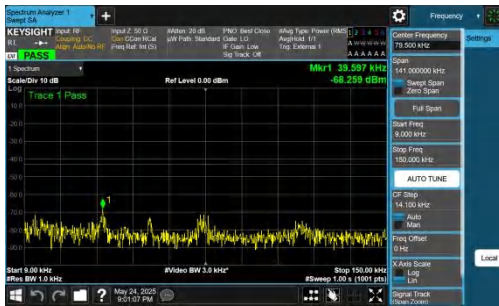
NTNV-DC_5A_n77A-PC2-30-5+25-M+M-QPSK-IDLE-DFT-BPSK-Inner_1RB_Left-0.009-0.15-PASS
