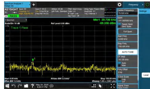
NTNV-DC_5A_n77A-PC2-30-5+15-M+H-QPSK-IDLE-DFT-QPSK-Inner_1RB_Right-0.009-0.15-PASS
