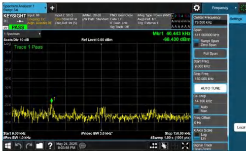
NTNV-DC_5A_n77A-PC2-30-5+15-M+M-QPSK-IDLE-DFT-BPSK-I nner_1RB_Left-0.009-0.15-PASS
