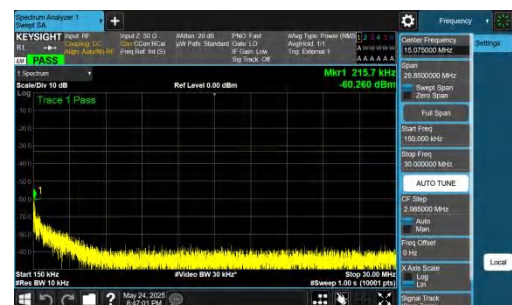
NTNV-DC_5A_n77A-PC2-30-5+20-M+H-QPSK-IDLE-DFT-QPSK-In ner_1RB_Left-0.15-30-PASS
