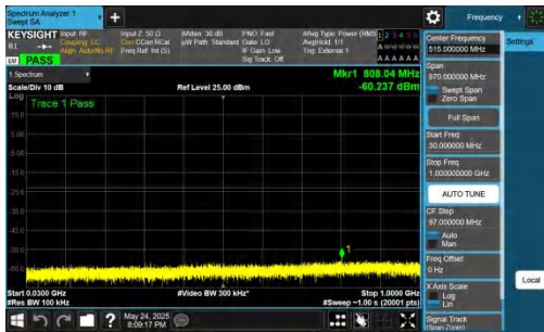
NTNV-DC_5A_n77A-PC2-30-5+15-M+M-QPSK-IDLE-DFT-QPSK-I nner_1RB_Left-30-1000-PASS
