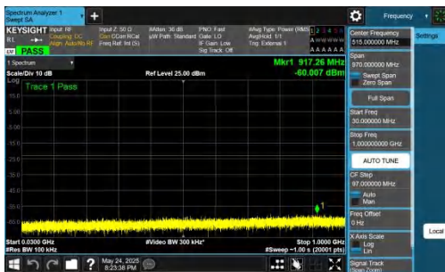
NTNV-DC_5A_n77A-PC2-30-5+20-M+L-QPSK-IDLE-DFT-BPSK-In ner_1RB_Left-30-1000-PASS
