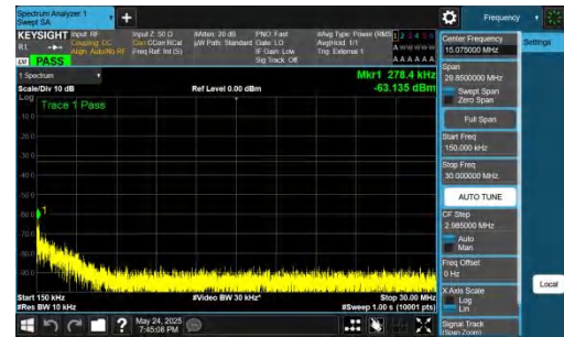
NTNV-DC_5A_n77A-PC2-30-5+10-M+H-QPSK-IDLE-DFT-BPSK-Inner_1RB_Left-0.15-30-PASS
