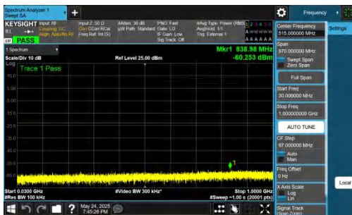
NTNV-DC_5A_n77A-PC2-30-5+10-M+H-QPSK-IDLE-DFT-BPSK-Inner_1RB_Left-30-1000-PASS
