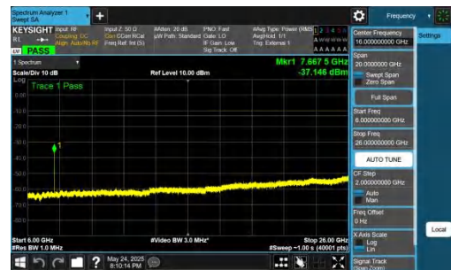
NTNV-DC_5A_n77A-PC2-30-5+15-M+M-QPSK-IDLE-DFT-QPSK-In ner_1RB_Left-6000-26000-PASS
