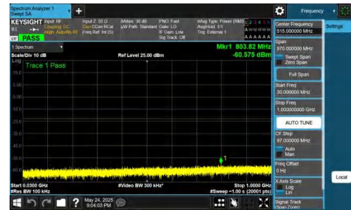
NTNV-DC_5A_n77A-PC2-30-5+25-M+M-QPSK-IDLE-DFT-BPSK-In ner_1RB_Right-30-1000-PASS
