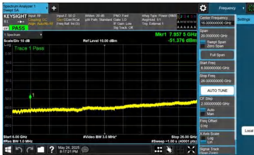
NTNV-DC_5A_n77A-PC2-30-5+15-M+H-QPSK-IDLE-DFT-BPSK-Inner_1RB_Right-6000-26000-PASS
