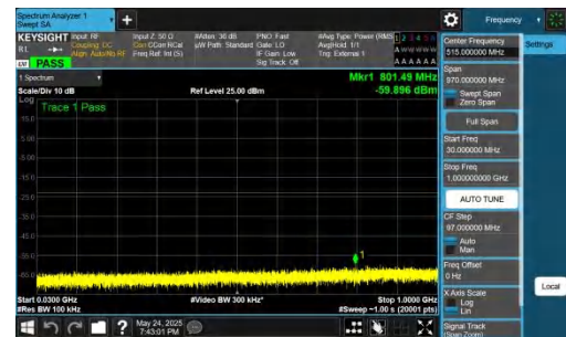
NTNV-DC_5A_n77A-PC2-30-5+10-M+M-QPSK-IDLE-DFT-QPSK-In ner_1RB_Right-30-1000-PASS
