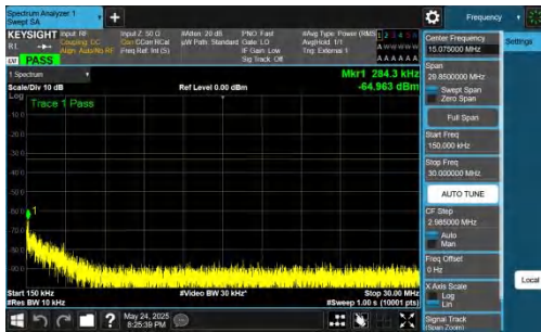
NTNV-DC_5A_n77A-PC2-30-5+20-M+L-QPSK-IDLE-DFT-BPSK-In ner_1RB_Right-0.15-30-PASS
