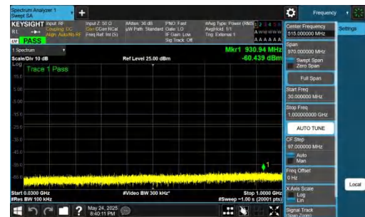
NTNV-DC_5A_n77A-PC2-30-5+20-M+M-QPSK-IDLE-DFT-QPSK-In ner_1RB_Right-30-1000-PASS
