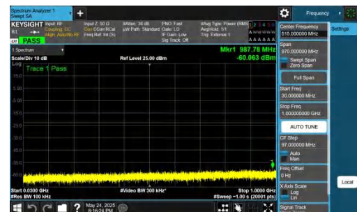
NTNV-DC_5A_n77A-PC2-30-5+15-M+H-QPSK-IDLE-DFT-BPSK-In ner_1RB_Right-30-1000-PASS
