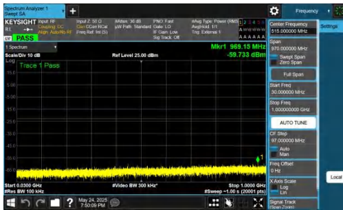
NTNV-DC_5A_n77A-PC2-30-5+10-M+H-QPSK-IDLE-DFT-QPSK-I nner_1RB_Left-30-1000-PASS
