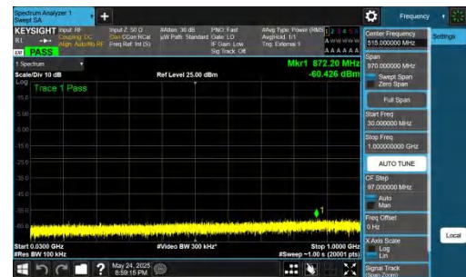
NTNV-DC_5A_n77A-PC2-30-5+25-M+L-QPSK-IDLE-DFT-QPSK-In ner_1RB_Right-30-1000-PASS
