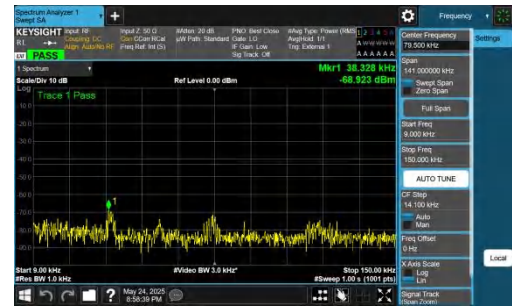
NTNV-DC_5A_n77A-PC2-30-5+25-M+L-QPSK-IDLE-DFT-QPSK-In ner_1RB_Right-0.009-0.15-PASS
