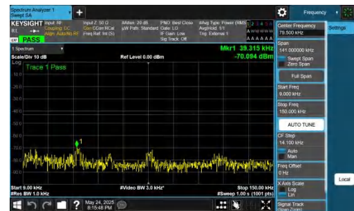
NTNV-DC_5A_n77A-PC2-30-5+15-M+H-QPSK-IDLE-DFT-BPSK-In ner_1RB_Right-0.009-0.15-PASS
