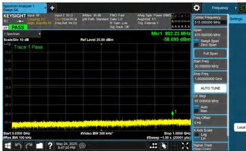
NTNV-DC_5A_n77A-PC2-30-5+20-M+H-QPSK-IDLE-DFT-QPSK-I nner_1RB_Left-30-1000-PASS
