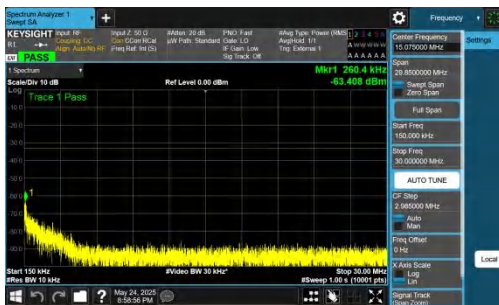
NTNV-DC_5A_n77A-PC2-30-5+25-M+L-QPSK-IDLE-DFT-QPSK-In ner_1RB_Right-0.15-30-PASS
