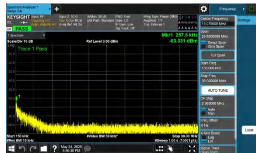
NTNV-DC_5A_n77A-PC2-30-5+25-M+L-QPSK-IDLE-DFT-QPSK-In ner_1RB_Left-0.15-30-PASS
