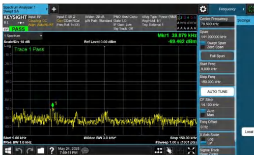
NTNV-DC_5A_n77A-PC2-30-5+15-M+L-QPSK-IDLE-DFT-QPSK-In ner_1RB_Left-0.009-0.15-PASS
