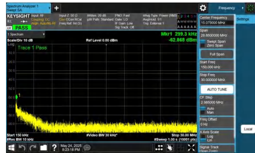
NTNV-DC_5A_n77A-PC2-30-5+20-M+L-QPSK-IDLE-DFT-BPSK-In ner_1RB_Left-0.15-30-PASS
