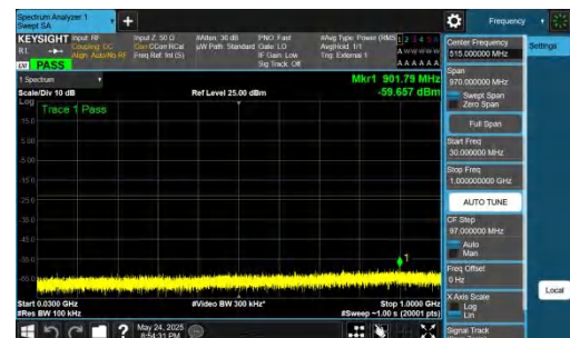
NTNV-DC_5A_n77A-PC2-30-5+25-M+L-QPSK-IDLE-DFT-BPSK-In ner_1RB_Right-30-1000-PASS
