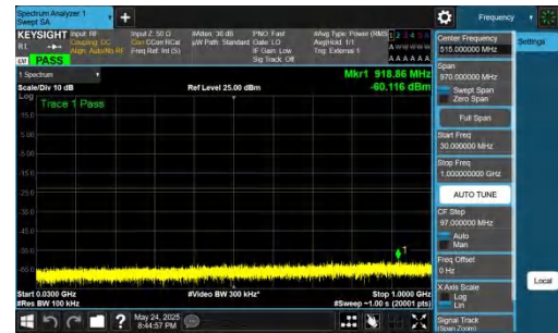
NTNV-DC_5A_n77A-PC2-30-5+20-M+H-QPSK-IDLE-DFT-BPSK-In ner_1RB_Right-30-1000-PASS
