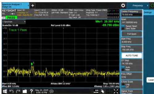
NTNV-DC_5A_n77A-PC2-30-5+25-M+L-QPSK-IDLE-DFT-QPSK-In ner_1RB_Left-0.009-0.15-PASS
