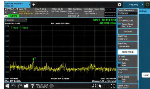
NTNV-DC_5A_n77A-PC2-30-5+10-M+M-QPSK-IDLE-DFT-QPSK-In ner_1RB_Right-0.009-0.15-PASS
