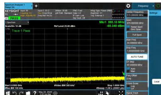
NTNV-DC_5A_n77A-PC2-30-5+15-M+L-QPSK-IDLE-DFT-BPSK-In ner_1RB_Right-30-1000-PASS
