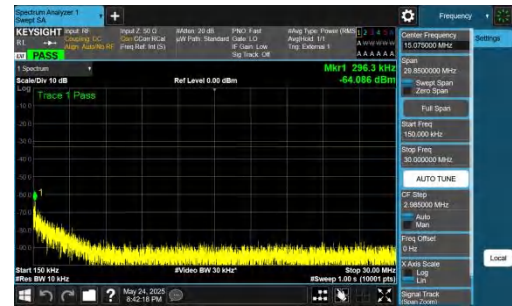
NTNV-DC_5A_n77A-PC2-30-5+20-M+H-QPSK-IDLE-DFT-BPSK-In ner_1RB_Left-0.15-30-PASS
