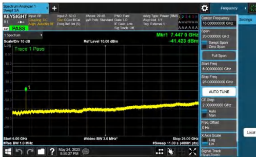
NTNV-DC_5A_n77A-PC2-30-5+25-M+L-QPSK-IDLE-DFT-BPSK-In ner_1RB_Right-6000-26000-PASS
