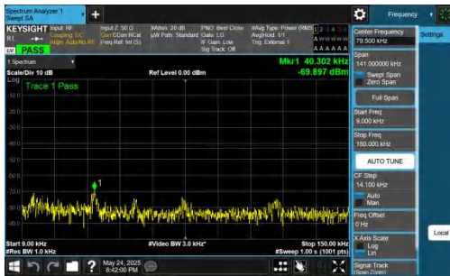
NTNV-DC_5A_n77A-PC2-30-5+20-M+H-QPSK-IDLE-DFT-BPSK-I nner_1RB_Left-0.009-0.15-PASS
