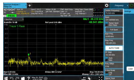
NTNV-DC_5A_n77A-PC2-30-5+20-M+L-QPSK-IDLE-DFT-BPSK-In ner_1RB_Right-0.009-0.15-PASS
