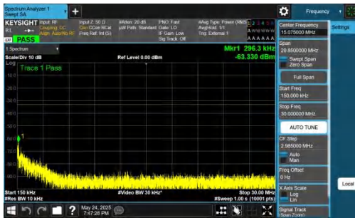
NTNV-DC_5A_n77A-PC2-30-5+10-M+H-QPSK-IDLE-DFT-BPSK-I nner_1RB_Right-0.15-30-PASS
