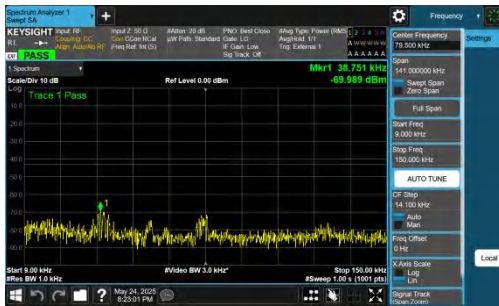
NTNV-DC_5A_n77A-PC2-30-5+20-M+L-QPSK-IDLE-DFT-BPSK-In ner_1RB_Left-0.009-0.15-PASS
