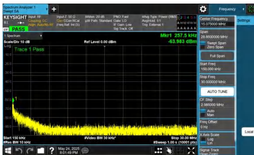
NTNV-DC_5A_n77A-PC2-30-5+15-M+L-QPSK-IDLE-DFT-QPSK-In_ner_1RB_Right-0.15-30-PASS
