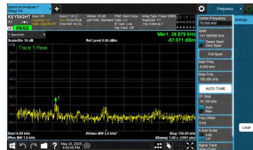
NTNV-DC_5A_n77A-PC2-30-5+25-M+L-QPSK-IDLE-DFT-BPSK-In ner_1RB_Right-0.009-0.15-PASS
