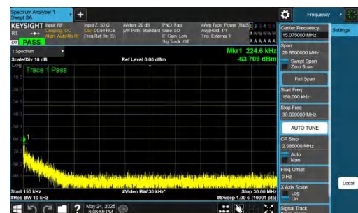
NTNV-DC_5A_n77A-PC2-30-5+15-M+M-QPSK-IDLE-DFT-QPSK-In ner_1RB_Left-0.15-30-PASS
