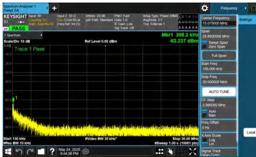
NTNV-DC_5A_n77A-PC2-30-5+20-M+H-QPSK-IDLE-DFT-BPSK-In nner_1RB_Right-0.15-30-PASS
