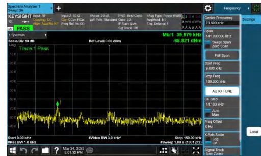
NTNV-DC_5A_n77A-PC2-30-5+15-M+L-QPSK-IDLE-DFT-QPSK-In_ner_1RB_Right-0.009-0.15-PASS
