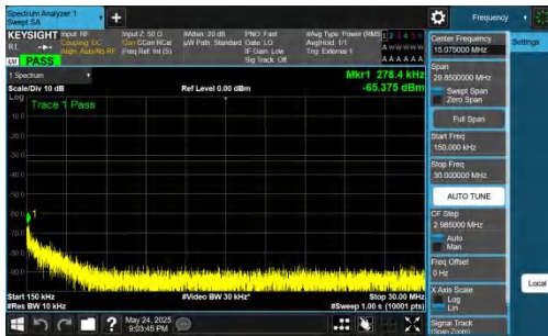
NTNV-DC_5A_n77A-PC2-30-5+25-M+M-QPSK-IDLE-DFT-BPSK-I nner_1RB_Right-0.15-30-PASS
