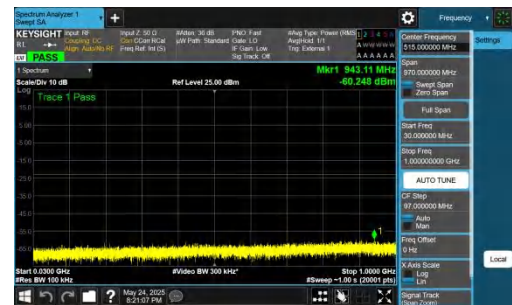
NTNV-DC_5A_n77A-PC2-30-5+15-M+H-QPSK-IDLE-DFT-QPSK-Inner_1RB_Right-30-1000-PASS
