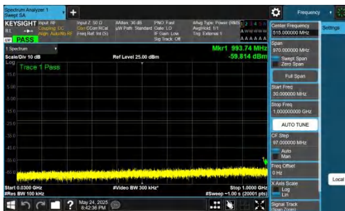
NTNV-DC_5A_n77A-PC2-30-5+20-M+H-QPSK-IDLE-DFT-BPSK-I nner_1RB_Left-30-1000-PASS
