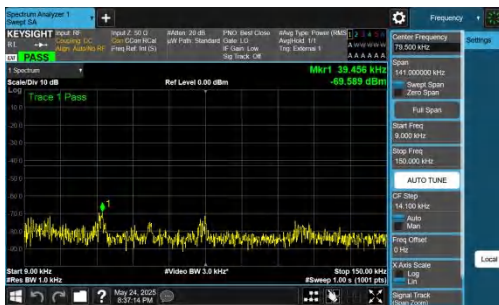
NTVN-DC_5A_n77A-PC2-30-5+20-M+M-QPSK-IDLE-DFT-QPSK-Inner_1RB_Left-0.009-0.15-PASS
