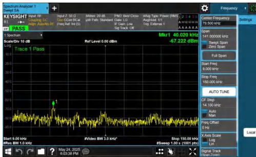
NTNV-DC_5A_n77A-PC2-30-5+90-M+L-QPSK-IDLE-DFT-BPSK-In ner_1RB_Left-0.009-0.15-PASS
