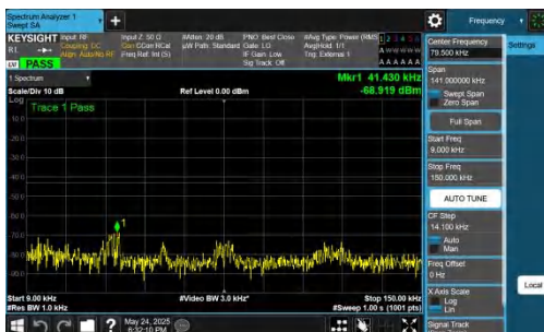
NTNV-DC_5A_n77A-PC2-30-5+100-M+M-QPSK-IDLE-DFT-BPSK-Inner_1RB_Left-0.009-0.15-PASS
