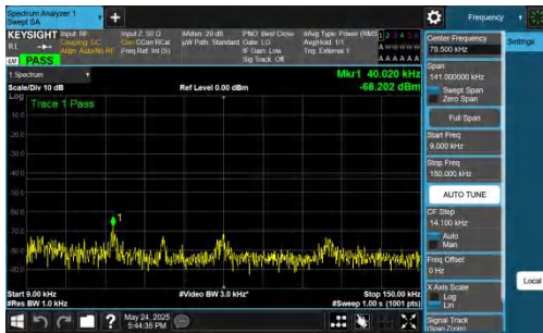
NTVN-DC_5A_n77A-PC2-30-5+80-M+M-QPSK-IDLE-DFT-BPSK-Inner_1RB_Left-0.009-0.15-PASS
