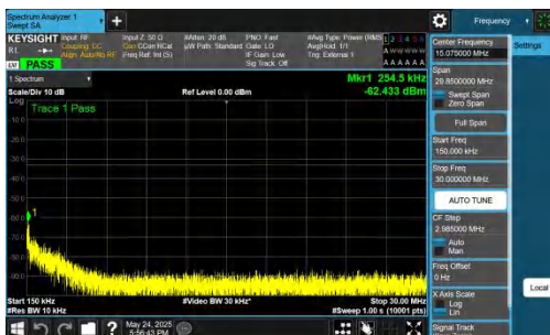
NTNV-DC_5A_n77A-PC2-30-5+80-M+H-QPSK-IDLE-DFT-BPSK-I nner_1RB_Right-0.15-30-PASS
