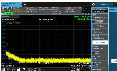
NTNV-DC_5A_n77A-PC2-30-5+100-M+M-QPSK-IDLE-DFT-BPSK- Inner_1RB_Right-0.15-30-PASS
