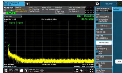
NTNV-DC_5A_n77A-PC2-30-5+90-M+H-QPSK-IDLE-DFT-BPSK-Inner_1RB_Left-0.15-30-PASS
