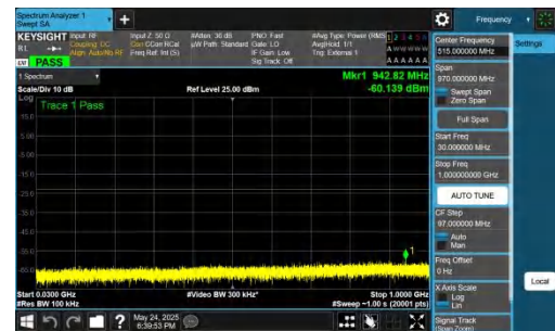
NTNV-DC_5A_n77A-PC2-30-5+100-M+M-QPSK-IDLE-DFT-QPSK-I nner_1RB_Right-30-1000-PASS
