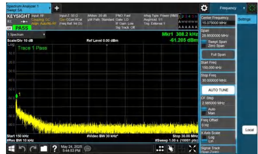
NTVN-DC_5A_n77A-PC2-30-5+80-M+M-QPSK-IDLE-DFT-BPSK-Inner_1RB_Left-0.15-30-PASS
