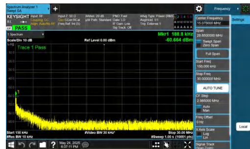
NTNV-DC_5A_n77A-PC2-30-5+100-M+M-QPSK-IDLE-DFT-QPSK-I nner_1RB_Left-0.15-30-PASS
