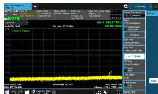
NTNV-DC_5A_n77A-PC2-30-5+90-M+L-QPSK-IDLE-DFT-QPSK-In ner_1RB_Right-30-1000-PASS
