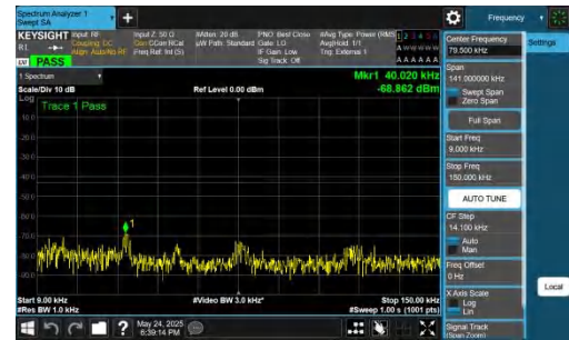
NTNV-DC_5A_n77A-PC2-30-5+100-M+M-QPSK-IDLE-DFT-QPSK-I nner_1RB_Right-0.009-0.15-PASS
