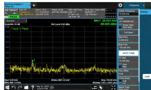
NTNV-DC_5A_n77A-PC2-30-5+100-M+M-QPSK-IDLE-DFT-BPSK-I nner_1RB_Right-0.009-0.15-PASS
