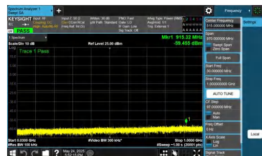
NTNV-DC_5A_n77A-PC2-30-5+80-M+M-QPSK-IDLE-DFT-QPSK-In ner_1RB_Right-30-1000-PASS
