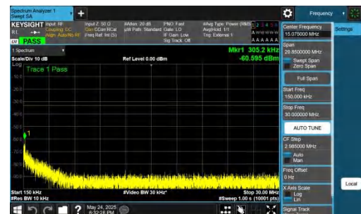
NTNV-DC_5A_n77A-PC2-30-5+100-M+M-QPSK-IDLE-DFT-BPSK-Inner_1RB_Left-0.15-30-PASS
