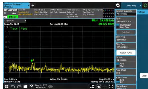
NTNV-DC_5A_n77A-PC2-30-5+80-M+H-QPSK-IDLE-DFT-QPSK-In ner 1RB Right-0.009-0.15-PASS
