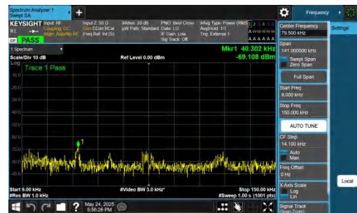
NTNV-DC_5A_n77A-PC2-30-5+80-M+H-QPSK-IDLE-DFT-BPSK-In ner_1RB_Right-0.009-0.15-PASS
