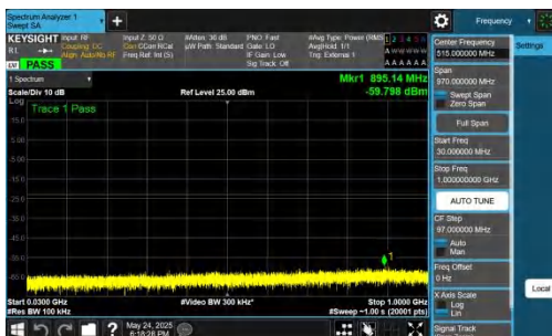
NTNV-DC_5A_n77A-PC2-30-5+90-M+M-QPSK-IDLE-DFT-QPSK-I nner_1RB_Left-30-1000-PASS
