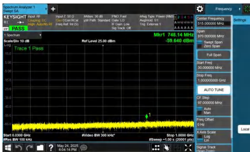
NTNV-DC_5A_n77A-PC2-30-5+90-M+L-QPSK-IDLE-DFT-BPSK-In ner_1RB_Left-30-1000-PASS
