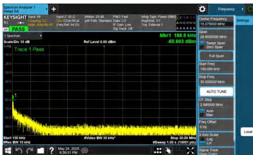
NTNV-DC_5A_n77A-PC2-30-5+100-M+M-QPSK-IDLE-DFT-QPSK- Inner_1RB_Right-0.15-30-PASS
