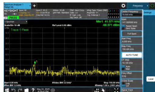
NTNV-DC_5A_n77A-PC2-30-5+90-M+H-QPSK-IDLE-DFT-QPSK-Inner_1RB_Right-0.009-0.15-PASS
