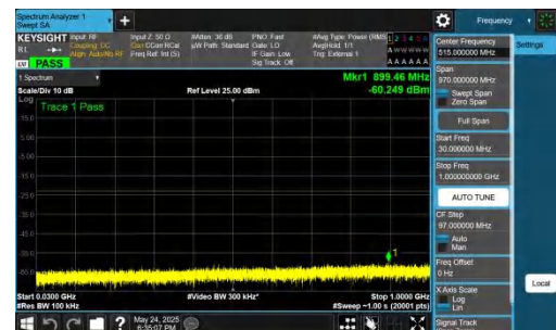
NTNV-DC_5A_n77A-PC2-30-5+100-M+M-QPSK-IDLE-DFT-BPSK-I nner_1RB_Right-30-1000-PASS
