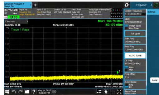
NTVN-DC_5A_n77A-PC2-30-5+90-M+H-QPSK-IDLE-DFT-BPSK-Inner_1RB_Right-30-1000-PASS
