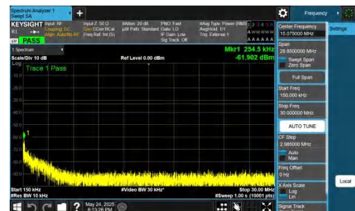
NTNV-DC_5A_n77A-PC2-30-5+90-M+M-QPSK-IDLE-DFT-BPSK-In ner_1RB_Left-0.15-30-PASS
