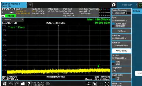
NTNV-DC_5A_n77A-PC2-30-5+100-M+M-QPSK-IDLE-DFT-QPSK- Inner_1RB_Left-30-1000-PASS
