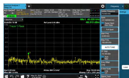
NTNV-DC_5A_n77A-PC2-30-5+90-M+H-QPSK-IDLE-DFT-BPSK-Inner_1RB_Right-0.009-0.15-PASS
