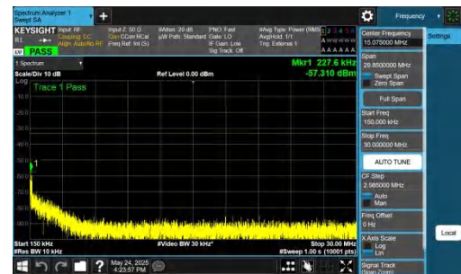
NTNV-DC_5A_n77A-PC2-30-5+50-M+M-QPSK-IDLE-DFT-QPSK-Inner_1RB_Left-0.15-30-PASS
