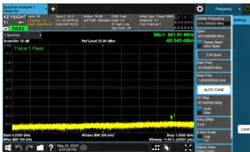
NTNV-DC_5A_n77A-PC2-30-5+70-M+L-QPSK-IDLE-DFT-BPSK-In ner_1RB_Left-30-1000-PASS
