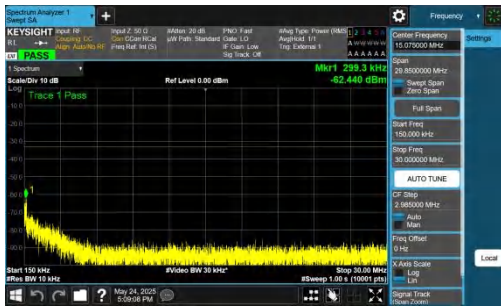
NTNV-DC_5A_n77A-PC2-30-5+70-M+L-QPSK-IDLE-DFT-BPSK-In ner_1RB_Right-0.15-30-PASS
