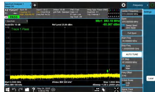
NTNV-DC_5A_n77A-PC2-30-5+80-M+L-QPSK-IDLE-DFT-BPSK-In ner_1RB_Right-30-1000-PASS
