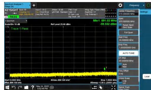
NTNV-DC_5A_n77A-PC2-30-5+80-M+L-QPSK-IDLE-DFT-QPSK-In ner_1RB_Right-30-1000-PASS
