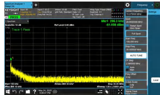
NTNV-DC_5A_n77A-PC2-30-5+70-M+L-QPSK-IDLE-DFT-BPSK-In ner_1RB_Left-0.15-30-PASS
