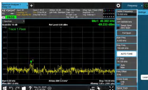
NTNV-DC_5A_n77A-PC2-30-5+60-M+L-QPSK-IDLE-DFT-BPSK-Inner_1RB_Left-0.009-0.15-PASS
