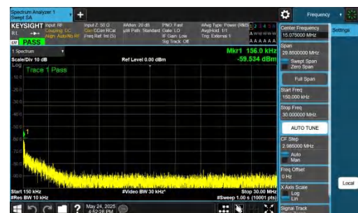
NTNV-DC_5A_n77A-PC2-30-5+60-M+M-QPSK-IDLE-DFT-QPSK-In ner_1RB_Left-0.15-30-PASS
