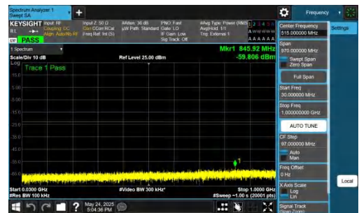
NTNV-DC_5A_n77A-PC2-30-5+60-M+H-QPSK-IDLE-DFT-QPSK-Inner_1RB_Right-30-1000-PASS
