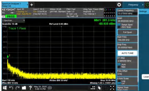
NTNV-DC_5A_n77A-PC2-30-5+70-M+H-QPSK-IDLE-DFT-BPSK-Inner_1RB_Right-0.15-30-PASS
