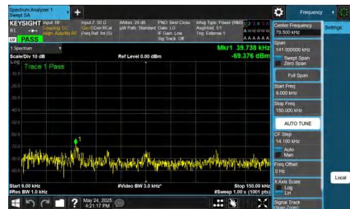
NTNV-DC_5A_n77A-PC2-30-5+50-M+M-QPSK-IDLE-DFT-BPSK-In ner_1RB_Right-0.009-0.15-PASS
