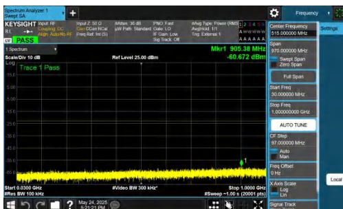
NTVN-DC_5A_n77A-PC2-30-5+70-M+M-QPSK-IDLE-DFT-QPSK-Inner_1RB_Left-30-1000-PASS
