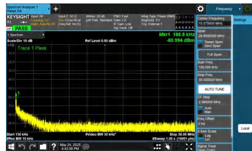
NTNV-DC_5A_n77A-PC2-30-5+60-M+L-QPSK-IDLE-DFT-QPSK-In ner_1RB_Left-0.15-30-PASS
