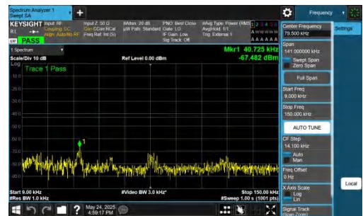
NTNV-DC_5A_n77A-PC2-30-5+60-M+H-QPSK-IDLE-DFT-BPSK-In ner_1RB_Right-0.009-0.15-PASS
