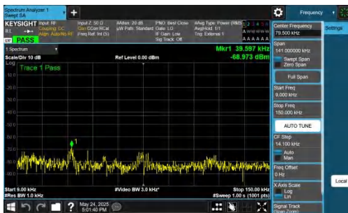
NTNV-DC_5A_n77A-PC2-30-5+60-M+H-QPSK-IDLE-DFT-QPSK-Inner_1RB_Left-0.009-0.15-PASS
