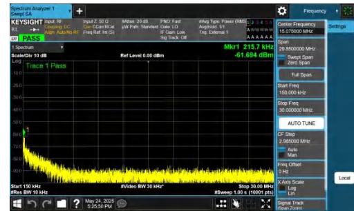
NTNV-DC_5A_n77A-PC2-30-5+70-M+H-QPSK-IDLE-DFT-BPSK-Inner_1RB_Left-0.15-30-PASS
