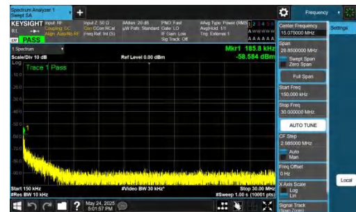
NTNV-DC_5A_n77A-PC2-30-5+60-M+H-QPSK-IDLE-DFT-QPSK-Inner_1RB_Left-0.15-30-PASS
