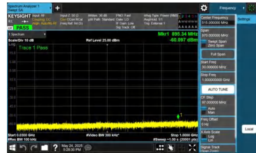
NTNV-DC_5A_n77A-PC2-30-5+70-M+H-QPSK-IDLE-DFT-BPSK-Inner_1RB_Right-30-1000-PASS
