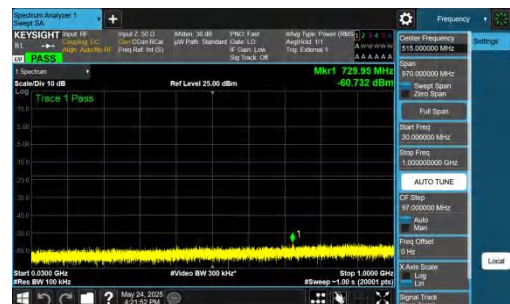
NTNV-DC_5A_n77A-PC2-30-5+50-M+M-QPSK-IDLE-DFT-BPSK-In ner_1RB_Right-30-1000-PASS
