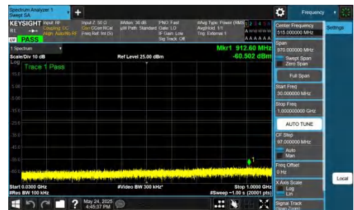
NTNV-DC_5A_n77A-PC2-30-5+60-M+L-QPSK-IDLE-DFT-QPSK-In ner_1RB_Right-30-1000-PASS
