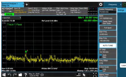
NTVN-DC_5A_n77A-PC2-30-5+70-M+M-QPSK-IDLE-DFT-QPSK-Inner_1RB_Left-0.009-0.15-PASS
