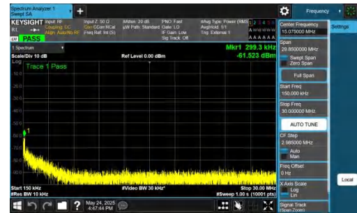
NTVN-DC_5A_n77A-PC2-30-5+60-M+M-QPSK-IDLE-DFT-BPSK-Inner_1RB_Left-0.15-30-PASS
