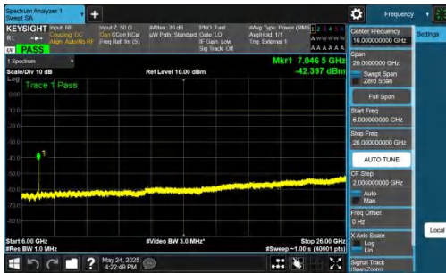
NTNV-DC_5A_n77A-PC2-30-5+50-M+M-QPSK-IDLE-DFT-BPSK-Inner_1RB_Right-6000-26000-PASS
