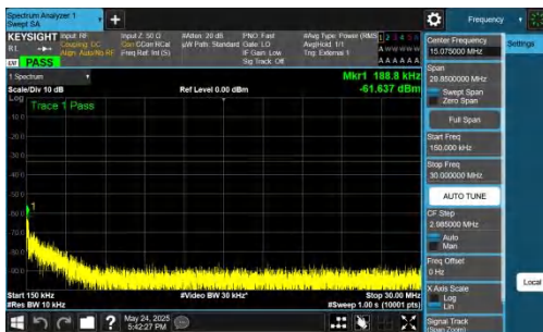
NTNV-DC_5A_n77A-PC2-30-5+80-M+L-QPSK-IDLE-DFT-QPSK-In ner_1RB_Right-0.15-30-PASS
