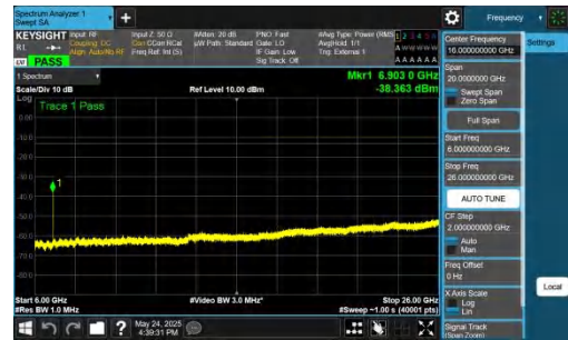
NTNV-DC_5A_n77A-PC2-30-5+60-M+L-QPSK-IDLE-DFT-BPSK-In ner_1RB_Left-6000-26000-PASS
