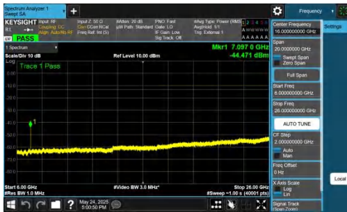
NTNV-DC_5A_n77A-PC2-30-5+60-M+H-QPSK-IDLE-DFT-BPSK-Inner_1RB_Right-6000-26000-PASS
