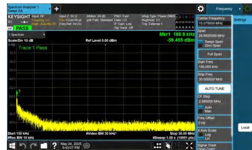
NTNV-DC_5A_n77A-PC2-30-5+80-M+L-QPSK-IDLE-DFT-QPSK-In ner_1RB_Left-0.15-30-PASS
