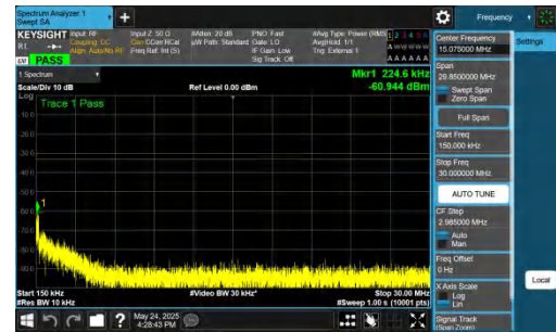
NTNV-DC_5A_n77A-PC2-30-5+50-M+H-QPSK-IDLE-DFT-BPSK-In ner_1RB_Left-0.15-30-PASS
