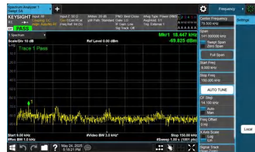
NTVN-DC_5A_n77A-PC2-30-5+70-M+M-QPSK-IDLE-DFT-BPSK-Inner_1RB_Right-0.009-0.15-PASS
