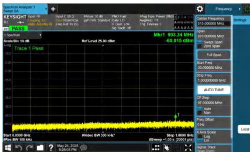
NTNV-DC_5A_n77A-PC2-30-5+70-M+H-QPSK-IDLE-DFT-BPSK-Inner_1RB_Left-30-1000-PASS
