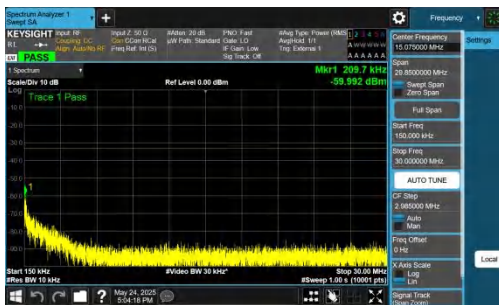
NTNV-DC_5A_n77A-PC2-30-5+60-M+H-QPSK-IDLE-DFT-QPSK-Inner_1RB_Right-0.15-30-PASS
