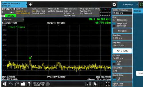
NTNV-DC_5A_n77A-PC2-30-5+70-M+L-QPSK-IDLE-DFT-BPSK-In ner_1RB_Left-0.009-0.15-PASS
