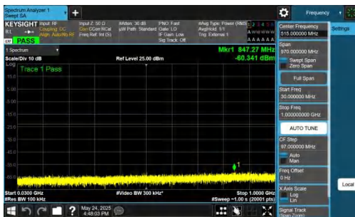
NTVN-DC_5A_n77A-PC2-30-5+60-M+M-QPSK-IDLE-DFT-BPSK-Inner_1RB_Left-30-1000-PASS
