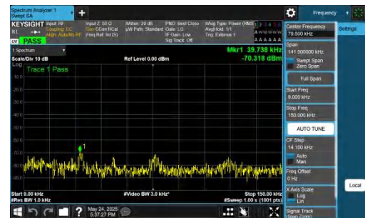
NTNV-DC_5A_n77A-PC2-30-5+80-M+L-QPSK-IDLE-DFT-BPSK-In ner_1RB_Right-0.009-0.15-PASS
