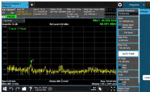
NTNV-DC_5A_n77A-PC2-30-5+70-M+H-QPSK-IDLE-DFT-BPSK-Inner_1RB_Left-0.009-0.15-PASS
