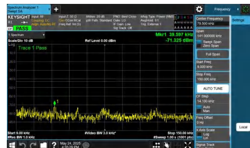
NTNV-DC_5A_n77A-PC2-30-5+50-M+H-QPSK-IDLE-DFT-QPSK-In ner_1RB_Right-0.009-0.15-PASS
