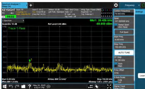
NTNV-DC_5A_n77A-PC2-30-5+60-M+L-QPSK-IDLE-DFT-QPSK-In ner_1RB_Left-0.009-0.15-PASS
