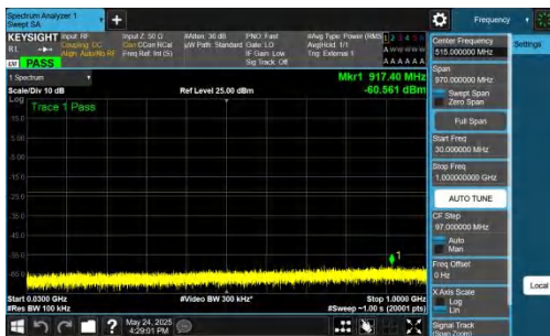
NTNV-DC_5A_n77A-PC2-30-5+50-M+H-QPSK-IDLE-DFT-BPSK-I nner_1RB_Left-30-1000-PASS
