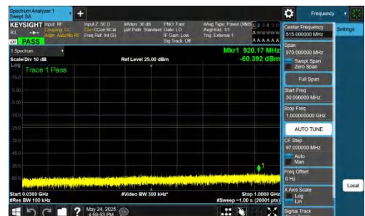
NTNV-DC_5A_n77A-PC2-30-5+60-M+H-QPSK-IDLE-DFT-BPSK-In ner_1RB_Right-30-1000-PASS
