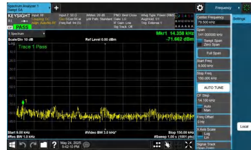
NTNV-DC_5A_n77A-PC2-30-5+80-M+L-QPSK-IDLE-DFT-QPSK-In ner_1RB_Right-0.009-0.15-PASS
