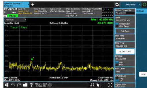
NTNV-DC_5A_n77A-PC2-30-5+70-M+M-QPSK-IDLE-DFT-QPSK-In ner_1RB_Right-0.009-0.15-PASS
