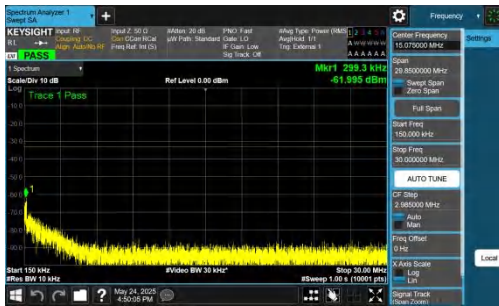
NTNV-DC_5A_n77A-PC2-30-5+60-M+M-QPSK-IDLE-DFT-BPSK-I nner_1RB_Right-0.15-30-PASS
