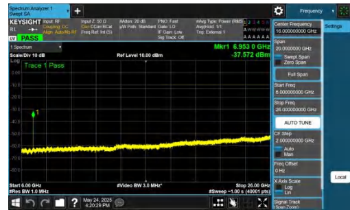
NTNV-DC_5A_n77A-PC2-30-5+50-M+M-QPSK-IDLE-DFT-BPSK-In ner_1RB_Left-6000-26000-PASS
