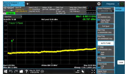
NTNV-DC_5A_n77A-PC2-30-5+60-M+H-QPSK-IDLE-DFT-BPSK-In ner_1RB_Left-6000-26000-PASS
