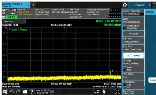
NTNV-DC_5A_n77A-PC2-30-5+60-M+M-QPSK-IDLE-DFT-QPSK-I nner_1RB_Left-30-1000-PASS
