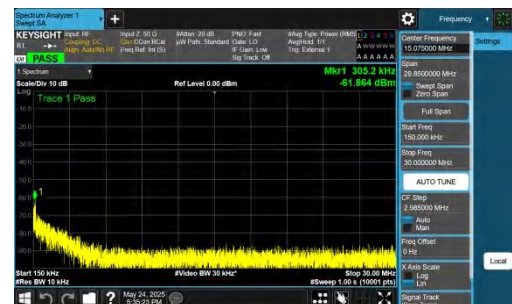
NTNV-DC_5A_n77A-PC2-30-5+80-M+L-QPSK-IDLE-DFT-BPSK-Inner_1RB_Left-0.15-30-PASS
