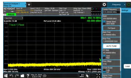
NTNV-DC_5A_n77A-PC2-30-5+70-M+M-QPSK-IDLE-DFT-QPSK-In ner_1RB_Right-30-1000-PASS
