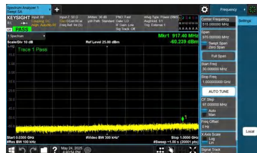
NTNV-DC_5A_n77A-PC2-30-5+60-M+L-QPSK-IDLE-DFT-BPSK-In ner_1RB_Right-30-1000-PASS
