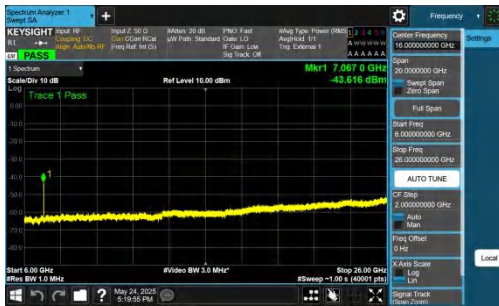
NTVN-DC_5A_n77A-PC2-30-5+70-M+M-QPSK-IDLE-DFT-BPSK-Inner_1RB_Right-6000-26000-PASS
