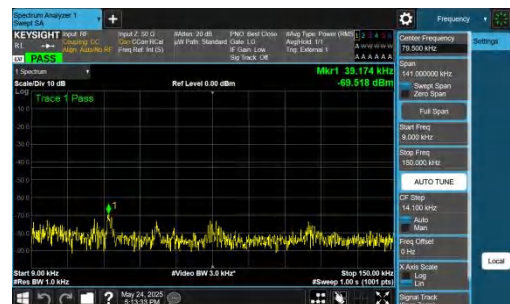
NTNV-DC_5A_n77A-PC2-30-5+70-M+L-QPSK-IDLE-DFT-QPSK-In ner_1RB_Right-0.009-0.15-PASS
