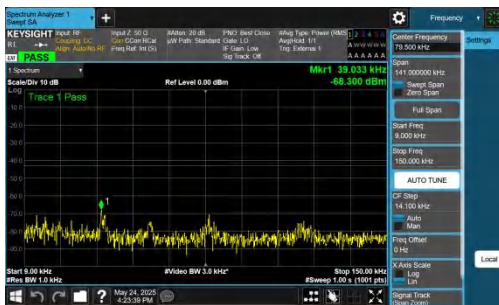
NTNV-DC_5A_n77A-PC2-30-5+50-M+M-QPSK-IDLE-DFT-QPSK-Inner_1RB_Left-0.009-0.15-PASS
