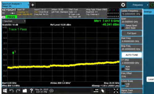
NTNV-DC_5A_n77A-PC2-30-5+60-M+L-QPSK-IDLE-DFT-BPSK-In ner_1RB_Right-6000-26000-PASS
