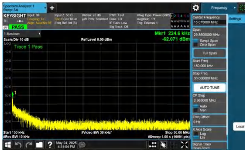
NTNV-DC_5A_n77A-PC2-30-5+50-M+H-QPSK-IDLE-DFT-BPSK-In nner_1RB_Right-0.15-30-PASS
