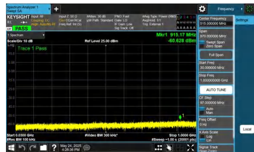
NTNV-DC_5A_n77A-PC2-30-5+50-M+M-QPSK-IDLE-DFT-QPSK-Inner_1RB_Right-30-1000-PASS
