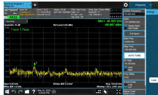
NTNV-DC_5A_n77A-PC2-30-5+50-M+M-QPSK-IDLE-DFT-QPSK-Inner_1RB_Right-0.009-0.15-PASS
