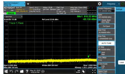
NTNV-DC_5A_n77A-PC2-30-5+60-M+M-QPSK-IDLE-DFT-BPSK-In ner_1RB_Right-30-1000-PASS
