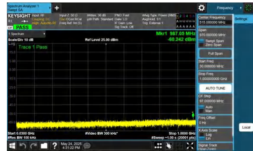
NTNV-DC_5A_n77A-PC2-30-5+50-M+H-QPSK-IDLE-DFT-BPSK-In ner_1RB_Right-30-1000-PASS
