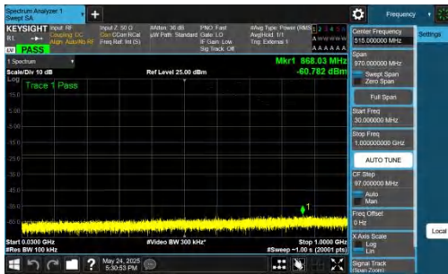
NTNV-DC_5A_n77A-PC2-30-5+70-M+H-QPSK-IDLE-DFT-QPSK-Inner_1RB_Left-30-1000-PASS
