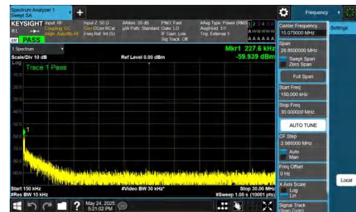
NTVN-DC_5A_n77A-PC2-30-5+70-M+M-QPSK-IDLE-DFT-QPSK-Inner_1RB_Left-0.15-30-PASS
