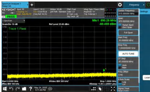
NTNV-DC_5A_n77A-PC2-30-5+70-M+L-QPSK-IDLE-DFT-QPSK-In ner_1RB_Left-30-1000-PASS
