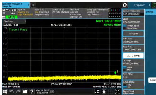
NTNV-DC_5A_n77A-PC2-30-5+50-M+H-QPSK-IDLE-DFT-QPSK-I nner_1RB_Left-30-1000-PASS
