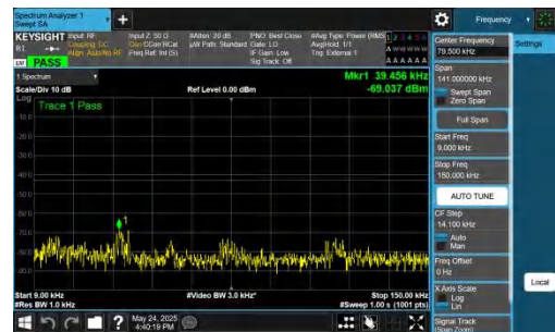
NTNV-DC_5A_n77A-PC2-30-5+60-M+L-QPSK-IDLE-DFT-BPSK-In ner_1RB_Right-0.009-0.15-PASS
