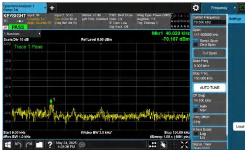
NTNV-DC_5A_n77A-PC2-30-5+50-M+H-QPSK-IDLE-DFT-BPSK-I nner_1RB_Left-0.009-0.15-PASS
