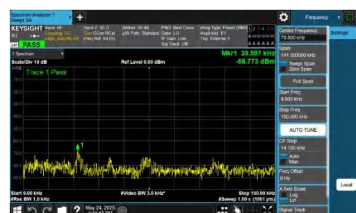
NTVN-DC_5A_n77A-PC2-30-5+60-M+M-QPSK-IDLE-DFT-BPSK-Inner_1RB_Right-0.009-0.15-PASS
