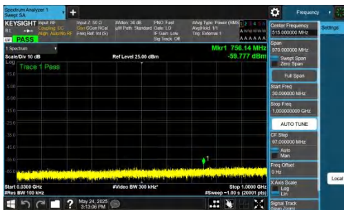
NTNV-DC_5A_n77A-PC2-30-5+30-M+L-QPSK-IDLE-DFT-BPSK-In ner_1RB_Left-30-1000-PASS
