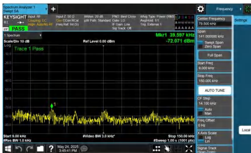
NTNV-DC_5A_n77A-PC2-30-5+40-M+L-QPSK-IDLE-DFT-QPSK-In ner_1RB_Left-0.009-0.15-PASS
