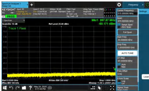
NTNV-DC_5A_n77A-PC2-30-5+30-M+L-QPSK-IDLE-DFT-QPSK-In ner_1RB_Left-30-1000-PASS
