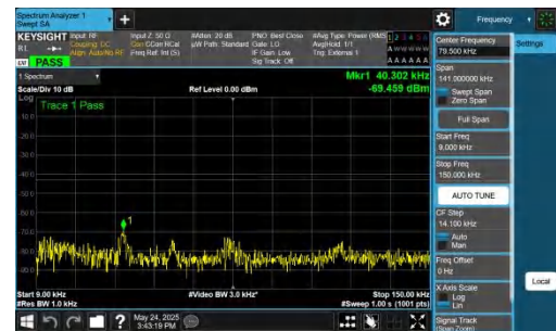
NTNV-DC_5A_n77A-PC2-30-5+40-M+L-QPSK-IDLE-DFT-BPSK-In ner_1RB_Right-0.009-0.15-PASS
