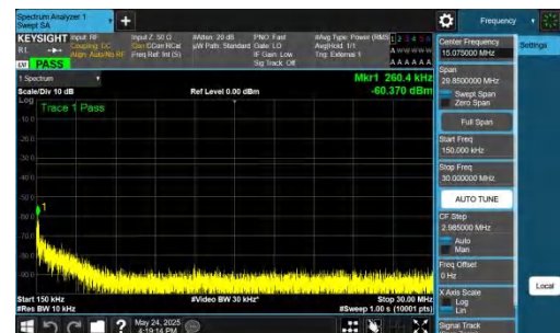
NTNV-DC_5A_n77A-PC2-30-5+50-M+M-QPSK-IDLE-DFT-BPSK-In ner_1RB_Left-0.15-30-PASS
