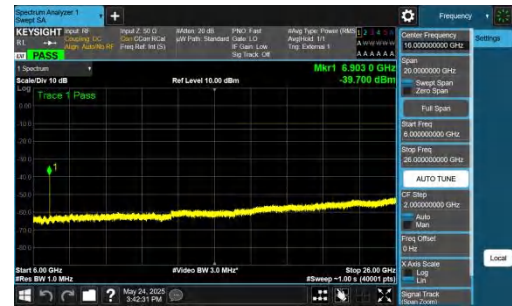
NTNV-DC_5A_n77A-PC2-30-5+40-M+L-QPSK-IDLE-DFT-BPSK-In ner_1RB_Left-6000-26000-PASS
