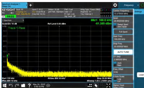
NTNV-DC_5A_n77A-PC2-30-5+40-M+L-QPSK-IDLE-DFT-QPSK-In ner_1RB_Right-0.15-30-PASS
