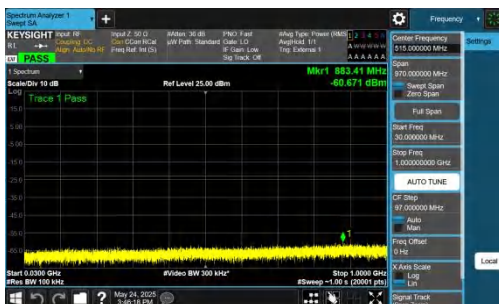
NTNV-DC_5A_n77A-PC2-30-5+40-M+L-QPSK-IDLE-DFT-QPSK-In ner_1RB_Left-30-1000-PASS
