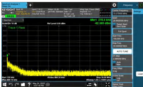
NTNV-DC_5A_n77A-PC2-30-5+40-M+H-QPSK-IDLE-DFT-QPSK-Inner_1RB_Right-0.15-30-PASS
