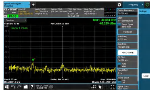
NTNV-DC_5A_n77A-PC2-30-5+40-M+L-QPSK-IDLE-DFT-QPSK-In ner_1RB_Right-0.009-0.15-PASS
