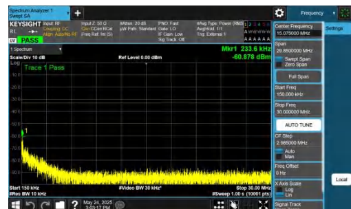
NTNV-DC_5A_n77A-PC2-30-5+25-M+H-QPSK-IDLE-DFT-BPSK-Inner_1RB_Left-0.15-30-PASS
