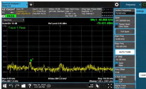
NTNV-DC_5A_n77A-PC2-30-5+30-M+H-QPSK-IDLE-DFT-BPSK-In nner_1RB_Left-0.009-0.15-PASS
