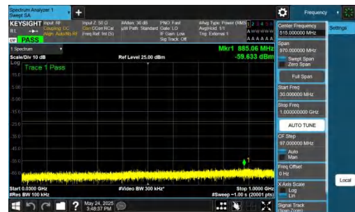
NTNV-DC_5A_n77A-PC2-30-5+40-M+L-QPSK-IDLE-DFT-QPSK-In ner_1RB_Right-30-1000-PASS
