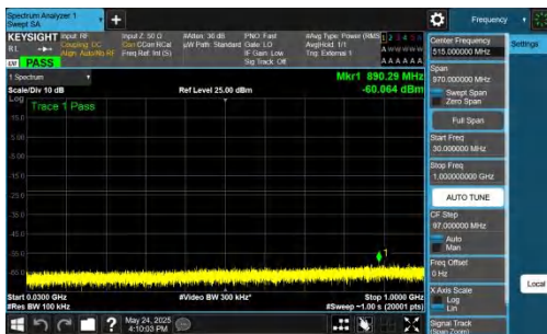
NTNV-DC_5A_n77A-PC2-30-5+50-M+L-QPSK-IDLE-DFT-BPSK-In ner_1RB_Left-30-1000-PASS
