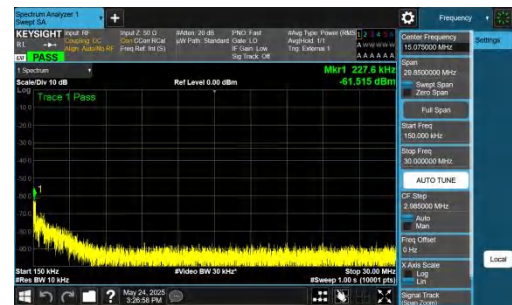
NTNV-DC_5A_n77A-PC2-30-5+30-M+M-QPSK-IDLE-DFT-QPSK-Inner_1RB_Left-0.15-30-PASS
