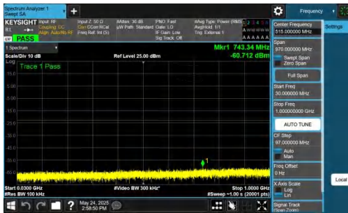
NTNV-DC_5A_n77A-PC2-30-5+25-M+M-QPSK-IDLE-DFT-QPSK-I nner_1RB_Left-30-1000-PASS
