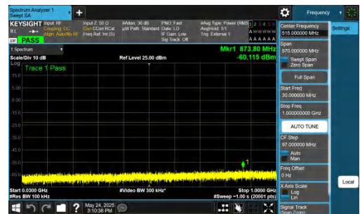
NTNV-DC_5A_n77A-PC2-30-5+25-M+H-QPSK-IDLE-DFT-QPSK-Inner_1RB_Right-30-1000-PASS
