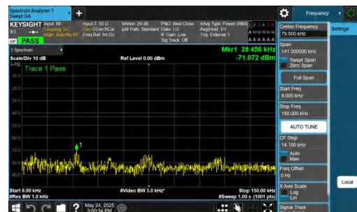
NTNV-DC_5A_n77A-PC2-30-5+25-M+M-QPSK-IDLE-DFT-QPSK-In ner_1RB_Right-0.009-0.15-PASS
