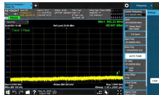
NTNV-DC_5A_n77A-PC2-30-5+30-M+M-QPSK-IDLE-DFT-QPSK-In ner_1RB_Right-30-1000-PASS
