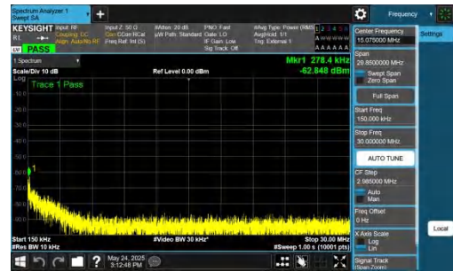
NTNV-DC_5A_n77A-PC2-30-5+30-M+L-QPSK-IDLE-DFT-BPSK-In ner_1RB_Left-0.15-30-PASS
