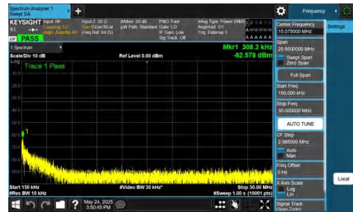
NTVN-DC_5A_n77A-PC2-30-5+40-M+M-QPSK-IDLE-DFT-BPSK-Inner_1RB_Left-0.15-30-PASS
