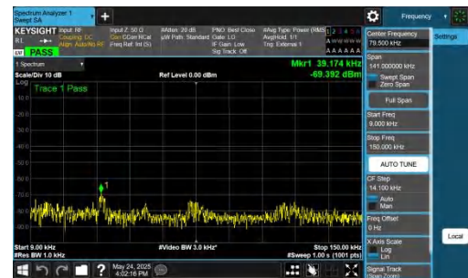
NTNV-DC_5A_n77A-PC2-30-5+40-M+H-QPSK-IDLE-DFT-BPSK-In ner_1RB_Right-0.009-0.15-PASS
