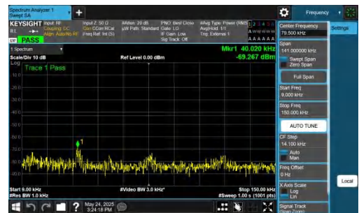
NTNV-DC_5A_n77A-PC2-30-5+30-M+M-QPSK-IDLE-DFT-BPSK-Inner_1RB_Right-0.009-0.15-PASS
