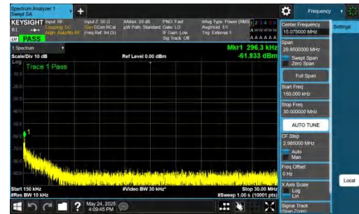
NTNV-DC_5A_n77A-PC2-30-5+50-M+L-QPSK-IDLE-DFT-BPSK-In ner_1RB_Left-0.15-30-PASS
