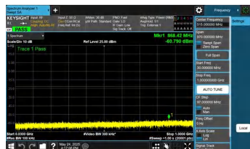
NTNV-DC_5A_n77A-PC2-30-5+50-M+L-QPSK-IDLE-DFT-QPSK-In ner_1RB_Right-30-1000-PASS
