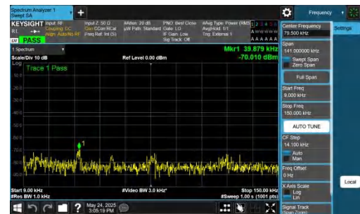
NTNV-DC_5A_n77A-PC2-30-5+25-M+H-QPSK-IDLE-DFT-BPSK-In ner_1RB_Right-0.009-0.15-PASS
