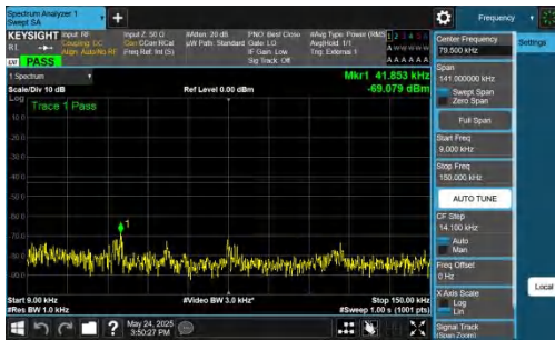
NTVN-DC_5A_n77A-PC2-30-5+40-M+M-QPSK-IDLE-DFT-BPSK-Inner_1RB_Left-0.009-0.15-PASS
