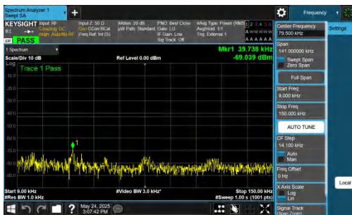
NTNV-DC_5A_n77A-PC2-30-5+25-M+H-QPSK-IDLE-DFT-QPSK-Inner_1RB_Left-0.009-0.15-PASS
