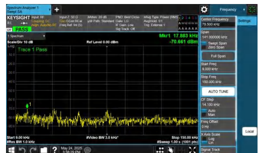
NTNV-DC_5A_n77A-PC2-30-5+30-M+H-QPSK-IDLE-DFT-QPSK-In ner_1RB_Right-0.009-0.15-PASS
