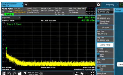
NTNV-DC_5A_n77A-PC2-30-5+25-M+H-QPSK-IDLE-DFT-BPSK-I nner_1RB_Right-0.15-30-PASS
