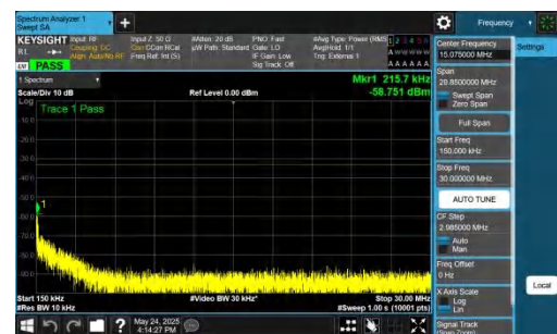
NTNV-DC_5A_n77A-PC2-30-5+50-M+L-QPSK-IDLE-DFT-QPSK-In ner_1RB_Left-0.15-30-PASS
