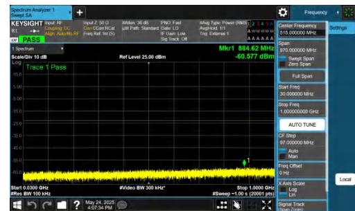
NTNV-DC_5A_n77A-PC2-30-5+40-M+H-QPSK-IDLE-DFT-QPSK-Inner_1RB_Right-30-1000-PASS
