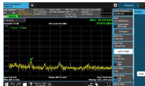
NTNV-DC_5A_n77A-PC2-30-5+50-M+L-QPSK-IDLE-DFT-QPSK-In ner_1RB_Right-0.009-0.15-PASS
