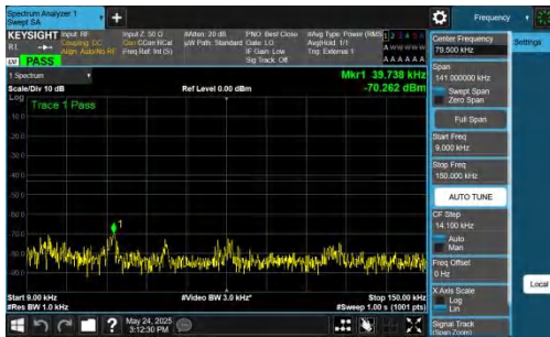
NTNV-DC_5A_n77A-PC2-30-5+30-M+L-QPSK-IDLE-DFT-BPSK-In ner_1RB_Left-0.009-0.15-PASS
