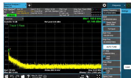
NTNV-DC_5A_n77A-PC2-30-5+30-M+L-QPSK-IDLE-DFT-QPSK-In ner_1RB_Left-0.15-30-PASS
