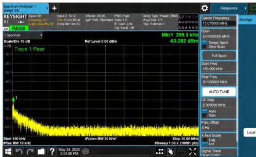
NTNV-DC_5A_n77A-PC2-30-5+40-M+M-QPSK-IDLE-DFT-BPSK-I nner_1RB_Right-0.15-30-PASS
