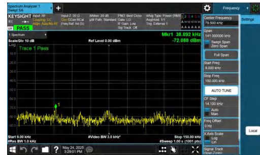
NTNV-DC_5A_n77A-PC2-30-5+30-M+M-QPSK-IDLE-DFT-QPSK-In ner_1RB_Right-0.009-0.15-PASS
