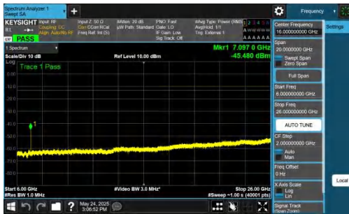
NTNV-DC_5A_n77A-PC2-30-5+25-M+H-QPSK-IDLE-DFT-BPSK-Inner_1RB_Right-6000-26000-PASS
