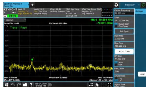
NTNV-DC_5A_n77A-PC2-30-5+30-M+L-QPSK-IDLE-DFT-QPSK-In ner_1RB_Right-0.009-0.15-PASS
