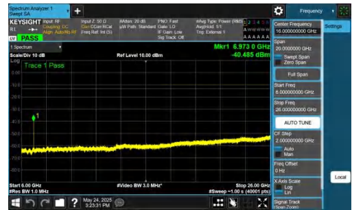
NTNV-DC_5A_n77A-PC2-30-5+30-M+M-QPSK-IDLE-DFT-BPSK-Inner_1RB_Left-6000-26000-PASS
