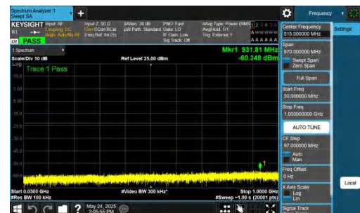
NTNV-DC_5A_n77A-PC2-30-5+25-M+H-QPSK-IDLE-DFT-BPSK-In ner_1RB_Right-30-1000-PASS
