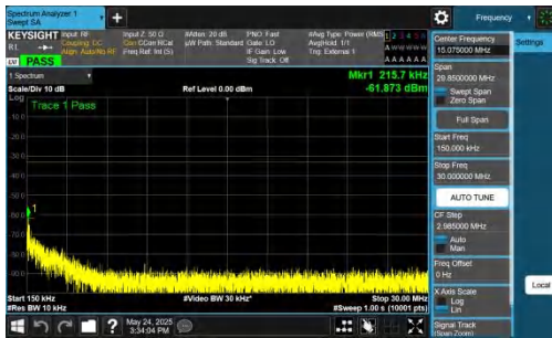
NTVN-DC_5A_n77A-PC2-30-5+30-M+H-QPSK-IDLE-DFT-BPSK-In_nner_1RB_Right-0.15-30-PASS
