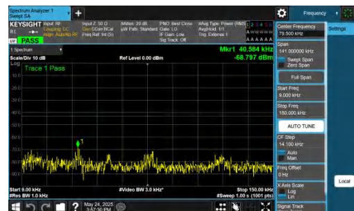
NTVN-DC_5A_n77A-PC2-30-5+40-M+M-QPSK-IDLE-DFT-QPSK-Inner_1RB_Right-0.009-0.15-PASS
