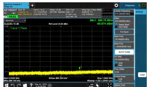
NTNV-DC_5A_n77A-PC2-30-5+30-M+M-QPSK-IDLE-DFT-BPSK-Inner_1RB_Right-30-1000-PASS
