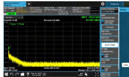
NTNV-DC_5A_n77A-PC2-30-5+30-M+H-QPSK-IDLE-DFT-BPSK-In ner_1RB_Left-0.15-30-PASS
