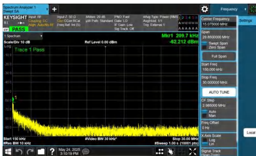
NTNV-DC_5A_n77A-PC2-30-5+25-M+H-QPSK-IDLE-DFT-QPSK-Inner_1RB_Right-0.15-30-PASS
