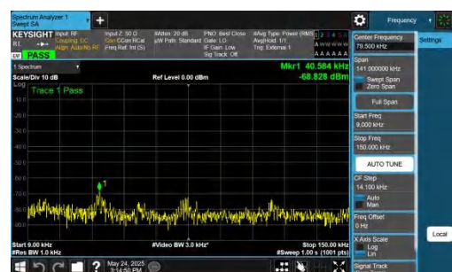
NTNV-DC_5A_n77A-PC2-30-5+30-M+L-QPSK-IDLE-DFT-BPSK-In ner_1RB_Right-0.009-0.15-PASS
