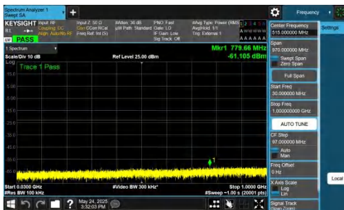
NTNV-DC_5A_n77A-PC2-30-5+30-M+H-QPSK-IDLE-DFT-BPSK-In nner_1RB_Left-30-1000-PASS
