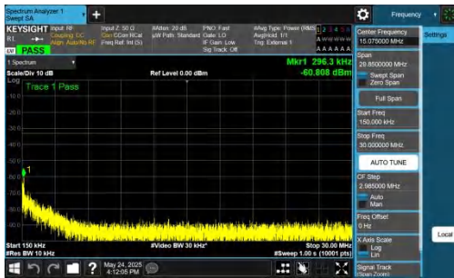
NTNV-DC_5A_n77A-PC2-30-5+50-M+L-QPSK-IDLE-DFT-BPSK-In ner_1RB_Right-0.15-30-PASS
