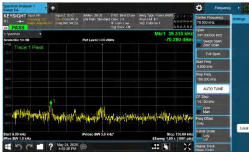
NTNV-DC_5A_n77A-PC2-30-5+50-M+L-QPSK-IDLE-DFT-BPSK-In ner_1RB_Left-0.009-0.15-PASS
