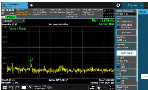
NTNV-DC_5A_n77A-PC2-30-5+30-M+M-QPSK-IDLE-DFT-QPSK-Inner_1RB_Left-0.009-0.15-PASS
