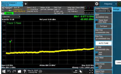
NTNV-DC_5A_n77A-PC2-30-5+40-M+L-QPSK-IDLE-DFT-BPSK-In ner_1RB_Right-6000-26000-PASS
