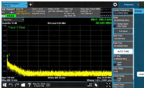
NTNV-DC_5A_n77A-PC2-30-5+30-M+L-QPSK-IDLE-DFT-BPSK-In ner_1RB_Right-0.15-30-PASS
