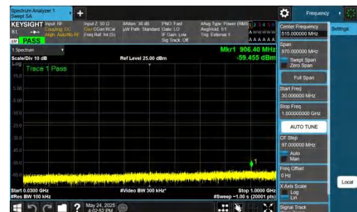
NTNV-DC_5A_n77A-PC2-30-5+40-M+H-QPSK-IDLE-DFT-BPSK-In ner_1RB_Right-30-1000-PASS
