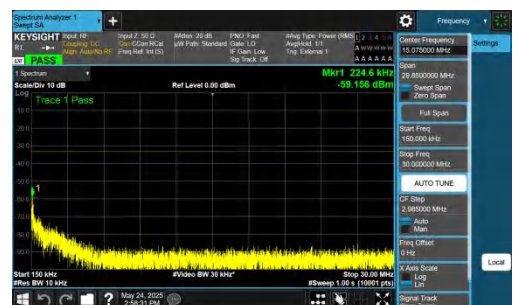
NTNV-DC_5A_n77A-PC2-30-5+25-M+M-QPSK-IDLE-DFT-QPSK-In ner_1RB_Left-0.15-30-PASS
