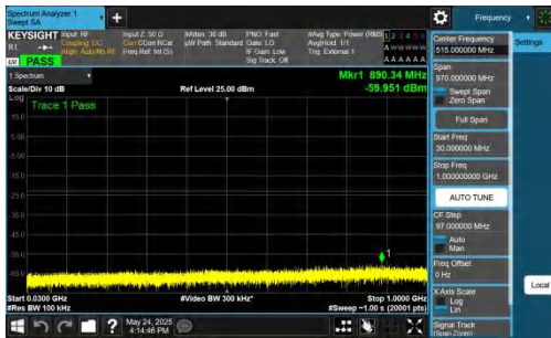
NTNV-DC_5A_n77A-PC2-30-5+50-M+L-QPSK-IDLE-DFT-QPSK-In ner_1RB_Left-30-1000-PASS
