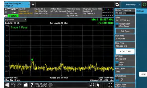
NTNV-DC_5A_n77A-PC2-30-5+40-M+H-QPSK-IDLE-DFT-QPSK-Inner_1RB_Right-0.009-0.15-PASS
