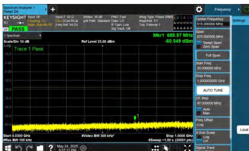
NTNV-DC_5A_n77A-PC2-30-5+30-M+M-QPSK-IDLE-DFT-QPSK-Inner_1RB_Left-30-1000-PASS
