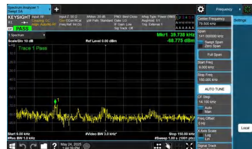
NTNV-DC_5A_n77A-PC2-30-5+10-M+H-QPSK-IDLE-DFT-QPSK-Inner_1RB_Right-0.009-0.15-PASS
