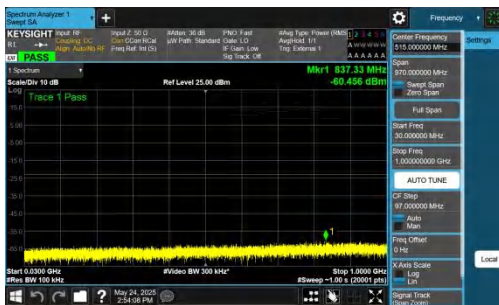
NTVN-DC_5A_n77A-PC2-30-5+25-M+M-QPSK-IDLE-DFT-BPSK-Inner_1RB_Left-30-1000-PASS
