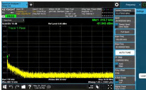
NTNV-DC_5A_n77A-PC2-30-5+10-M+H-QPSK-IDLE-DFT-BPSK-In nner_1RB_Right-0.15-30-PASS
