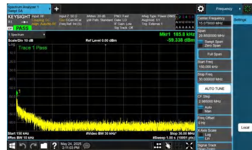
NTNV-DC_5A_n77A-PC2-30-5+15-M+H-QPSK-IDLE-DFT-QPSK-Inner_1RB_Left-0.15-30-PASS
