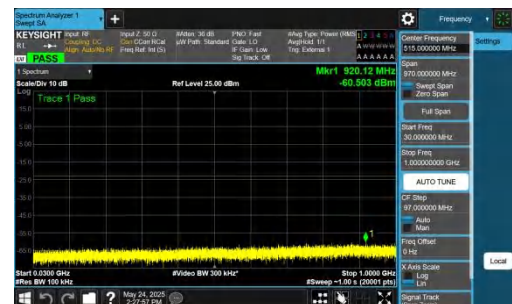
NTNV-DC_5A_n77A-PC2-30-5+20-M+M-QPSK-IDLE-DFT-BPSK-In ner_1RB_Right-30-1000-PASS
