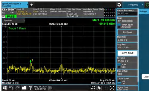
NTNV-DC_5A_n77A-PC2-30-5+20-M+H-QPSK-IDLE-DFT-BPSK-In nner_1RB_Left-0.009-0.15-PASS
