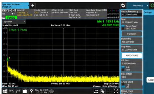
NTNV-DC_5A_n77A-PC2-30-5+20-M+M-QPSK-IDLE-DFT-QPSK-I nner_1RB_Right-0.15-30-PASS
