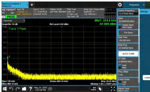
NTNV-DC_5A_n77A-PC2-30-5+20-M+H-QPSK-IDLE-DFT-BPSK-I nner_1RB_Right-0.15-30-PASS
