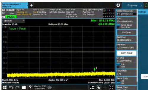
NTNV-DC_5A_n77A-PC2-30-5+20-M+H-QPSK-IDLE-DFT-BPSK-In nner_1RB_Left-30-1000-PASS
