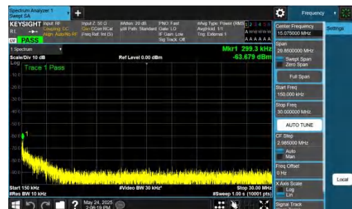
NTNV-DC_5A_n77A-PC2-30-5+15-M+H-QPSK-IDLE-DFT-BPSK-Inner_1RB_Left-0.15-30-PASS
