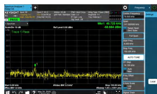
NTNV-DC_5A_n77A-PC2-30-5+10-M+H-QPSK-IDLE-DFT-BPSK-In ner_1RB_Right-0.009-0.15-PASS
