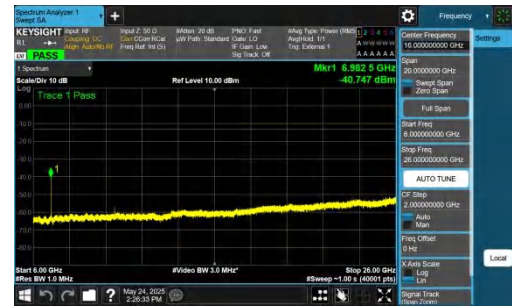
NTNV-DC_5A_n77A-PC2-30-5+20-M+M-QPSK-IDLE-DFT-BPSK-In ner_1RB_Left-6000-26000-PASS
