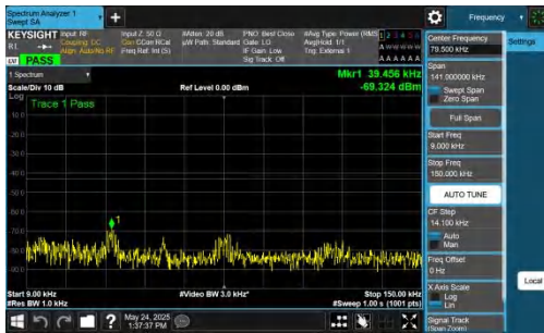
NTNV-DC_5A_n77A-PC2-30-5+10-M+H-QPSK-IDLE-DFT-BPSK-I nner_1RB_Left-0.009-0.15-PASS
