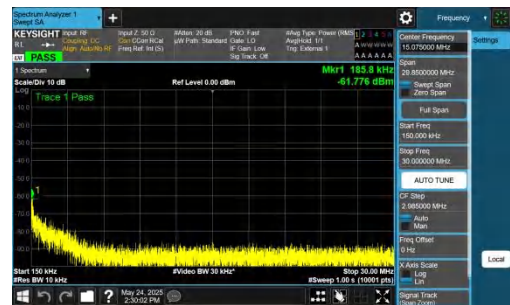
NTNV-DC_5A_n77A-PC2-30-5+20-M+M-QPSK-IDLE-DFT-QPSK-Inner_1RB_Left-0.15-30-PASS
