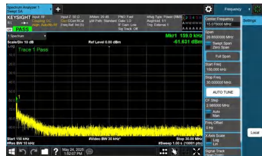
NTNV-DC_5A_n77A-PC2-30-5+15-M+L-QPSK-IDLE-DFT-QPSK-In ner_1RB_Left-0.15-30-PASS
