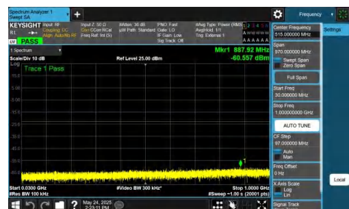
NTNV-DC_5A_n77A-PC2-30-5+20-M+L-QPSK-IDLE-DFT-QPSK-In ner_1RB_Right-30-1000-PASS
