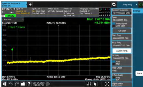
NTNV-DC_5A_n77A-PC2-30-5+20-M+M-QPSK-IDLE-DFT-BPSK-Inner_1RB_Right-6000-26000-PASS
