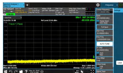
NTNV-DC_5A_n77A-PC2-30-5+20-M+H-QPSK-IDLE-DFT-QPSK-In ner_1RB_Right-30-1000-PASS
