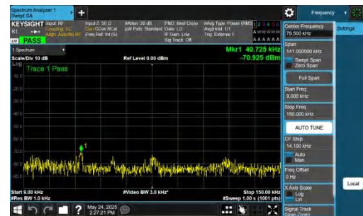
NTNV-DC_5A_n77A-PC2-30-5+20-M+M-QPSK-IDLE-DFT-BPSK-In ner_1RB_Right-0.009-0.15-PASS
