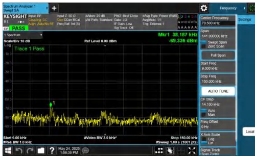
NTNV-DC_5A_n77A-PC2-30-5+15-M+M-QPSK-IDLE-DFT-BPSK-In nner_1RB_Left-0.009-0.15-PASS
