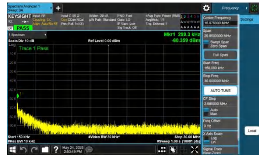
NTVN-DC_5A_n77A-PC2-30-5+25-M+M-QPSK-IDLE-DFT-BPSK-Inner_1RB_Left-0.15-30-PASS
