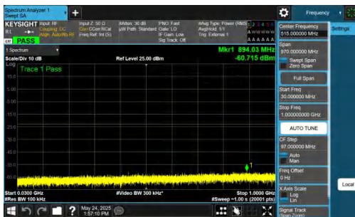
NTNV-DC_5A_n77A-PC2-30-5+15-M+M-QPSK-IDLE-DFT-BPSK-In nner_1RB_Left-30-1000-PASS
