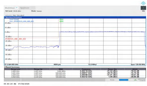
NTNV-DC_5A_n77A-PC2-30-5+80-M+L-QPSK-IDLE-DFT-BPSK-O uter_Full-PASS
