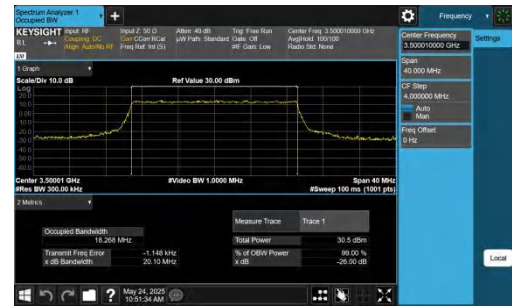
NTNV-DC_5A_n77A-PC2-30-5+20-M+M-QPSK-IDLE-CP-16QAM-O uter_Full-Ant1-PASS
