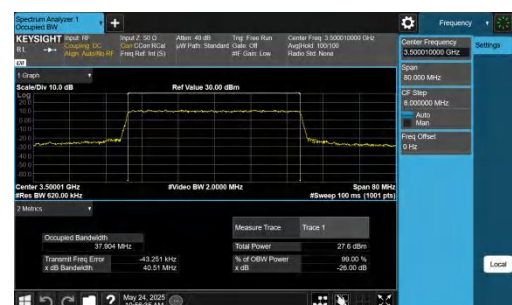
NTNV-DC_5A_n77A-PC2-30-5+40-M+M-QPSK-IDLE-CP-256QAM- Outer_Full-Ant1-PASS
