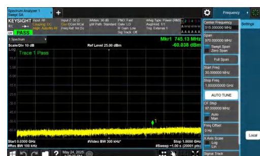
NTNV-DC_5A_n77A-PC2-30-5+10-M+L-QPSK-IDLE-DFT-QPSK-In ner_1RB_Right-30-1000-PASS
