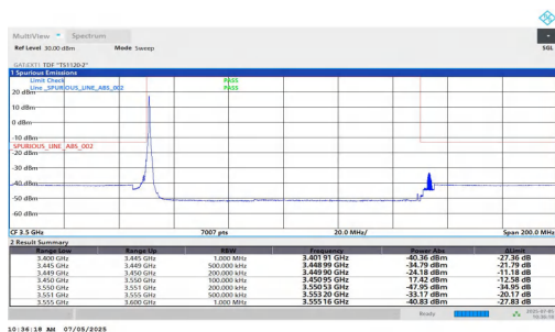
NTNV-DC_5A_n77A-PC2-30-5+100-M+L-QPSK-IDLE-DFT-BPSK- Edge 1RB Left-PASS
