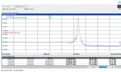
NTNV-DC_5A_n77A-PC2-30-5+30-M+L-QPSK-IDLE-DFT-QPSK-E dge_1RB_Left-PASS
