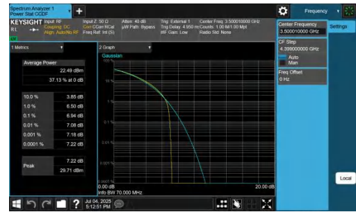
NTNV-DC_5A_n77A-PC2-30-5+70-M+M-QPSK-IDLE-CP-16QAM-O uter_Full-PASS
