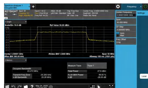
NTNV-DC_5A_n77A-PC2-30-5+25-M+M-QPSK-IDLE-CP-256QAM- Outer_Full-Ant1-PASS
