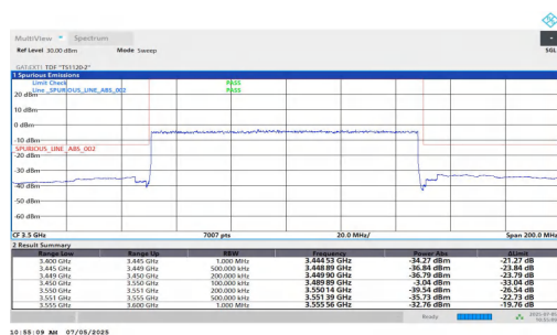
NTNV-DC_5A_n77A-PC2-30-5+100-M+L-QPSK-IDLE-DFT-QPSK- Outer Full-PASS
