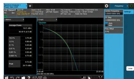
NTNV-DC_5A_n77A-PC2-30-5+40-M+M-QPSK-IDLE-CP-256QAM- Outter_Full-PASS
