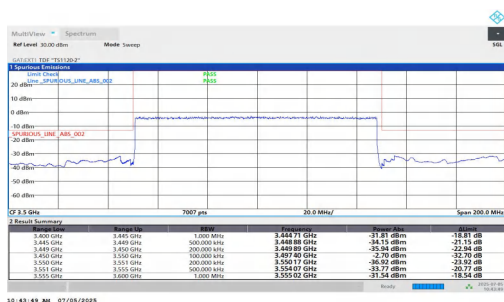
NTNV-DC_5A_n77A-PC2-30-5+100-M+L-QPSK-IDLE-DFT-BPSK- Outer Full-PASS
