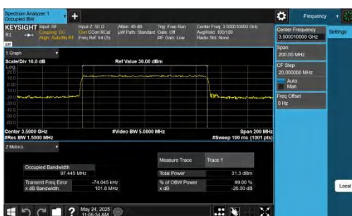
NTNV-DC_5A_n77A-PC2-30-5+100-M+M-QPSK-IDLE-CP-64QAM -Outer_Full-Ant1-PASS
