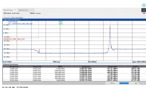
NTNV-DC_5A_n77A-PC2-30-5+100-M+L-QPSK-IDLE-DFT-QPSK- Edge 1RB Right-PASS
