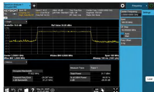
NTNV-DC_5A_n77A-PC2-30-5+80-M+M-QPSK-IDLE-CP-16QAM-O uter_Full-Ant1-PASS
