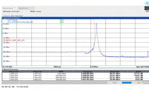
NTNV-DC_5A_n77A-PC2-30-5+30-M+L-QPSK-IDLE-DFT-BPSK-E dge_1RB_Left-PASS
