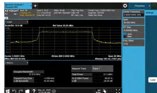
NTNV-DC_5A_n77A-PC2-30-5+40-M+M-QPSK-IDLE-CP-16QAM-O uter_Full-Ant1-PASS
