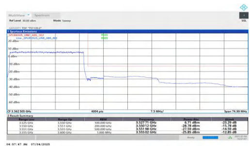
NTNV-DC_5A_n77A-PC2-30-5+25-M+H-QPSK-IDLE-DFT-QPSK-O uter_Full-PASS
