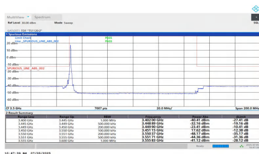
NTNV-DC_5A_n77A-PC2-30-5+100-M+L-QPSK-IDLE-DFT-QPSK- Edge 1RB Left-PASS
