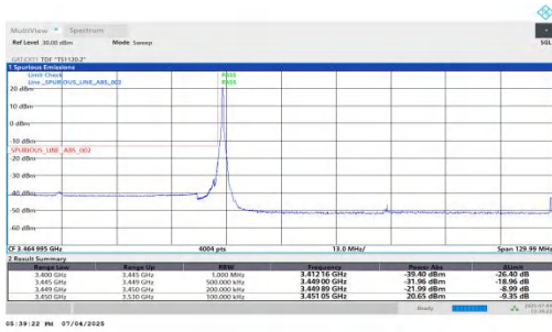
NTNV-DC_5A_n77A-PC2-30-5+80-M+L-QPSK-IDLE-DFT-BPSK-E dge_1RB_Left-PASS
