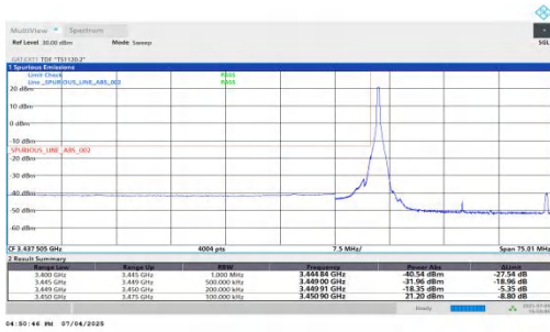
NTNV-DC_5A_n77A-PC2-30-5+25-M+L-QPSK-IDLE-DFT-BPSK-E dge_1RB_Left-PASS
