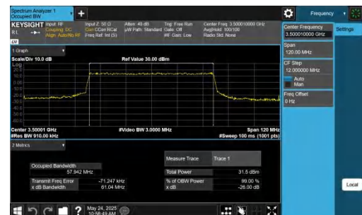
NTNV-DC_5A_n77A-PC2-30-5+60-M+M-QPSK-IDLE-CP-16QAM-O uter_Full-Ant1-PASS
