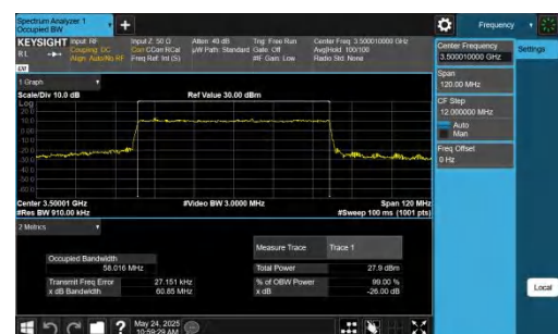
NTNV-DC_5A_n77A-PC2-30-5+60-M+M-QPSK-IDLE-CP-256QAM- Outer_Full-Ant1-PASS
