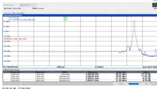
NTNV-DC_5A_n77A-PC2-30-5+10-M+L-QPSK-IDLE-DFT-QPSK-E dge_1RB_Left-PASS
