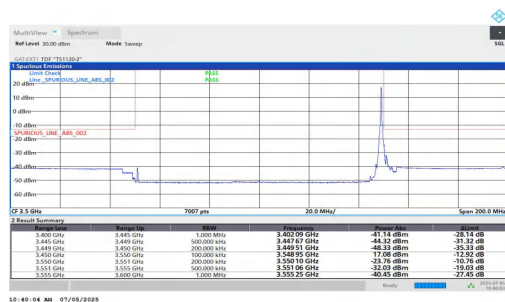
NTNV-DC_5A_n77A-PC2-30-5+100-M+L-QPSK-IDLE-DFT-BPSK- Edge 1RB Right-PASS
