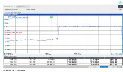
NTNV-DC_5A_n77A-PC2-30-5+60-M+L-QPSK-IDLE-DFT-BPSK-O uter_Full-PASS
