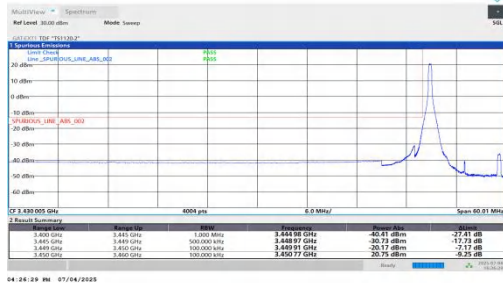
NTNV-DC_5A_n77A-PC2-30-5+10-M+L-QPSK-IDLE-DFT-BPSK-E dge_1RB_Left-PASS
