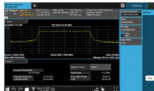
NTNV-DC_5A_n77A-PC2-30-5+25-M+M-QPSK-IDLE-CP-16QAM-O uter_Full-Ant1-PASS
