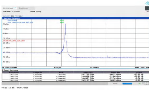
NTNV-DC_5A_n77A-PC2-30-5+70-M+L-QPSK-IDLE-DFT-BPSK-E dge_1RB_Left-PASS
