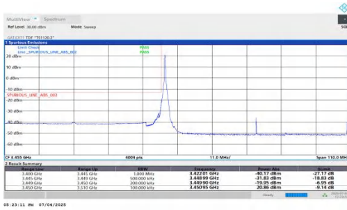
NTNV-DC_5A_n77A-PC2-30-5+60-M+L-QPSK-IDLE-DFT-BPSK-E dge_1RB_Left-PASS
