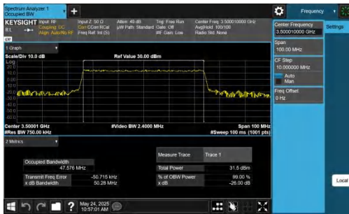
NTNV-DC_5A_n77A-PC2-30-5+50-M+M-QPSK-IDLE-CP-QPSK-O uter_Full-Ant1-PASS
