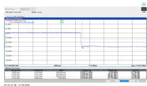
NTNV-DC_5A_n77A-PC2-30-5+60-M+H-QPSK-IDLE-DFT-QPSK-O uter_Full-PASS
