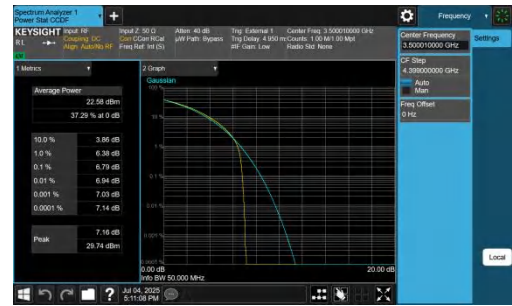
NTNV-DC_5A_n77A-PC2-30-5+50-M+M-QPSK-IDLE-CP-16QAM-O uter_Full-PASS
