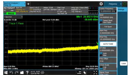
NTNV-n78(3700-3800)-PC2-30-80-L-DFT-BPSK-Inner_1RB_Left-6000 -26000-PASS
