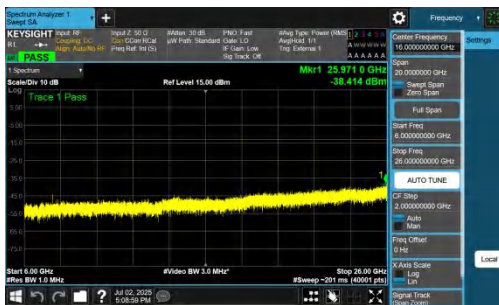
NTNV-n78(3700-3800)-PC2-30-90-L-DFT-QPSK-Inner_1RB_Right-60 00-26000-PASS
