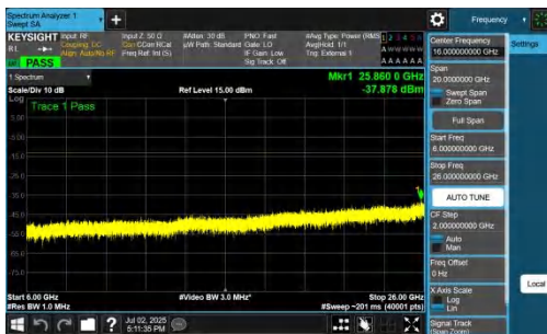
NTNV-n78(3700-3800)-PC2-30-90-H-DFT-QPSK-Inner_1RB_Right-6 000-26000-PASS
