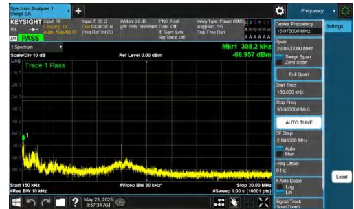
NTNV-n78(3700-3800)-PC2-30-90-H-DFT-BPSK-Inner_1RB_Left-0.15- 30-PASS
