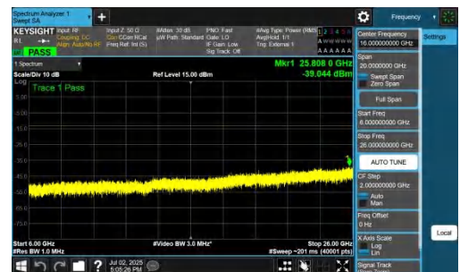
NTNV-n78(3700-3800)-PC2-30-80-M-DFT-BPSK-Inner_1RB_Left-600 0-26000-PASS
