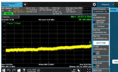
NTNV-n78(3700-3800)-PC2-30-70-H-DFT-BPSK-Inner_1RB_Right-6000-26000-PASS
