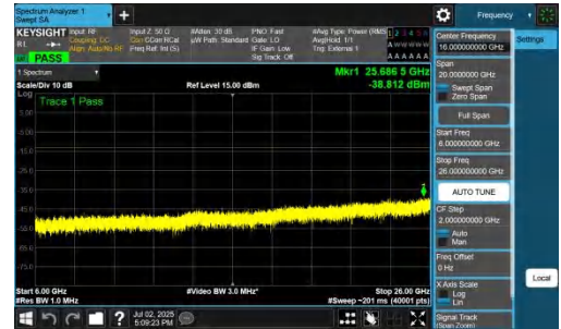
NTNV-n78(3700-3800)-PC2-30-90-M-DFT-BPSK-Inner_1RB_Left-600 0-26000-PASS
