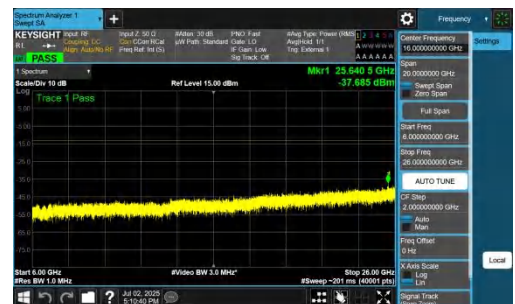
NTNV-n78(3700-3800)-PC2-30-90-H-DFT-BPSK-Inner_1RB_Left-6000 -26000-PASS
