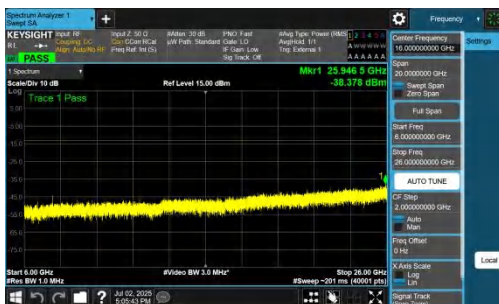
NTNV-n78(3700-3800)-PC2-30-80-M-DFT-BPSK-Inner_1RB_Right-6000-26000-PASS
