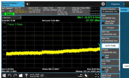
NTNV-n78(3700-3800)-PC2-30-80-L-DFT-BPSK-Inner_1RB_Right-6000-26000-PASS
