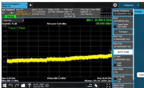
NTNV-n78(3700-3800)-PC2-30-70-H-DFT-QPSK-Inner_1RB_Right-6 000-26000-PASS
