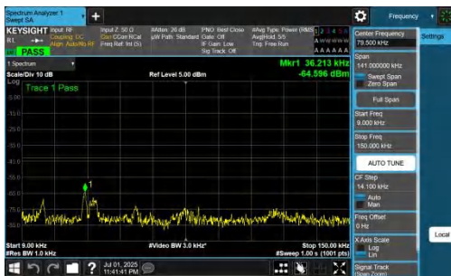
NTNV-n78(3700-3800)-PC2-30-100-L-DFT-QPSK-Inner_1RB_Left-0.009-0.15-PASS
