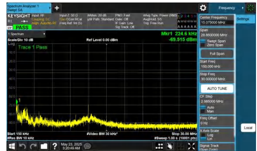
NTNV-n78(3700-3800)-PC2-30-70-H-DFT-BPSK-Inner_1RB_Left-0.15- 30-PASS
