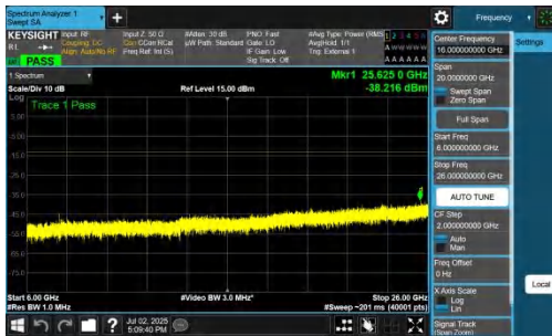
NTNV-n78(3700-3800)-PC2-30-90-M-DFT-BPSK-Inner_1RB_Right-6000-26000-PASS
