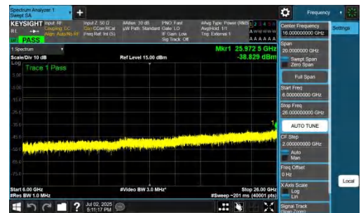
NTVN-n78(3700-3800)-PC2-30-90-H-DFT-QPSK-Inner_1RB_Left-6000-0-26000-PASS
