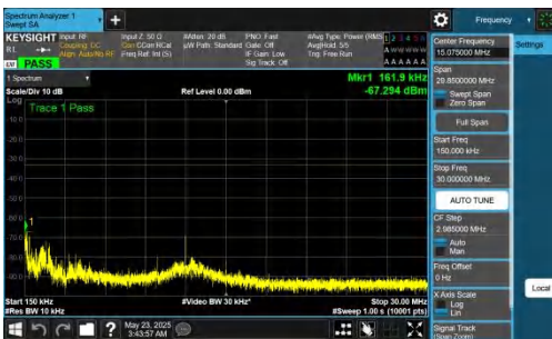
NTNV-n78(3700-3800)-PC2-30-80-H-DFT-QPSK-Inner_1RB_Right-0. 15-30-PASS
