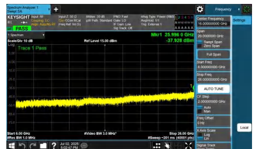
NTNV-n78(3700-3800)-PC2-30-70-H-DFT-BPSK-Inner_1RB_Left-6000 -26000-PASS
