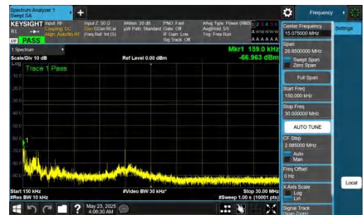
NTNV-n78(3700-3800)-PC2-30-100-L-DFT-QPSK-Inner_1RB_Left-0.15-5-30-PASS
