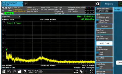
NTVN-n78(3700-3800)-PC2-30-90-L-DFT-BPSK-Inner_1RB_Right-0.15-30-PASS
