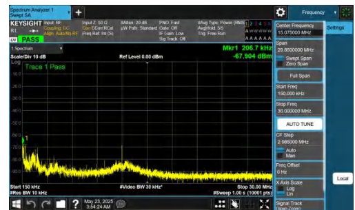
NTNV-n78(3700-3800)-PC2-30-90-M-DFT-QPSK-Inner_1RB_Left-0.15-0.30-PASS
