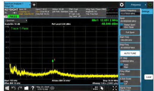
NTNV-n78(3700-3800)-PC2-30-80-M-DFT-BPSK-Inner_1RB_Left-0.15 -30-PASS
