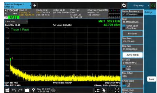
NTNV-n78(3700-3800)-PC2-30-80-L-DFT-QPSK-Inner_1RB_Left-0.15-30-PASS
