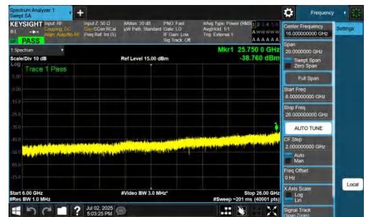
NTNV-n78(3700-3800)-PC2-30-70-H-DFT-QPSK-Inner_1RB_Left-6000-0-26000-PASS
