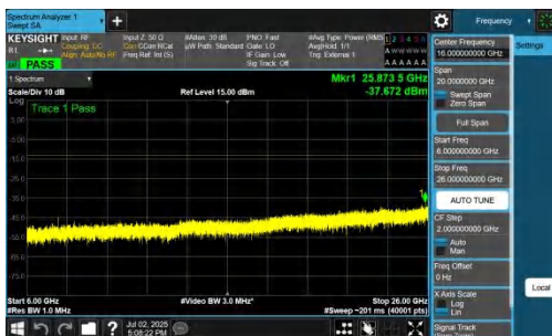
NTVN-n78(3700-3800)-PC2-30-90-L-DFT-BPSK-Inner_1RB_Right-6000-26000-PASS
