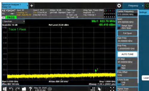
NTNV-n78(3700-3800)-PC2-30-80-L-DFT-QPSK-Inner_1RB_Left-30-1000-PASS
