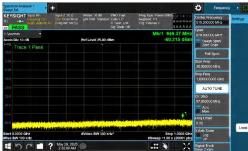
NTNV-n78(3450-3550)-PC2-30-80-M-DFT-QPSK-Inner_1RB_Left-30-1000-PASS
