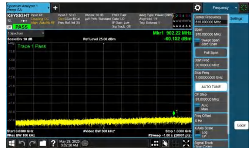
NTNV-n78(3450-3550)-PC2-30-90-L-DFT-BPSK-Inner_1RB_Right-30-1000-PASS
