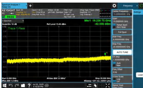
NTNV-n78(3450-3550)-PC2-30-80-M-DFT-QPSK-Inner_1RB_Right-6 000-20000-PASS
