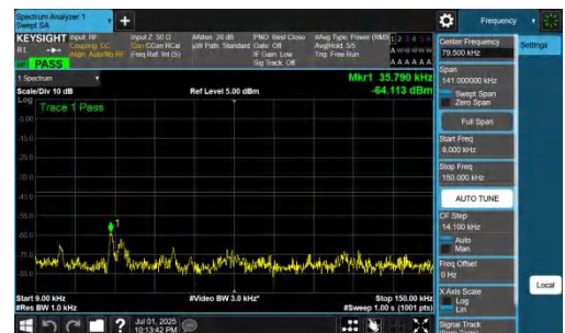
NTNV-n78(3450-3550)-PC2-30-80-M-DFT-QPSK-Inner_1RB_Right-0.009-0.15-PASS
