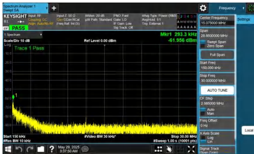
NTNV-n78(3450-3550)-PC2-30-90-H-DFT-BPSK-Inner_1RB_Right-0.15-30-PASS
