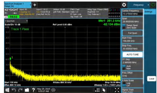
NTNV-n78(3450-3550)-PC2-30-90-H-DFT-BPSK-Inner_1RB_Left-0.15- 30-PASS
