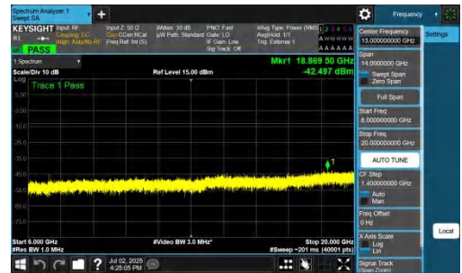
NTNV-n78(3450-3550)-PC2-30-100-L-DFT-BPSK-Inner_1RB_Left-600 0-20000-PASS
