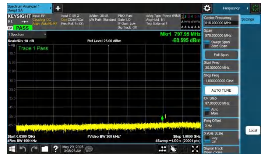
NTNV-n78(3450-3550)-PC2-30-90-H-DFT-BPSK-Inner_1RB_Right-30-1000-PASS
