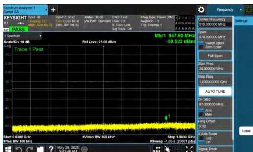
NTVN-n78(3450-3550)-PC2-30-90-H-DFT-QPSK-Inner_1RB_Left-30-1000-PASS
