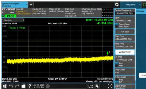
NTNV-n78(3450-3550)-PC2-30-90-M-DFT-BPSK-Inner_1RB_Right-6000-20000-PASS
