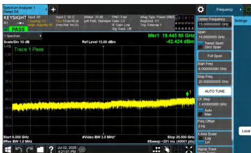
NTNV-n78(3450-3550)-PC2-30-90-L-DFT-BPSK-Inner_1RB_Right-6000-20000-PASS
