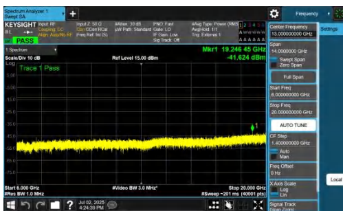
NTNV-n78(3450-3550)-PC2-30-90-H-DFT-QPSK-Inner_1RB_Right-6 000-20000-PASS
