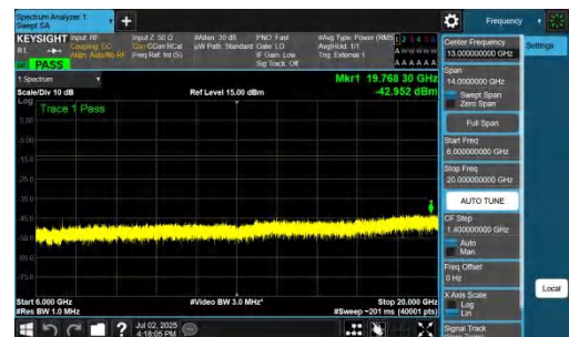
NTNV-n78(3450-3550)-PC2-30-80-M-DFT-BPSK-Inner_1RB_Left-600 0-20000-PASS
