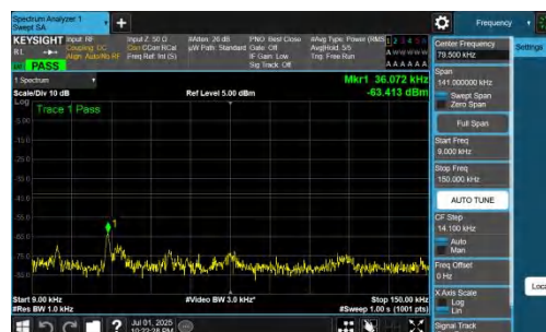
NTVN-n78(3450-3550)-PC2-30-90-H-DFT-QPSK-Inner_1RB_Right-0.009-0.15-PASS
