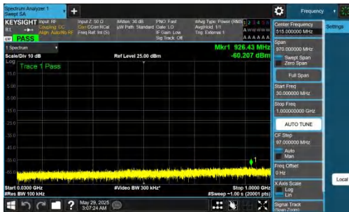
NTNV-n78(3450-3550)-PC2-30-90-L-DFT-QPSK-Inner_1RB_Left-30-1000-PASS
