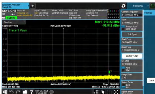
NTNV-n78(3450-3550)-PC2-30-80-H-DFT-QPSK-Inner_1RB_Left-30-1000-PASS
