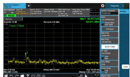
NTNV-n78(3450-3550)-PC2-30-90-H-DFT-BPSK-Inner_1RB_Right-0.0 09-0.15-PASS
