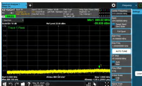
NTNV-n78(3450-3550)-PC2-30-90-M-DFT-QPSK-Inner_1RB_Left-30-1000-PASS
