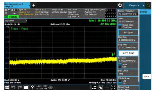
NTNV-n78(3450-3550)-PC2-30-90-L-DFT-QPSK-Inner_1RB_Left-6000-20000-PASS
