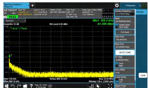
NTNV-n78(3450-3550)-PC2-30-90-M-DFT-BPSK-Inner_1RB_Left-0.15 -30-PASS
