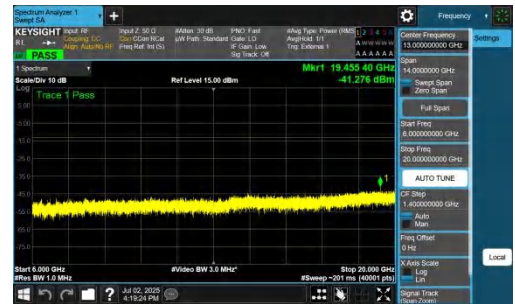
NTNV-n78(3450-3550)-PC2-30-80-H-DFT-BPSK-Inner_1RB_Left-6000 -20000-PASS
