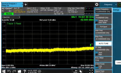
NTNV-n78(3450-3550)-PC2-30-80-M-DFT-BPSK-Inner_1RB_Right-6000-20000-PASS
