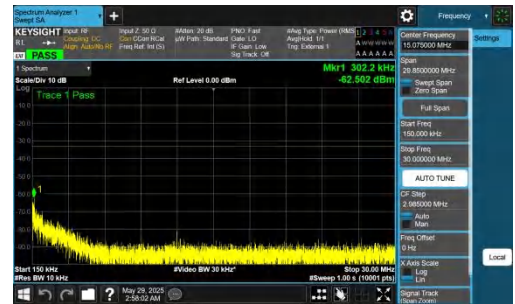
NTNV-n78(3450-3550)-PC2-30-90-L-DFT-BPSK-Inner_1RB_Left-0.15- 30-PASS
