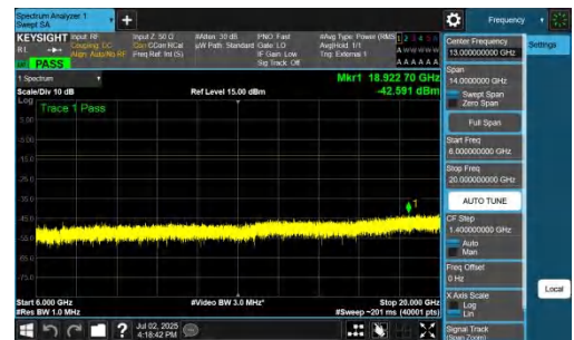
NTNV-n78(3450-3550)-PC2-30-80-M-DFT-QPSK-Inner_1RB_Left-6000-20000-PASS
