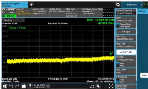
NTNV-n78(3450-3550)-PC2-30-80-H-DFT-BPSK-Inner_1RB_Right-6000-20000-PASS
